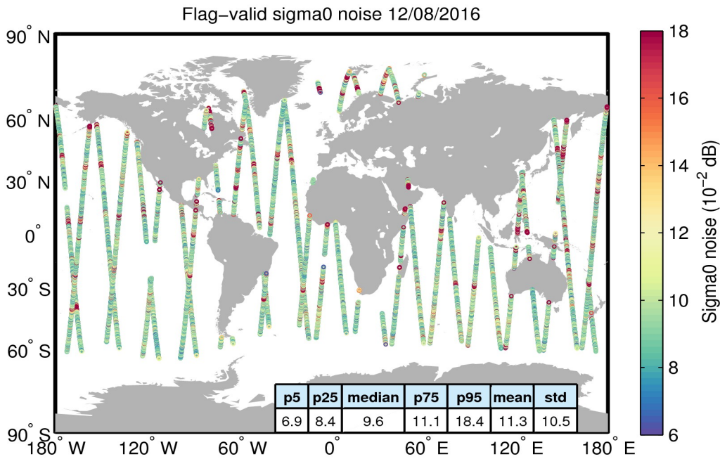
Figure 26. Geographical distribution of flag-valid 20-Hz sigma0 measurement noise over oceans and lakes for 12/08/2016. The statistical values shown in the table refer to the sigma0 noise and are calculated over all measurements shown in the figure.
