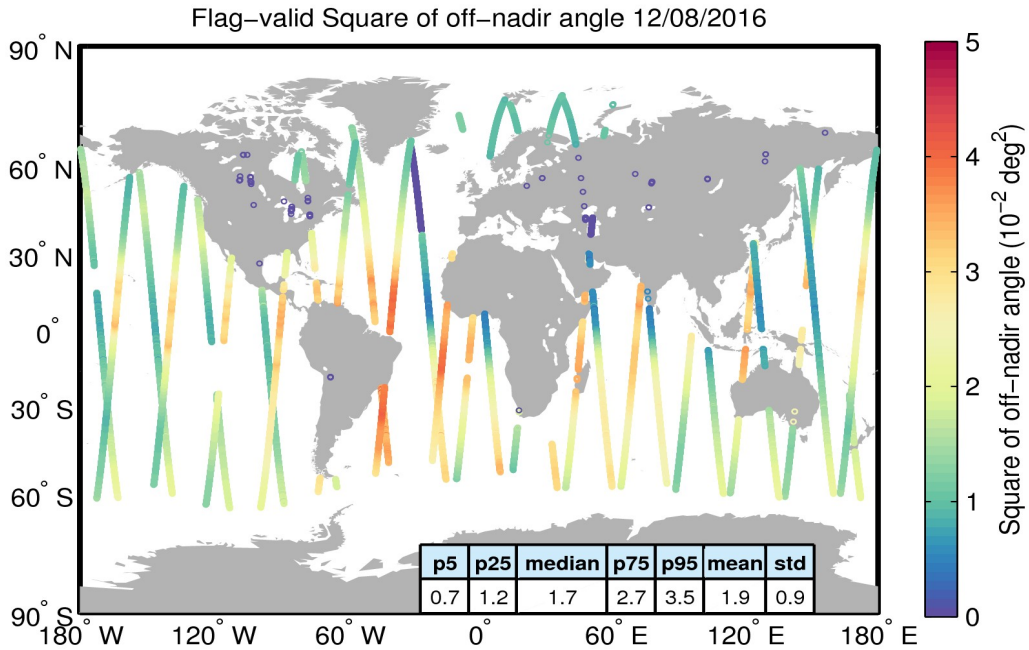
Figure 37. Geographical distribution of flag-valid mispointing data over oceans and lakes for 12/08/2016. The statistical values shown in the table refer to the mispointing in 10^{-2} deg 2 and are calculated over all measurements shown in the figure.
