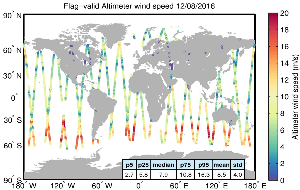
Figure 31. Geographical distribution of flag-valid wind data over oceans and lakes for 12/08/2016. The statistical values shown in the table refer to the wind in m/s and are calculated over all measurements shown in the figure.
