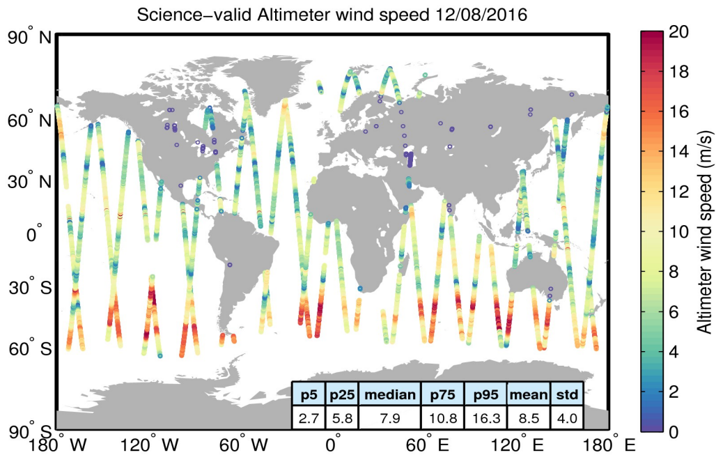
Figure 34. Geographical distribution of science-valid wind data over oceans and lakes for 12/08/2016. The statistical values shown in the table refer to the wind in m/s and are calculated over all measurements shown in the figure. Gray circles denote records that have been rejected based on the editing criteria described in Table 5.
