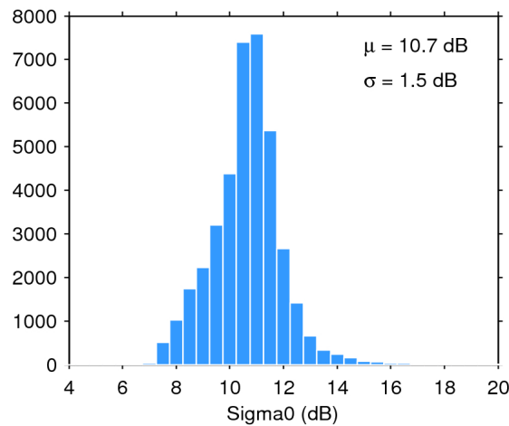
Figure 28. Histogram of science-valid sigma0 over oceans and lakes for 12/08/2016. The mean ( \mu ) and standard deviation ( \sigma ) are also shown. Note that values outside [4 20] dB are excluded from the histogram for the sake of readability but not from the computation of \mu and \sigma .
