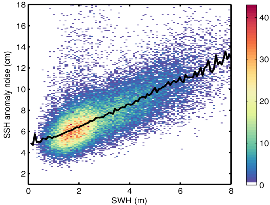
Figure 9. 2D histogram showing flag-valid SSH anomaly noise as a function of SWH for 12/08/2016. The black line denotes the median SSH anomaly noise as a function of SWH.
