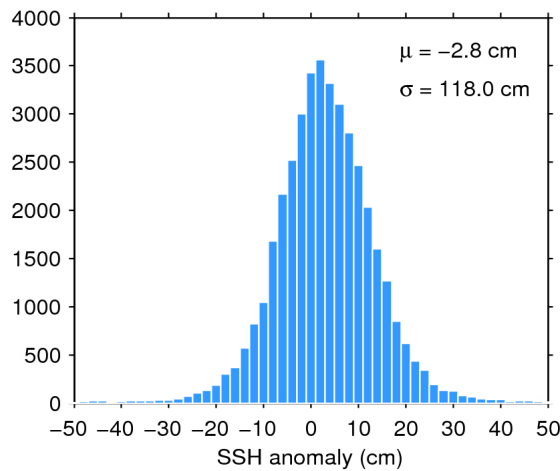
Figure 7. Histogram of flag-valid SSH anomaly over oceans and lakes for 12/08/2016. The mean ( \mu ) and standard deviation ( \sigma ) are also shown. Note that values outside [-50 50] cm are excluded from the histogram for the sake of readability but not from the computation of \mu and \sigma .
