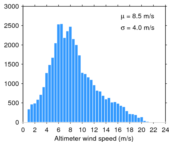
Figure 35. Histogram of science-valid wind over oceans and lakes for 12/08/2016. The mean ( \mu ) and standard deviation ( \sigma ) are also shown. Note that values larger than 24 m/s are excluded from the histogram for the sake of readability but not from the computation of \mu and \sigma .
