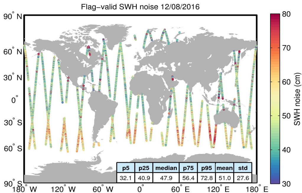
Figure 18. Geographical distribution of flag-valid 20-Hz SWH measurement noise over oceans and lakes for 12/08/2016. The statistical values shown in the table refer to the SWH noise and are calculated over all measurements shown in the figure.
