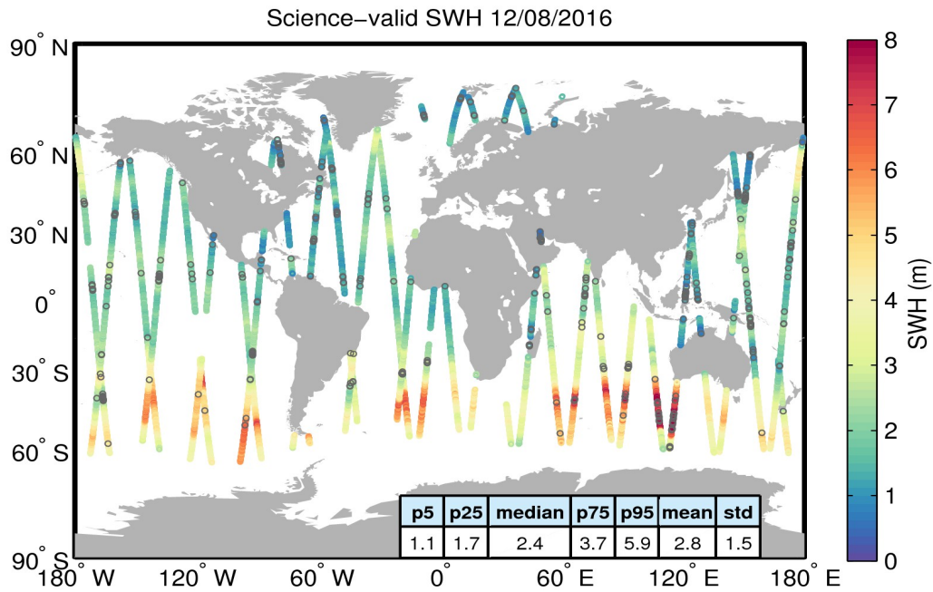
Figure 19. Geographical distribution of science-valid SWH data over oceans and lakes for 12/08/2016. The statistical values shown in the table refer to the SWH in m and are calculated over all measurements shown in the figure. Gray circles denote records that have been rejected based on the editing criteria described in Table 3.
