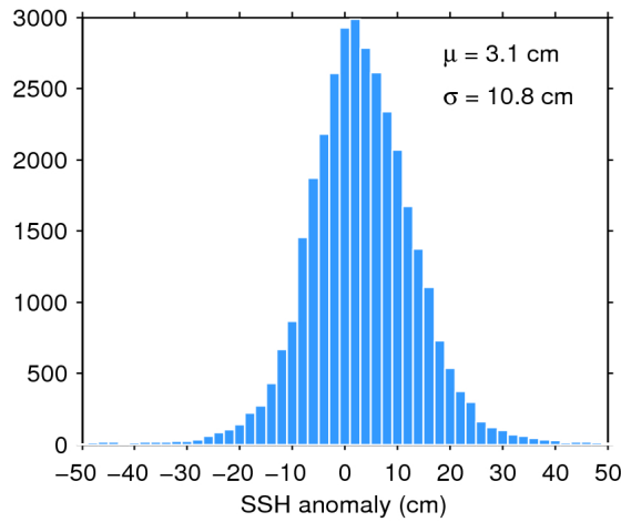
Figure 11. Histogram of science-valid SSH anomaly over oceans and lakes for 12/08/2016. The mean ( \mu ) and standard deviation ( \sigma ) are also shown. Note that values outside [-50 50] cm are excluded from the histogram for the sake of readability but not from the computation of \mu and \sigma .
