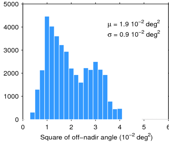
Figure 39. Histogram of flag-valid mispointing over oceans and lakes for 12/08/2016. The mean ( \mu ) and standard deviation ( \sigma ) are also shown. Note that values larger than 6 \cdot 10^{-2} \text{ deg}^2 are excluded from the histogram for the sake of readability but not from the computation of \mu and \sigma .
