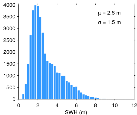
Figure 20. Histogram of science-valid SWH over oceans and lakes for 12/08/2016. The mean ( \mu ) and standard deviation ( \sigma ) are also shown. Note that values larger than 12 m are excluded from the histogram for the sake of readability but not from the computation of \mu and \sigma .
