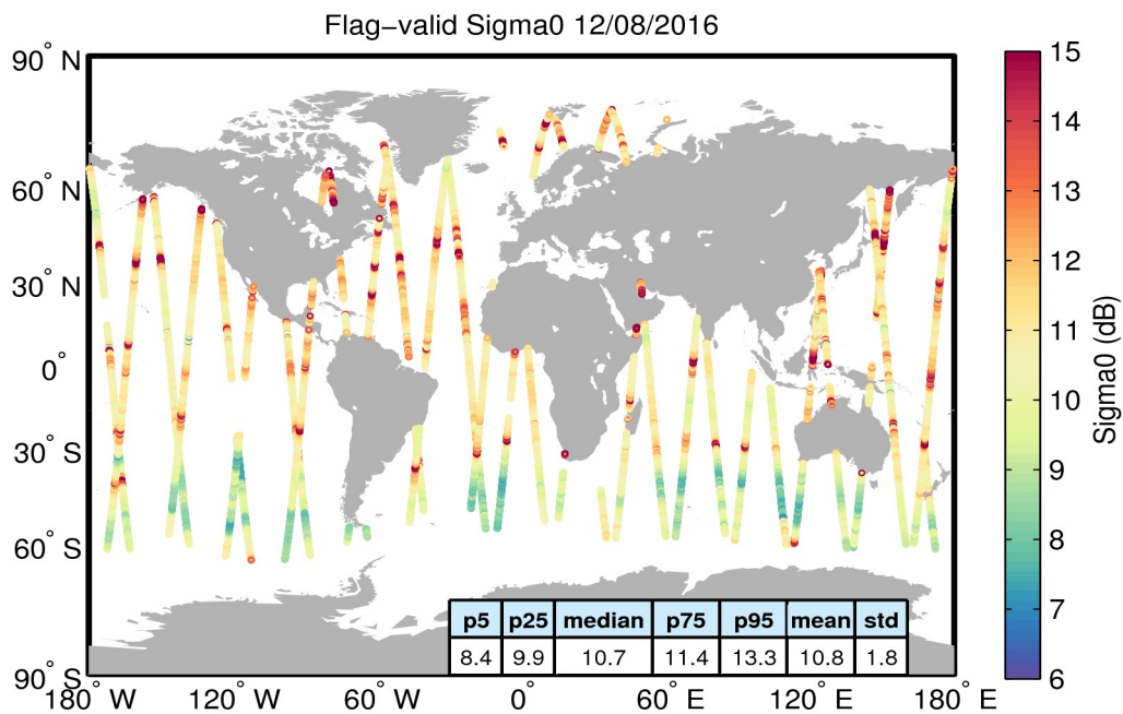
Figure 23. Geographical distribution of flag-valid sigma0 data over oceans and lakes for 12/08/2016. The statistical values shown in the table refer to the sigma0 in dB and are calculated over all measurements shown in the figure.
