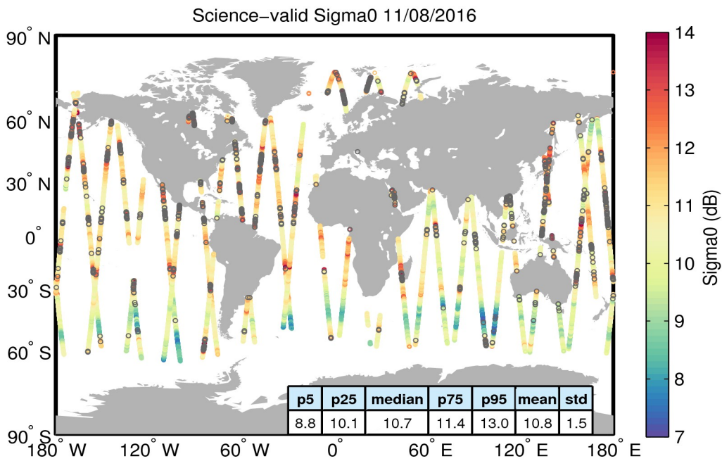
Figure 27. Geographical distribution of science-valid sigma0 data over oceans and lakes for 11/08/2016. The statistical values shown in the table refer to the sigma0 in dB and are calculated over all measurements shown in the figure. Gray circles denote records that have been rejected based on the editing criteria described in Table 4.
