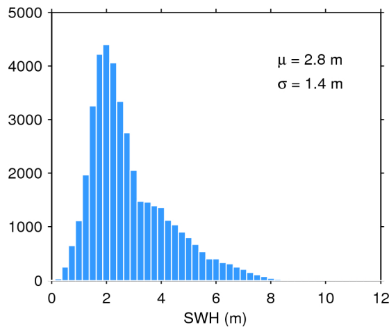
Figure 20. Histogram of science-valid SWH over oceans and lakes for 11/08/2016. The mean ( \mu ) and standard deviation ( \sigma ) are also shown. Note that values larger than 12 m are excluded from the histogram for the sake of readability but not from the computation of \mu and \sigma .
