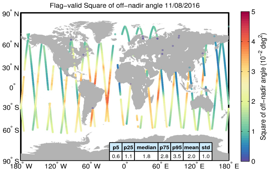
Figure 37. Geographical distribution of flag-valid mispointing data over oceans and lakes for 11/08/2016. The statistical values shown in the table refer to the mispointing in 10^{-2} deg 2 and are calculated over all measurements shown in the figure.
