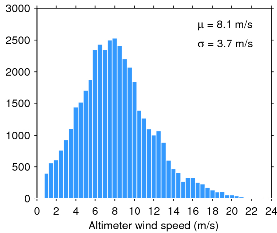
Figure 33. Histogram of flag-valid wind over oceans and lakes for 11/08/2016. The mean ( \mu ) and standard deviation ( \sigma ) are also shown. Note that values larger than 24 m/s are excluded from the histogram for the sake of readability but not from the computation of \mu and \sigma .
