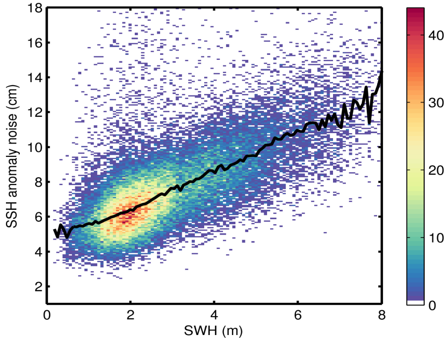
Figure 9. 2D histogram showing flag-valid SSH anomaly noise as a function of SWH for 11/08/2016. The black line denotes the median SSH anomaly noise as a function of SWH.
