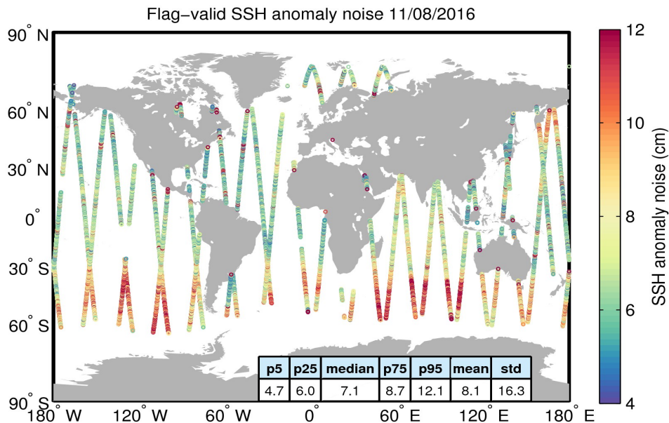
Figure 8. Geographical distribution of flag-valid 20-Hz SSH anomaly measurement noise over oceans and lakes for 11/08/2016. The statistical values shown in the table refer to the SSH anomaly noise and are calculated over all measurements shown in the figure.
