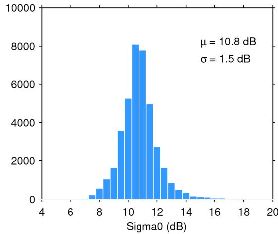
Figure 28. Histogram of science-valid sigma0 over oceans and lakes for 11/08/2016. The mean ( \mu ) and standard deviation ( \sigma ) are also shown. Note that values outside [4 20] dB are excluded from the histogram for the sake of readability but not from the computation of \mu and \sigma .
