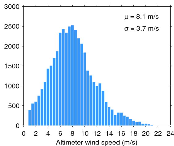
Figure 35. Histogram of science-valid wind over oceans and lakes for 11/08/2016. The mean ( \mu ) and standard deviation ( \sigma ) are also shown. Note that values larger than 24 m/s are excluded from the histogram for the sake of readability but not from the computation of \mu and \sigma .
