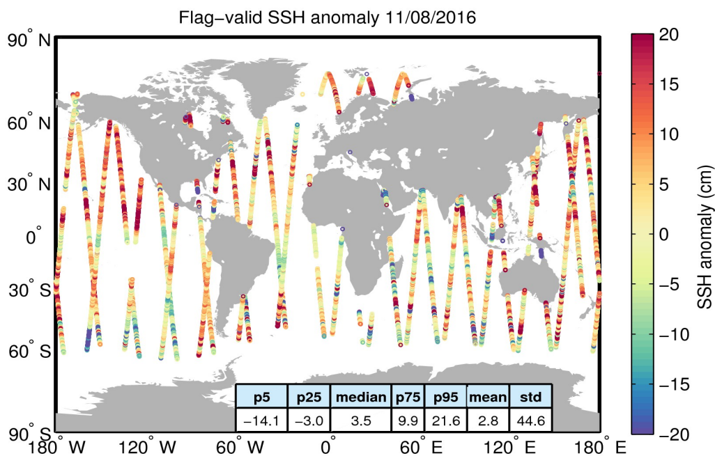
Figure 5. Geographical distribution of flag-valid 1-Hz SSH anomaly data over oceans and lakes for 11/08/2016. The statistical values shown in the table refer to the SSH anomaly in cm and are calculated over all measurements shown in the figure.
