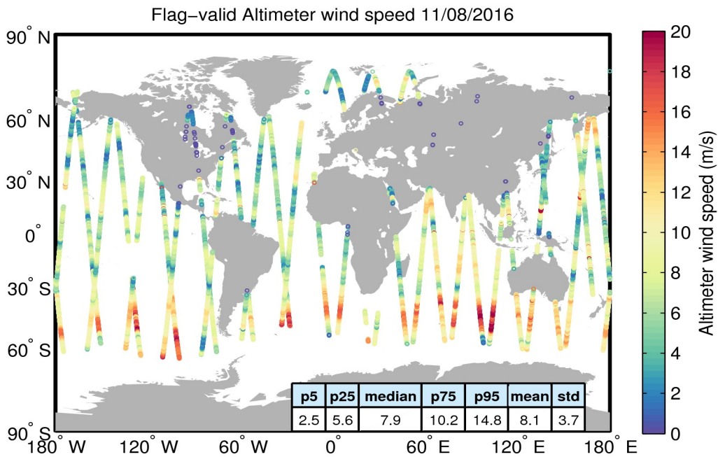
Figure 31. Geographical distribution of flag-valid wind data over oceans and lakes for 11/08/2016. The statistical values shown in the table refer to the wind in m/s and are calculated over all measurements shown in the figure.
