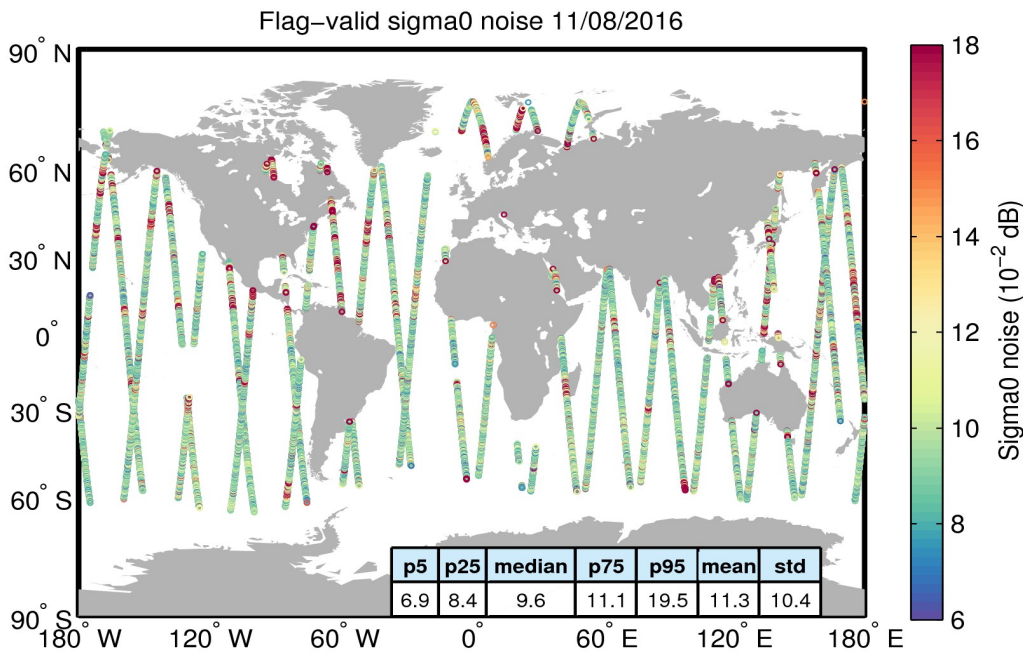
Figure 26. Geographical distribution of flag-valid 20-Hz sigma0 measurement noise over oceans and lakes for 11/08/2016. The statistical values shown in the table refer to the sigma0 noise and are calculated over all measurements shown in the figure.
