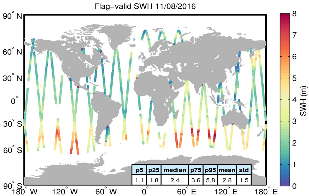
Figure 15. Geographical distribution of flag-valid SWH data over oceans and lakes for 11/08/2016. The statistical values shown in the table refer to the SWH in m and are calculated over all measurements shown in the figure.
