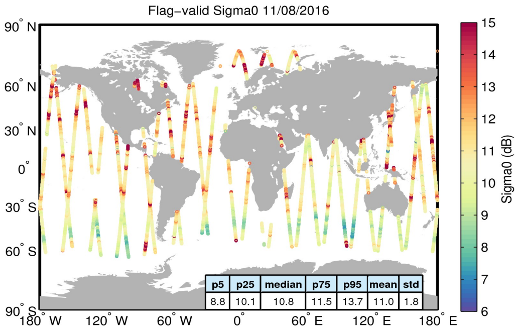
Figure 23. Geographical distribution of flag-valid sigma0 data over oceans and lakes for 11/08/2016. The statistical values shown in the table refer to the sigma0 in dB and are calculated over all measurements shown in the figure.
