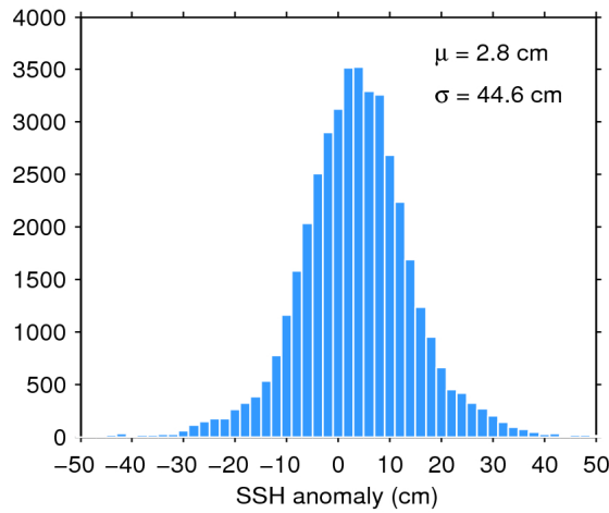
Figure 7. Histogram of flag-valid SSH anomaly over oceans and lakes for 11/08/2016. The mean ( \mu ) and standard deviation ( \sigma ) are also shown. Note that values outside [-50 50] cm are excluded from the histogram for the sake of readability but not from the computation of \mu and \sigma .
