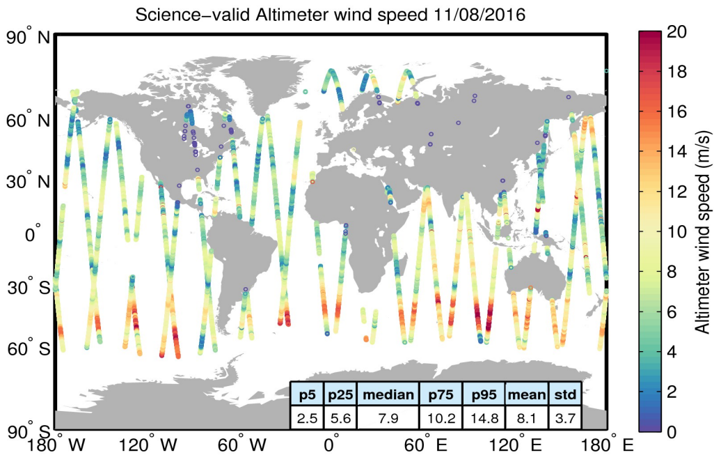
Figure 34. Geographical distribution of science-valid wind data over oceans and lakes for 11/08/2016. The statistical values shown in the table refer to the wind in m/s and are calculated over all measurements shown in the figure. Gray circles denote records that have been rejected based on the editing criteria described in Table 5.
