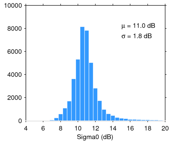
Figure 25. Histogram of flag-valid sigma0 over oceans and lakes for 11/08/2016. The mean ( \mu ) and standard deviation ( \sigma ) are also shown. Note that values outside [4 20] dB are excluded from the histogram for the sake of readability but not from the computation of \mu and \sigma .
