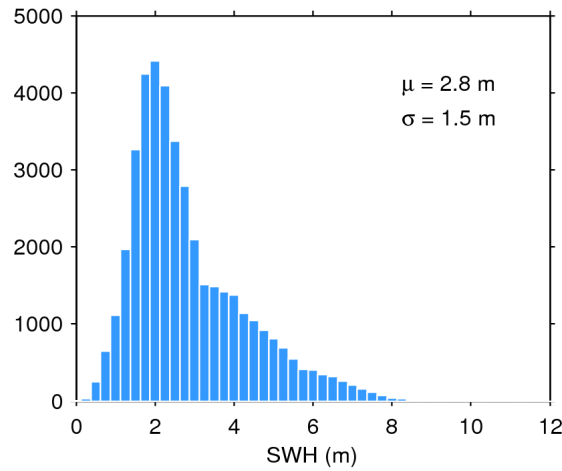
Figure 17. Histogram of flag-valid SWH over oceans and lakes for 11/08/2016. The mean ( \mu ) and standard deviation ( \sigma ) are also shown. Note that values larger than 12 m are excluded from the histogram for the sake of readability but not from the computation of \mu and \sigma .
