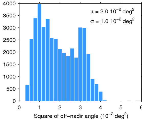
Figure 39. Histogram of flag-valid mispointing over oceans and lakes for 11/08/2016. The mean ( \mu ) and standard deviation ( \sigma ) are also shown. Note that values larger than 6 \cdot 10^{-2} \text{ deg}^2 are excluded from the histogram for the sake of readability but not from the computation of \mu and \sigma .
