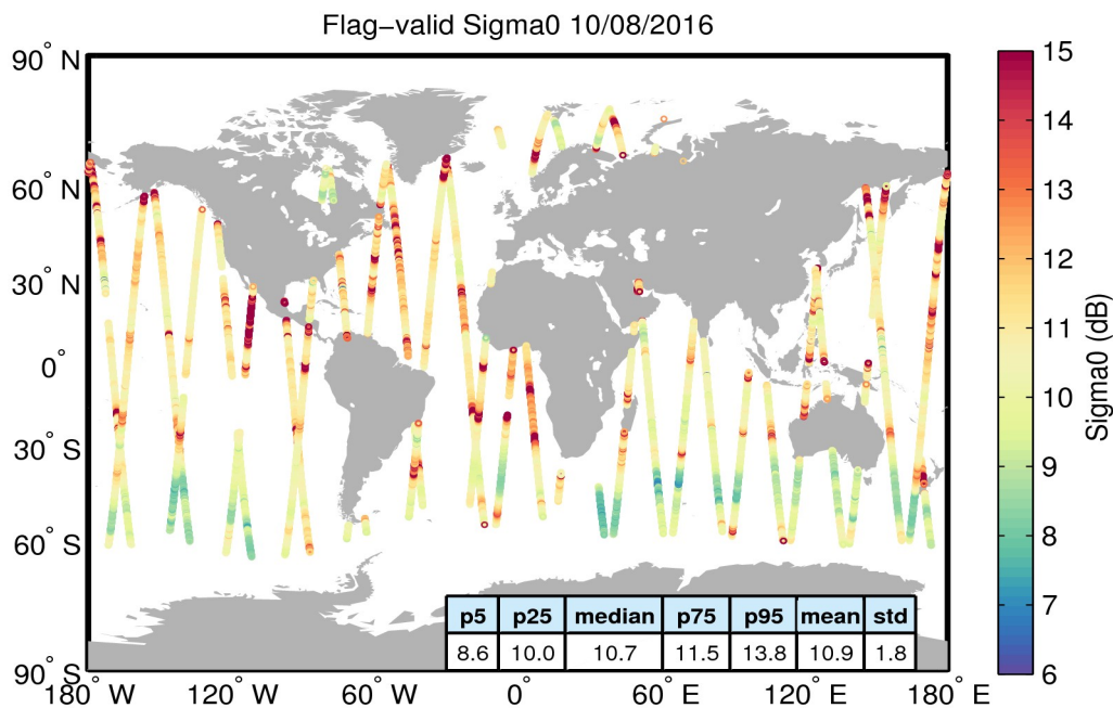
Figure 23. Geographical distribution of flag-valid sigma0 data over oceans and lakes for 10/08/2016. The statistical values shown in the table refer to the sigma0 in dB and are calculated over all measurements shown in the figure.
