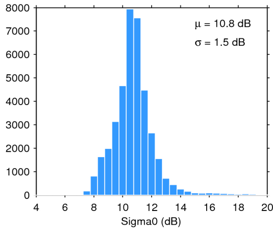
Figure 28. Histogram of science-valid sigma0 over oceans and lakes for 10/08/2016. The mean ( \mu ) and standard deviation ( \sigma ) are also shown. Note that values outside [4 20] dB are excluded from the histogram for the sake of readability but not from the computation of \mu and \sigma .
