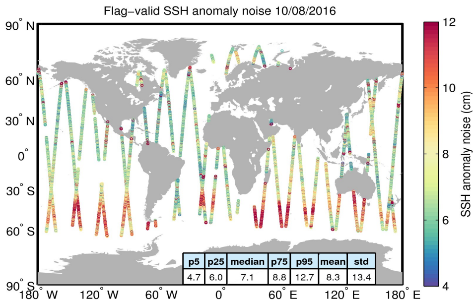
Figure 8. Geographical distribution of flag-valid 20-Hz SSH anomaly measurement noise over oceans and lakes for 10/08/2016. The statistical values shown in the table refer to the SSH anomaly noise and are calculated over all measurements shown in the figure.
