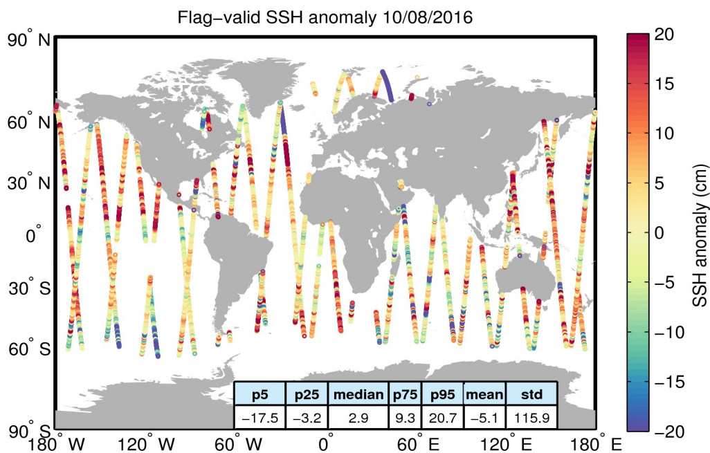
Figure 5. Geographical distribution of flag-valid 1-Hz SSH anomaly data over oceans and lakes for 10/08/2016. The statistical values shown in the table refer to the SSH anomaly in cm and are calculated over all measurements shown in the figure.
