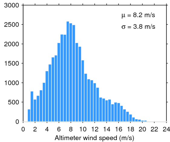
Figure 33. Histogram of flag-valid wind over oceans and lakes for 10/08/2016. The mean ( \mu ) and standard deviation ( \sigma ) are also shown. Note that values larger than 24 m/s are excluded from the histogram for the sake of readability but not from the computation of \mu and \sigma .
