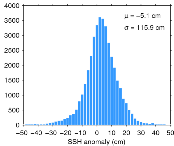
Figure 7. Histogram of flag-valid SSH anomaly over oceans and lakes for 10/08/2016. The mean ( \mu ) and standard deviation ( \sigma ) are also shown. Note that values outside [-50 50] cm are excluded from the histogram for the sake of readability but not from the computation of \mu and \sigma .
