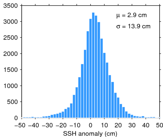
Figure 11. Histogram of science-valid SSH anomaly over oceans and lakes for 10/08/2016. The mean ( \mu ) and standard deviation ( \sigma ) are also shown. Note that values outside [-50 50] cm are excluded from the histogram for the sake of readability but not from the computation of \mu and \sigma .
