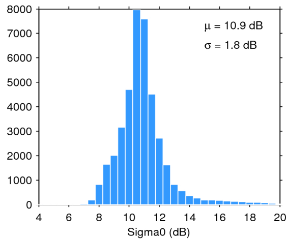
Figure 25. Histogram of flag-valid sigma0 over oceans and lakes for 10/08/2016. The mean ( \mu ) and standard deviation ( \sigma ) are also shown. Note that values outside [4 20] dB are excluded from the histogram for the sake of readability but not from the computation of \mu and \sigma .
