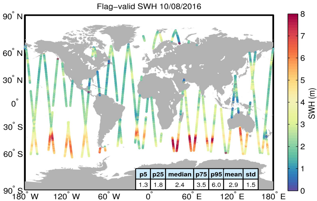
Figure 15. Geographical distribution of flag-valid SWH data over oceans and lakes for 10/08/2016. The statistical values shown in the table refer to the SWH in m and are calculated over all measurements shown in the figure.
