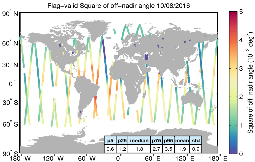
Figure 37. Geographical distribution of flag-valid mispointing data over oceans and lakes for 10/08/2016. The statistical values shown in the table refer to the mispointing in 10^{-2} deg 2 and are calculated over all measurements shown in the figure.
