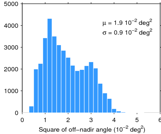
Figure 39. Histogram of flag-valid mispointing over oceans and lakes for 10/08/2016. The mean ( \mu ) and standard deviation ( \sigma ) are also shown. Note that values larger than 6 \cdot 10^{-2} \text{ deg}^2 are excluded from the histogram for the sake of readability but not from the computation of \mu and \sigma .
