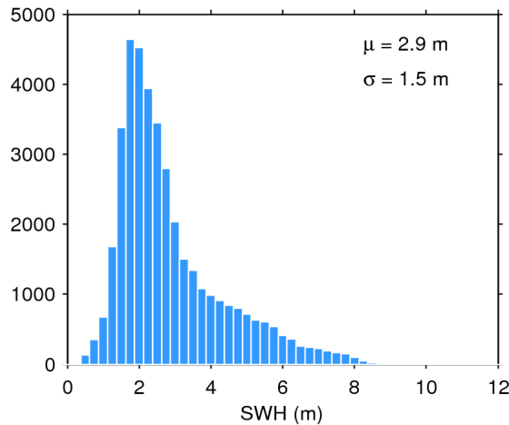
Figure 20. Histogram of science-valid SWH over oceans and lakes for 10/08/2016. The mean ( \mu ) and standard deviation ( \sigma ) are also shown. Note that values larger than 12 m are excluded from the histogram for the sake of readability but not from the computation of \mu and \sigma .
