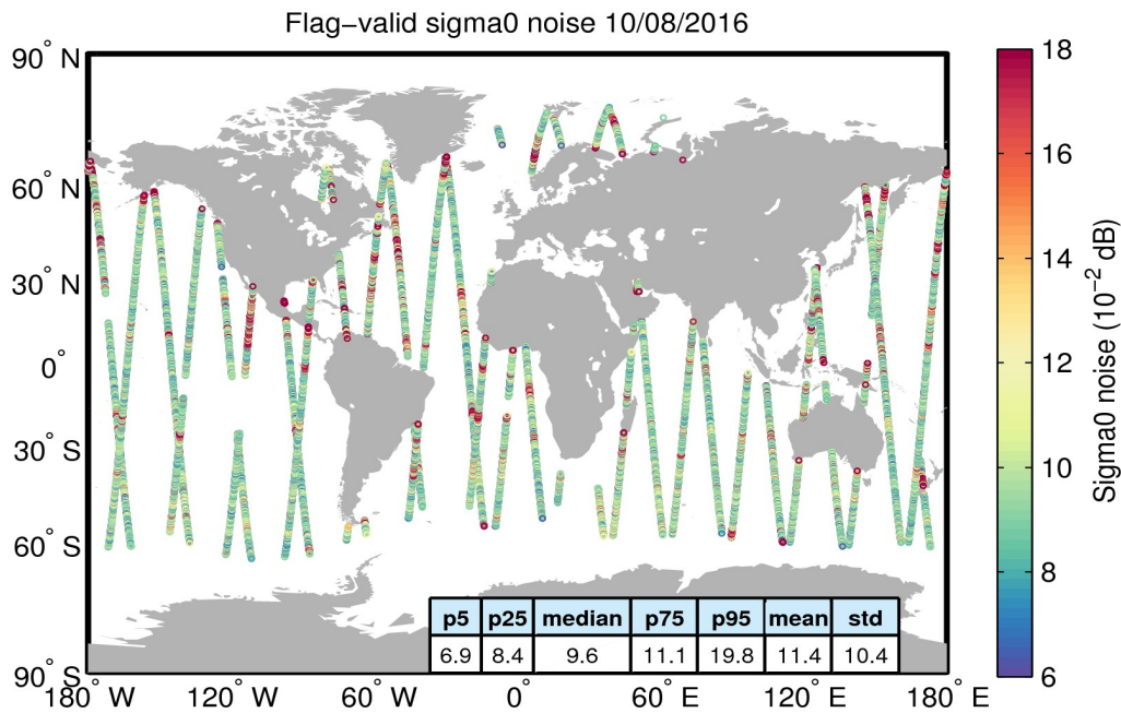
Figure 26. Geographical distribution of flag-valid 20-Hz sigma0 measurement noise over oceans and lakes for 10/08/2016. The statistical values shown in the table refer to the sigma0 noise and are calculated over all measurements shown in the figure.
