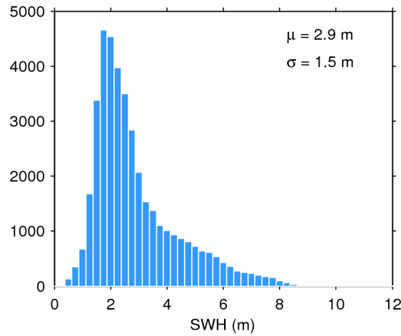
Figure 17. Histogram of flag-valid SWH over oceans and lakes for 10/08/2016. The mean ( \mu ) and standard deviation ( \sigma ) are also shown. Note that values larger than 12 m are excluded from the histogram for the sake of readability but not from the computation of \mu and \sigma .
