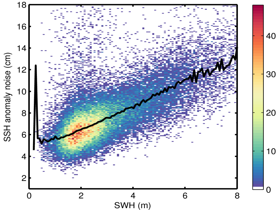
Figure 9. 2D histogram showing flag-valid SSH anomaly noise as a function of SWH for 10/08/2016. The black line denotes the median SSH anomaly noise as a function of SWH.
