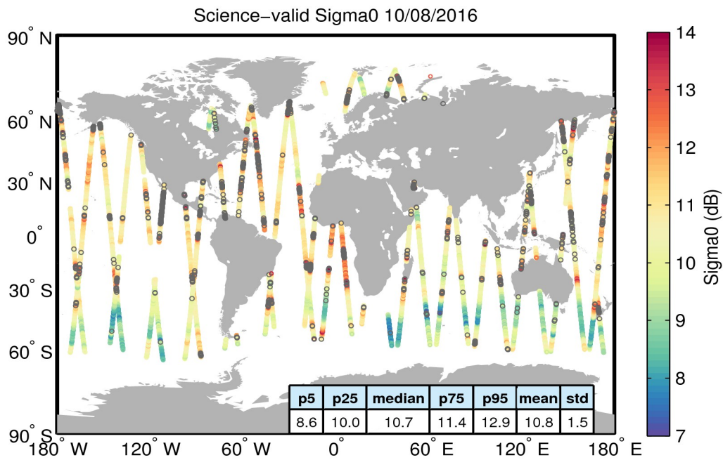
Figure 27. Geographical distribution of science-valid sigma0 data over oceans and lakes for 10/08/2016. The statistical values shown in the table refer to the sigma0 in dB and are calculated over all measurements shown in the figure. Gray circles denote records that have been rejected based on the editing criteria described in Table 4.
