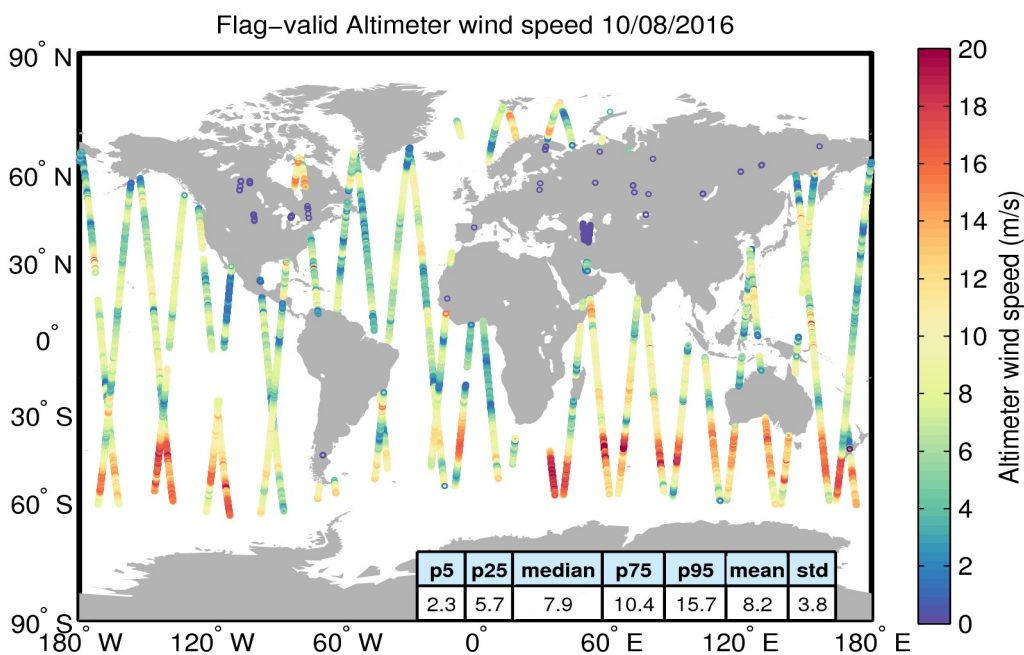
Figure 31. Geographical distribution of flag-valid wind data over oceans and lakes for 10/08/2016. The statistical values shown in the table refer to the wind in m/s and are calculated over all measurements shown in the figure.
