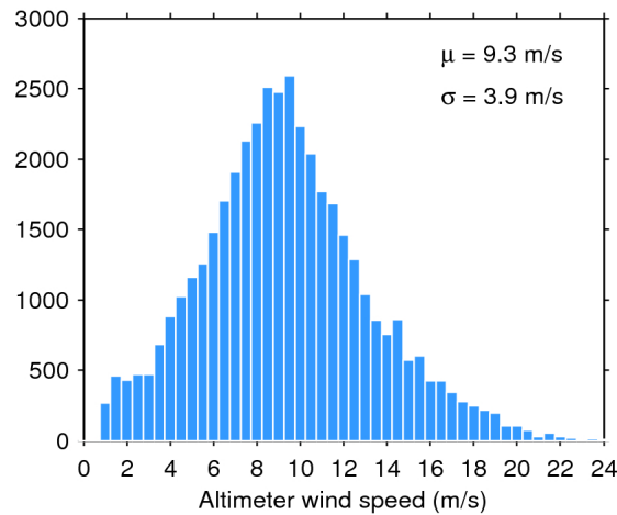
Figure 33. Histogram of flag-valid wind over oceans and lakes for 09/08/2016. The mean ( \mu ) and standard deviation ( \sigma ) are also shown. Note that values larger than 24 m/s are excluded from the histogram for the sake of readability but not from the computation of \mu and \sigma .
