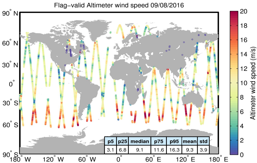
Figure 31. Geographical distribution of flag-valid wind data over oceans and lakes for 09/08/2016. The statistical values shown in the table refer to the wind in m/s and are calculated over all measurements shown in the figure.
