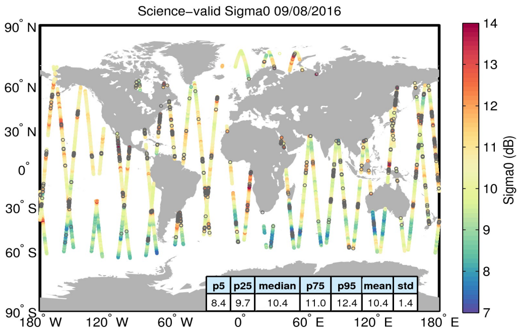
Figure 27. Geographical distribution of science-valid sigma0 data over oceans and lakes for 09/08/2016. The statistical values shown in the table refer to the sigma0 in dB and are calculated over all measurements shown in the figure. Gray circles denote records that have been rejected based on the editing criteria described in Table 4.
