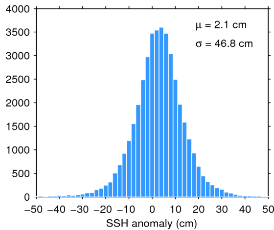
Figure 7. Histogram of flag-valid SSH anomaly over oceans and lakes for 09/08/2016. The mean ( \mu ) and standard deviation ( \sigma ) are also shown. Note that values outside [-50 50] cm are excluded from the histogram for the sake of readability but not from the computation of \mu and \sigma .
