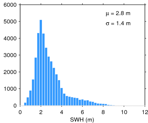
Figure 20. Histogram of science-valid SWH over oceans and lakes for 09/08/2016. The mean ( \mu ) and standard deviation ( \sigma ) are also shown. Note that values larger than 12 m are excluded from the histogram for the sake of readability but not from the computation of \mu and \sigma .
