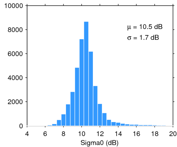
Figure 25. Histogram of flag-valid sigma0 over oceans and lakes for 09/08/2016. The mean ( \mu ) and standard deviation ( \sigma ) are also shown. Note that values outside [4 20] dB are excluded from the histogram for the sake of readability but not from the computation of \mu and \sigma .
