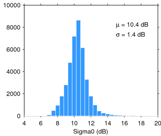
Figure 28. Histogram of science-valid sigma0 over oceans and lakes for 09/08/2016. The mean ( \mu ) and standard deviation ( \sigma ) are also shown. Note that values outside [4 20] dB are excluded from the histogram for the sake of readability but not from the computation of \mu and \sigma .
