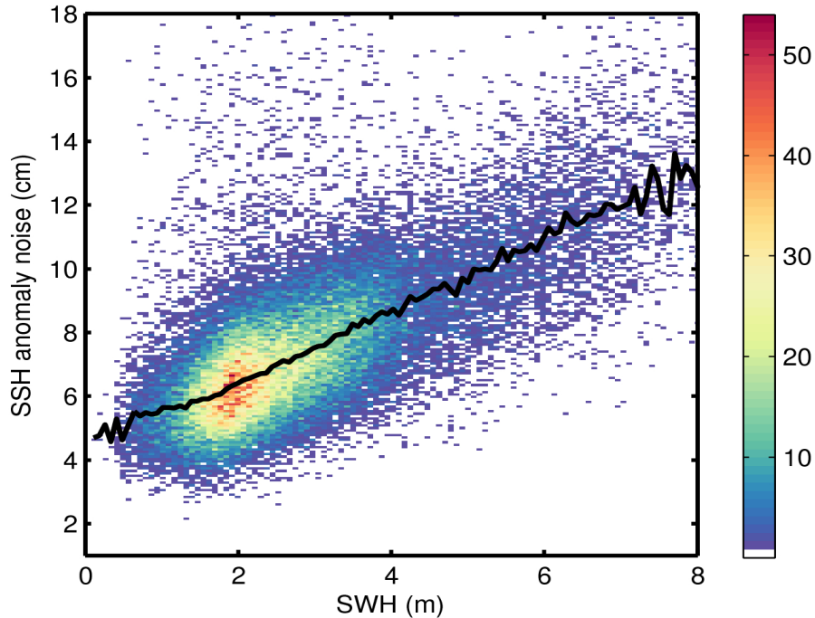
Figure 9. 2D histogram showing flag-valid SSH anomaly noise as a function of SWH for 09/08/2016. The black line denotes the median SSH anomaly noise as a function of SWH.
