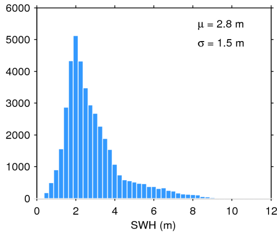
Figure 17. Histogram of flag-valid SWH over oceans and lakes for 09/08/2016. The mean ( \mu ) and standard deviation ( \sigma ) are also shown. Note that values larger than 12 m are excluded from the histogram for the sake of readability but not from the computation of \mu and \sigma .
