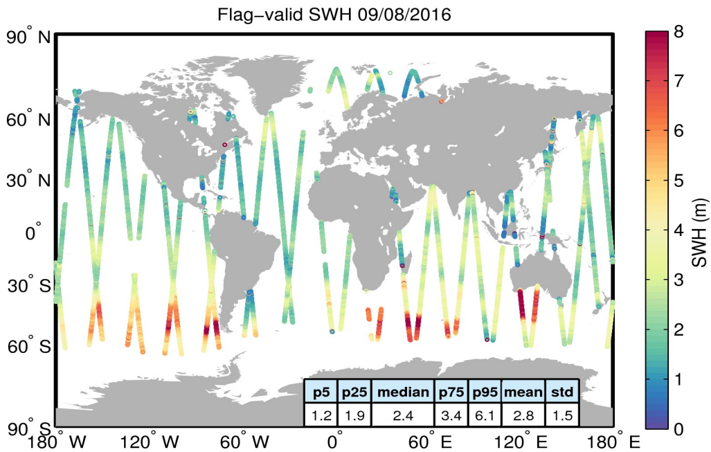
Figure 15. Geographical distribution of flag-valid SWH data over oceans and lakes for 09/08/2016. The statistical values shown in the table refer to the SWH in m and are calculated over all measurements shown in the figure.
