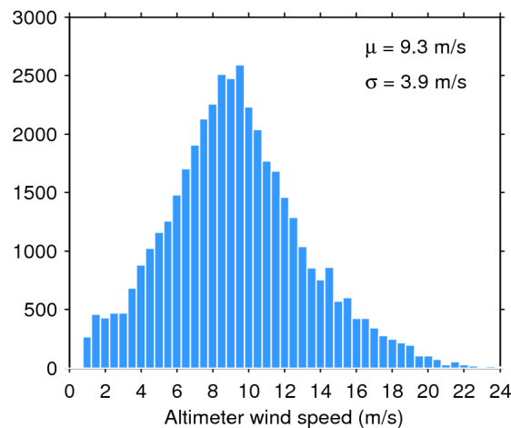
Figure 35. Histogram of science-valid wind over oceans and lakes for 09/08/2016. The mean ( \mu ) and standard deviation ( \sigma ) are also shown. Note that values larger than 24 m/s are excluded from the histogram for the sake of readability but not from the computation of \mu and \sigma .
