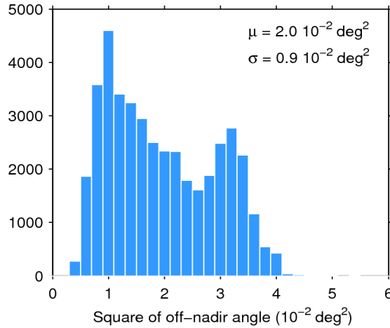
Figure 39. Histogram of flag-valid mispointing over oceans and lakes for 09/08/2016. The mean ( \mu ) and standard deviation ( \sigma ) are also shown. Note that values larger than 6 \cdot 10^{-2} \text{ deg}^2 are excluded from the histogram for the sake of readability but not from the computation of \mu and \sigma .
