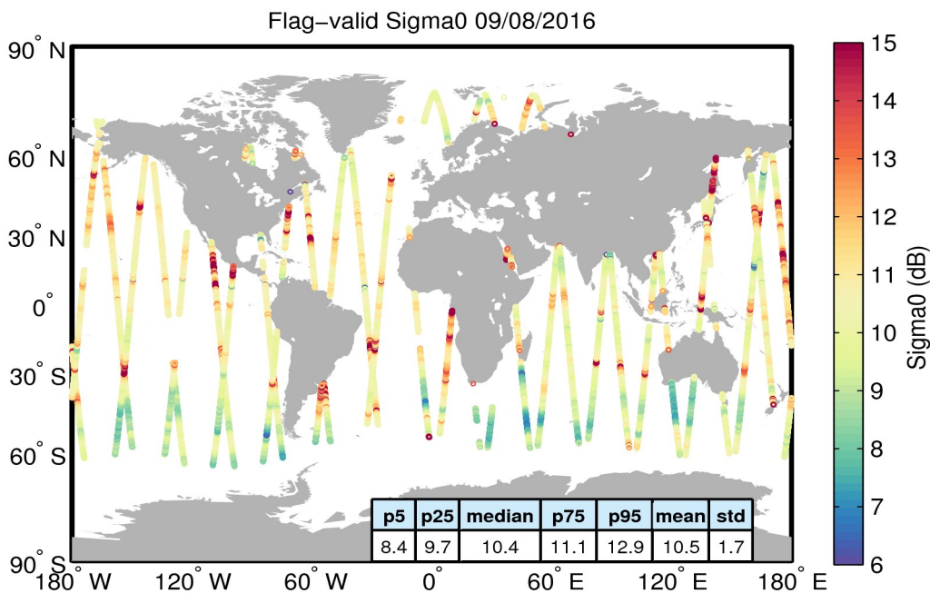
Figure 23. Geographical distribution of flag-valid sigma0 data over oceans and lakes for 09/08/2016. The statistical values shown in the table refer to the sigma0 in dB and are calculated over all measurements shown in the figure.
