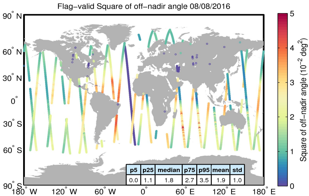
Figure 37. Geographical distribution of flag-valid mispointing data over oceans and lakes for 08/08/2016. The statistical values shown in the table refer to the mispointing in 10^{-2} deg 2 and are calculated over all measurements shown in the figure.
