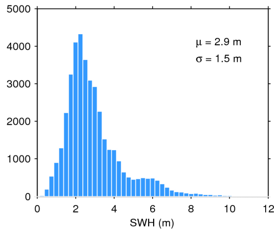
Figure 20. Histogram of science-valid SWH over oceans and lakes for 08/08/2016. The mean ( \mu ) and standard deviation ( \sigma ) are also shown. Note that values larger than 12 m are excluded from the histogram for the sake of readability but not from the computation of \mu and \sigma .
