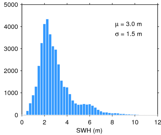
Figure 17. Histogram of flag-valid SWH over oceans and lakes for 08/08/2016. The mean ( \mu ) and standard deviation ( \sigma ) are also shown. Note that values larger than 12 m are excluded from the histogram for the sake of readability but not from the computation of \mu and \sigma .
