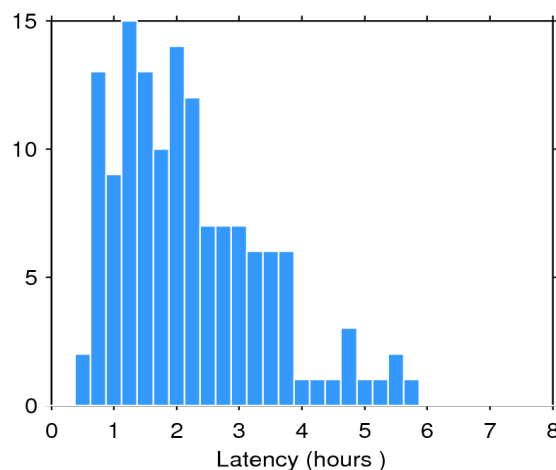
Figure 2. Histogram of the data latency for 08/08/2016. The y-axis denotes the number of files that are made available with a delay of x-hours with respect to the mean time of the records stored in the file.
