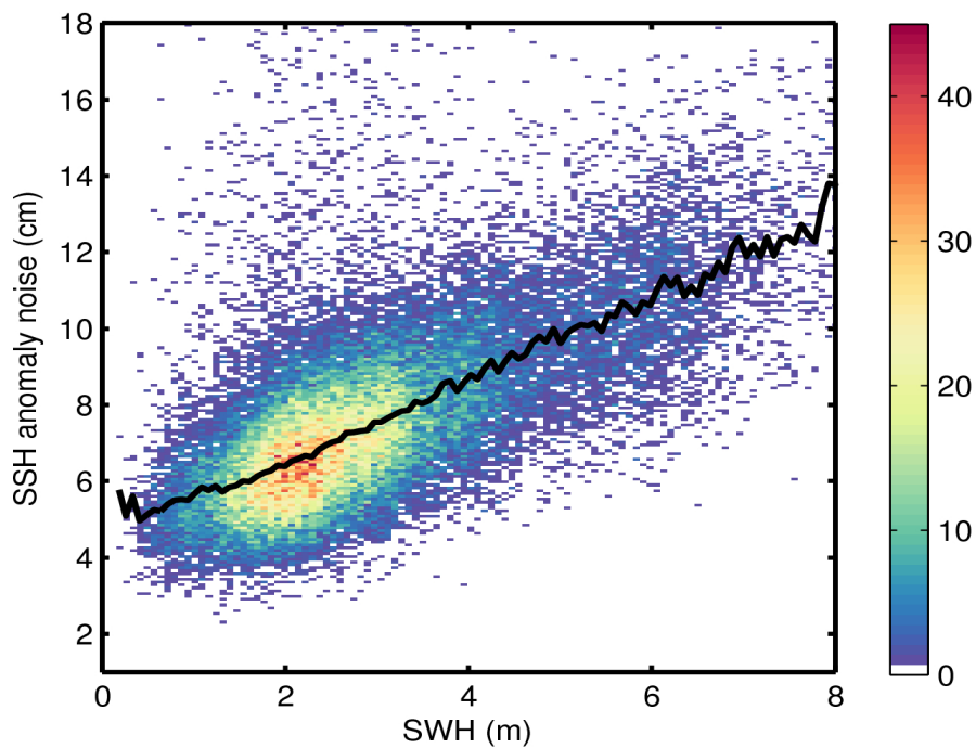
Figure 9. 2D histogram showing flag-valid SSH anomaly noise as a function of SWH for 08/08/2016. The black line denotes the median SSH anomaly noise as a function of SWH.
