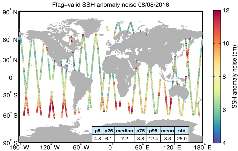
Figure 8. Geographical distribution of flag-valid 20-Hz SSH anomaly measurement noise over oceans and lakes for 08/08/2016. The statistical values shown in the table refer to the SSH anomaly noise and are calculated over all measurements shown in the figure.
