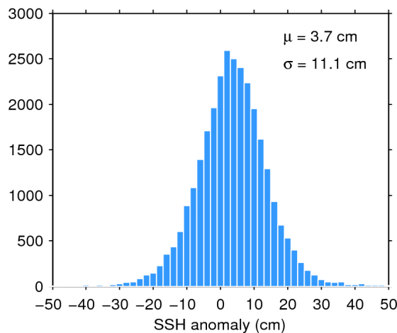
Figure 11. Histogram of science-valid SSH anomaly over oceans and lakes for 08/08/2016. The mean ( \mu ) and standard deviation ( \sigma ) are also shown. Note that values outside [-50 50] cm are excluded from the histogram for the sake of readability but not from the computation of \mu and \sigma .
