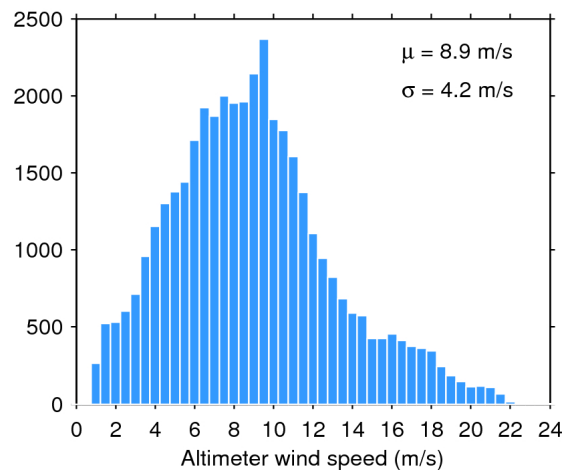
Figure 35. Histogram of science-valid wind over oceans and lakes for 08/08/2016. The mean ( \mu ) and standard deviation ( \sigma ) are also shown. Note that values larger than 24 m/s are excluded from the histogram for the sake of readability but not from the computation of \mu and \sigma .
