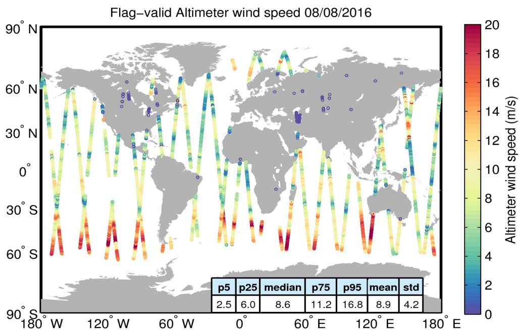
Figure 31. Geographical distribution of flag-valid wind data over oceans and lakes for 08/08/2016. The statistical values shown in the table refer to the wind in m/s and are calculated over all measurements shown in the figure.
