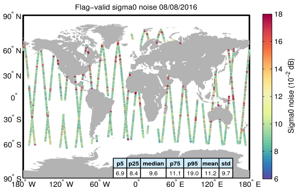
Figure 26. Geographical distribution of flag-valid 20-Hz sigma0 measurement noise over oceans and lakes for 08/08/2016. The statistical values shown in the table refer to the sigma0 noise and are calculated over all measurements shown in the figure.
