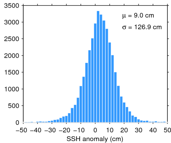
Figure 7. Histogram of flag-valid SSH anomaly over oceans and lakes for 08/08/2016. The mean ( \mu ) and standard deviation ( \sigma ) are also shown. Note that values outside [-50 50] cm are excluded from the histogram for the sake of readability but not from the computation of \mu and \sigma .
