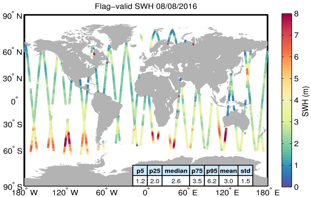
Figure 15. Geographical distribution of flag-valid SWH data over oceans and lakes for 08/08/2016. The statistical values shown in the table refer to the SWH in m and are calculated over all measurements shown in the figure.
