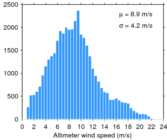
Figure 33. Histogram of flag-valid wind over oceans and lakes for 08/08/2016. The mean ( \mu ) and standard deviation ( \sigma ) are also shown. Note that values larger than 24 m/s are excluded from the histogram for the sake of readability but not from the computation of \mu and \sigma .
