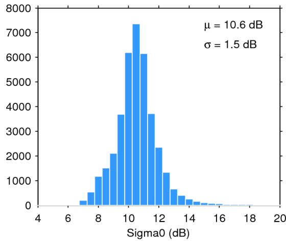
Figure 28. Histogram of science-valid sigma0 over oceans and lakes for 08/08/2016. The mean ( \mu ) and standard deviation ( \sigma ) are also shown. Note that values outside [4 20] dB are excluded from the histogram for the sake of readability but not from the computation of \mu and \sigma .
