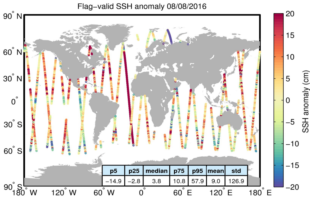
Figure 5. Geographical distribution of flag-valid 1-Hz SSH anomaly data over oceans and lakes for 08/08/2016. The statistical values shown in the table refer to the SSH anomaly in cm and are calculated over all measurements shown in the figure.
