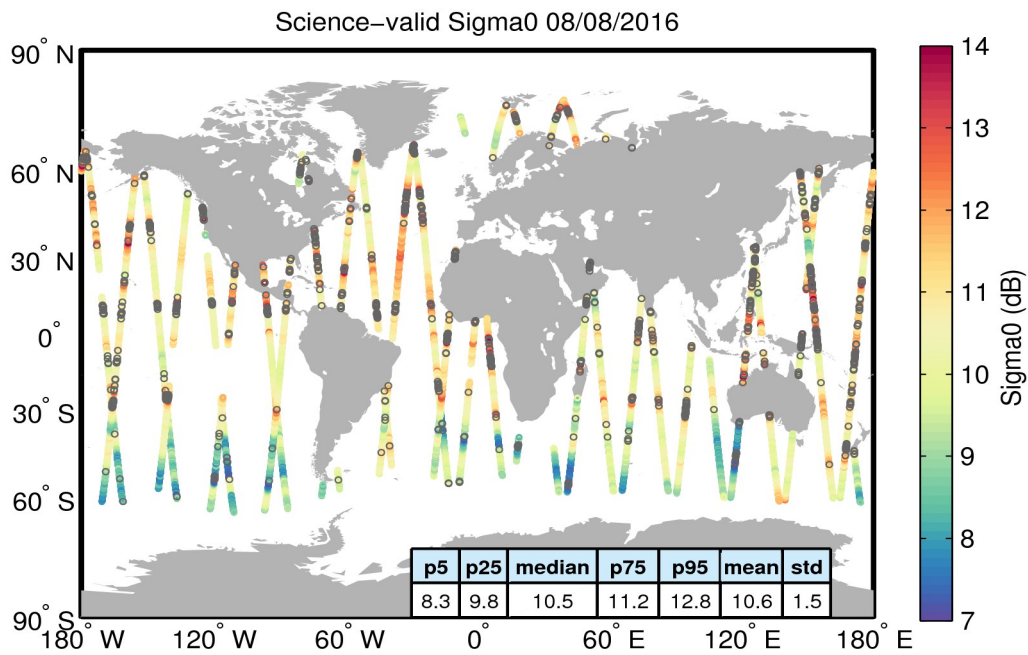
Figure 27. Geographical distribution of science-valid sigma0 data over oceans and lakes for 08/08/2016. The statistical values shown in the table refer to the sigma0 in dB and are calculated over all measurements shown in the figure. Gray circles denote records that have been rejected based on the editing criteria described in Table 4.
