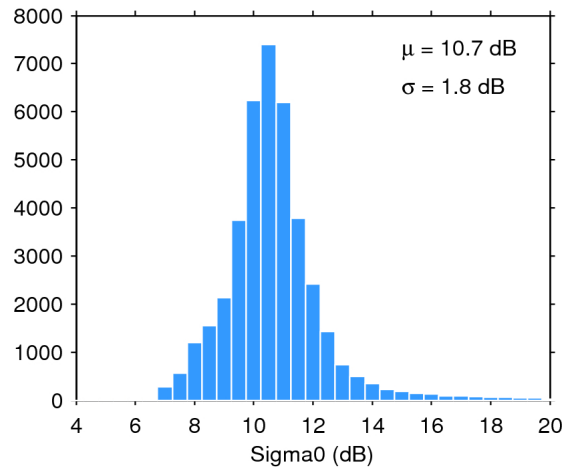
Figure 25. Histogram of flag-valid sigma0 over oceans and lakes for 08/08/2016. The mean ( \mu ) and standard deviation ( \sigma ) are also shown. Note that values outside [4 20] dB are excluded from the histogram for the sake of readability but not from the computation of \mu and \sigma .
