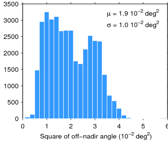
Figure 39. Histogram of flag-valid mispointing over oceans and lakes for 08/08/2016. The mean ( \mu ) and standard deviation ( \sigma ) are also shown. Note that values larger than 6 \cdot 10^{-2} \text{ deg}^2 are excluded from the histogram for the sake of readability but not from the computation of \mu and \sigma .
