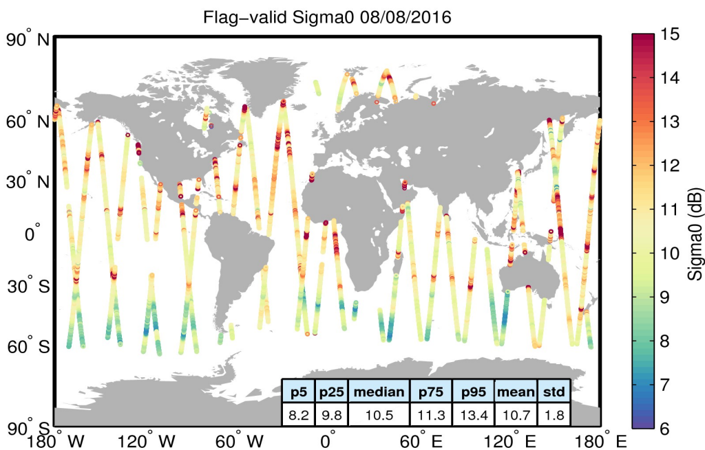
Figure 23. Geographical distribution of flag-valid sigma0 data over oceans and lakes for 08/08/2016. The statistical values shown in the table refer to the sigma0 in dB and are calculated over all measurements shown in the figure.
