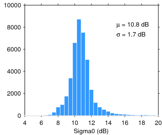
Figure 25. Histogram of flag-valid sigma0 over oceans and lakes for 07/08/2016. The mean ( \mu ) and standard deviation ( \sigma ) are also shown. Note that values outside [4 20] dB are excluded from the histogram for the sake of readability but not from the computation of \mu and \sigma .
