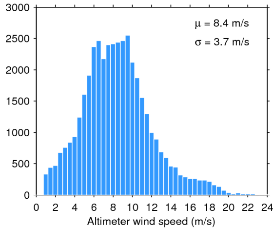
Figure 33. Histogram of flag-valid wind over oceans and lakes for 07/08/2016. The mean ( \mu ) and standard deviation ( \sigma ) are also shown. Note that values larger than 24 m/s are excluded from the histogram for the sake of readability but not from the computation of \mu and \sigma .
