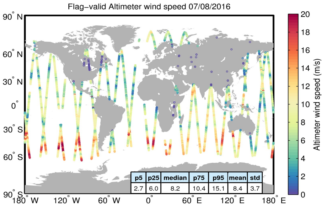
Figure 31. Geographical distribution of flag-valid wind data over oceans and lakes for 07/08/2016. The statistical values shown in the table refer to the wind in m/s and are calculated over all measurements shown in the figure.
