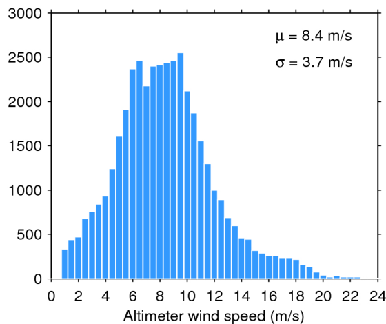
Figure 35. Histogram of science-valid wind over oceans and lakes for 07/08/2016. The mean ( \mu ) and standard deviation ( \sigma ) are also shown. Note that values larger than 24 m/s are excluded from the histogram for the sake of readability but not from the computation of \mu and \sigma .
