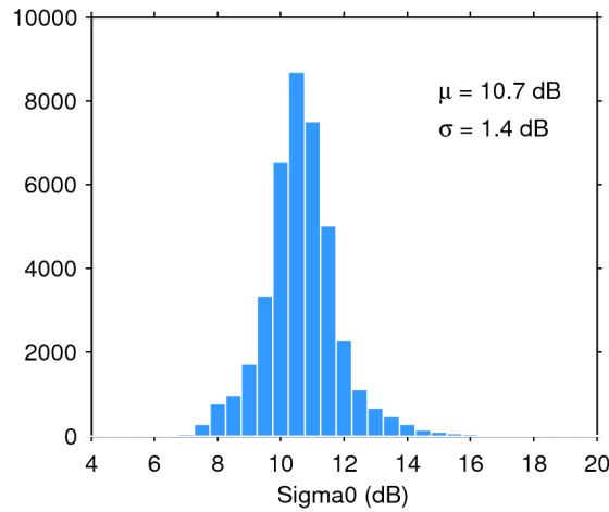
Figure 28. Histogram of science-valid sigma0 over oceans and lakes for 07/08/2016. The mean ( \mu ) and standard deviation ( \sigma ) are also shown. Note that values outside [4 20] dB are excluded from the histogram for the sake of readability but not from the computation of \mu and \sigma .
