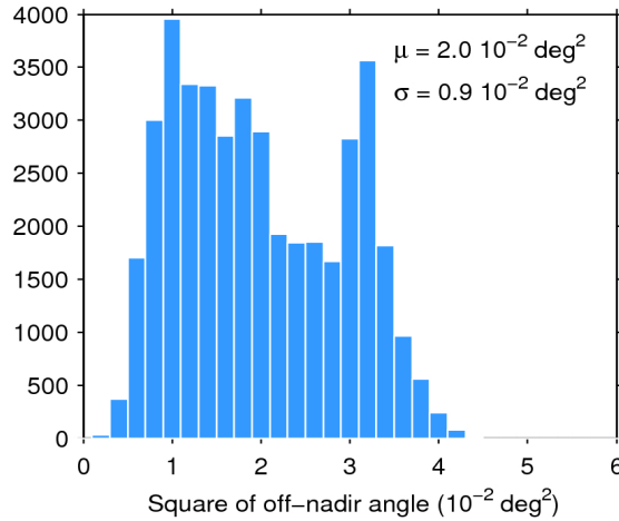
Figure 39. Histogram of flag-valid mispointing over oceans and lakes for 07/08/2016. The mean ( \mu ) and standard deviation ( \sigma ) are also shown. Note that values larger than 6 \cdot 10^{-2} \text{ deg}^2 are excluded from the histogram for the sake of readability but not from the computation of \mu and \sigma .
