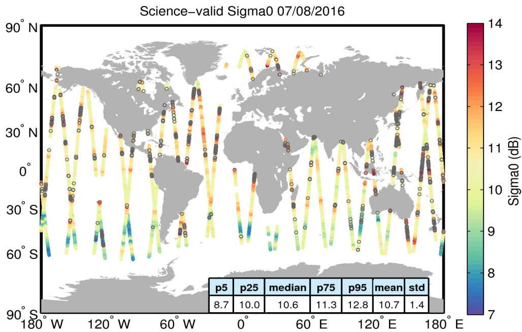
Figure 27. Geographical distribution of science-valid sigma0 data over oceans and lakes for 07/08/2016. The statistical values shown in the table refer to the sigma0 in dB and are calculated over all measurements shown in the figure. Gray circles denote records that have been rejected based on the editing criteria described in Table 4.
