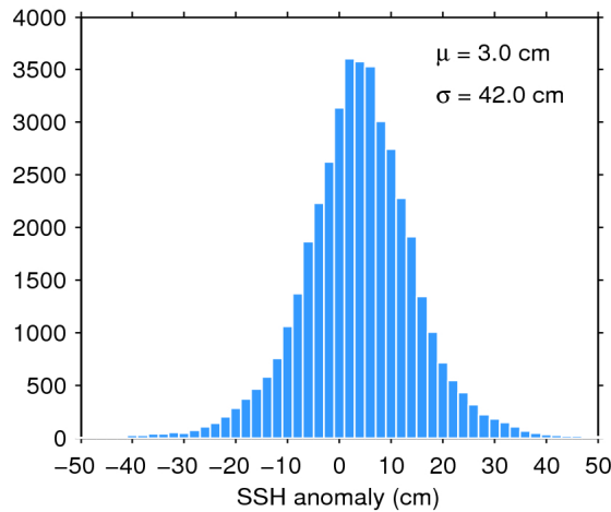
Figure 7. Histogram of flag-valid SSH anomaly over oceans and lakes for 07/08/2016. The mean ( \mu ) and standard deviation ( \sigma ) are also shown. Note that values outside [-50 50] cm are excluded from the histogram for the sake of readability but not from the computation of \mu and \sigma .
