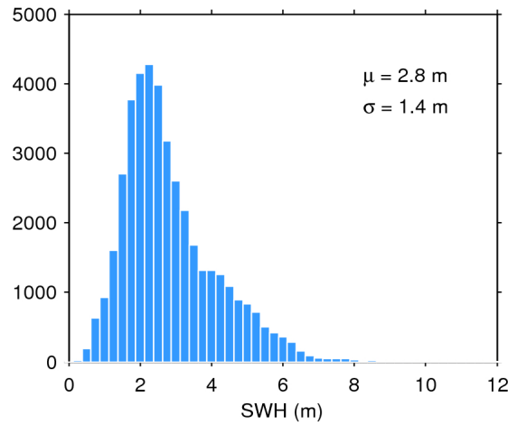
Figure 17. Histogram of flag-valid SWH over oceans and lakes for 07/08/2016. The mean ( \mu ) and standard deviation ( \sigma ) are also shown. Note that values larger than 12 m are excluded from the histogram for the sake of readability but not from the computation of \mu and \sigma .
