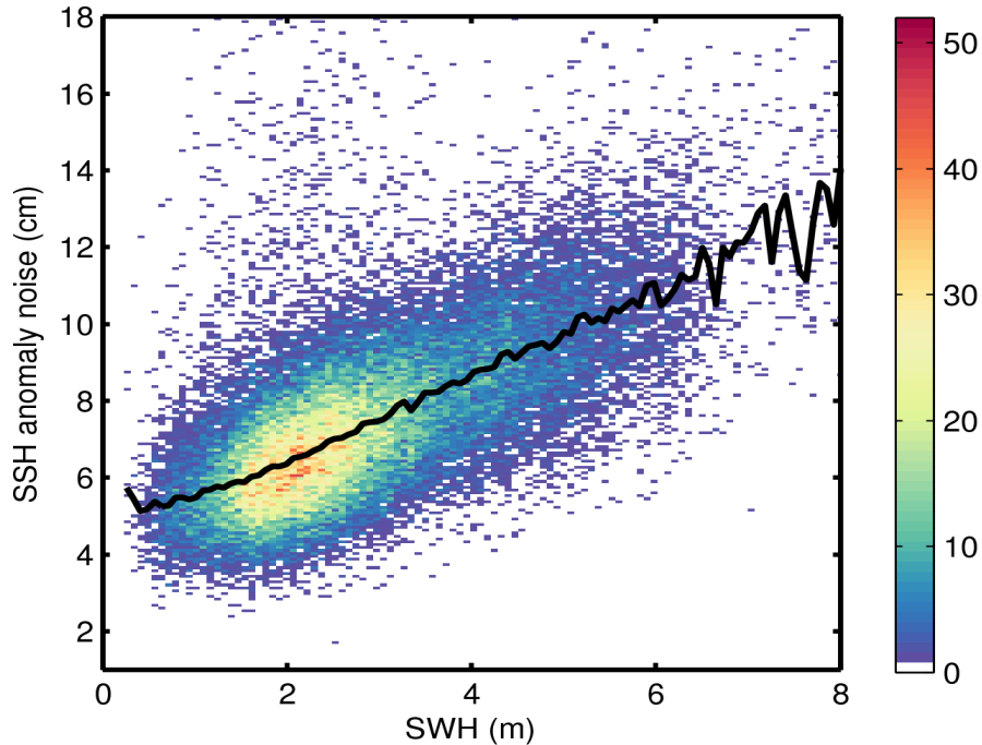
Figure 9. 2D histogram showing flag-valid SSH anomaly noise as a function of SWH for 07/08/2016. The black line denotes the median SSH anomaly noise as a function of SWH.
