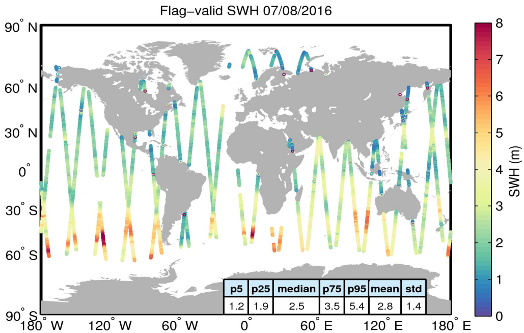
Figure 15. Geographical distribution of flag-valid SWH data over oceans and lakes for 07/08/2016. The statistical values shown in the table refer to the SWH in m and are calculated over all measurements shown in the figure.
