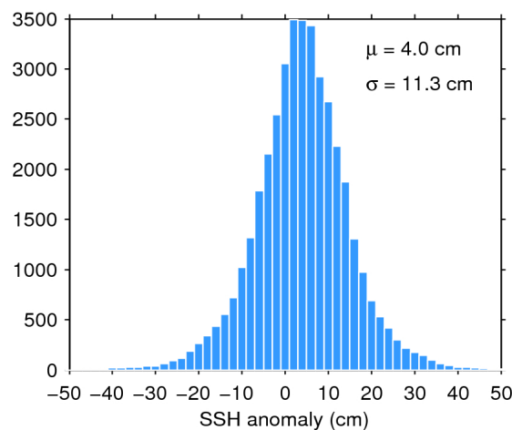
Figure 11. Histogram of science-valid SSH anomaly over oceans and lakes for 07/08/2016. The mean ( \mu ) and standard deviation ( \sigma ) are also shown. Note that values outside [-50 50] cm are excluded from the histogram for the sake of readability but not from the computation of \mu and \sigma .
