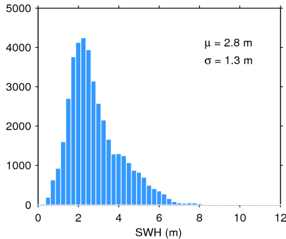
Figure 20. Histogram of science-valid SWH over oceans and lakes for 07/08/2016. The mean ( \mu ) and standard deviation ( \sigma ) are also shown. Note that values larger than 12 m are excluded from the histogram for the sake of readability but not from the computation of \mu and \sigma .
