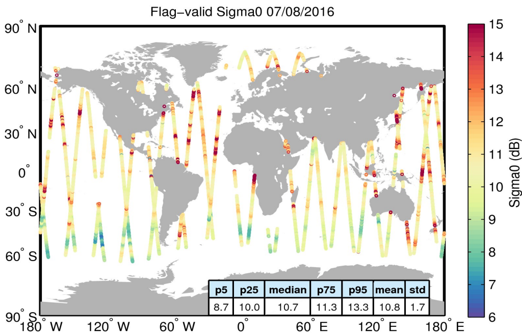
Figure 23. Geographical distribution of flag-valid sigma0 data over oceans and lakes for 07/08/2016. The statistical values shown in the table refer to the sigma0 in dB and are calculated over all measurements shown in the figure.
