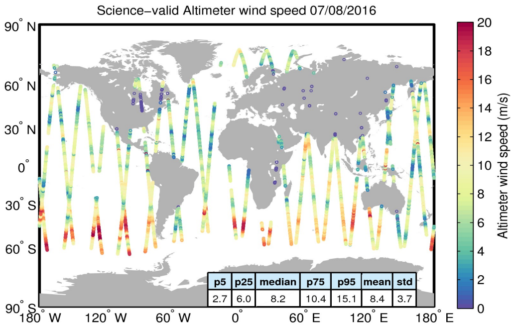
Figure 34. Geographical distribution of science-valid wind data over oceans and lakes for 07/08/2016. The statistical values shown in the table refer to the wind in m/s and are calculated over all measurements shown in the figure. Gray circles denote records that have been rejected based on the editing criteria described in Table 5.
