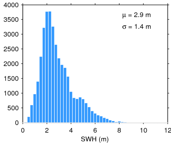
Figure 20. Histogram of science-valid SWH over oceans and lakes for 06/08/2016. The mean ( \mu ) and standard deviation ( \sigma ) are also shown. Note that values larger than 12 m are excluded from the histogram for the sake of readability but not from the computation of \mu and \sigma .
