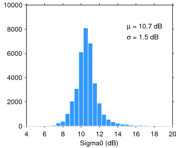
Figure 28. Histogram of science-valid sigma0 over oceans and lakes for 06/08/2016. The mean ( \mu ) and standard deviation ( \sigma ) are also shown. Note that values outside [4 20] dB are excluded from the histogram for the sake of readability but not from the computation of \mu and \sigma .
