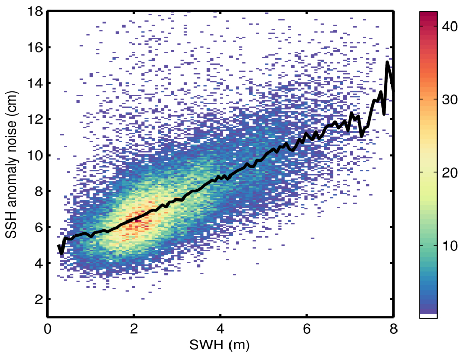
Figure 9. 2D histogram showing flag-valid SSH anomaly noise as a function of SWH for 06/08/2016. The black line denotes the median SSH anomaly noise as a function of SWH.
