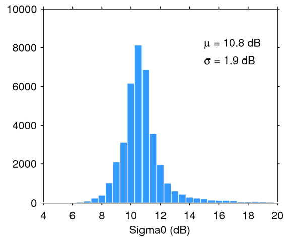
Figure 25. Histogram of flag-valid sigma0 over oceans and lakes for 06/08/2016. The mean ( \mu ) and standard deviation ( \sigma ) are also shown. Note that values outside [4 20] dB are excluded from the histogram for the sake of readability but not from the computation of \mu and \sigma .
