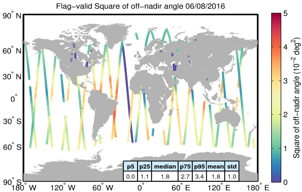
Figure 37. Geographical distribution of flag-valid mispointing data over oceans and lakes for 06/08/2016. The statistical values shown in the table refer to the mispointing in 10^{-2} deg 2 and are calculated over all measurements shown in the figure.
