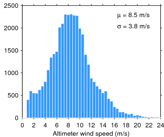
Figure 35. Histogram of science-valid wind over oceans and lakes for 06/08/2016. The mean ( \mu ) and standard deviation ( \sigma ) are also shown. Note that values larger than 24 m/s are excluded from the histogram for the sake of readability but not from the computation of \mu and \sigma .
