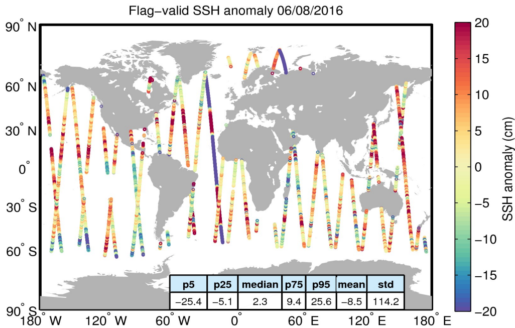
Figure 5. Geographical distribution of flag-valid 1-Hz SSH anomaly data over oceans and lakes for 06/08/2016. The statistical values shown in the table refer to the SSH anomaly in cm and are calculated over all measurements shown in the figure.
