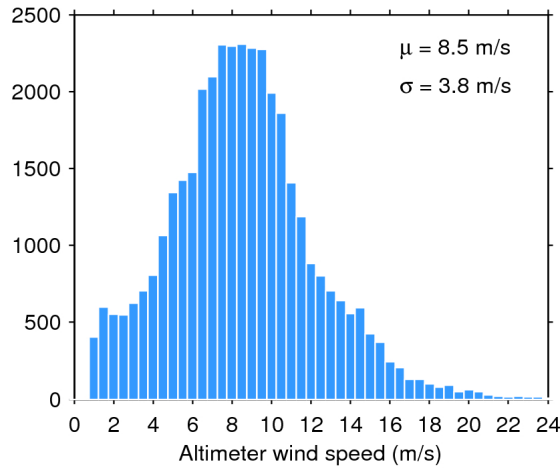
Figure 33. Histogram of flag-valid wind over oceans and lakes for 06/08/2016. The mean ( \mu ) and standard deviation ( \sigma ) are also shown. Note that values larger than 24 m/s are excluded from the histogram for the sake of readability but not from the computation of \mu and \sigma .
