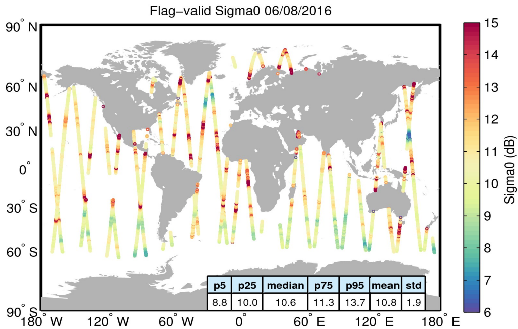
Figure 23. Geographical distribution of flag-valid sigma0 data over oceans and lakes for 06/08/2016. The statistical values shown in the table refer to the sigma0 in dB and are calculated over all measurements shown in the figure.
