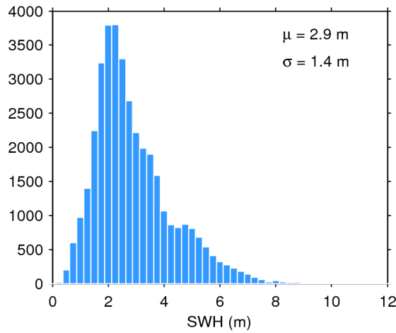
Figure 17. Histogram of flag-valid SWH over oceans and lakes for 06/08/2016. The mean ( \mu ) and standard deviation ( \sigma ) are also shown. Note that values larger than 12 m are excluded from the histogram for the sake of readability but not from the computation of \mu and \sigma .
