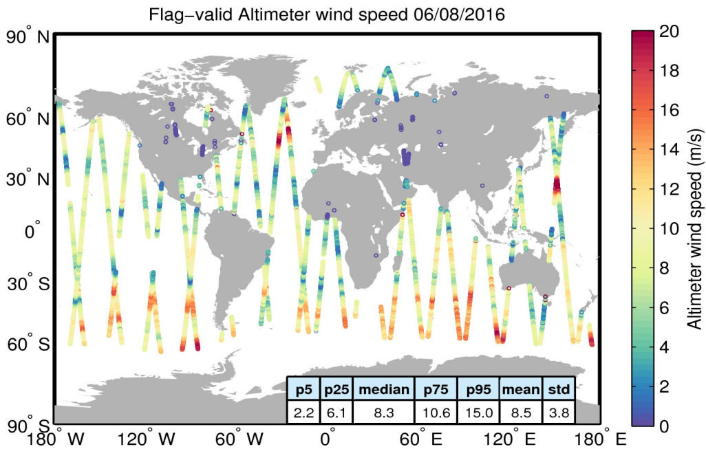
Figure 31. Geographical distribution of flag-valid wind data over oceans and lakes for 06/08/2016. The statistical values shown in the table refer to the wind in m/s and are calculated over all measurements shown in the figure.
