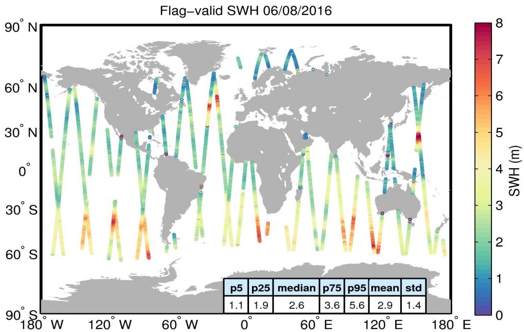
Figure 15. Geographical distribution of flag-valid SWH data over oceans and lakes for 06/08/2016. The statistical values shown in the table refer to the SWH in m and are calculated over all measurements shown in the figure.
