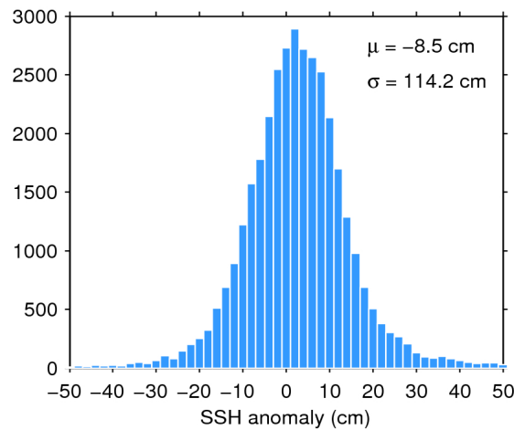
Figure 7. Histogram of flag-valid SSH anomaly over oceans and lakes for 06/08/2016. The mean ( \mu ) and standard deviation ( \sigma ) are also shown. Note that values outside [-50 50] cm are excluded from the histogram for the sake of readability but not from the computation of \mu and \sigma .
