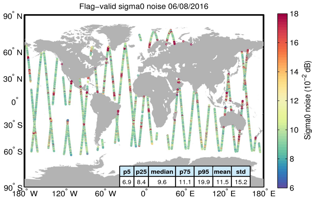
Figure 26. Geographical distribution of flag-valid 20-Hz sigma0 measurement noise over oceans and lakes for 06/08/2016. The statistical values shown in the table refer to the sigma0 noise and are calculated over all measurements shown in the figure.
