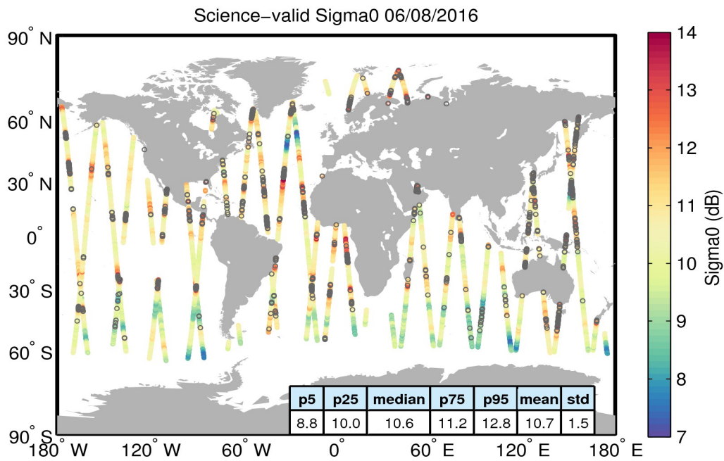
Figure 27. Geographical distribution of science-valid sigma0 data over oceans and lakes for 06/08/2016. The statistical values shown in the table refer to the sigma0 in dB and are calculated over all measurements shown in the figure. Gray circles denote records that have been rejected based on the editing criteria described in Table 4.
