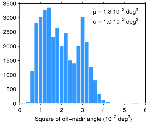
Figure 39. Histogram of flag-valid mispointing over oceans and lakes for 06/08/2016. The mean ( \mu ) and standard deviation ( \sigma ) are also shown. Note that values larger than 6 \cdot 10^{-2} \text{ deg}^2 are excluded from the histogram for the sake of readability but not from the computation of \mu and \sigma .
