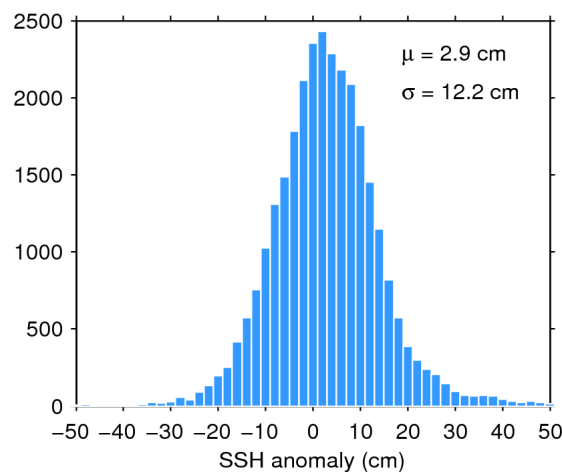
Figure 11. Histogram of science-valid SSH anomaly over oceans and lakes for 06/08/2016. The mean ( \mu ) and standard deviation ( \sigma ) are also shown. Note that values outside [-50 50] cm are excluded from the histogram for the sake of readability but not from the computation of \mu and \sigma .
