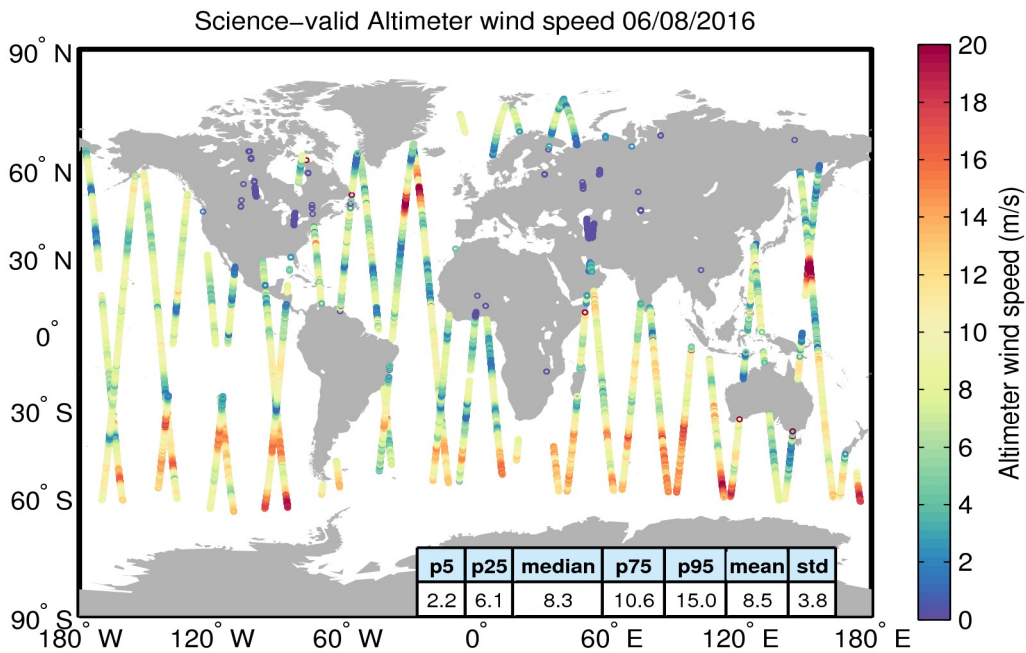
Figure 34. Geographical distribution of science-valid wind data over oceans and lakes for 06/08/2016. The statistical values shown in the table refer to the wind in m/s and are calculated over all measurements shown in the figure. Gray circles denote records that have been rejected based on the editing criteria described in Table 5.
