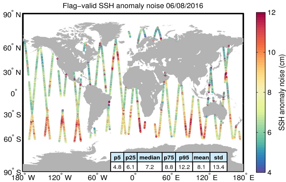
Figure 8. Geographical distribution of flag-valid 20-Hz SSH anomaly measurement noise over oceans and lakes for 06/08/2016. The statistical values shown in the table refer to the SSH anomaly noise and are calculated over all measurements shown in the figure.
