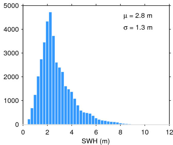
Figure 20. Histogram of science-valid SWH over oceans and lakes for 05/08/2016. The mean ( \mu ) and standard deviation ( \sigma ) are also shown. Note that values larger than 12 m are excluded from the histogram for the sake of readability but not from the computation of \mu and \sigma .
