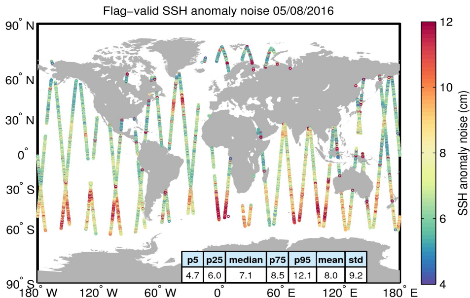
Figure 8. Geographical distribution of flag-valid 20-Hz SSH anomaly measurement noise over oceans and lakes for 05/08/2016. The statistical values shown in the table refer to the SSH anomaly noise and are calculated over all measurements shown in the figure.
