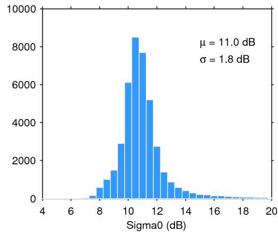
Figure 25. Histogram of flag-valid sigma0 over oceans and lakes for 05/08/2016. The mean ( \mu ) and standard deviation ( \sigma ) are also shown. Note that values outside [4 20] dB are excluded from the histogram for the sake of readability but not from the computation of \mu and \sigma .
