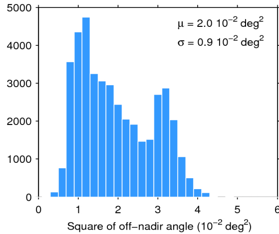
Figure 39. Histogram of flag-valid mispointing over oceans and lakes for 05/08/2016. The mean ( \mu ) and standard deviation ( \sigma ) are also shown. Note that values larger than 6 \cdot 10^{-2} \text{ deg}^2 are excluded from the histogram for the sake of readability but not from the computation of \mu and \sigma .
