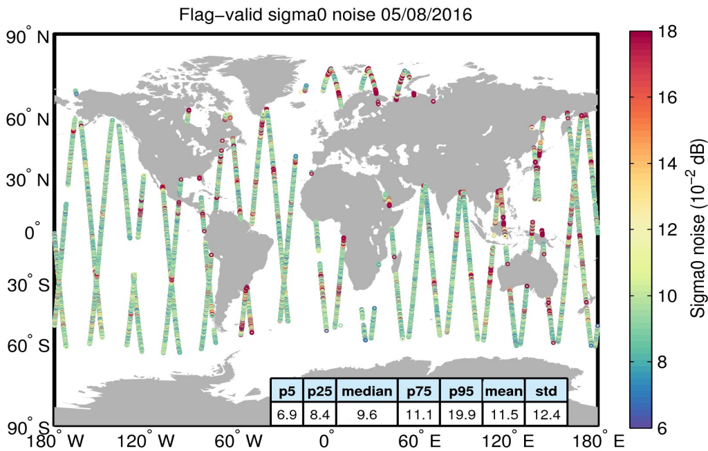
Figure 26. Geographical distribution of flag-valid 20-Hz sigma0 measurement noise over oceans and lakes for 05/08/2016. The statistical values shown in the table refer to the sigma0 noise and are calculated over all measurements shown in the figure.
