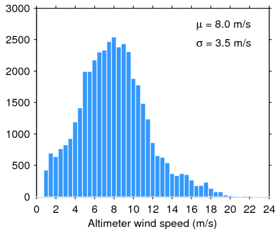
Figure 33. Histogram of flag-valid wind over oceans and lakes for 05/08/2016. The mean ( \mu ) and standard deviation ( \sigma ) are also shown. Note that values larger than 24 m/s are excluded from the histogram for the sake of readability but not from the computation of \mu and \sigma .
