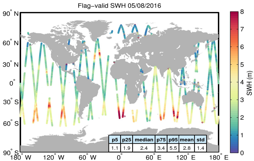
Figure 15. Geographical distribution of flag-valid SWH data over oceans and lakes for 05/08/2016. The statistical values shown in the table refer to the SWH in m and are calculated over all measurements shown in the figure.
