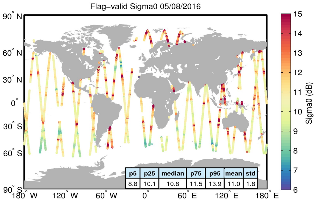
Figure 23. Geographical distribution of flag-valid sigma0 data over oceans and lakes for 05/08/2016. The statistical values shown in the table refer to the sigma0 in dB and are calculated over all measurements shown in the figure.
