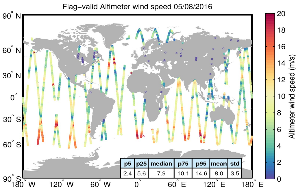
Figure 31. Geographical distribution of flag-valid wind data over oceans and lakes for 05/08/2016. The statistical values shown in the table refer to the wind in m/s and are calculated over all measurements shown in the figure.
