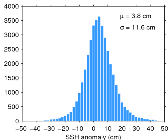
Figure 11. Histogram of science-valid SSH anomaly over oceans and lakes for 05/08/2016. The mean ( \mu ) and standard deviation ( \sigma ) are also shown. Note that values outside [-50 50] cm are excluded from the histogram for the sake of readability but not from the computation of \mu and \sigma .
