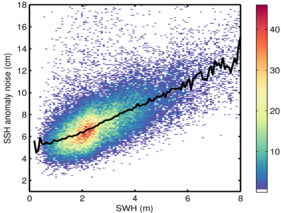
Figure 9. 2D histogram showing flag-valid SSH anomaly noise as a function of SWH for 05/08/2016. The black line denotes the median SSH anomaly noise as a function of SWH.
