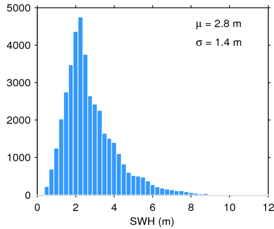
Figure 17. Histogram of flag-valid SWH over oceans and lakes for 05/08/2016. The mean ( \mu ) and standard deviation ( \sigma ) are also shown. Note that values larger than 12 m are excluded from the histogram for the sake of readability but not from the computation of \mu and \sigma .
