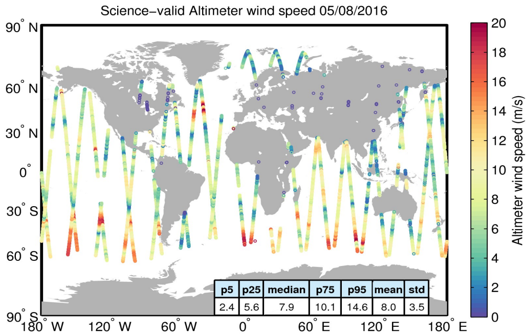
Figure 34. Geographical distribution of science-valid wind data over oceans and lakes for 05/08/2016. The statistical values shown in the table refer to the wind in m/s and are calculated over all measurements shown in the figure. Gray circles denote records that have been rejected based on the editing criteria described in Table 5.
