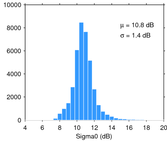
Figure 28. Histogram of science-valid sigma0 over oceans and lakes for 05/08/2016. The mean ( \mu ) and standard deviation ( \sigma ) are also shown. Note that values outside [4 20] dB are excluded from the histogram for the sake of readability but not from the computation of \mu and \sigma .
