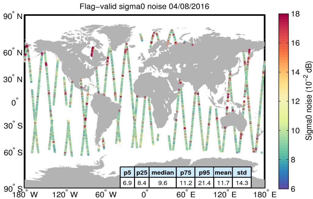
Figure 26. Geographical distribution of flag-valid 20-Hz sigma0 measurement noise over oceans and lakes for 04/08/2016. The statistical values shown in the table refer to the sigma0 noise and are calculated over all measurements shown in the figure.
