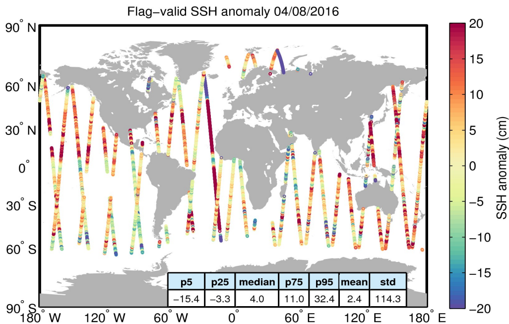
Figure 5. Geographical distribution of flag-valid 1-Hz SSH anomaly data over oceans and lakes for 04/08/2016. The statistical values shown in the table refer to the SSH anomaly in cm and are calculated over all measurements shown in the figure.
