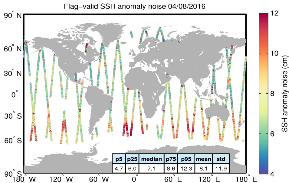
Figure 8. Geographical distribution of flag-valid 20-Hz SSH anomaly measurement noise over oceans and lakes for 04/08/2016. The statistical values shown in the table refer to the SSH anomaly noise and are calculated over all measurements shown in the figure.
