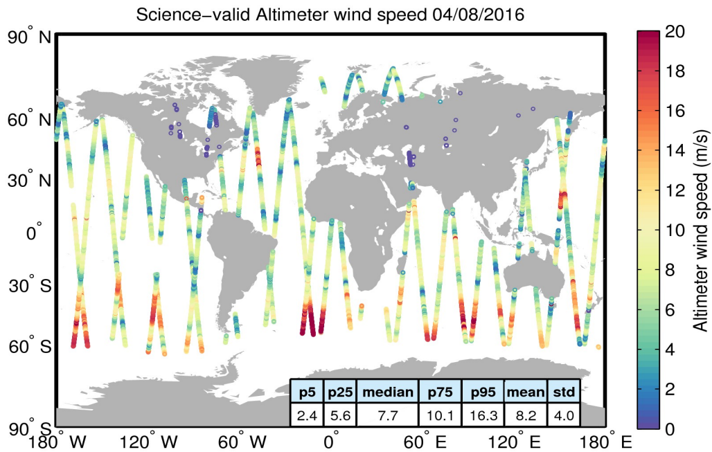
Figure 34. Geographical distribution of science-valid wind data over oceans and lakes for 04/08/2016. The statistical values shown in the table refer to the wind in m/s and are calculated over all measurements shown in the figure. Gray circles denote records that have been rejected based on the editing criteria described in Table 5.
