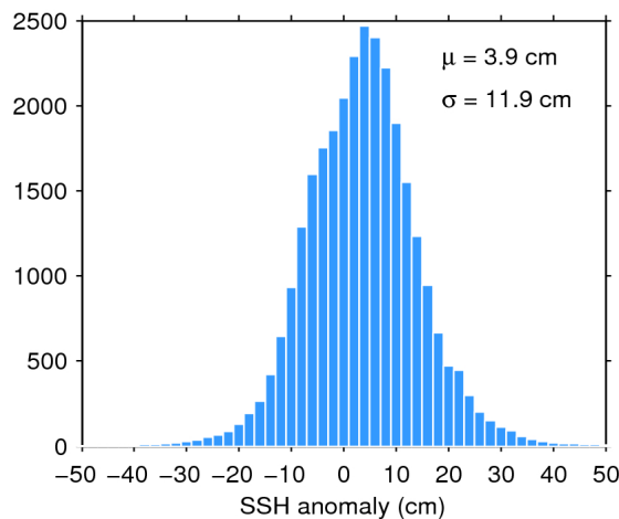
Figure 11. Histogram of science-valid SSH anomaly over oceans and lakes for 04/08/2016. The mean ( \mu ) and standard deviation ( \sigma ) are also shown. Note that values outside [-50 50] cm are excluded from the histogram for the sake of readability but not from the computation of \mu and \sigma .
