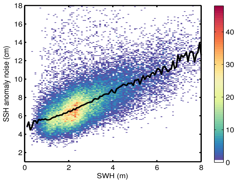
Figure 9. 2D histogram showing flag-valid SSH anomaly noise as a function of SWH for 04/08/2016. The black line denotes the median SSH anomaly noise as a function of SWH.
