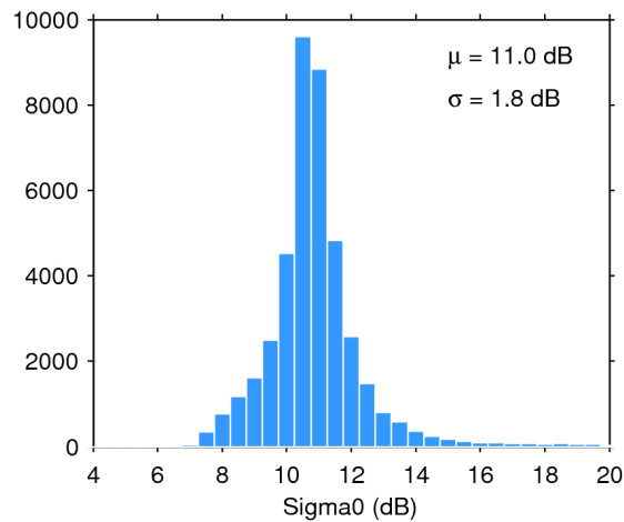
Figure 25. Histogram of flag-valid sigma0 over oceans and lakes for 03/08/2016. The mean ( \mu ) and standard deviation ( \sigma ) are also shown. Note that values outside [4 20] dB are excluded from the histogram for the sake of readability but not from the computation of \mu and \sigma .
