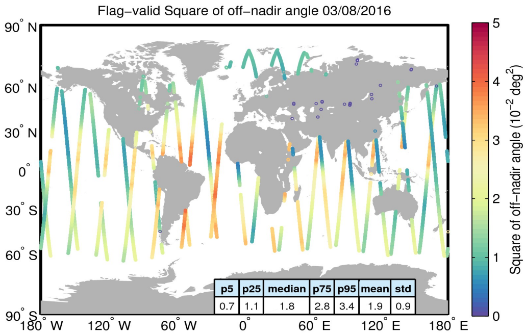
Figure 37. Geographical distribution of flag-valid mispointing data over oceans and lakes for 03/08/2016. The statistical values shown in the table refer to the mispointing in 10^{-2} deg 2 and are calculated over all measurements shown in the figure.
