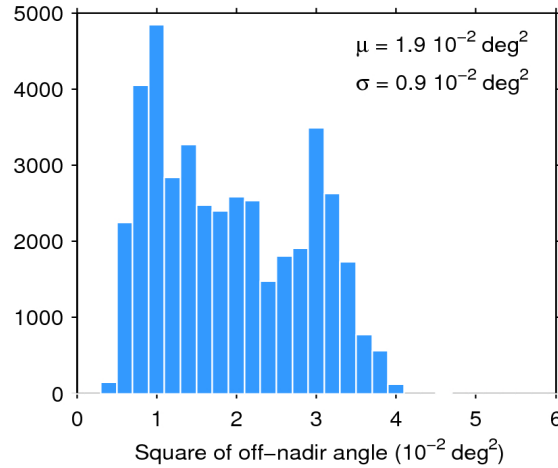
Figure 39. Histogram of flag-valid mispointing over oceans and lakes for 03/08/2016. The mean ( \mu ) and standard deviation ( \sigma ) are also shown. Note that values larger than 6 \cdot 10^{-2} \text{ deg}^2 are excluded from the histogram for the sake of readability but not from the computation of \mu and \sigma .
