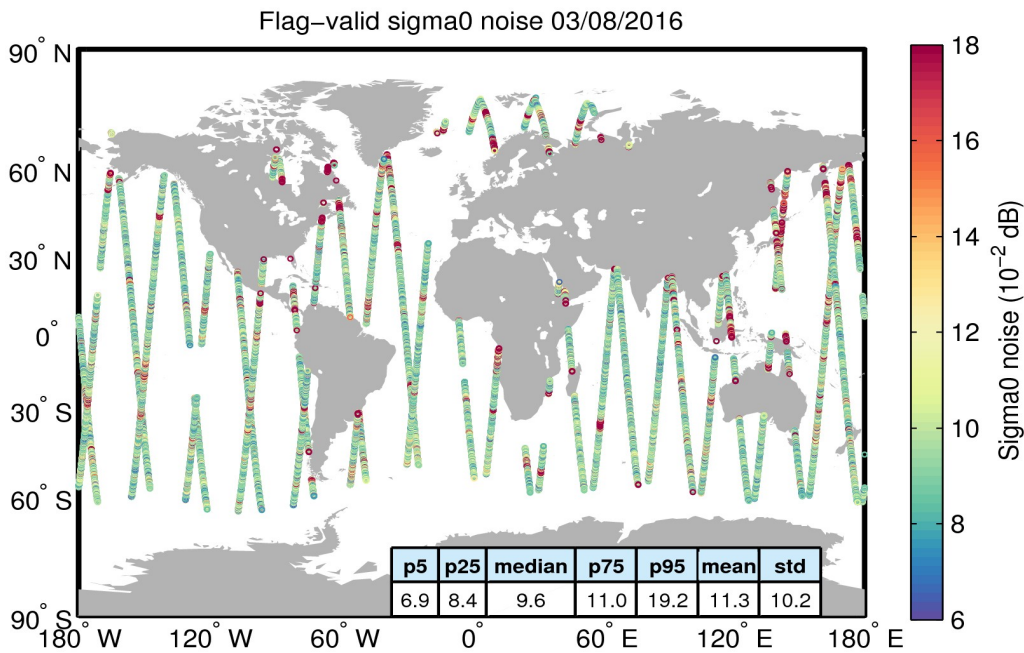
Figure 26. Geographical distribution of flag-valid 20-Hz sigma0 measurement noise over oceans and lakes for 03/08/2016. The statistical values shown in the table refer to the sigma0 noise and are calculated over all measurements shown in the figure.
