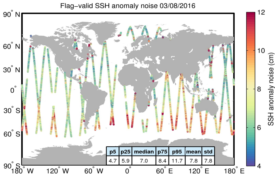
Figure 8. Geographical distribution of flag-valid 20-Hz SSH anomaly measurement noise over oceans and lakes for 03/08/2016. The statistical values shown in the table refer to the SSH anomaly noise and are calculated over all measurements shown in the figure.
