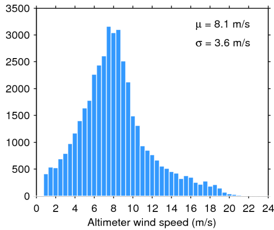
Figure 33. Histogram of flag-valid wind over oceans and lakes for 03/08/2016. The mean ( \mu ) and standard deviation ( \sigma ) are also shown. Note that values larger than 24 m/s are excluded from the histogram for the sake of readability but not from the computation of \mu and \sigma .
