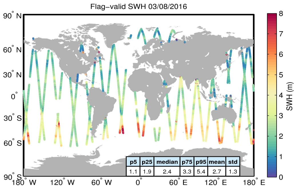
Figure 15. Geographical distribution of flag-valid SWH data over oceans and lakes for 03/08/2016. The statistical values shown in the table refer to the SWH in m and are calculated over all measurements shown in the figure.
