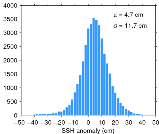
Figure 11. Histogram of science-valid SSH anomaly over oceans and lakes for 03/08/2016. The mean ( \mu ) and standard deviation ( \sigma ) are also shown. Note that values outside [-50 50] cm are excluded from the histogram for the sake of readability but not from the computation of \mu and \sigma .
