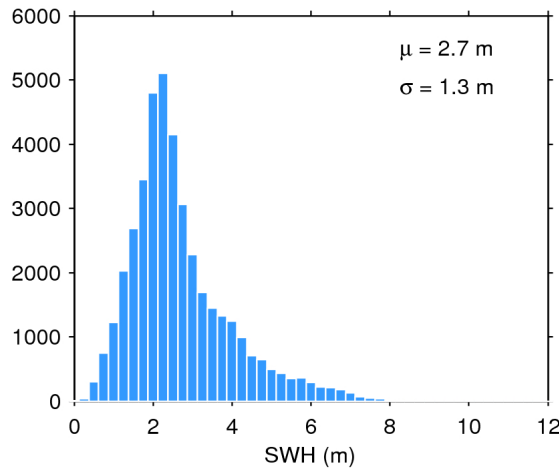
Figure 20. Histogram of science-valid SWH over oceans and lakes for 03/08/2016. The mean ( \mu ) and standard deviation ( \sigma ) are also shown. Note that values larger than 12 m are excluded from the histogram for the sake of readability but not from the computation of \mu and \sigma .
