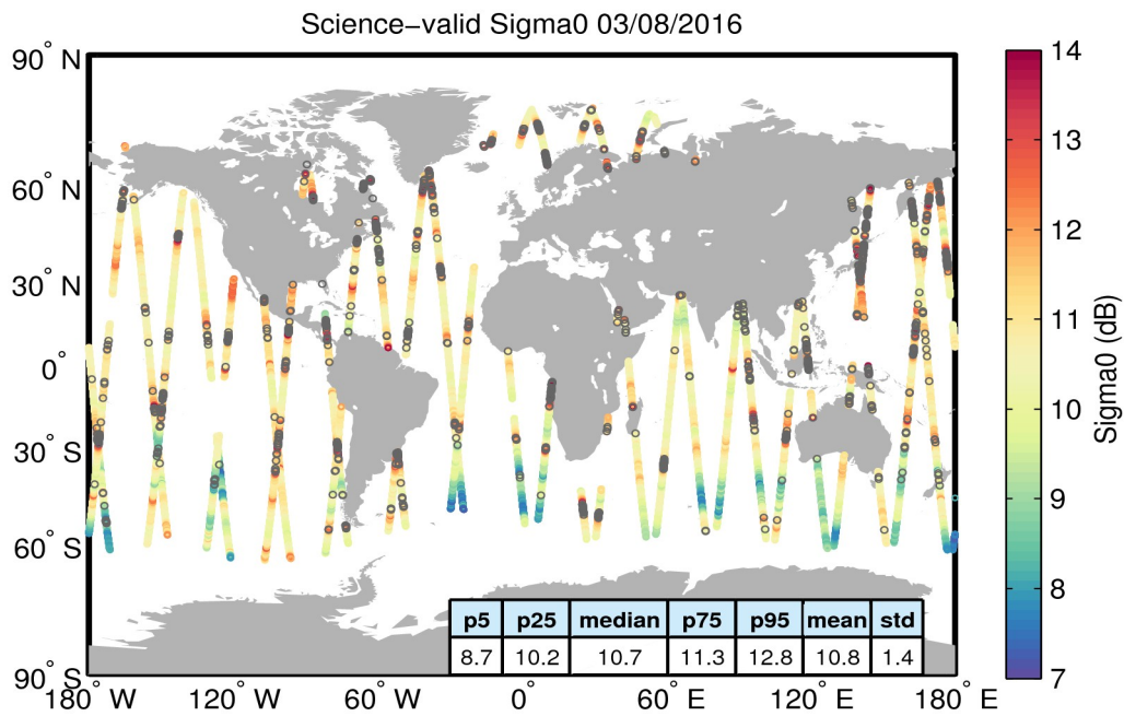
Figure 27. Geographical distribution of science-valid sigma0 data over oceans and lakes for 03/08/2016. The statistical values shown in the table refer to the sigma0 in dB and are calculated over all measurements shown in the figure. Gray circles denote records that have been rejected based on the editing criteria described in Table 4.
