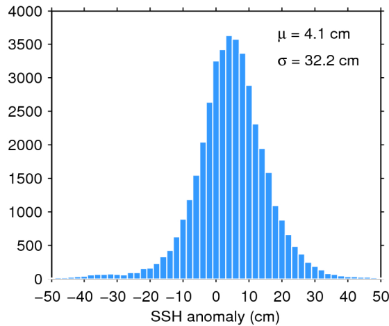
Figure 7. Histogram of flag-valid SSH anomaly over oceans and lakes for 03/08/2016. The mean ( \mu ) and standard deviation ( \sigma ) are also shown. Note that values outside [-50 50] cm are excluded from the histogram for the sake of readability but not from the computation of \mu and \sigma .
