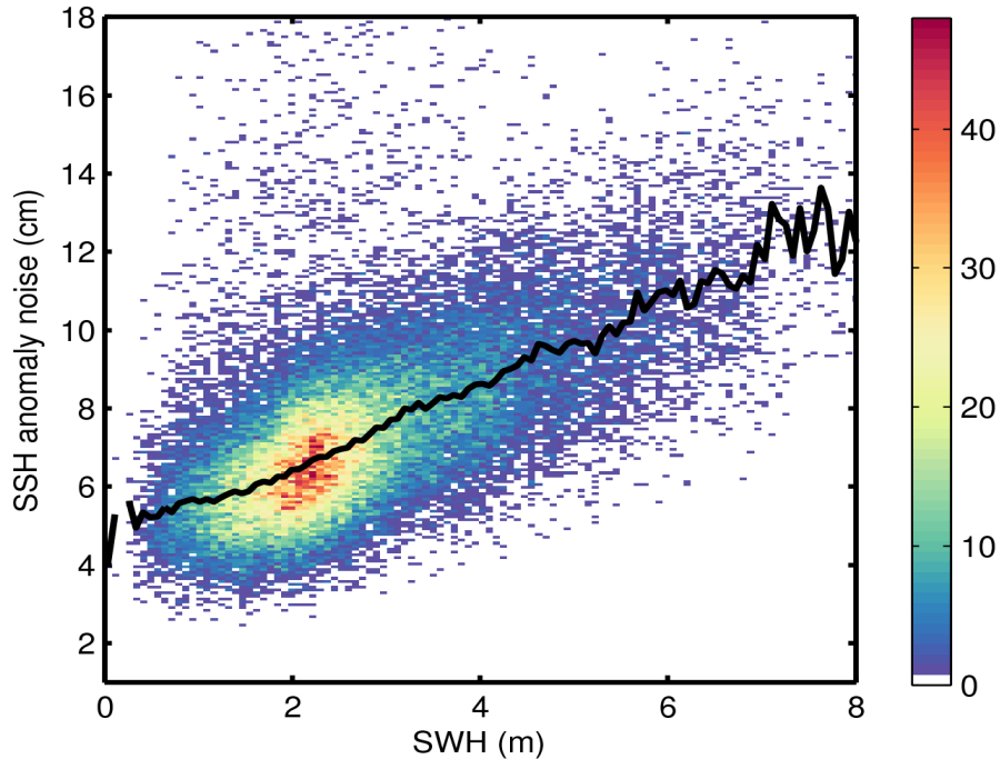
Figure 9. 2D histogram showing flag-valid SSH anomaly noise as a function of SWH for 03/08/2016. The black line denotes the median SSH anomaly noise as a function of SWH.
