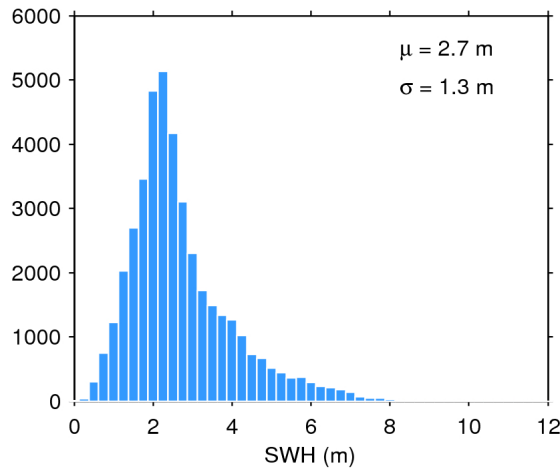
Figure 17. Histogram of flag-valid SWH over oceans and lakes for 03/08/2016. The mean ( \mu ) and standard deviation ( \sigma ) are also shown. Note that values larger than 12 m are excluded from the histogram for the sake of readability but not from the computation of \mu and \sigma .
