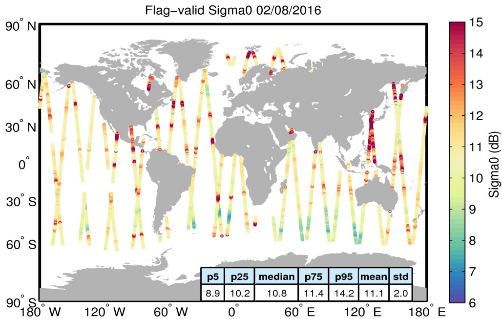
Figure 23. Geographical distribution of flag-valid sigma0 data over oceans and lakes for 02/08/2016. The statistical values shown in the table refer to the sigma0 in dB and are calculated over all measurements shown in the figure.
