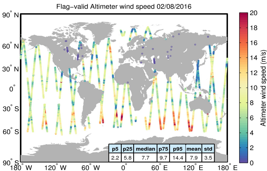
Figure 31. Geographical distribution of flag-valid wind data over oceans and lakes for 02/08/2016. The statistical values shown in the table refer to the wind in m/s and are calculated over all measurements shown in the figure.
