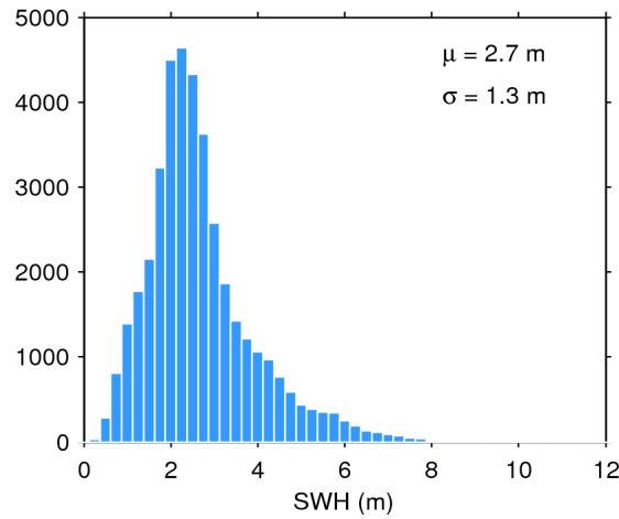
Figure 17. Histogram of flag-valid SWH over oceans and lakes for 02/08/2016. The mean ( \mu ) and standard deviation ( \sigma ) are also shown. Note that values larger than 12 m are excluded from the histogram for the sake of readability but not from the computation of \mu and \sigma .
