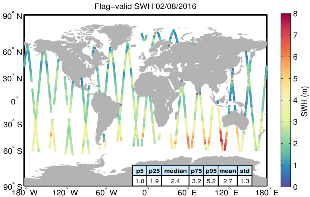
Figure 15. Geographical distribution of flag-valid SWH data over oceans and lakes for 02/08/2016. The statistical values shown in the table refer to the SWH in m and are calculated over all measurements shown in the figure.
