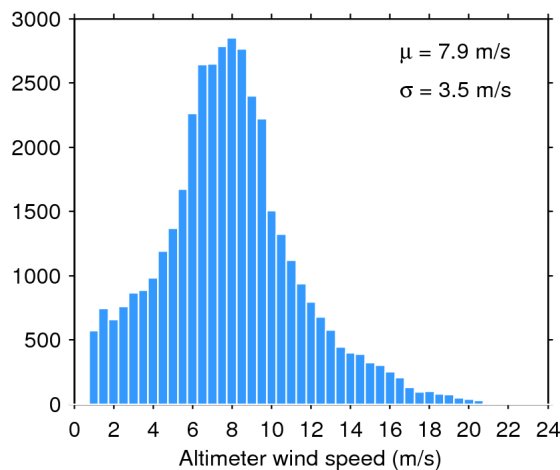
Figure 35. Histogram of science-valid wind over oceans and lakes for 02/08/2016. The mean ( \mu ) and standard deviation ( \sigma ) are also shown. Note that values larger than 24 m/s are excluded from the histogram for the sake of readability but not from the computation of \mu and \sigma .
