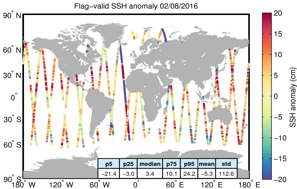
Figure 5. Geographical distribution of flag-valid 1-Hz SSH anomaly data over oceans and lakes for 02/08/2016. The statistical values shown in the table refer to the SSH anomaly in cm and are calculated over all measurements shown in the figure.
