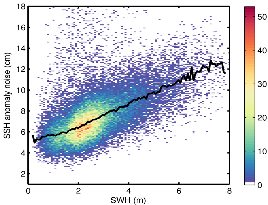
Figure 9. 2D histogram showing flag-valid SSH anomaly noise as a function of SWH for 02/08/2016. The black line denotes the median SSH anomaly noise as a function of SWH.
