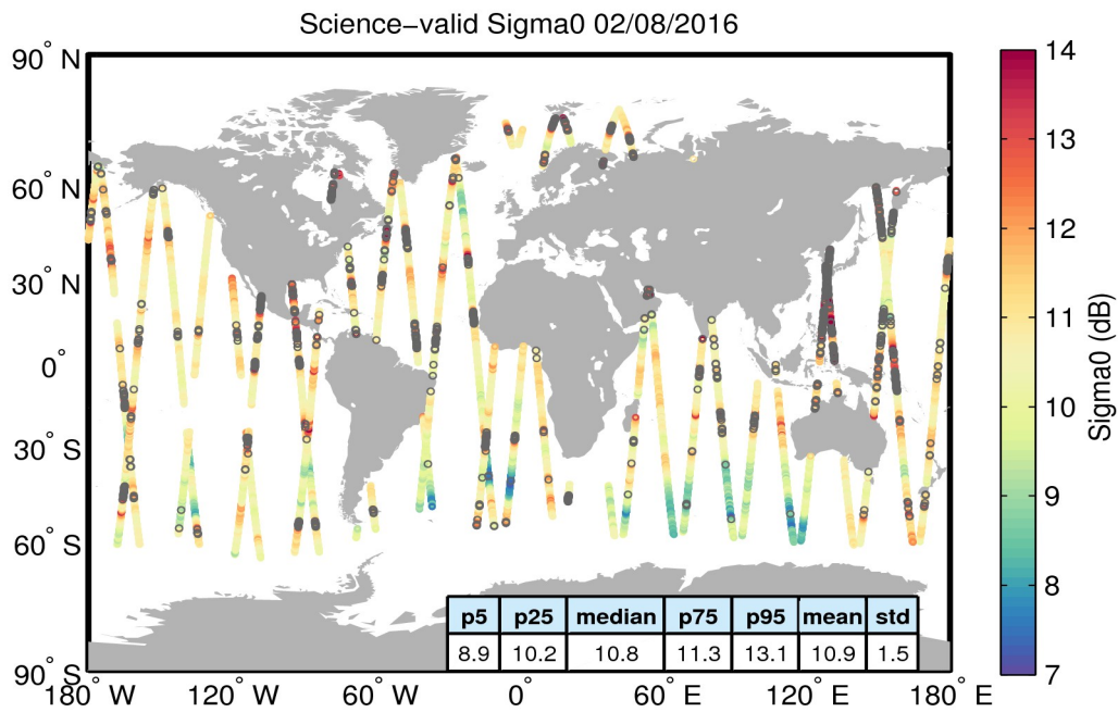
Figure 27. Geographical distribution of science-valid sigma0 data over oceans and lakes for 02/08/2016. The statistical values shown in the table refer to the sigma0 in dB and are calculated over all measurements shown in the figure. Gray circles denote records that have been rejected based on the editing criteria described in Table 4.
