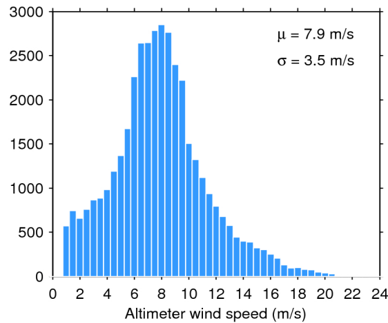
Figure 33. Histogram of flag-valid wind over oceans and lakes for 02/08/2016. The mean ( \mu ) and standard deviation ( \sigma ) are also shown. Note that values larger than 24 m/s are excluded from the histogram for the sake of readability but not from the computation of \mu and \sigma .
