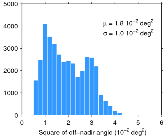
Figure 39. Histogram of flag-valid mispointing over oceans and lakes for 02/08/2016. The mean ( \mu ) and standard deviation ( \sigma ) are also shown. Note that values larger than 6 \cdot 10^{-2} \text{ deg}^2 are excluded from the histogram for the sake of readability but not from the computation of \mu and \sigma .
