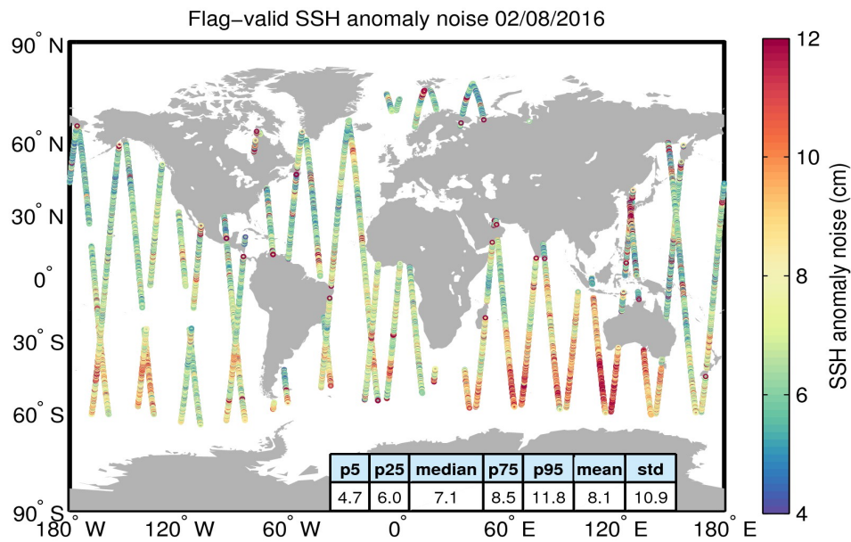
Figure 8. Geographical distribution of flag-valid 20-Hz SSH anomaly measurement noise over oceans and lakes for 02/08/2016. The statistical values shown in the table refer to the SSH anomaly noise and are calculated over all measurements shown in the figure.
