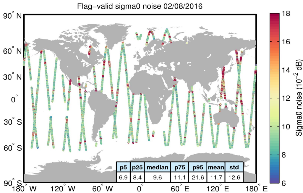
Figure 26. Geographical distribution of flag-valid 20-Hz sigma0 measurement noise over oceans and lakes for 02/08/2016. The statistical values shown in the table refer to the sigma0 noise and are calculated over all measurements shown in the figure.
