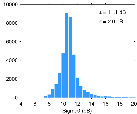
Figure 25. Histogram of flag-valid sigma0 over oceans and lakes for 02/08/2016. The mean ( \mu ) and standard deviation ( \sigma ) are also shown. Note that values outside [4 20] dB are excluded from the histogram for the sake of readability but not from the computation of \mu and \sigma .
