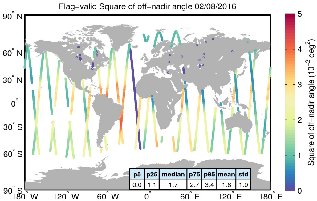
Figure 37. Geographical distribution of flag-valid mispointing data over oceans and lakes for 02/08/2016. The statistical values shown in the table refer to the mispointing in 10^{-2} deg 2 and are calculated over all measurements shown in the figure.
