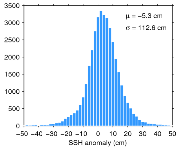
Figure 7. Histogram of flag-valid SSH anomaly over oceans and lakes for 02/08/2016. The mean ( \mu ) and standard deviation ( \sigma ) are also shown. Note that values outside [-50 50] cm are excluded from the histogram for the sake of readability but not from the computation of \mu and \sigma .
