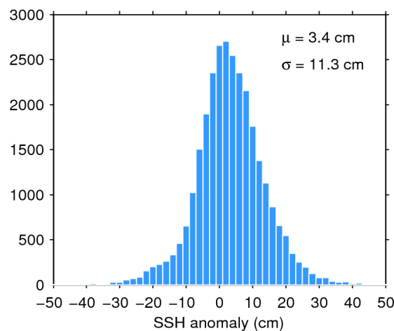
Figure 11. Histogram of science-valid SSH anomaly over oceans and lakes for 02/08/2016. The mean ( \mu ) and standard deviation ( \sigma ) are also shown. Note that values outside [-50 50] cm are excluded from the histogram for the sake of readability but not from the computation of \mu and \sigma .
