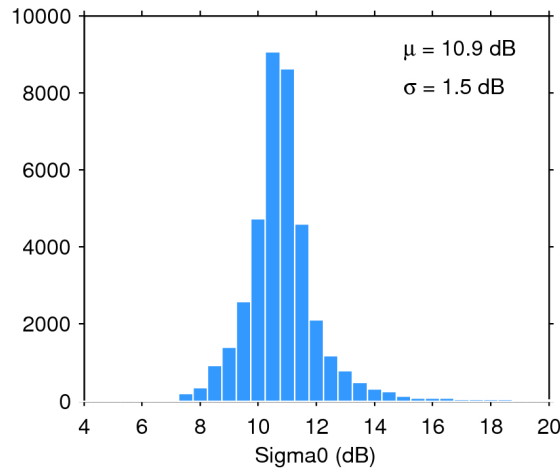
Figure 28. Histogram of science-valid sigma0 over oceans and lakes for 02/08/2016. The mean ( \mu ) and standard deviation ( \sigma ) are also shown. Note that values outside [4 20] dB are excluded from the histogram for the sake of readability but not from the computation of \mu and \sigma .
