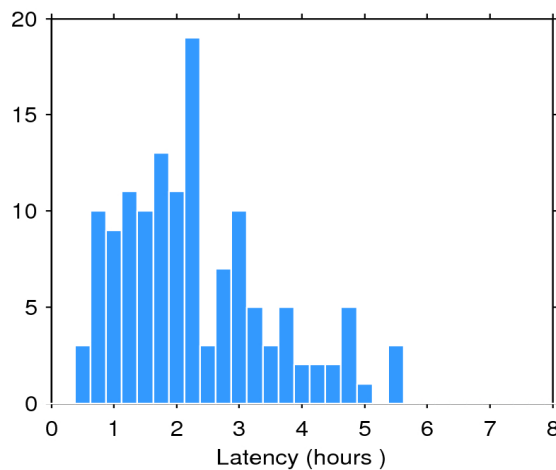
Figure 2. Histogram of the data latency for 02/08/2016. The y-axis denotes the number of files that are made available with a delay of x-hours with respect to the mean time of the records stored in the file.
