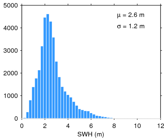
Figure 20. Histogram of science-valid SWH over oceans and lakes for 02/08/2016. The mean ( \mu ) and standard deviation ( \sigma ) are also shown. Note that values larger than 12 m are excluded from the histogram for the sake of readability but not from the computation of \mu and \sigma .
