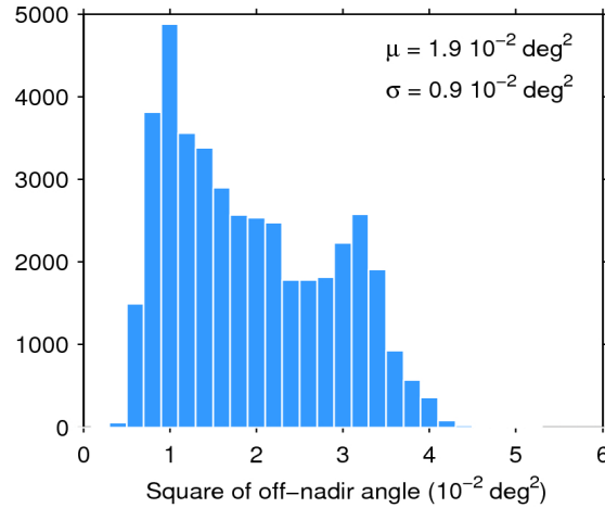
Figure 39. Histogram of flag-valid mispointing over oceans and lakes for 01/08/2016. The mean ( \mu ) and standard deviation ( \sigma ) are also shown. Note that values larger than 6 \cdot 10^{-2} \text{ deg}^2 are excluded from the histogram for the sake of readability but not from the computation of \mu and \sigma .
