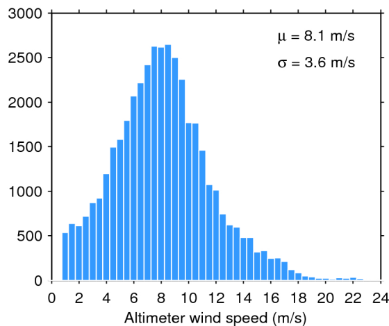
Figure 35. Histogram of science-valid wind over oceans and lakes for 01/08/2016. The mean ( \mu ) and standard deviation ( \sigma ) are also shown. Note that values larger than 24 m/s are excluded from the histogram for the sake of readability but not from the computation of \mu and \sigma .
