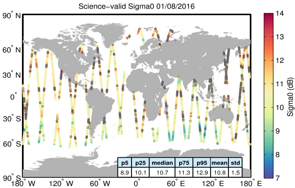
Figure 27. Geographical distribution of science-valid sigma0 data over oceans and lakes for 01/08/2016. The statistical values shown in the table refer to the sigma0 in dB and are calculated over all measurements shown in the figure. Gray circles denote records that have been rejected based on the editing criteria described in Table 4.
