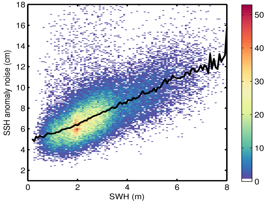
Figure 9. 2D histogram showing flag-valid SSH anomaly noise as a function of SWH for 01/08/2016. The black line denotes the median SSH anomaly noise as a function of SWH.
