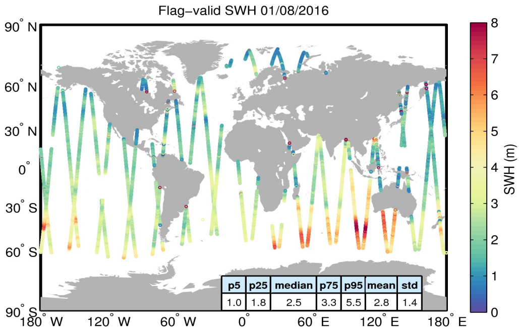
Figure 15. Geographical distribution of flag-valid SWH data over oceans and lakes for 01/08/2016. The statistical values shown in the table refer to the SWH in m and are calculated over all measurements shown in the figure.
