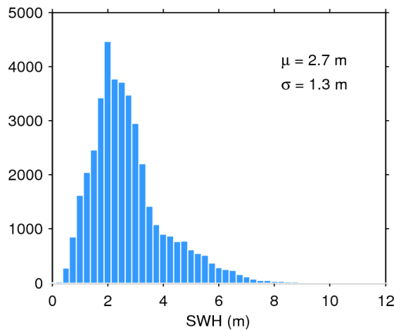
Figure 20. Histogram of science-valid SWH over oceans and lakes for 01/08/2016. The mean ( \mu ) and standard deviation ( \sigma ) are also shown. Note that values larger than 12 m are excluded from the histogram for the sake of readability but not from the computation of \mu and \sigma .
