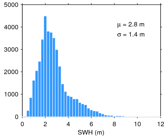
Figure 17. Histogram of flag-valid SWH over oceans and lakes for 01/08/2016. The mean ( \mu ) and standard deviation ( \sigma ) are also shown. Note that values larger than 12 m are excluded from the histogram for the sake of readability but not from the computation of \mu and \sigma .
