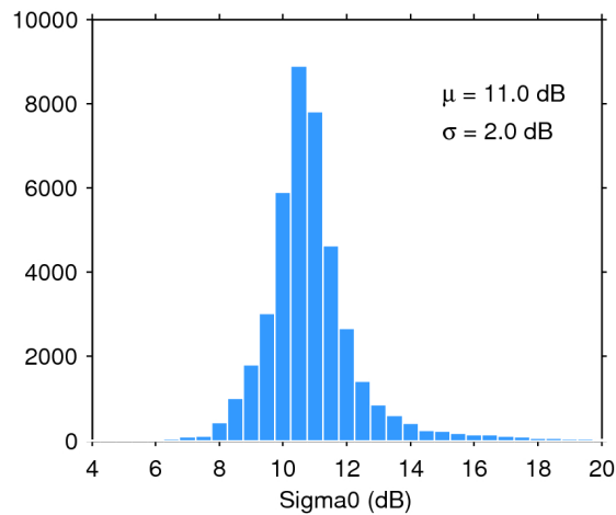
Figure 25. Histogram of flag-valid sigma0 over oceans and lakes for 01/08/2016. The mean ( \mu ) and standard deviation ( \sigma ) are also shown. Note that values outside [4 20] dB are excluded from the histogram for the sake of readability but not from the computation of \mu and \sigma .
