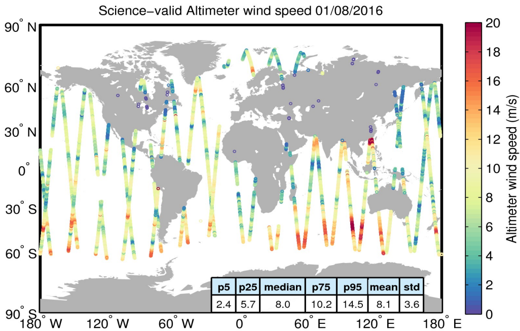
Figure 34. Geographical distribution of science-valid wind data over oceans and lakes for 01/08/2016. The statistical values shown in the table refer to the wind in m/s and are calculated over all measurements shown in the figure. Gray circles denote records that have been rejected based on the editing criteria described in Table 5.
