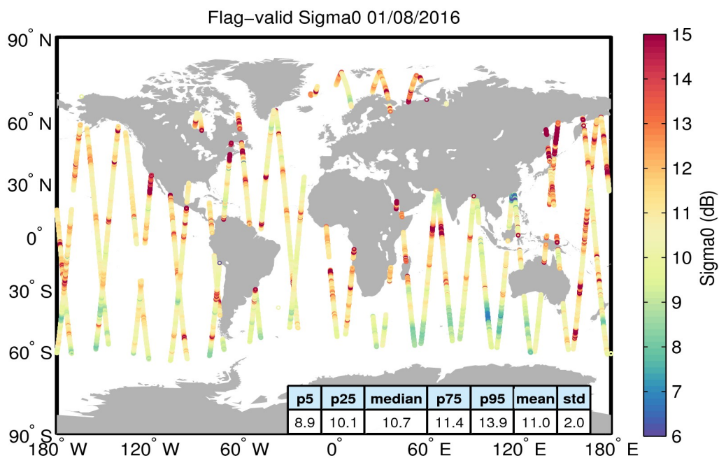
Figure 23. Geographical distribution of flag-valid sigma0 data over oceans and lakes for 01/08/2016. The statistical values shown in the table refer to the sigma0 in dB and are calculated over all measurements shown in the figure.
