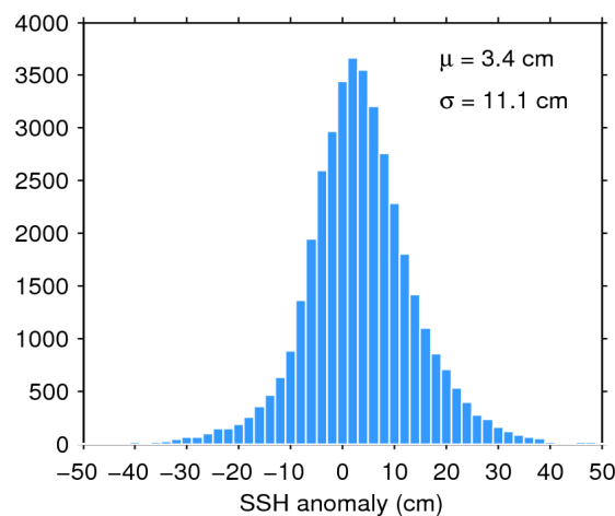
Figure 11. Histogram of science-valid SSH anomaly over oceans and lakes for 01/08/2016. The mean ( \mu ) and standard deviation ( \sigma ) are also shown. Note that values outside [-50 50] cm are excluded from the histogram for the sake of readability but not from the computation of \mu and \sigma .
