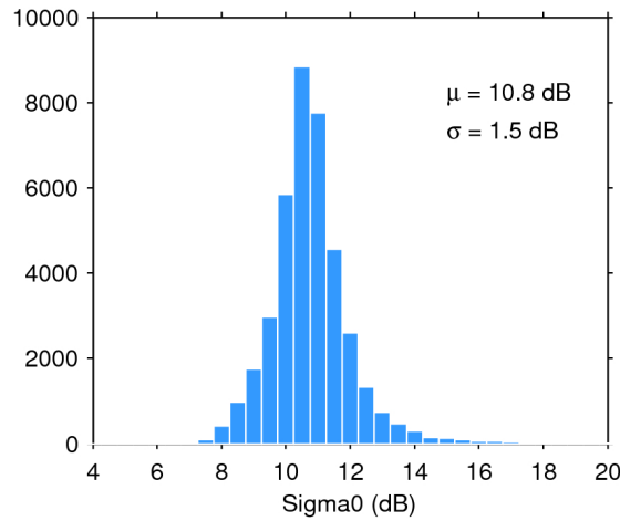
Figure 28. Histogram of science-valid sigma0 over oceans and lakes for 01/08/2016. The mean ( \mu ) and standard deviation ( \sigma ) are also shown. Note that values outside [4 20] dB are excluded from the histogram for the sake of readability but not from the computation of \mu and \sigma .
