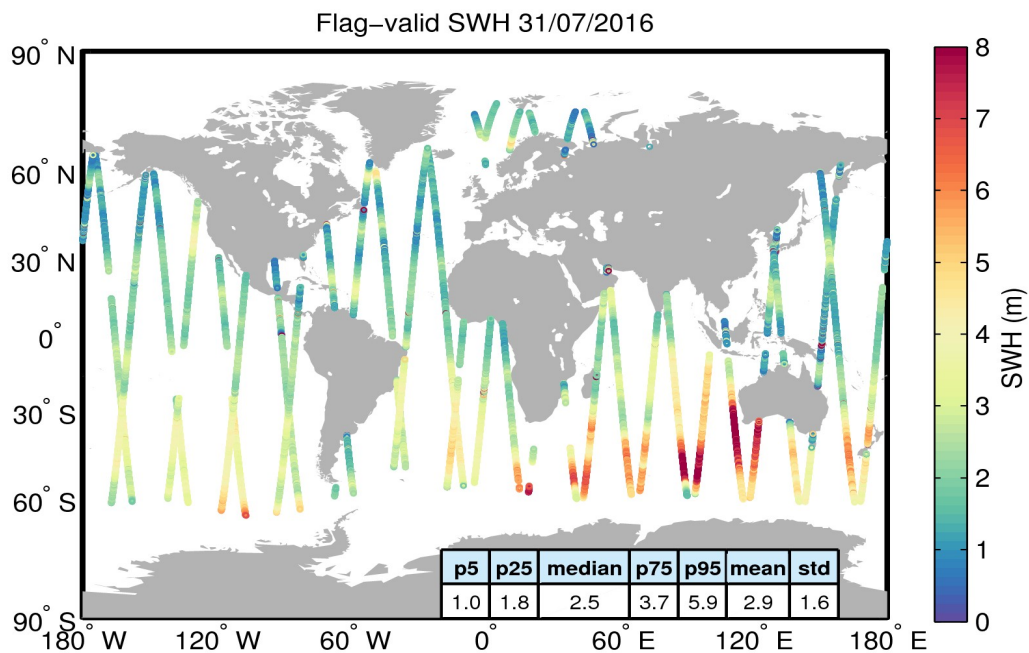
Figure 15. Geographical distribution of flag-valid SWH data over oceans and lakes for 31/07/2016. The statistical values shown in the table refer to the SWH in m and are calculated over all measurements shown in the figure.
