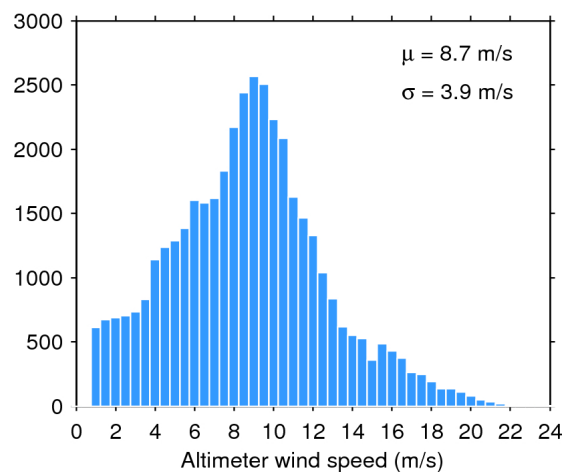
Figure 35. Histogram of science-valid wind over oceans and lakes for 31/07/2016. The mean ( \mu ) and standard deviation ( \sigma ) are also shown. Note that values larger than 24 m/s are excluded from the histogram for the sake of readability but not from the computation of \mu and \sigma .
