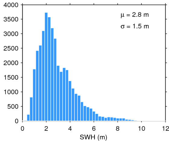
Figure 20. Histogram of science-valid SWH over oceans and lakes for 31/07/2016. The mean ( \mu ) and standard deviation ( \sigma ) are also shown. Note that values larger than 12 m are excluded from the histogram for the sake of readability but not from the computation of \mu and \sigma .
