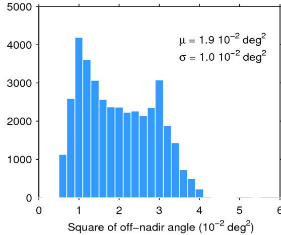
Figure 39. Histogram of flag-valid mispointing over oceans and lakes for 31/07/2016. The mean ( \mu ) and standard deviation ( \sigma ) are also shown. Note that values larger than 6 \cdot 10^{-2} \text{ deg}^2 are excluded from the histogram for the sake of readability but not from the computation of \mu and \sigma .
