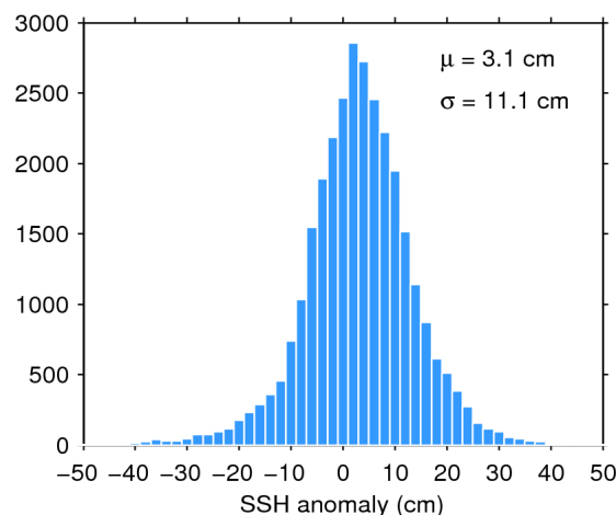
Figure 11. Histogram of science-valid SSH anomaly over oceans and lakes for 31/07/2016. The mean ( \mu ) and standard deviation ( \sigma ) are also shown. Note that values outside [-50 50] cm are excluded from the histogram for the sake of readability but not from the computation of \mu and \sigma .
