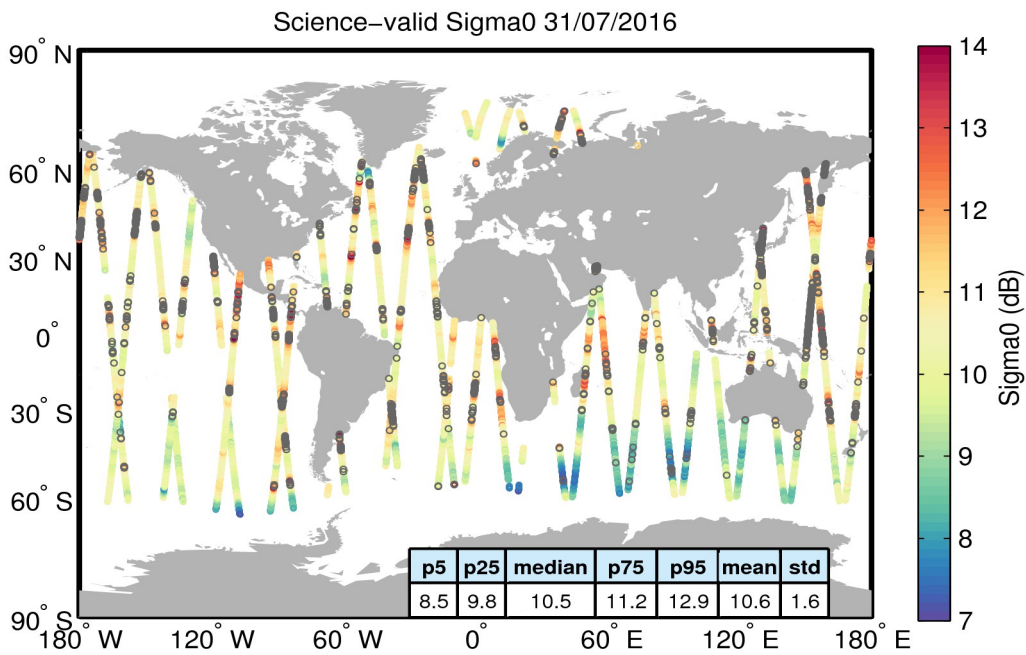
Figure 27. Geographical distribution of science-valid sigma0 data over oceans and lakes for 31/07/2016. The statistical values shown in the table refer to the sigma0 in dB and are calculated over all measurements shown in the figure. Gray circles denote records that have been rejected based on the editing criteria described in Table 4.
