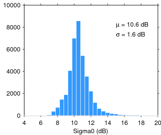
Figure 28. Histogram of science-valid sigma0 over oceans and lakes for 31/07/2016. The mean ( \mu ) and standard deviation ( \sigma ) are also shown. Note that values outside [4 20] dB are excluded from the histogram for the sake of readability but not from the computation of \mu and \sigma .
