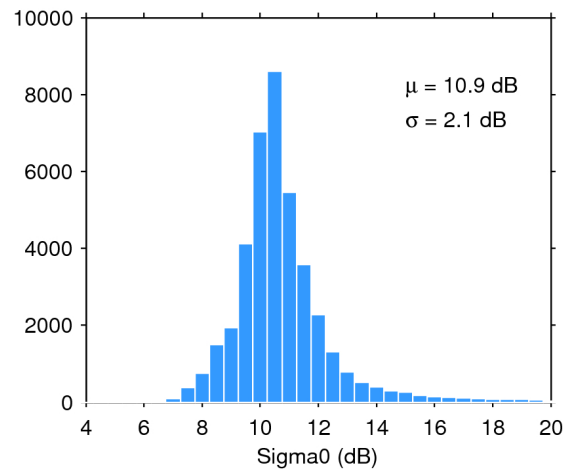
Figure 25. Histogram of flag-valid sigma0 over oceans and lakes for 31/07/2016. The mean ( \mu ) and standard deviation ( \sigma ) are also shown. Note that values outside [4 20] dB are excluded from the histogram for the sake of readability but not from the computation of \mu and \sigma .
