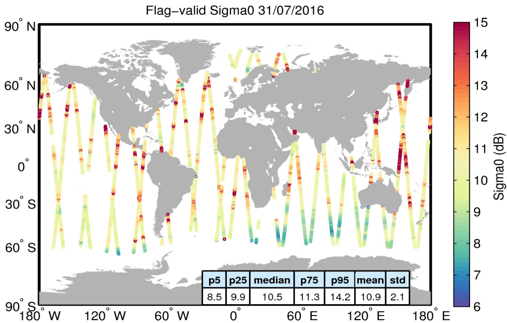
Figure 23. Geographical distribution of flag-valid sigma0 data over oceans and lakes for 31/07/2016. The statistical values shown in the table refer to the sigma0 in dB and are calculated over all measurements shown in the figure.
