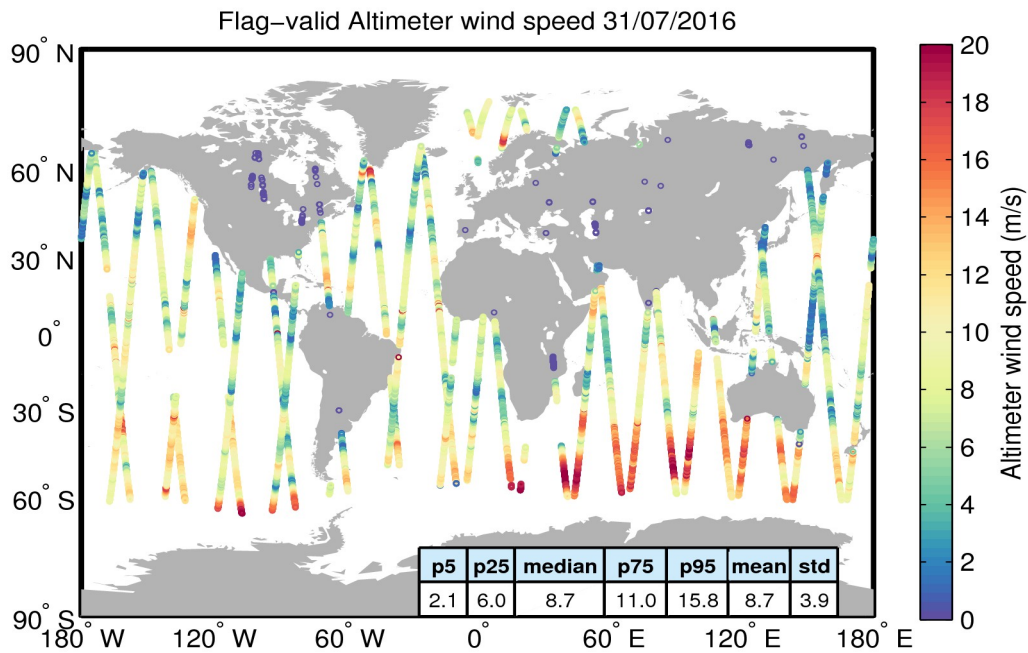
Figure 31. Geographical distribution of flag-valid wind data over oceans and lakes for 31/07/2016. The statistical values shown in the table refer to the wind in m/s and are calculated over all measurements shown in the figure.
