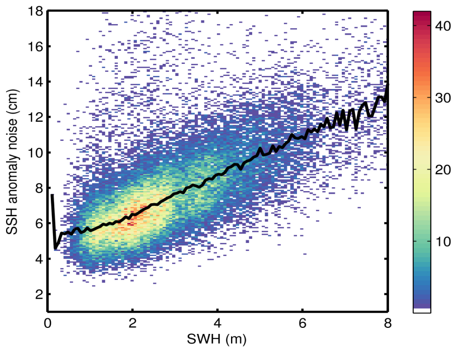
Figure 9. 2D histogram showing flag-valid SSH anomaly noise as a function of SWH for 31/07/2016. The black line denotes the median SSH anomaly noise as a function of SWH.
