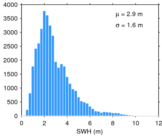
Figure 17. Histogram of flag-valid SWH over oceans and lakes for 31/07/2016. The mean ( \mu ) and standard deviation ( \sigma ) are also shown. Note that values larger than 12 m are excluded from the histogram for the sake of readability but not from the computation of \mu and \sigma .
