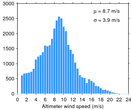
Figure 33. Histogram of flag-valid wind over oceans and lakes for 31/07/2016. The mean ( \mu ) and standard deviation ( \sigma ) are also shown. Note that values larger than 24 m/s are excluded from the histogram for the sake of readability but not from the computation of \mu and \sigma .
