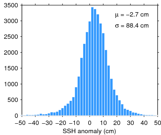
Figure 7. Histogram of flag-valid SSH anomaly over oceans and lakes for 31/07/2016. The mean ( \mu ) and standard deviation ( \sigma ) are also shown. Note that values outside [-50 50] cm are excluded from the histogram for the sake of readability but not from the computation of \mu and \sigma .
