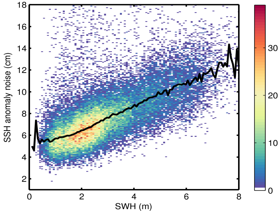
Figure 9. 2D histogram showing flag-valid SSH anomaly noise as a function of SWH for 30/07/2016. The black line denotes the median SSH anomaly noise as a function of SWH.
