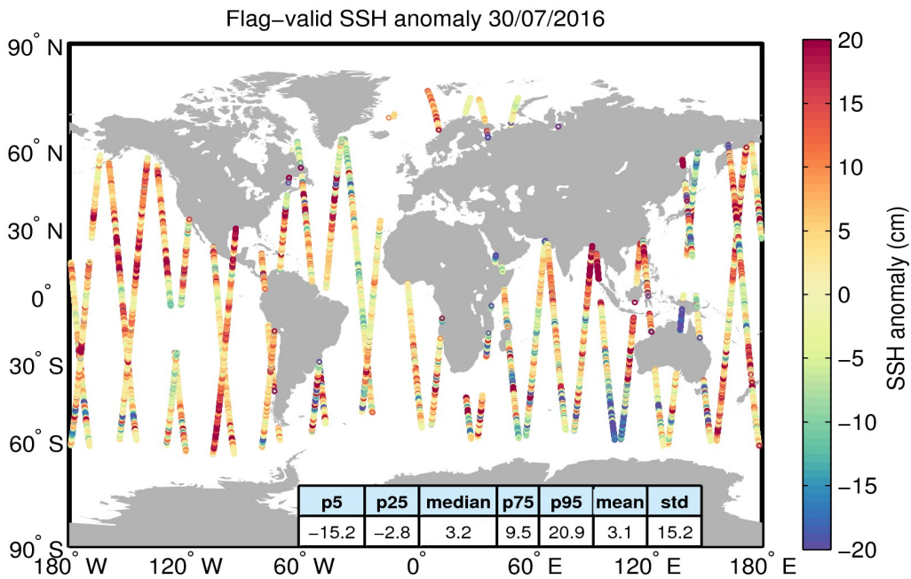
Figure 5. Geographical distribution of flag-valid 1-Hz SSH anomaly data over oceans and lakes for 30/07/2016. The statistical values shown in the table refer to the SSH anomaly in cm and are calculated over all measurements shown in the figure.
