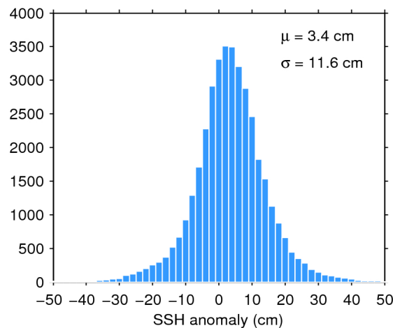
Figure 11. Histogram of science-valid SSH anomaly over oceans and lakes for 30/07/2016. The mean ( \mu ) and standard deviation ( \sigma ) are also shown. Note that values outside [-50 50] cm are excluded from the histogram for the sake of readability but not from the computation of \mu and \sigma .
