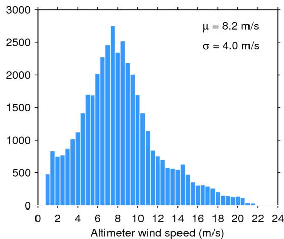
Figure 35. Histogram of science-valid wind over oceans and lakes for 30/07/2016. The mean ( \mu ) and standard deviation ( \sigma ) are also shown. Note that values larger than 24 m/s are excluded from the histogram for the sake of readability but not from the computation of \mu and \sigma .
