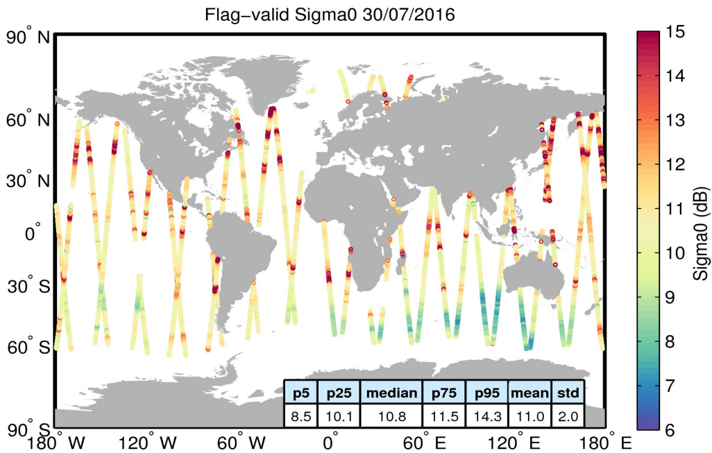
Figure 23. Geographical distribution of flag-valid sigma0 data over oceans and lakes for 30/07/2016. The statistical values shown in the table refer to the sigma0 in dB and are calculated over all measurements shown in the figure.
