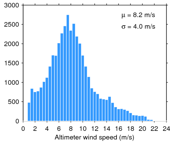
Figure 33. Histogram of flag-valid wind over oceans and lakes for 30/07/2016. The mean ( \mu ) and standard deviation ( \sigma ) are also shown. Note that values larger than 24 m/s are excluded from the histogram for the sake of readability but not from the computation of \mu and \sigma .
