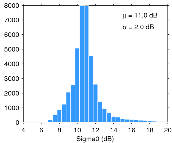
Figure 25. Histogram of flag-valid sigma0 over oceans and lakes for 30/07/2016. The mean ( \mu ) and standard deviation ( \sigma ) are also shown. Note that values outside [4 20] dB are excluded from the histogram for the sake of readability but not from the computation of \mu and \sigma .
