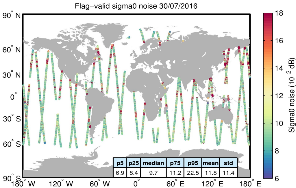
Figure 26. Geographical distribution of flag-valid 20-Hz sigma0 measurement noise over oceans and lakes for 30/07/2016. The statistical values shown in the table refer to the sigma0 noise and are calculated over all measurements shown in the figure.
