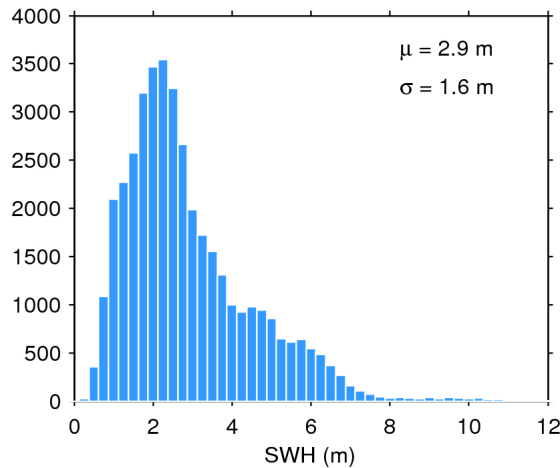
Figure 20. Histogram of science-valid SWH over oceans and lakes for 30/07/2016. The mean ( \mu ) and standard deviation ( \sigma ) are also shown. Note that values larger than 12 m are excluded from the histogram for the sake of readability but not from the computation of \mu and \sigma .
