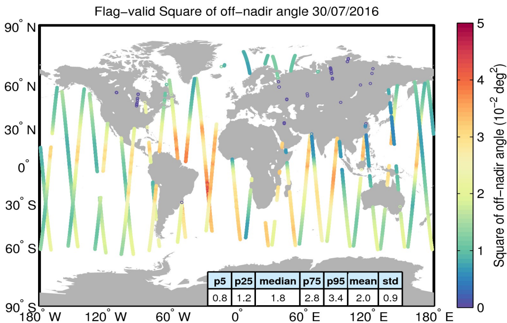
Figure 37. Geographical distribution of flag-valid mispointing data over oceans and lakes for 30/07/2016. The statistical values shown in the table refer to the mispointing in 10^{-2} deg 2 and are calculated over all measurements shown in the figure.
