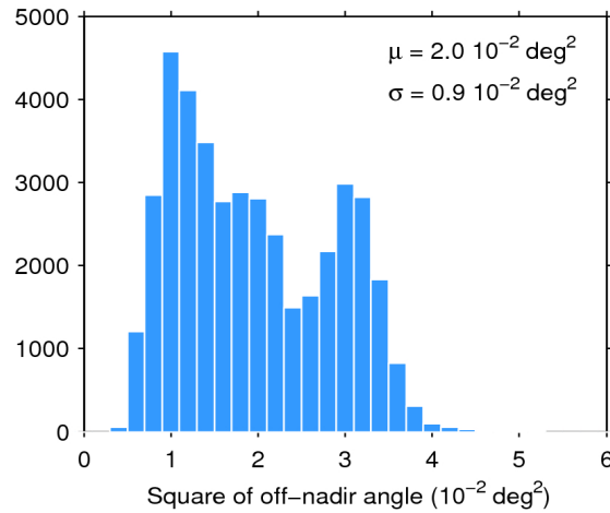
Figure 39. Histogram of flag-valid mispointing over oceans and lakes for 30/07/2016. The mean ( \mu ) and standard deviation ( \sigma ) are also shown. Note that values larger than 6 \cdot 10^{-2} \text{ deg}^2 are excluded from the histogram for the sake of readability but not from the computation of \mu and \sigma .
