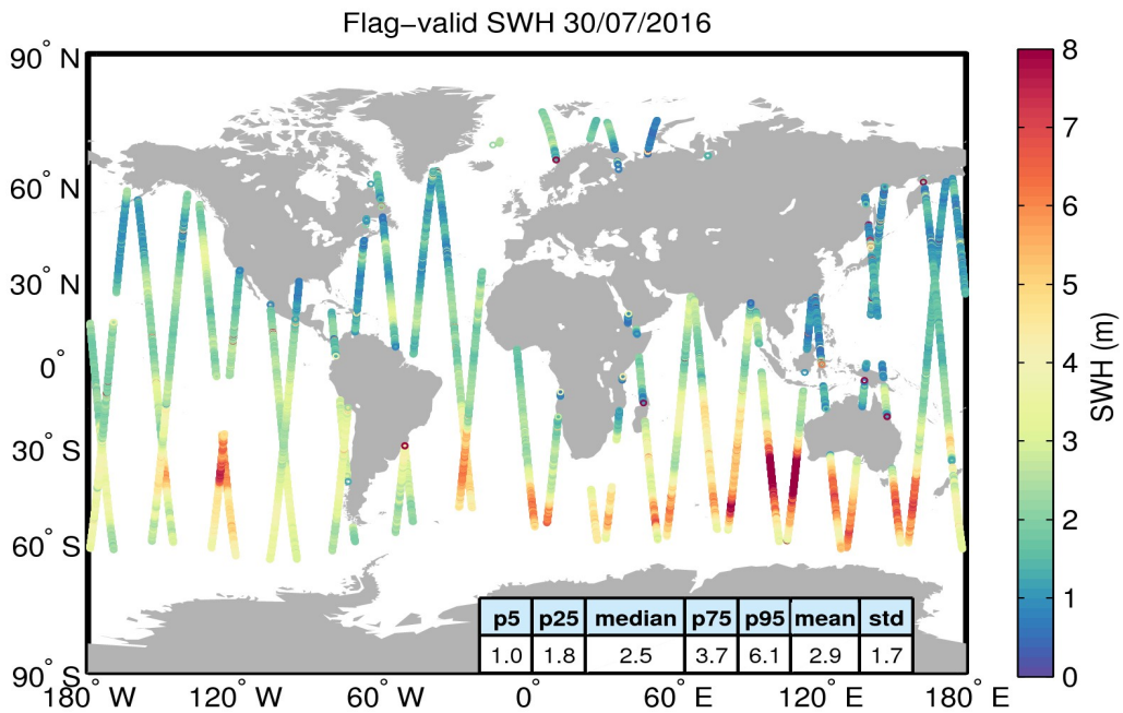
Figure 15. Geographical distribution of flag-valid SWH data over oceans and lakes for 30/07/2016. The statistical values shown in the table refer to the SWH in m and are calculated over all measurements shown in the figure.
