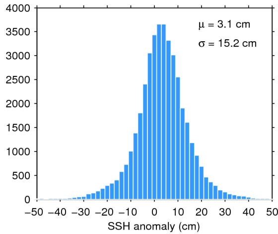
Figure 7. Histogram of flag-valid SSH anomaly over oceans and lakes for 30/07/2016. The mean ( \mu ) and standard deviation ( \sigma ) are also shown. Note that values outside [-50 50] cm are excluded from the histogram for the sake of readability but not from the computation of \mu and \sigma .
