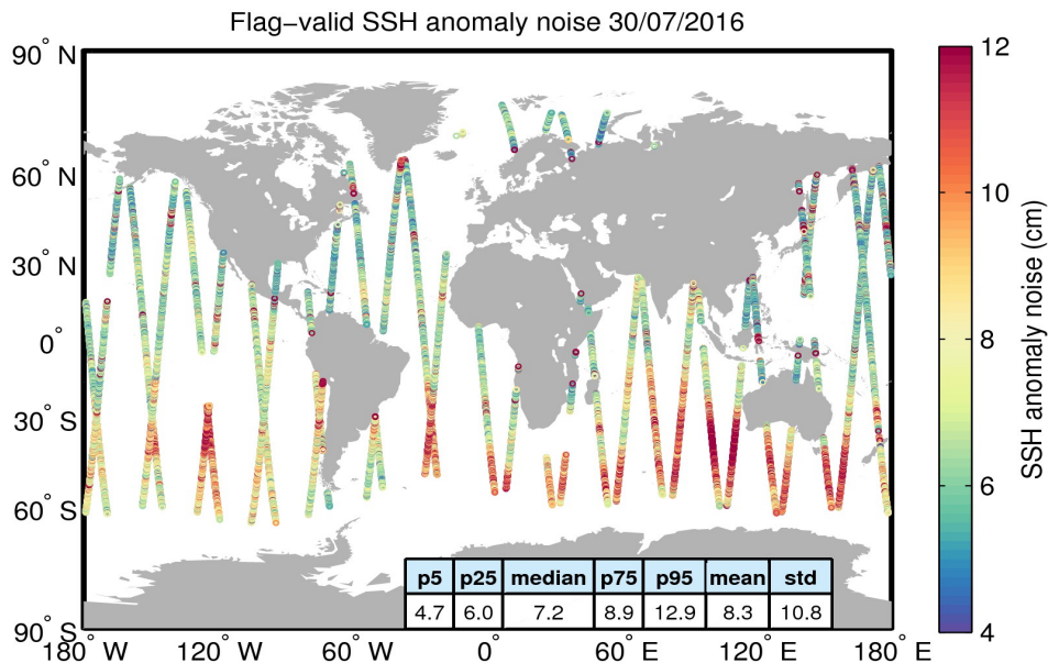
Figure 8. Geographical distribution of flag-valid 20-Hz SSH anomaly measurement noise over oceans and lakes for 30/07/2016. The statistical values shown in the table refer to the SSH anomaly noise and are calculated over all measurements shown in the figure.
