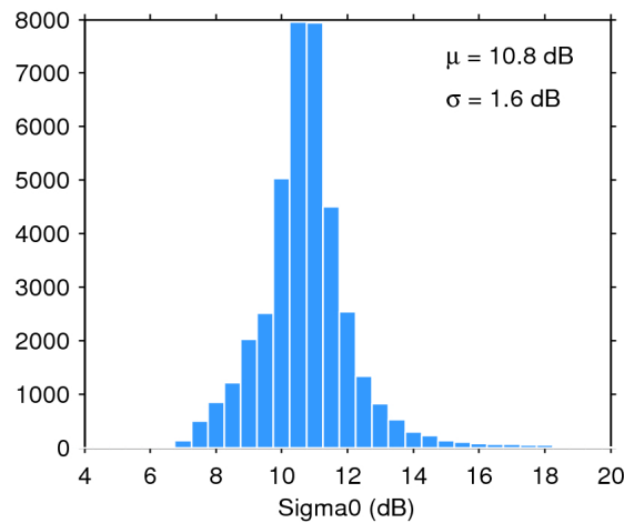
Figure 28. Histogram of science-valid sigma0 over oceans and lakes for 30/07/2016. The mean ( \mu ) and standard deviation ( \sigma ) are also shown. Note that values outside [4 20] dB are excluded from the histogram for the sake of readability but not from the computation of \mu and \sigma .
