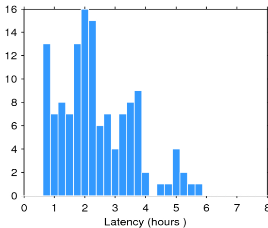
Figure 2. Histogram of the data latency for 30/07/2016. The y-axis denotes the number of files that are made available with a delay of x-hours with respect to the mean time of the records stored in the file.
