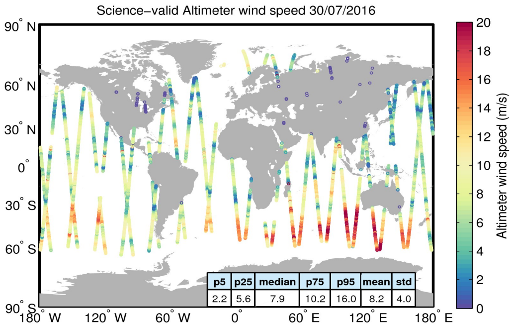
Figure 34. Geographical distribution of science-valid wind data over oceans and lakes for 30/07/2016. The statistical values shown in the table refer to the wind in m/s and are calculated over all measurements shown in the figure. Gray circles denote records that have been rejected based on the editing criteria described in Table 5.
