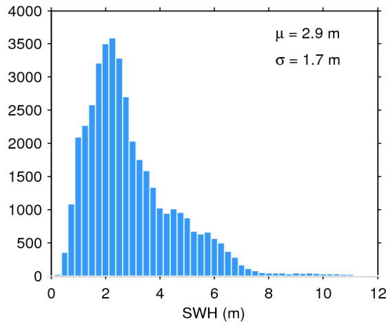
Figure 17. Histogram of flag-valid SWH over oceans and lakes for 30/07/2016. The mean ( \mu ) and standard deviation ( \sigma ) are also shown. Note that values larger than 12 m are excluded from the histogram for the sake of readability but not from the computation of \mu and \sigma .
