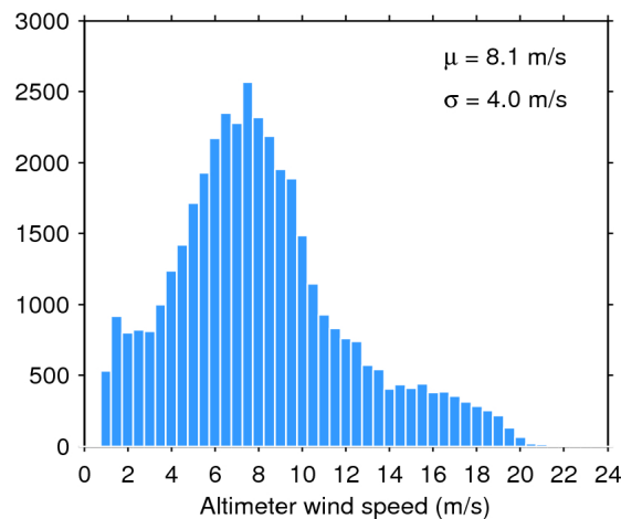
Figure 35. Histogram of science-valid wind over oceans and lakes for 28/07/2016. The mean ( \mu ) and standard deviation ( \sigma ) are also shown. Note that values larger than 24 m/s are excluded from the histogram for the sake of readability but not from the computation of \mu and \sigma .
