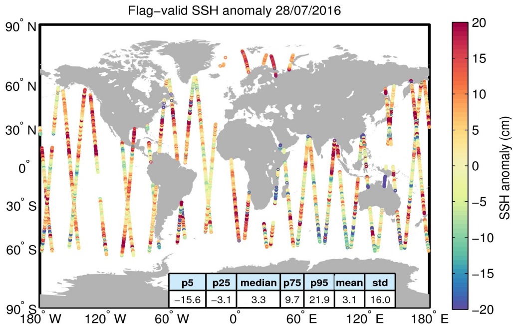
Figure 5. Geographical distribution of flag-valid 1-Hz SSH anomaly data over oceans and lakes for 28/07/2016. The statistical values shown in the table refer to the SSH anomaly in cm and are calculated over all measurements shown in the figure.
