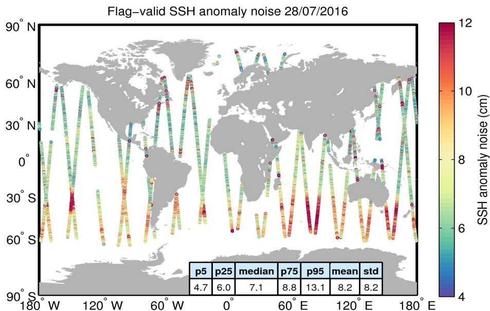
Figure 8. Geographical distribution of flag-valid 20-Hz SSH anomaly measurement noise over oceans and lakes for 28/07/2016. The statistical values shown in the table refer to the SSH anomaly noise and are calculated over all measurements shown in the figure.
