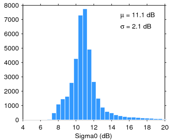
Figure 25. Histogram of flag-valid sigma0 over oceans and lakes for 28/07/2016. The mean ( \mu ) and standard deviation ( \sigma ) are also shown. Note that values outside [4 20] dB are excluded from the histogram for the sake of readability but not from the computation of \mu and \sigma .
