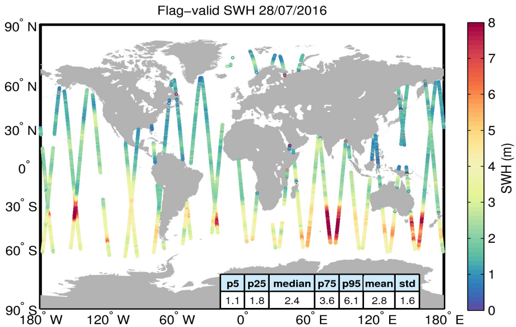
Figure 15. Geographical distribution of flag-valid SWH data over oceans and lakes for 28/07/2016. The statistical values shown in the table refer to the SWH in m and are calculated over all measurements shown in the figure.
