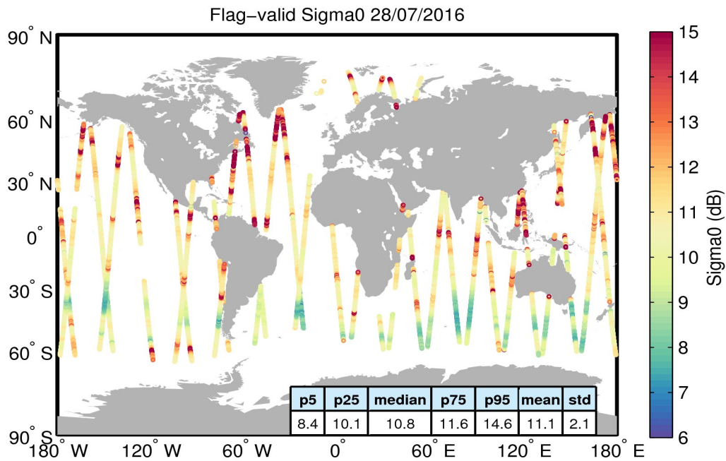
Figure 23. Geographical distribution of flag-valid sigma0 data over oceans and lakes for 28/07/2016. The statistical values shown in the table refer to the sigma0 in dB and are calculated over all measurements shown in the figure.
