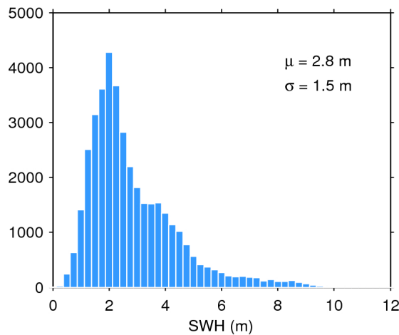
Figure 20. Histogram of science-valid SWH over oceans and lakes for 28/07/2016. The mean ( \mu ) and standard deviation ( \sigma ) are also shown. Note that values larger than 12 m are excluded from the histogram for the sake of readability but not from the computation of \mu and \sigma .
