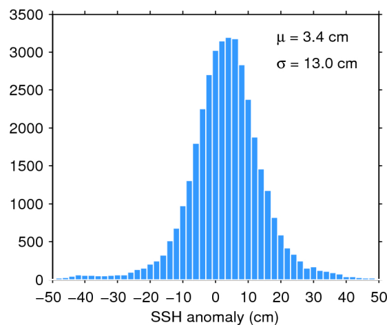
Figure 11. Histogram of science-valid SSH anomaly over oceans and lakes for 28/07/2016. The mean ( \mu ) and standard deviation ( \sigma ) are also shown. Note that values outside [-50 50] cm are excluded from the histogram for the sake of readability but not from the computation of \mu and \sigma .
