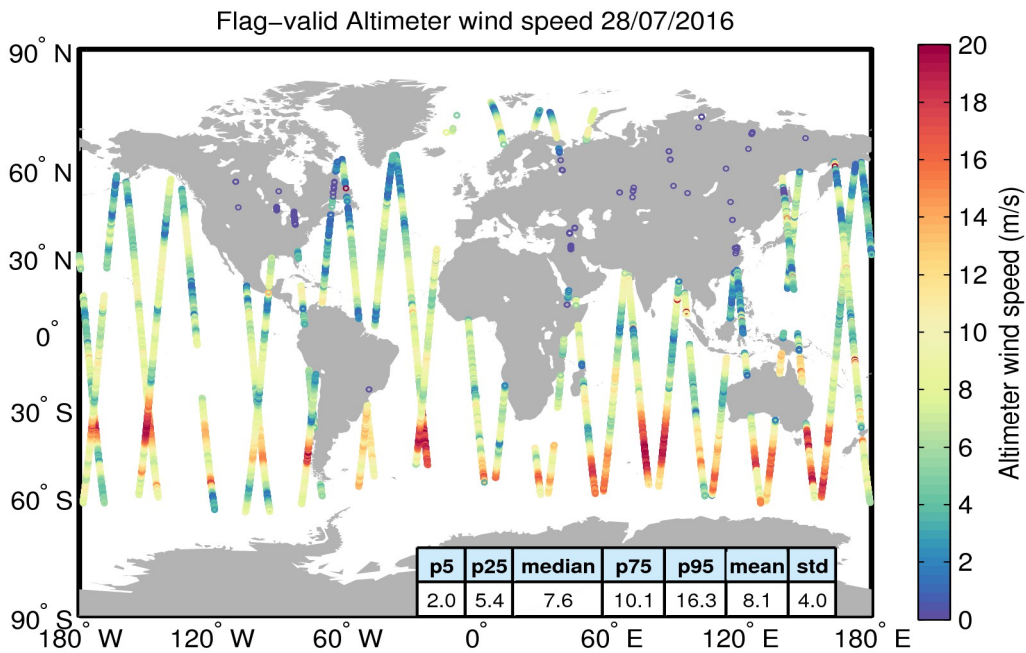
Figure 31. Geographical distribution of flag-valid wind data over oceans and lakes for 28/07/2016. The statistical values shown in the table refer to the wind in m/s and are calculated over all measurements shown in the figure.
