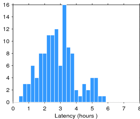
Figure 2. Histogram of the data latency for 28/07/2016. The y-axis denotes the number of files that are made available with a delay of x-hours with respect to the mean time of the records stored in the file.
