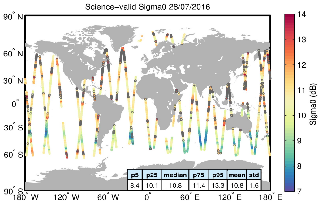
Figure 27. Geographical distribution of science-valid sigma0 data over oceans and lakes for 28/07/2016. The statistical values shown in the table refer to the sigma0 in dB and are calculated over all measurements shown in the figure. Gray circles denote records that have been rejected based on the editing criteria described in Table 4.
