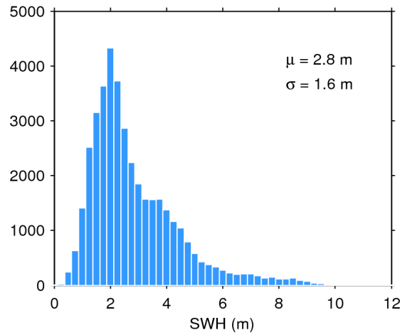
Figure 17. Histogram of flag-valid SWH over oceans and lakes for 28/07/2016. The mean ( \mu ) and standard deviation ( \sigma ) are also shown. Note that values larger than 12 m are excluded from the histogram for the sake of readability but not from the computation of \mu and \sigma .
