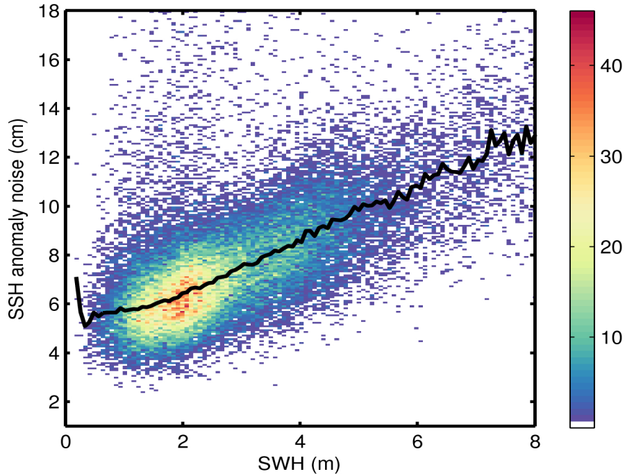
Figure 9. 2D histogram showing flag-valid SSH anomaly noise as a function of SWH for 28/07/2016. The black line denotes the median SSH anomaly noise as a function of SWH.
