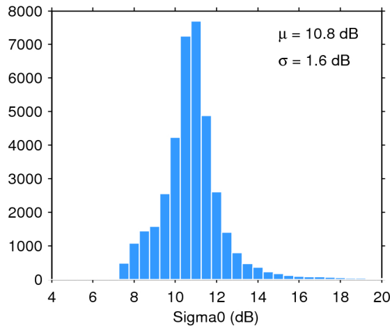
Figure 28. Histogram of science-valid sigma0 over oceans and lakes for 28/07/2016. The mean ( \mu ) and standard deviation ( \sigma ) are also shown. Note that values outside [4 20] dB are excluded from the histogram for the sake of readability but not from the computation of \mu and \sigma .
