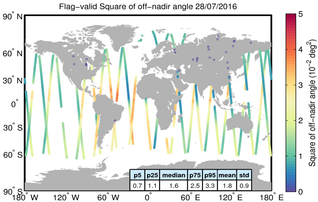
Figure 37. Geographical distribution of flag-valid mispointing data over oceans and lakes for 28/07/2016. The statistical values shown in the table refer to the mispointing in 10^{-2} deg 2 and are calculated over all measurements shown in the figure.
