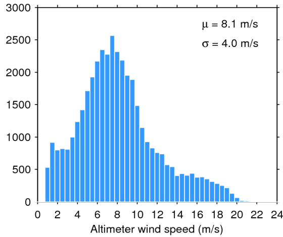
Figure 33. Histogram of flag-valid wind over oceans and lakes for 28/07/2016. The mean ( \mu ) and standard deviation ( \sigma ) are also shown. Note that values larger than 24 m/s are excluded from the histogram for the sake of readability but not from the computation of \mu and \sigma .
