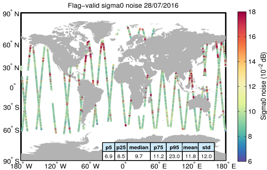
Figure 26. Geographical distribution of flag-valid 20-Hz sigma0 measurement noise over oceans and lakes for 28/07/2016. The statistical values shown in the table refer to the sigma0 noise and are calculated over all measurements shown in the figure.
