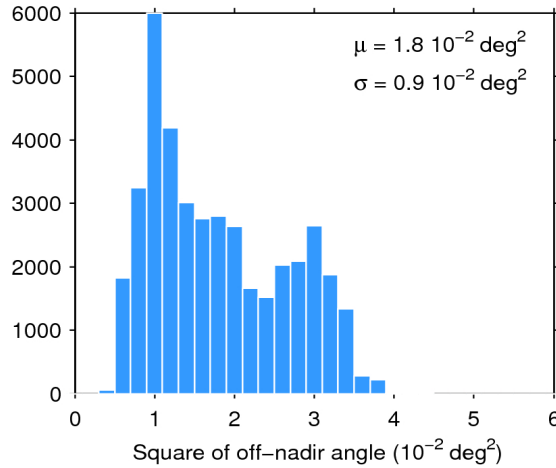
Figure 39. Histogram of flag-valid mispointing over oceans and lakes for 28/07/2016. The mean ( \mu ) and standard deviation ( \sigma ) are also shown. Note that values larger than 6 \cdot 10^{-2} \text{ deg}^2 are excluded from the histogram for the sake of readability but not from the computation of \mu and \sigma .
