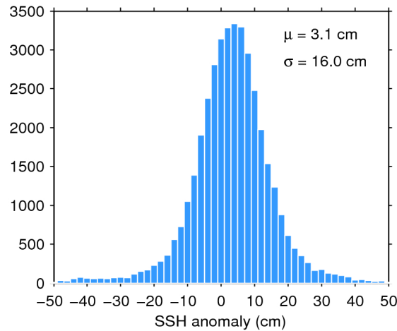
Figure 7. Histogram of flag-valid SSH anomaly over oceans and lakes for 28/07/2016. The mean ( \mu ) and standard deviation ( \sigma ) are also shown. Note that values outside [-50\ 50] cm are excluded from the histogram for the sake of readability but not from the computation of \mu and \sigma .
