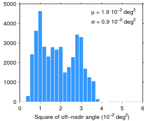
Figure 39. Histogram of flag-valid mispointing over oceans and lakes for 27/07/2016. The mean ( \mu ) and standard deviation ( \sigma ) are also shown. Note that values larger than 6 \cdot 10^{-2} \text{ deg}^2 are excluded from the histogram for the sake of readability but not from the computation of \mu and \sigma .
