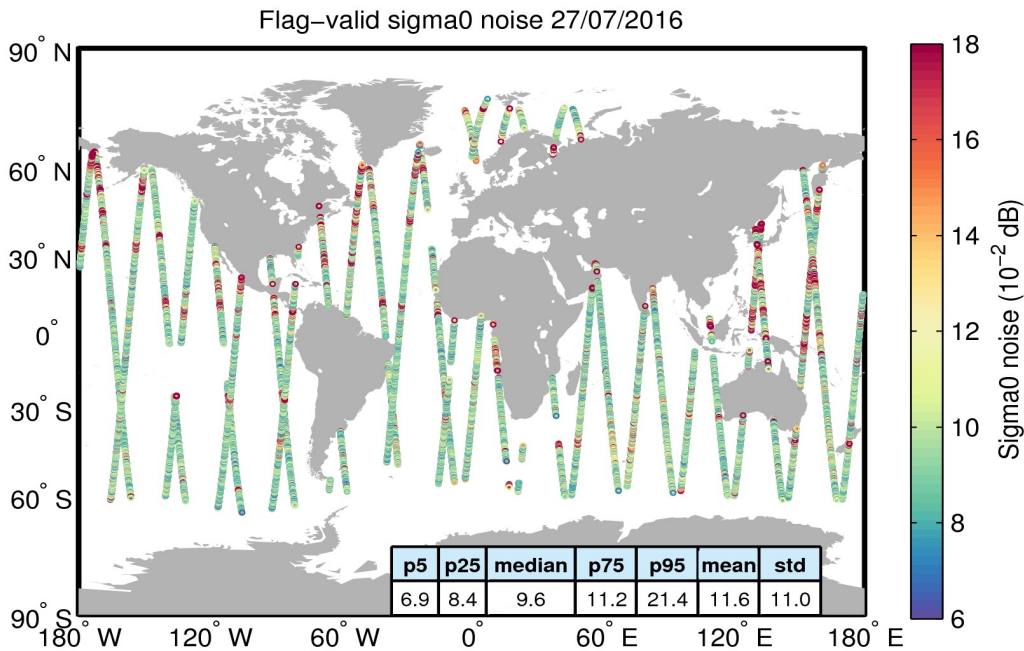
Figure 26. Geographical distribution of flag-valid 20-Hz sigma0 measurement noise over oceans and lakes for 27/07/2016. The statistical values shown in the table refer to the sigma0 noise and are calculated over all measurements shown in the figure.
