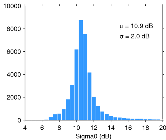
Figure 25. Histogram of flag-valid sigma0 over oceans and lakes for 27/07/2016. The mean ( \mu ) and standard deviation ( \sigma ) are also shown. Note that values outside [4 20] dB are excluded from the histogram for the sake of readability but not from the computation of \mu and \sigma .
