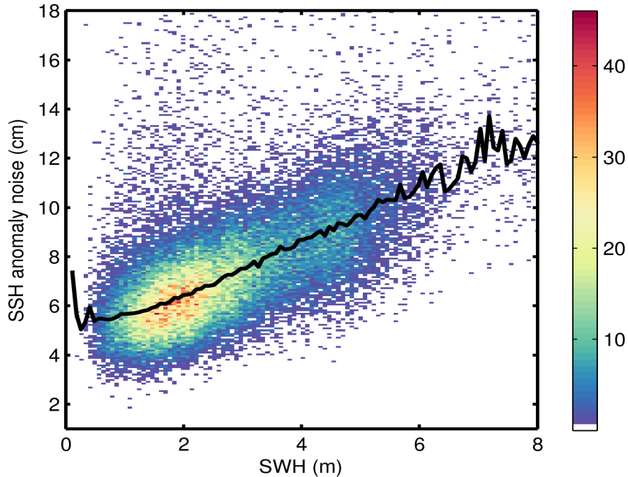
Figure 9. 2D histogram showing flag-valid SSH anomaly noise as a function of SWH for 27/07/2016. The black line denotes the median SSH anomaly noise as a function of SWH.
