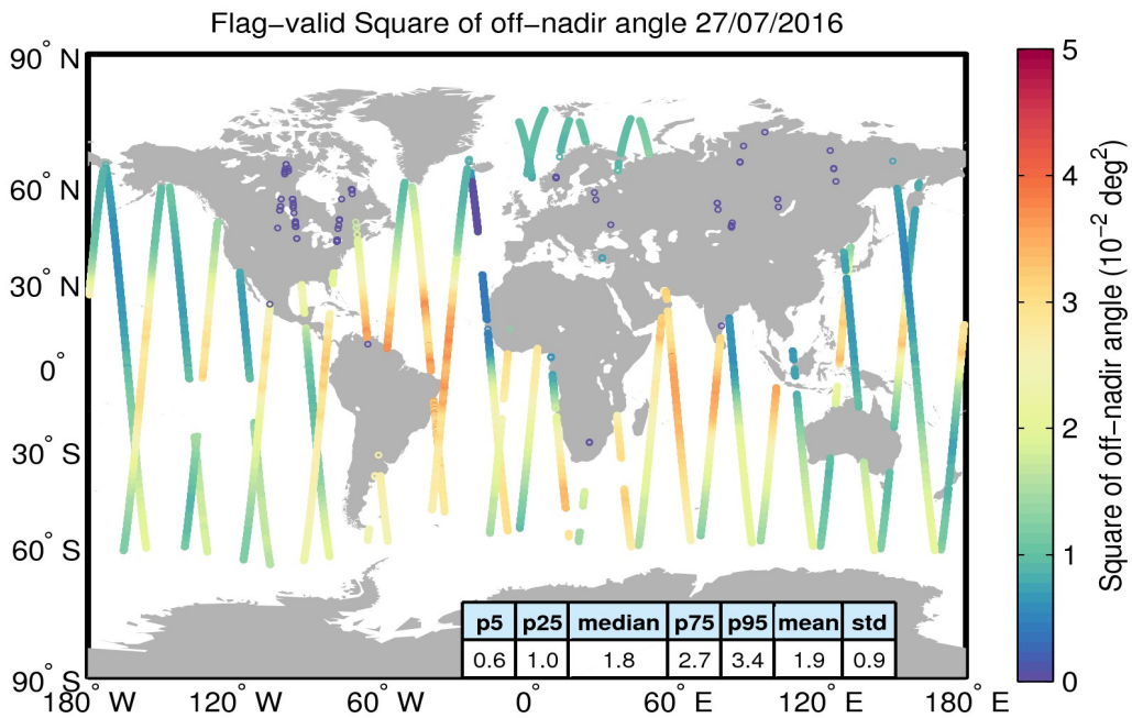
Figure 37. Geographical distribution of flag-valid mispointing data over oceans and lakes for 27/07/2016. The statistical values shown in the table refer to the mispointing in 10^{-2} deg 2 and are calculated over all measurements shown in the figure.
