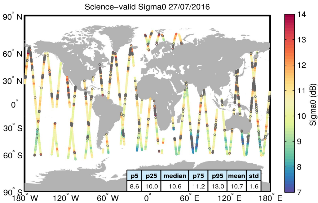
Figure 27. Geographical distribution of science-valid sigma0 data over oceans and lakes for 27/07/2016. The statistical values shown in the table refer to the sigma0 in dB and are calculated over all measurements shown in the figure. Gray circles denote records that have been rejected based on the editing criteria described in Table 4.
