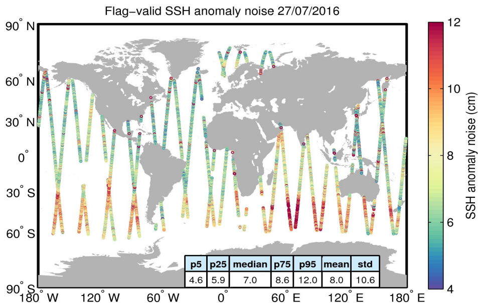
Figure 8. Geographical distribution of flag-valid 20-Hz SSH anomaly measurement noise over oceans and lakes for 27/07/2016. The statistical values shown in the table refer to the SSH anomaly noise and are calculated over all measurements shown in the figure.
