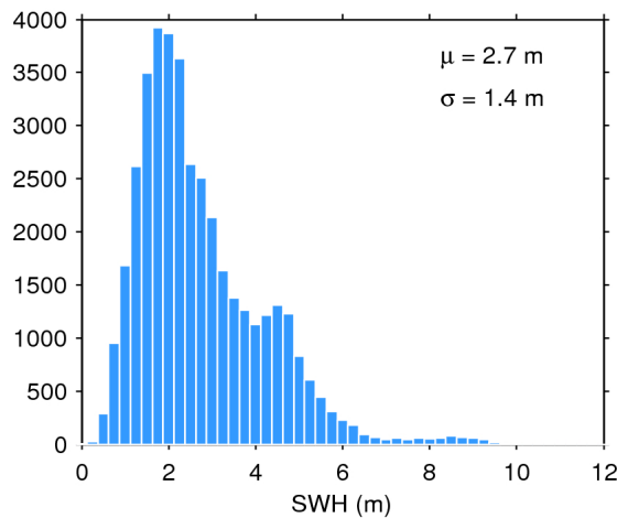
Figure 20. Histogram of science-valid SWH over oceans and lakes for 27/07/2016. The mean ( \mu ) and standard deviation ( \sigma ) are also shown. Note that values larger than 12 m are excluded from the histogram for the sake of readability but not from the computation of \mu and \sigma .
