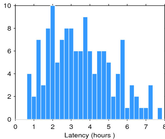
Figure 2. Histogram of the data latency for 27/07/2016. The y-axis denotes the number of files that are made available with a delay of x-hours with respect to the mean time of the records stored in the file.
