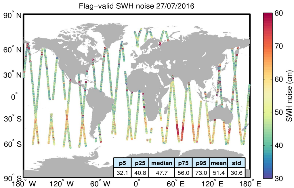
Figure 18. Geographical distribution of flag-valid 20-Hz SWH measurement noise over oceans and lakes for 27/07/2016. The statistical values shown in the table refer to the SWH noise and are calculated over all measurements shown in the figure.
