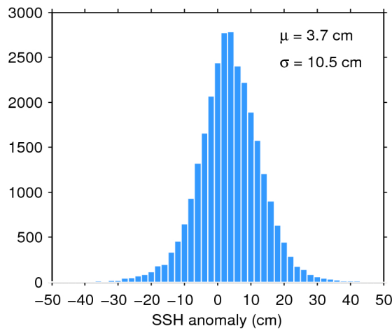
Figure 11. Histogram of science-valid SSH anomaly over oceans and lakes for 27/07/2016. The mean ( \mu ) and standard deviation ( \sigma ) are also shown. Note that values outside [-50 50] cm are excluded from the histogram for the sake of readability but not from the computation of \mu and \sigma .
