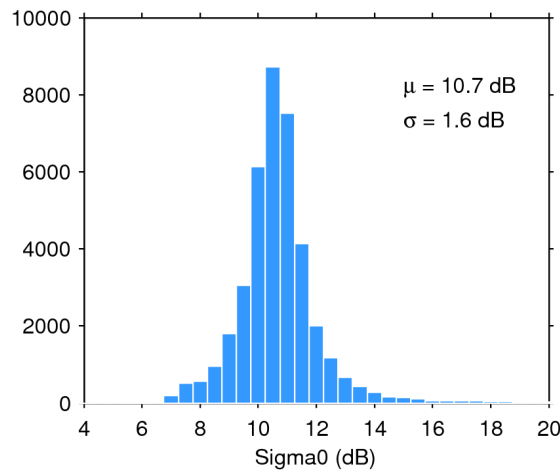
Figure 28. Histogram of science-valid sigma0 over oceans and lakes for 27/07/2016. The mean ( \mu ) and standard deviation ( \sigma ) are also shown. Note that values outside [4 20] dB are excluded from the histogram for the sake of readability but not from the computation of \mu and \sigma .
