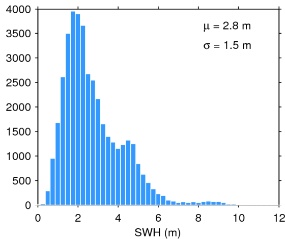
Figure 17. Histogram of flag-valid SWH over oceans and lakes for 27/07/2016. The mean ( \mu ) and standard deviation ( \sigma ) are also shown. Note that values larger than 12 m are excluded from the histogram for the sake of readability but not from the computation of \mu and \sigma .
