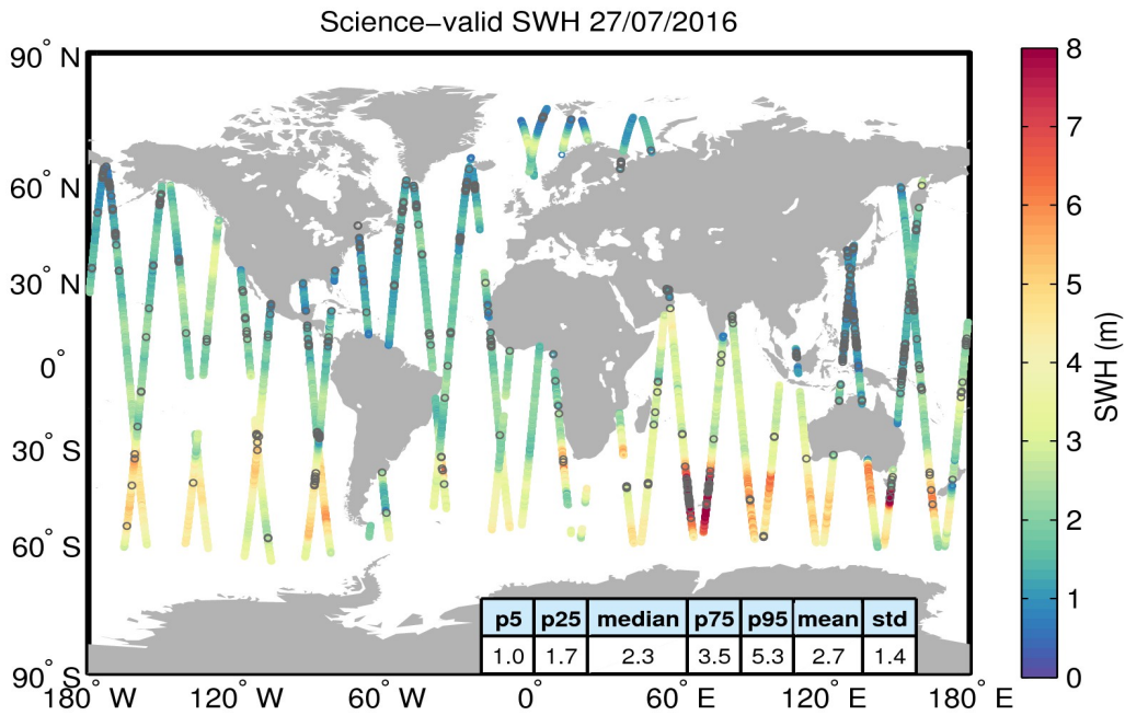
Figure 19. Geographical distribution of science-valid SWH data over oceans and lakes for 27/07/2016. The statistical values shown in the table refer to the SWH in m and are calculated over all measurements shown in the figure. Gray circles denote records that have been rejected based on the editing criteria described in Table 3.
