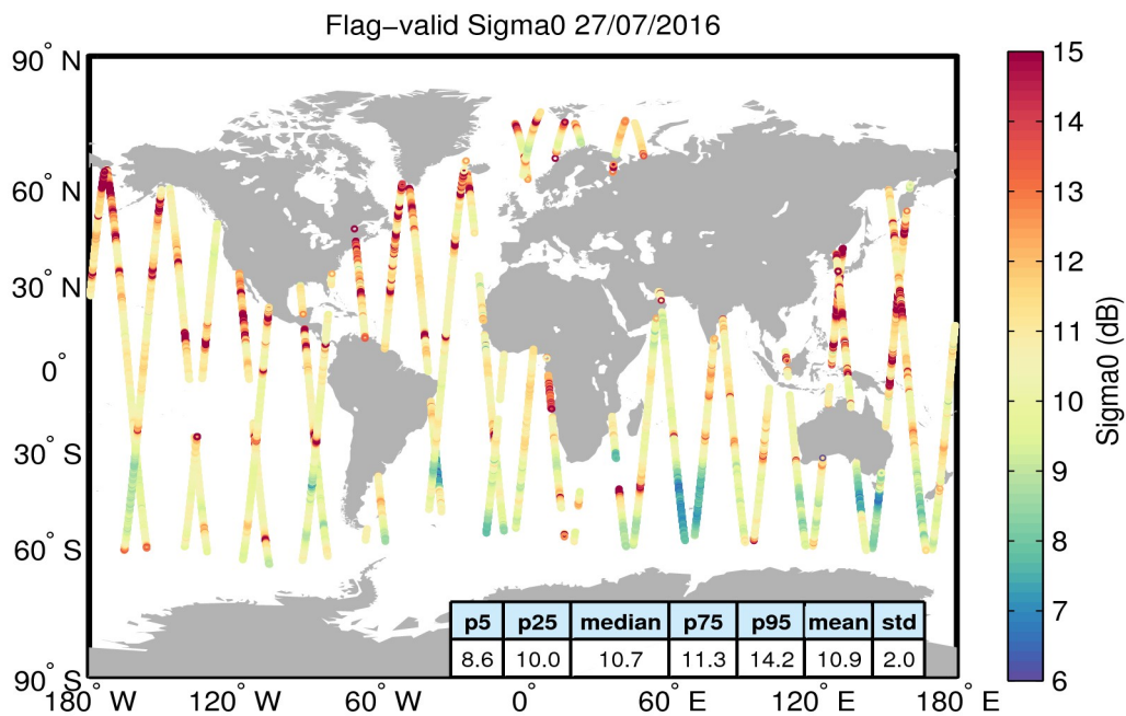
Figure 23. Geographical distribution of flag-valid sigma0 data over oceans and lakes for 27/07/2016. The statistical values shown in the table refer to the sigma0 in dB and are calculated over all measurements shown in the figure.
