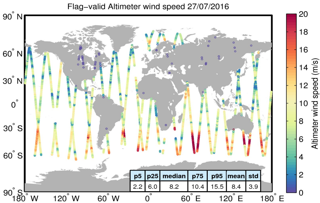
Figure 31. Geographical distribution of flag-valid wind data over oceans and lakes for 27/07/2016. The statistical values shown in the table refer to the wind in m/s and are calculated over all measurements shown in the figure.
