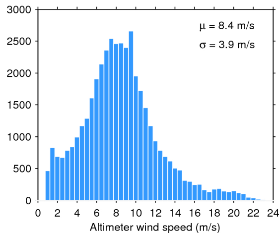
Figure 35. Histogram of science-valid wind over oceans and lakes for 27/07/2016. The mean ( \mu ) and standard deviation ( \sigma ) are also shown. Note that values larger than 24 m/s are excluded from the histogram for the sake of readability but not from the computation of \mu and \sigma .
