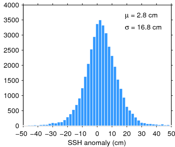
Figure 7. Histogram of flag-valid SSH anomaly over oceans and lakes for 26/07/2016. The mean ( \mu ) and standard deviation ( \sigma ) are also shown. Note that values outside [-50 50] cm are excluded from the histogram for the sake of readability but not from the computation of \mu and \sigma .
