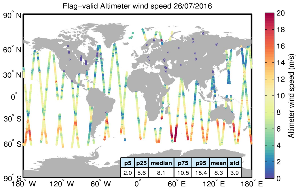
Figure 31. Geographical distribution of flag-valid wind data over oceans and lakes for 26/07/2016. The statistical values shown in the table refer to the wind in m/s and are calculated over all measurements shown in the figure.
