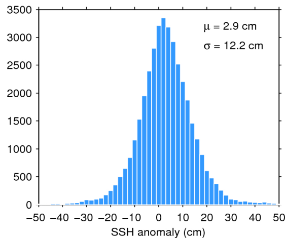
Figure 11. Histogram of science-valid SSH anomaly over oceans and lakes for 26/07/2016. The mean ( \mu ) and standard deviation ( \sigma ) are also shown. Note that values outside [-50 50] cm are excluded from the histogram for the sake of readability but not from the computation of \mu and \sigma .
