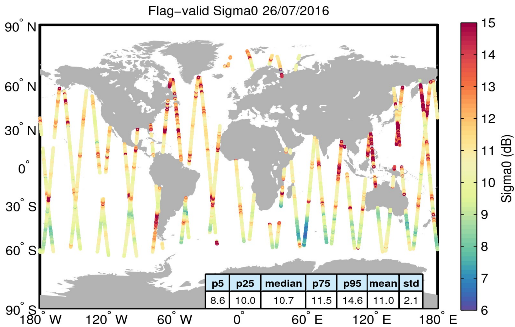
Figure 23. Geographical distribution of flag-valid sigma0 data over oceans and lakes for 26/07/2016. The statistical values shown in the table refer to the sigma0 in dB and are calculated over all measurements shown in the figure.
