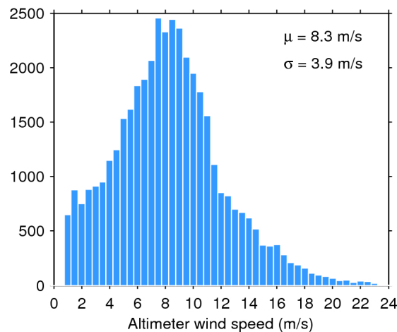
Figure 35. Histogram of science-valid wind over oceans and lakes for 26/07/2016. The mean ( \mu ) and standard deviation ( \sigma ) are also shown. Note that values larger than 24 m/s are excluded from the histogram for the sake of readability but not from the computation of \mu and \sigma .
