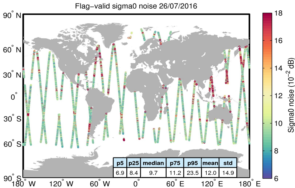
Figure 26. Geographical distribution of flag-valid 20-Hz sigma0 measurement noise over oceans and lakes for 26/07/2016. The statistical values shown in the table refer to the sigma0 noise and are calculated over all measurements shown in the figure.
