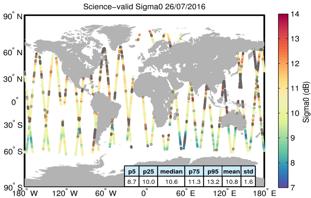
Figure 27. Geographical distribution of science-valid sigma0 data over oceans and lakes for 26/07/2016. The statistical values shown in the table refer to the sigma0 in dB and are calculated over all measurements shown in the figure. Gray circles denote records that have been rejected based on the editing criteria described in Table 4.
