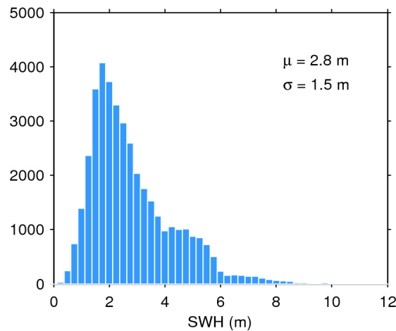
Figure 20. Histogram of science-valid SWH over oceans and lakes for 26/07/2016. The mean ( \mu ) and standard deviation ( \sigma ) are also shown. Note that values larger than 12 m are excluded from the histogram for the sake of readability but not from the computation of \mu and \sigma .
