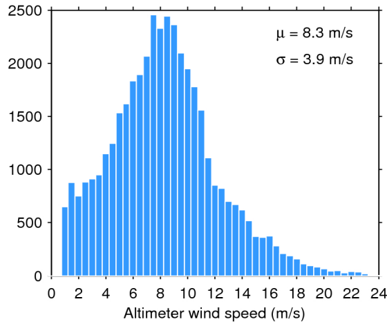
Figure 33. Histogram of flag-valid wind over oceans and lakes for 26/07/2016. The mean ( \mu ) and standard deviation ( \sigma ) are also shown. Note that values larger than 24 m/s are excluded from the histogram for the sake of readability but not from the computation of \mu and \sigma .
