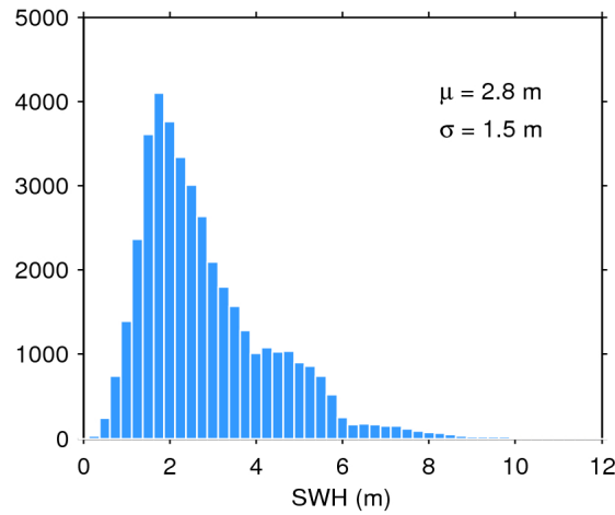
Figure 17. Histogram of flag-valid SWH over oceans and lakes for 26/07/2016. The mean ( \mu ) and standard deviation ( \sigma ) are also shown. Note that values larger than 12 m are excluded from the histogram for the sake of readability but not from the computation of \mu and \sigma .
