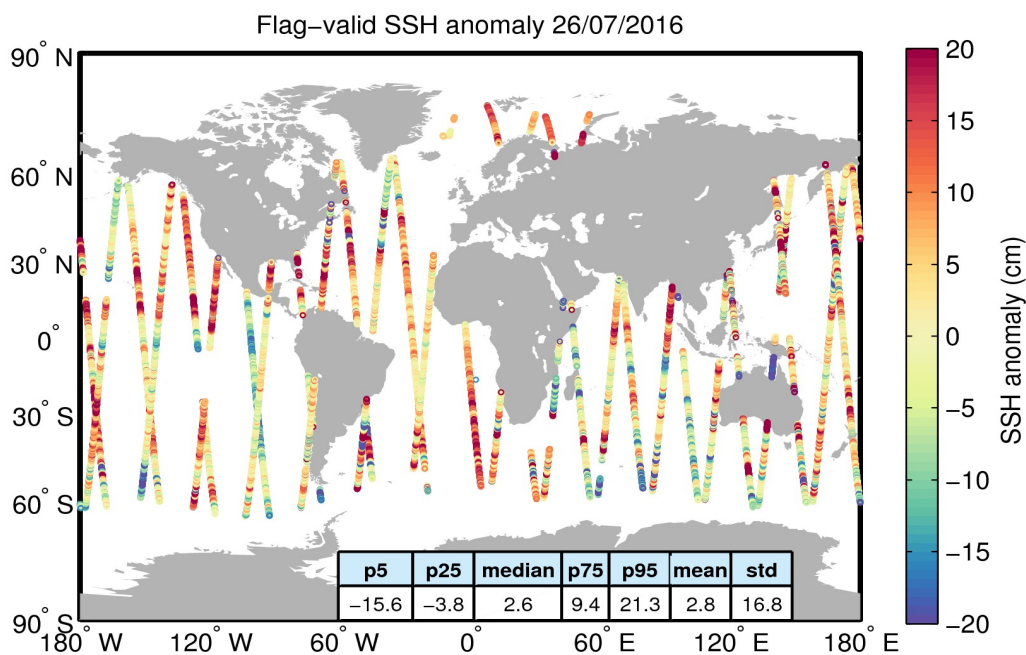
Figure 5. Geographical distribution of flag-valid 1-Hz SSH anomaly data over oceans and lakes for 26/07/2016. The statistical values shown in the table refer to the SSH anomaly in cm and are calculated over all measurements shown in the figure.
