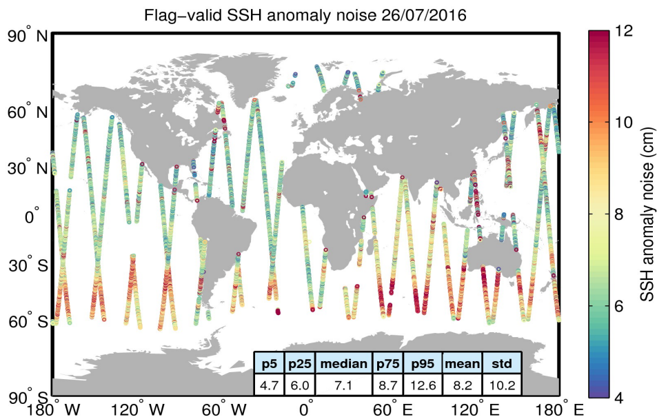
Figure 8. Geographical distribution of flag-valid 20-Hz SSH anomaly measurement noise over oceans and lakes for 26/07/2016. The statistical values shown in the table refer to the SSH anomaly noise and are calculated over all measurements shown in the figure.
