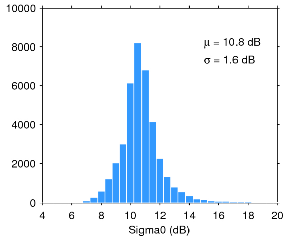
Figure 28. Histogram of science-valid sigma0 over oceans and lakes for 26/07/2016. The mean ( \mu ) and standard deviation ( \sigma ) are also shown. Note that values outside [4 20] dB are excluded from the histogram for the sake of readability but not from the computation of \mu and \sigma .
