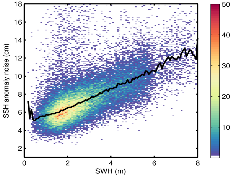
Figure 9. 2D histogram showing flag-valid SSH anomaly noise as a function of SWH for 26/07/2016. The black line denotes the median SSH anomaly noise as a function of SWH.
