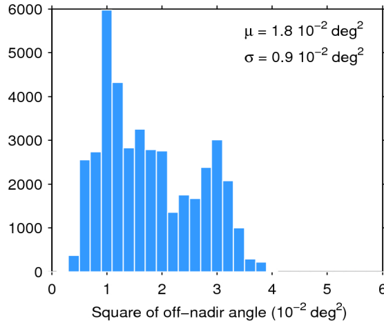
Figure 39. Histogram of flag-valid mispointing over oceans and lakes for 26/07/2016. The mean ( \mu ) and standard deviation ( \sigma ) are also shown. Note that values larger than 6 \cdot 10^{-2} \text{ deg}^2 are excluded from the histogram for the sake of readability but not from the computation of \mu and \sigma .
