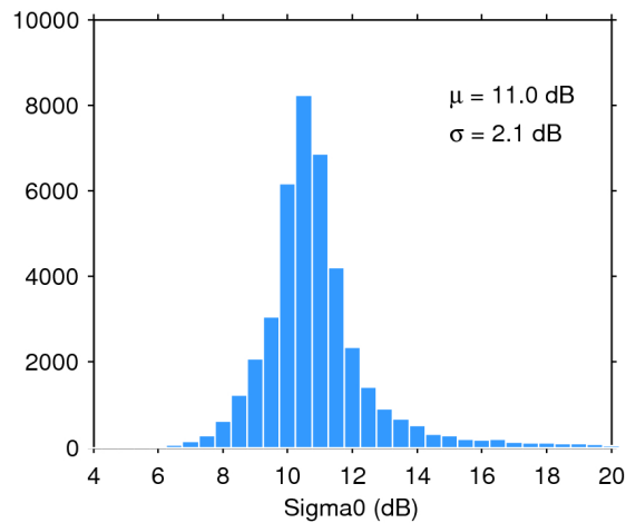
Figure 25. Histogram of flag-valid sigma0 over oceans and lakes for 26/07/2016. The mean ( \mu ) and standard deviation ( \sigma ) are also shown. Note that values outside [4 20] dB are excluded from the histogram for the sake of readability but not from the computation of \mu and \sigma .
