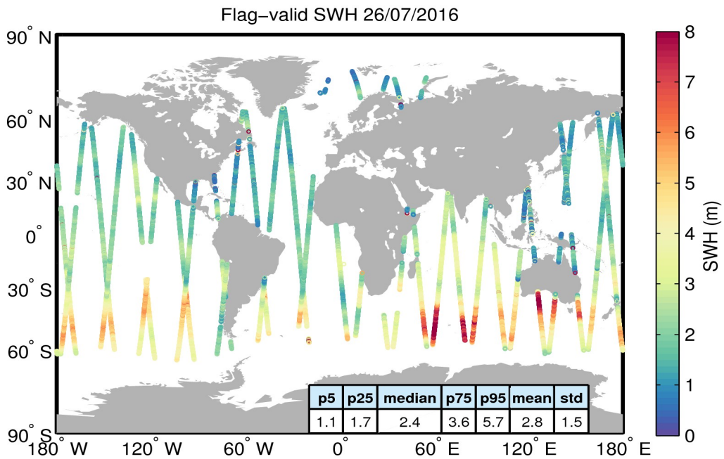
Figure 15. Geographical distribution of flag-valid SWH data over oceans and lakes for 26/07/2016. The statistical values shown in the table refer to the SWH in m and are calculated over all measurements shown in the figure.
