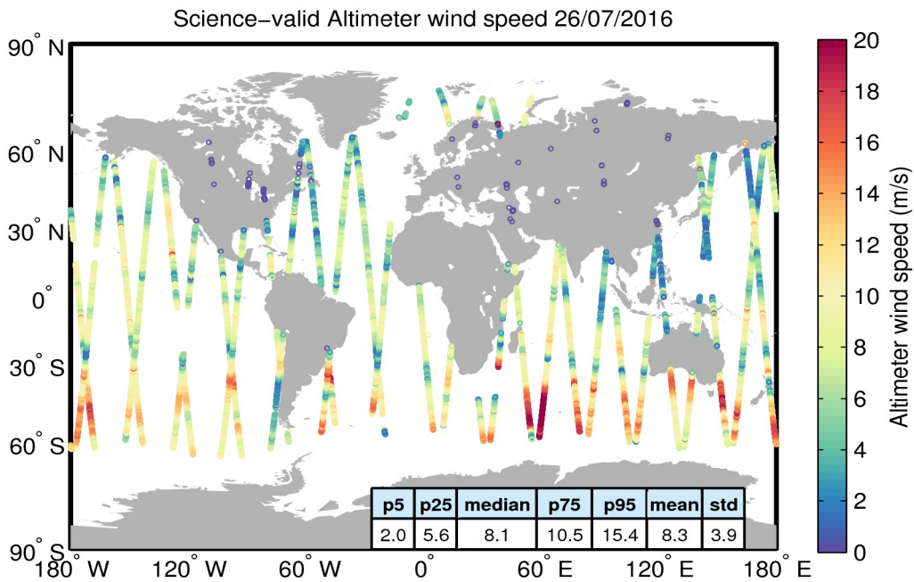
Figure 34. Geographical distribution of science-valid wind data over oceans and lakes for 26/07/2016. The statistical values shown in the table refer to the wind in m/s and are calculated over all measurements shown in the figure. Gray circles denote records that have been rejected based on the editing criteria described in Table 5.
