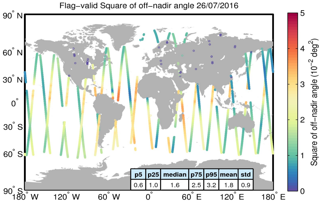
Figure 37. Geographical distribution of flag-valid mispointing data over oceans and lakes for 26/07/2016. The statistical values shown in the table refer to the mispointing in 10^{-2} deg 2 and are calculated over all measurements shown in the figure.
