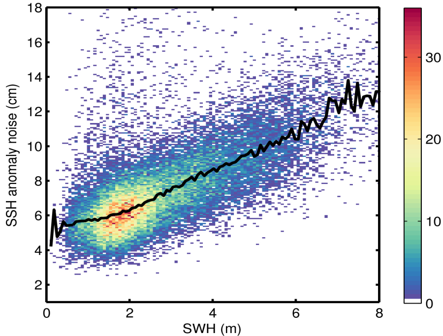
Figure 9. 2D histogram showing flag-valid SSH anomaly noise as a function of SWH for 25/07/2016. The black line denotes the median SSH anomaly noise as a function of SWH.
