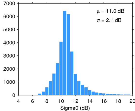
Figure 25. Histogram of flag-valid sigma0 over oceans and lakes for 25/07/2016. The mean ( \mu ) and standard deviation ( \sigma ) are also shown. Note that values outside [4 20] dB are excluded from the histogram for the sake of readability but not from the computation of \mu and \sigma .
