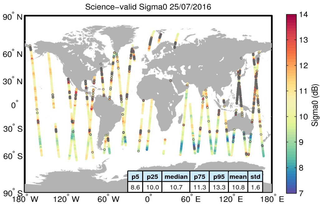
Figure 27. Geographical distribution of science-valid sigma0 data over oceans and lakes for 25/07/2016. The statistical values shown in the table refer to the sigma0 in dB and are calculated over all measurements shown in the figure. Gray circles denote records that have been rejected based on the editing criteria described in Table 4.
