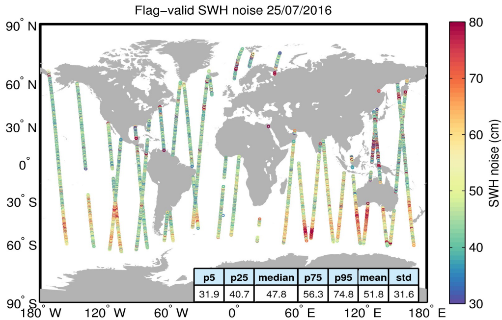
Figure 18. Geographical distribution of flag-valid 20-Hz SWH measurement noise over oceans and lakes for 25/07/2016. The statistical values shown in the table refer to the SWH noise and are calculated over all measurements shown in the figure.
