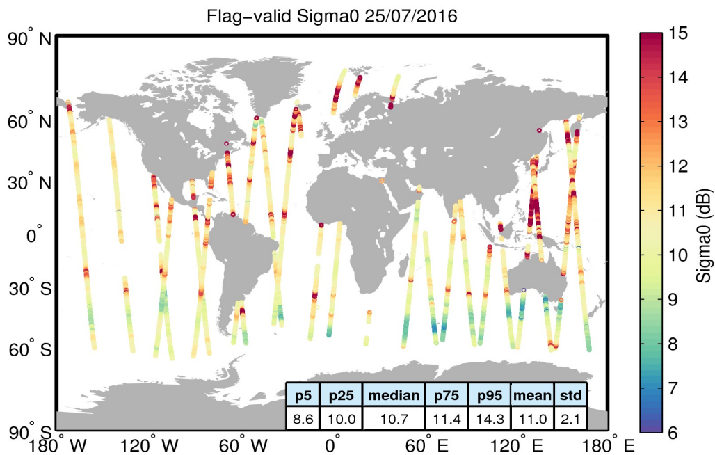
Figure 23. Geographical distribution of flag-valid sigma0 data over oceans and lakes for 25/07/2016. The statistical values shown in the table refer to the sigma0 in dB and are calculated over all measurements shown in the figure.
