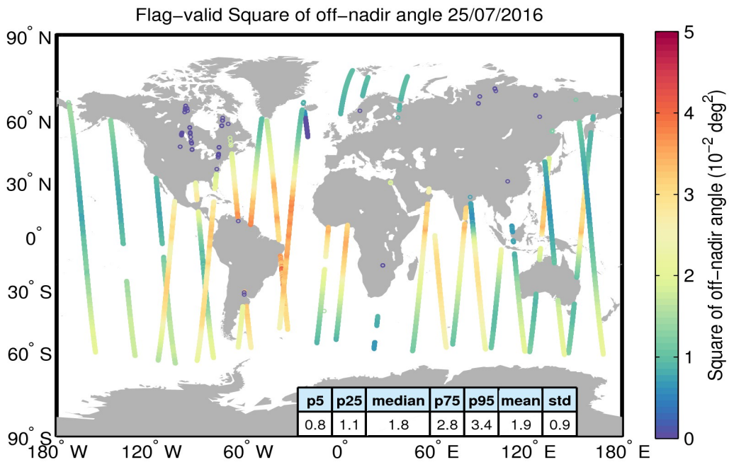
Figure 37. Geographical distribution of flag-valid mispointing data over oceans and lakes for 25/07/2016. The statistical values shown in the table refer to the mispointing in 10^{-2} deg 2 and are calculated over all measurements shown in the figure.
