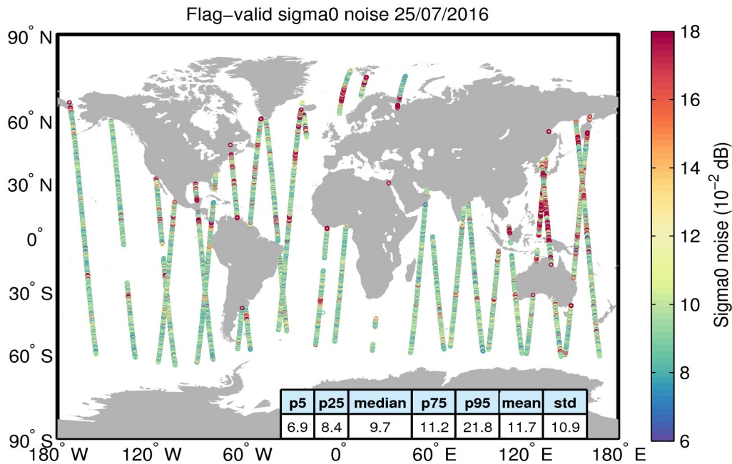
Figure 26. Geographical distribution of flag-valid 20-Hz sigma0 measurement noise over oceans and lakes for 25/07/2016. The statistical values shown in the table refer to the sigma0 noise and are calculated over all measurements shown in the figure.
