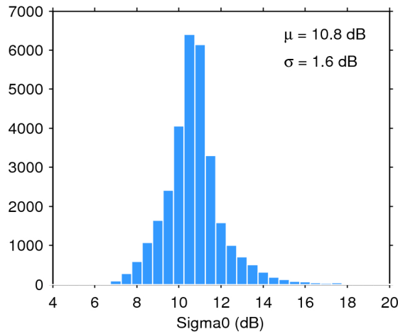
Figure 28. Histogram of science-valid sigma0 over oceans and lakes for 25/07/2016. The mean ( \mu ) and standard deviation ( \sigma ) are also shown. Note that values outside [4 20] dB are excluded from the histogram for the sake of readability but not from the computation of \mu and \sigma .
