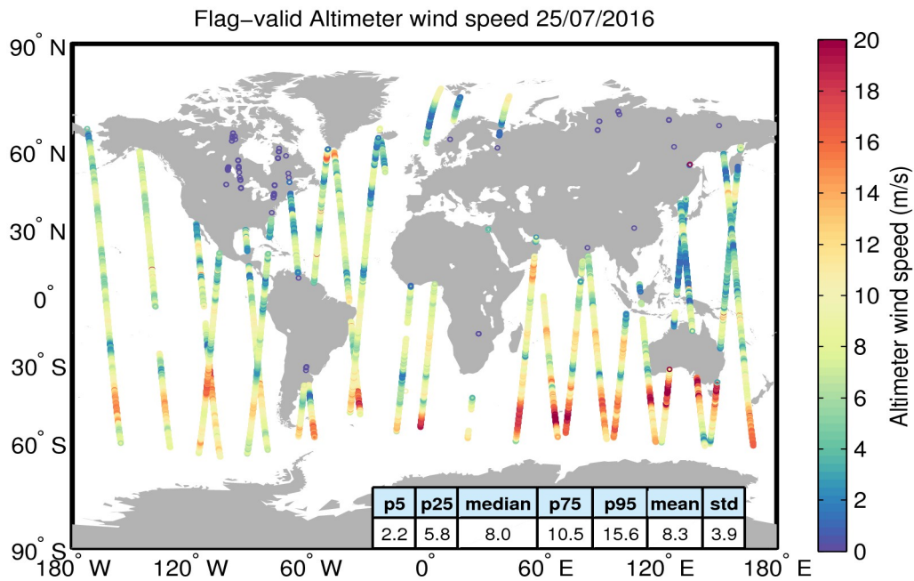
Figure 31. Geographical distribution of flag-valid wind data over oceans and lakes for 25/07/2016. The statistical values shown in the table refer to the wind in m/s and are calculated over all measurements shown in the figure.
