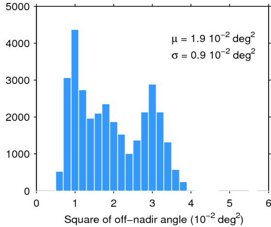
Figure 39. Histogram of flag-valid mispointing over oceans and lakes for 25/07/2016. The mean ( \mu ) and standard deviation ( \sigma ) are also shown. Note that values larger than 6 \cdot 10^{-2} \text{ deg}^2 are excluded from the histogram for the sake of readability but not from the computation of \mu and \sigma .
