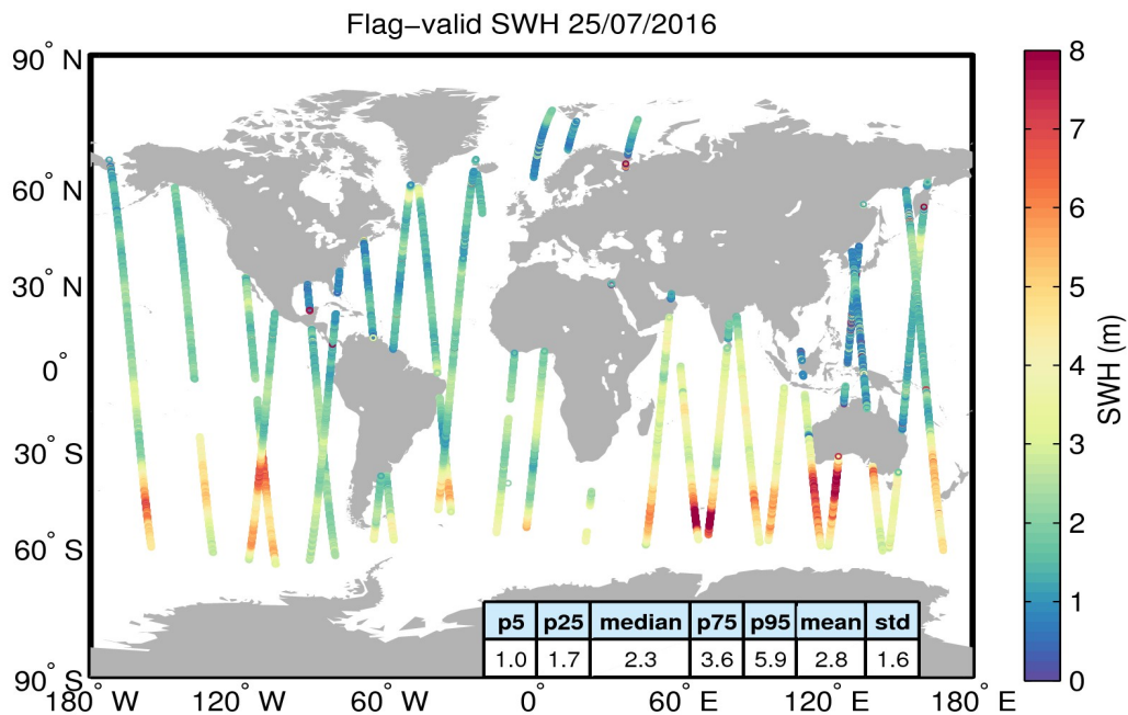
Figure 15. Geographical distribution of flag-valid SWH data over oceans and lakes for 25/07/2016. The statistical values shown in the table refer to the SWH in m and are calculated over all measurements shown in the figure.
