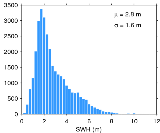
Figure 17. Histogram of flag-valid SWH over oceans and lakes for 25/07/2016. The mean ( \mu ) and standard deviation ( \sigma ) are also shown. Note that values larger than 12 m are excluded from the histogram for the sake of readability but not from the computation of \mu and \sigma .
