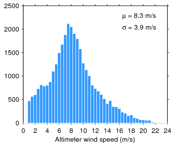
Figure 35. Histogram of science-valid wind over oceans and lakes for 25/07/2016. The mean ( \mu ) and standard deviation ( \sigma ) are also shown. Note that values larger than 24 m/s are excluded from the histogram for the sake of readability but not from the computation of \mu and \sigma .
