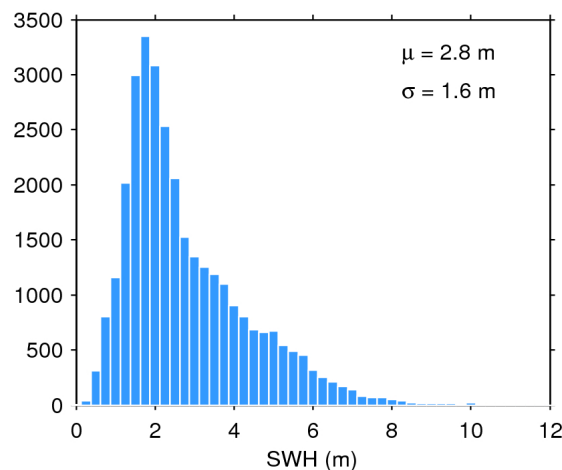
Figure 20. Histogram of science-valid SWH over oceans and lakes for 25/07/2016. The mean ( \mu ) and standard deviation ( \sigma ) are also shown. Note that values larger than 12 m are excluded from the histogram for the sake of readability but not from the computation of \mu and \sigma .
