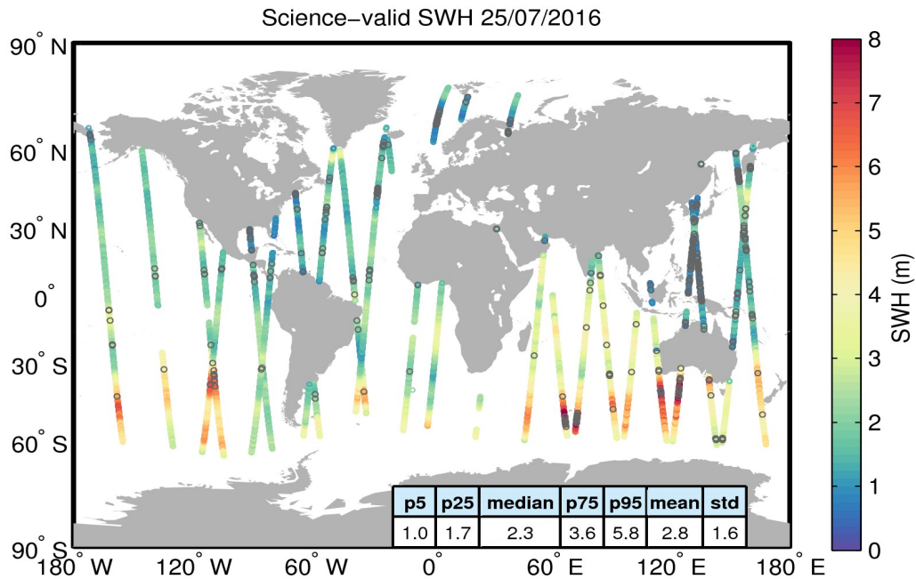
Figure 19. Geographical distribution of science-valid SWH data over oceans and lakes for 25/07/2016. The statistical values shown in the table refer to the SWH in m and are calculated over all measurements shown in the figure. Gray circles denote records that have been rejected based on the editing criteria described in Table 3.
