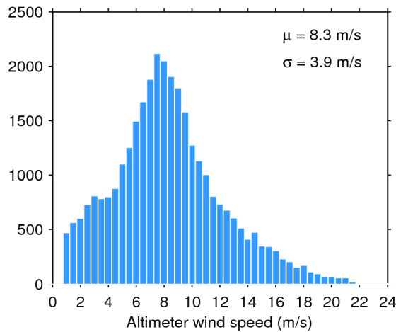
Figure 33. Histogram of flag-valid wind over oceans and lakes for 25/07/2016. The mean ( \mu ) and standard deviation ( \sigma ) are also shown. Note that values larger than 24 m/s are excluded from the histogram for the sake of readability but not from the computation of \mu and \sigma .
