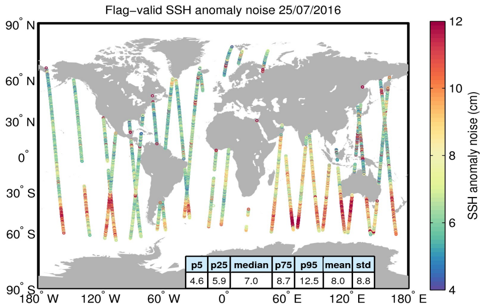
Figure 8. Geographical distribution of flag-valid 20-Hz SSH anomaly measurement noise over oceans and lakes for 25/07/2016. The statistical values shown in the table refer to the SSH anomaly noise and are calculated over all measurements shown in the figure.
