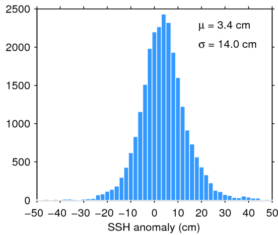
Figure 11. Histogram of science-valid SSH anomaly over oceans and lakes for 25/07/2016. The mean ( \mu ) and standard deviation ( \sigma ) are also shown. Note that values outside [-50 50] cm are excluded from the histogram for the sake of readability but not from the computation of \mu and \sigma .
