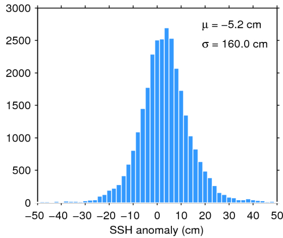
Figure 7. Histogram of flag-valid SSH anomaly over oceans and lakes for 25/07/2016. The mean ( \mu ) and standard deviation ( \sigma ) are also shown. Note that values outside [-50 50] cm are excluded from the histogram for the sake of readability but not from the computation of \mu and \sigma .
