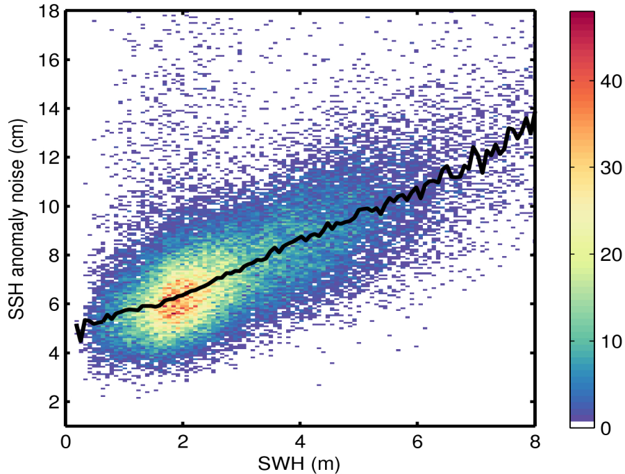
Figure 9. 2D histogram showing flag-valid SSH anomaly noise as a function of SWH for 24/07/2016. The black line denotes the median SSH anomaly noise as a function of SWH.
