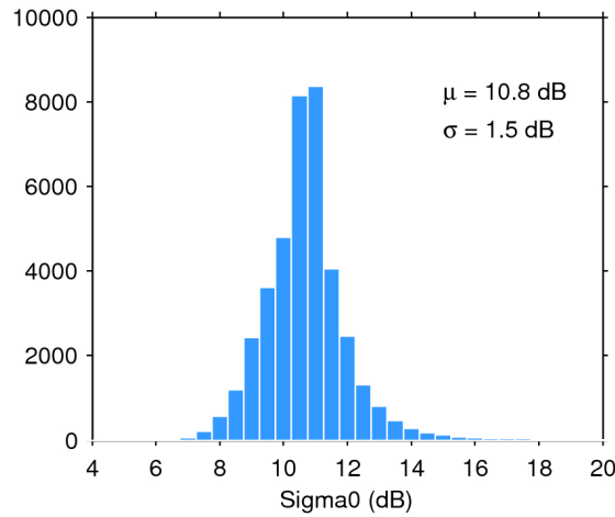
Figure 28. Histogram of science-valid sigma0 over oceans and lakes for 24/07/2016. The mean ( \mu ) and standard deviation ( \sigma ) are also shown. Note that values outside [4 20] dB are excluded from the histogram for the sake of readability but not from the computation of \mu and \sigma .
