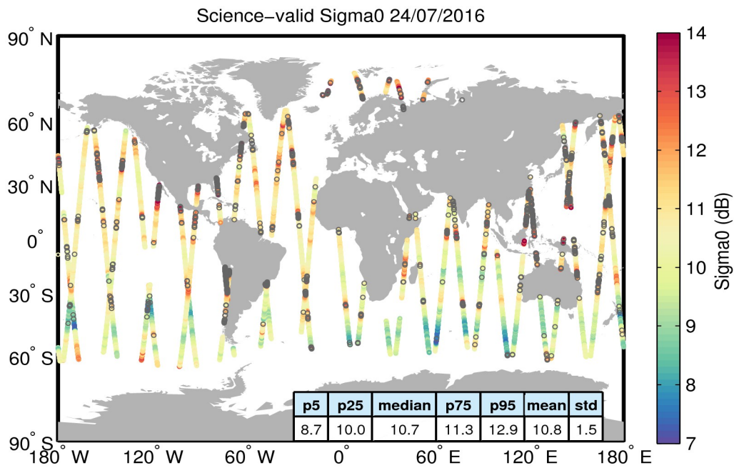
Figure 27. Geographical distribution of science-valid sigma0 data over oceans and lakes for 24/07/2016. The statistical values shown in the table refer to the sigma0 in dB and are calculated over all measurements shown in the figure. Gray circles denote records that have been rejected based on the editing criteria described in Table 4.
