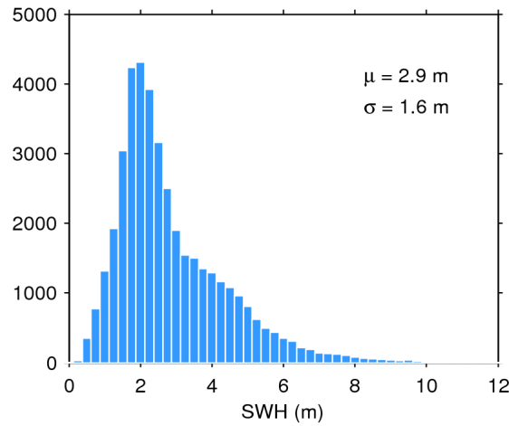
Figure 17. Histogram of flag-valid SWH over oceans and lakes for 24/07/2016. The mean ( \mu ) and standard deviation ( \sigma ) are also shown. Note that values larger than 12 m are excluded from the histogram for the sake of readability but not from the computation of \mu and \sigma .
