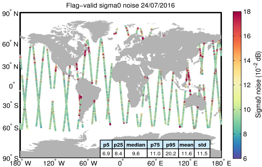
Figure 26. Geographical distribution of flag-valid 20-Hz sigma0 measurement noise over oceans and lakes for 24/07/2016. The statistical values shown in the table refer to the sigma0 noise and are calculated over all measurements shown in the figure.
