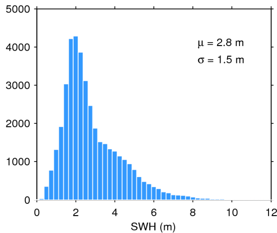
Figure 20. Histogram of science-valid SWH over oceans and lakes for 24/07/2016. The mean ( \mu ) and standard deviation ( \sigma ) are also shown. Note that values larger than 12 m are excluded from the histogram for the sake of readability but not from the computation of \mu and \sigma .
