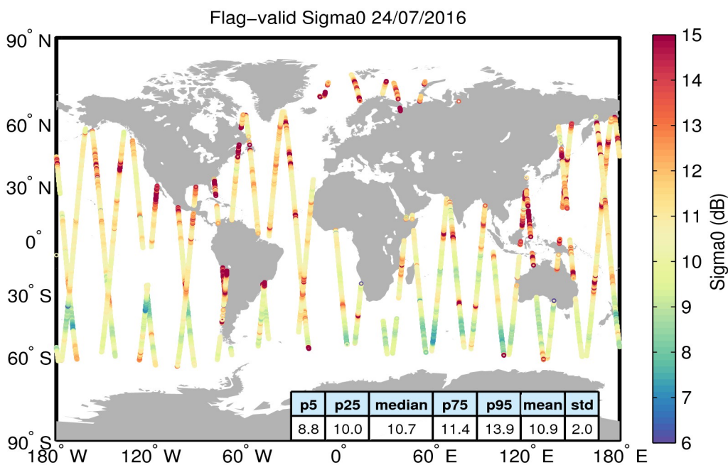
Figure 23. Geographical distribution of flag-valid sigma0 data over oceans and lakes for 24/07/2016. The statistical values shown in the table refer to the sigma0 in dB and are calculated over all measurements shown in the figure.
