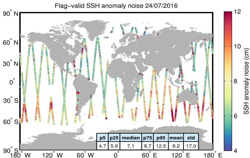
Figure 8. Geographical distribution of flag-valid 20-Hz SSH anomaly measurement noise over oceans and lakes for 24/07/2016. The statistical values shown in the table refer to the SSH anomaly noise and are calculated over all measurements shown in the figure.
