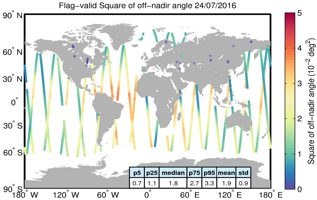
Figure 37. Geographical distribution of flag-valid mispointing data over oceans and lakes for 24/07/2016. The statistical values shown in the table refer to the mispointing in 10^{-2} deg 2 and are calculated over all measurements shown in the figure.
