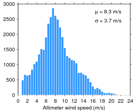
Figure 33. Histogram of flag-valid wind over oceans and lakes for 24/07/2016. The mean ( \mu ) and standard deviation ( \sigma ) are also shown. Note that values larger than 24 m/s are excluded from the histogram for the sake of readability but not from the computation of \mu and \sigma .
