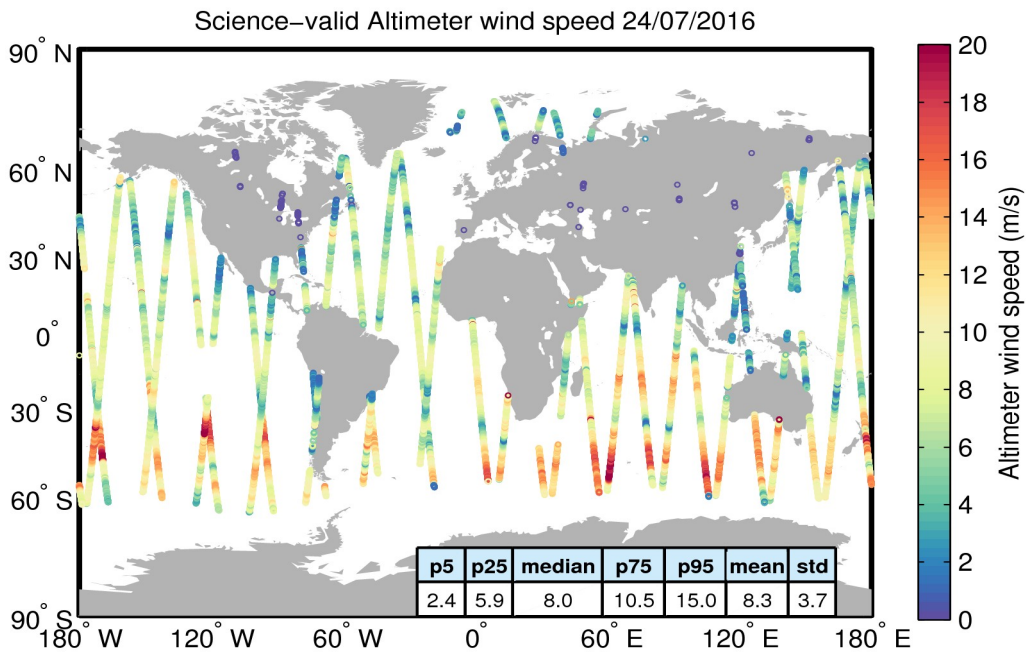
Figure 34. Geographical distribution of science-valid wind data over oceans and lakes for 24/07/2016. The statistical values shown in the table refer to the wind in m/s and are calculated over all measurements shown in the figure. Gray circles denote records that have been rejected based on the editing criteria described in Table 5.
