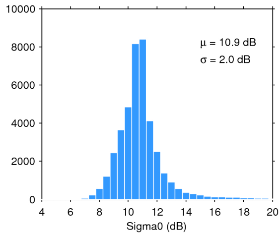
Figure 25. Histogram of flag-valid sigma0 over oceans and lakes for 24/07/2016. The mean ( \mu ) and standard deviation ( \sigma ) are also shown. Note that values outside [4 20] dB are excluded from the histogram for the sake of readability but not from the computation of \mu and \sigma .
