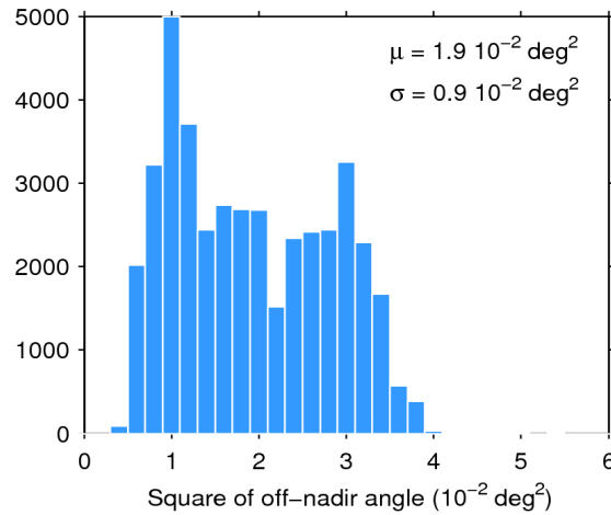
Figure 39. Histogram of flag-valid mispointing over oceans and lakes for 24/07/2016. The mean ( \mu ) and standard deviation ( \sigma ) are also shown. Note that values larger than 6 \cdot 10^{-2} \text{ deg}^2 are excluded from the histogram for the sake of readability but not from the computation of \mu and \sigma .
