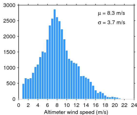
Figure 35. Histogram of science-valid wind over oceans and lakes for 24/07/2016. The mean ( \mu ) and standard deviation ( \sigma ) are also shown. Note that values larger than 24 m/s are excluded from the histogram for the sake of readability but not from the computation of \mu and \sigma .
