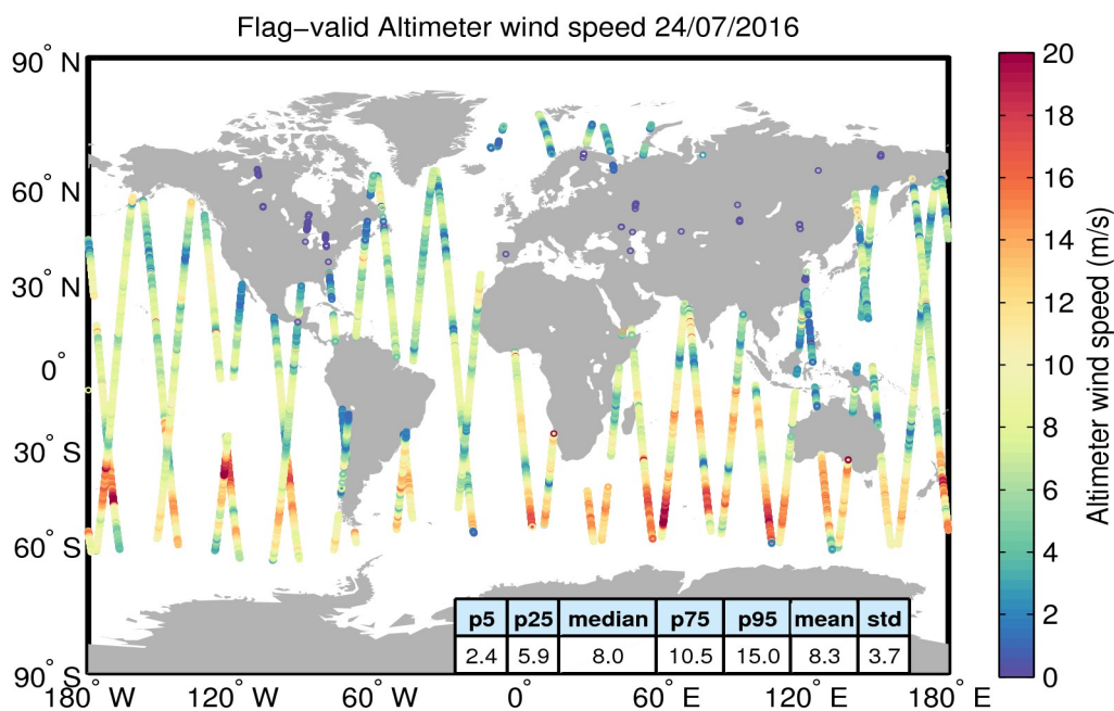
Figure 31. Geographical distribution of flag-valid wind data over oceans and lakes for 24/07/2016. The statistical values shown in the table refer to the wind in m/s and are calculated over all measurements shown in the figure.
