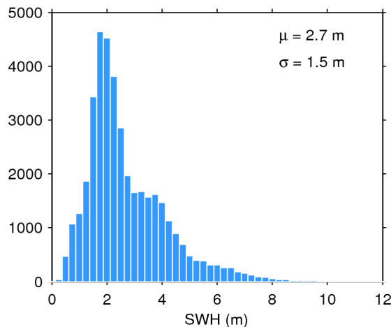
Figure 20. Histogram of science-valid SWH over oceans and lakes for 23/07/2016. The mean ( \mu ) and standard deviation ( \sigma ) are also shown. Note that values larger than 12 m are excluded from the histogram for the sake of readability but not from the computation of \mu and \sigma .
