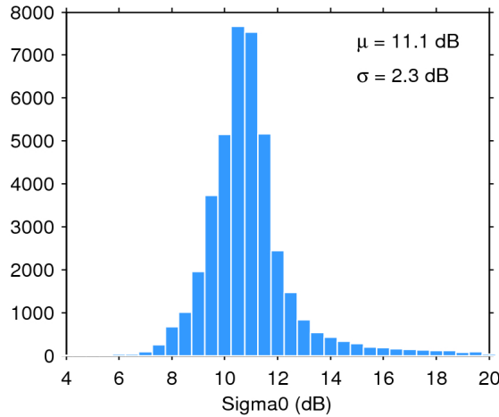
Figure 25. Histogram of flag-valid sigma0 over oceans and lakes for 23/07/2016. The mean ( \mu ) and standard deviation ( \sigma ) are also shown. Note that values outside [4 20] dB are excluded from the histogram for the sake of readability but not from the computation of \mu and \sigma .
