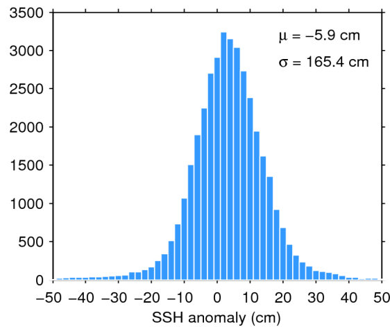
Figure 7. Histogram of flag-valid SSH anomaly over oceans and lakes for 23/07/2016. The mean ( \mu ) and standard deviation ( \sigma ) are also shown. Note that values outside [-50 50] cm are excluded from the histogram for the sake of readability but not from the computation of \mu and \sigma .
