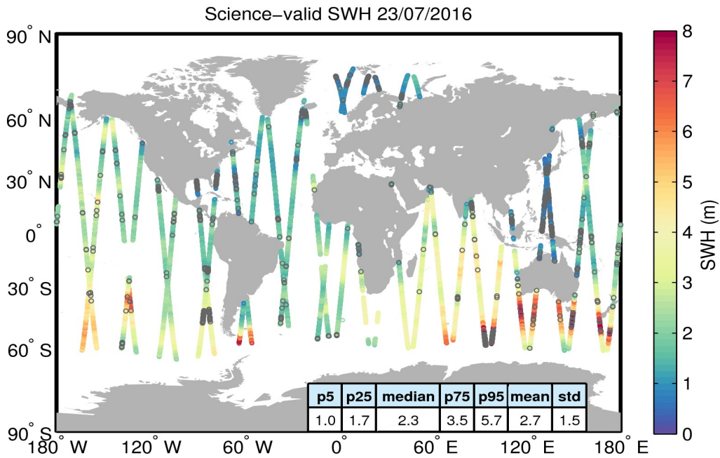
Figure 19. Geographical distribution of science-valid SWH data over oceans and lakes for 23/07/2016. The statistical values shown in the table refer to the SWH in m and are calculated over all measurements shown in the figure. Gray circles denote records that have been rejected based on the editing criteria described in Table 3.
