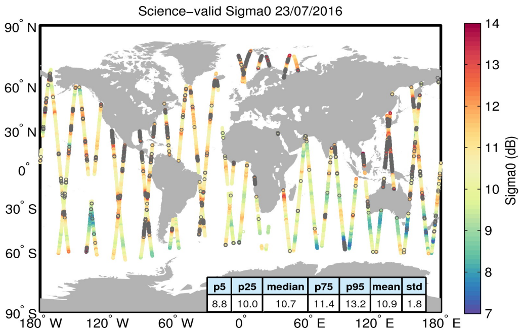
Figure 27. Geographical distribution of science-valid sigma0 data over oceans and lakes for 23/07/2016. The statistical values shown in the table refer to the sigma0 in dB and are calculated over all measurements shown in the figure. Gray circles denote records that have been rejected based on the editing criteria described in Table 4.
