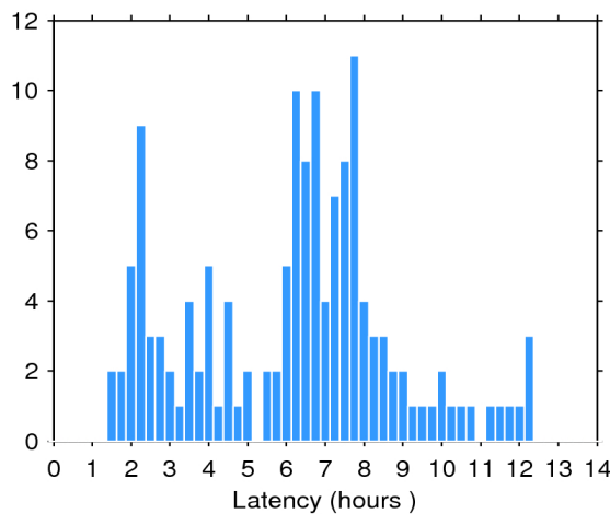
Figure 2. Histogram of the data latency for 23/07/2016. The y-axis denotes the number of files that are made available with a delay of x-hours with respect to the mean time of the records stored in the file.
