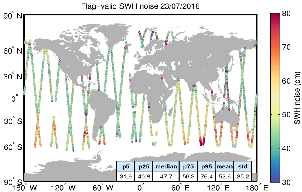
Figure 18. Geographical distribution of flag-valid 20-Hz SWH measurement noise over oceans and lakes for 23/07/2016. The statistical values shown in the table refer to the SWH noise and are calculated over all measurements shown in the figure.
