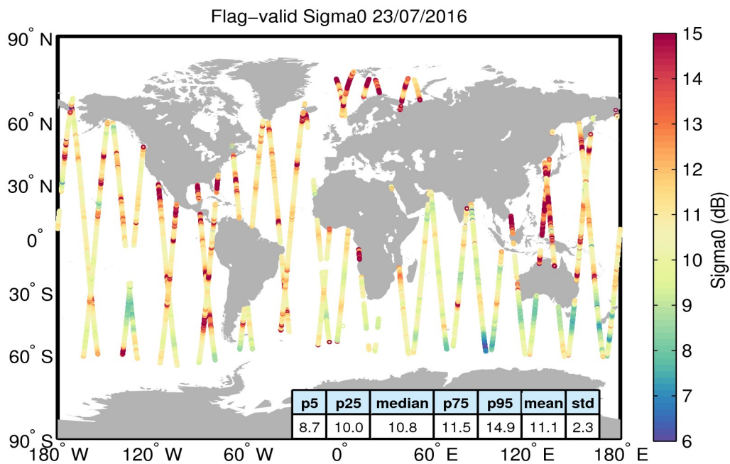
Figure 23. Geographical distribution of flag-valid sigma0 data over oceans and lakes for 23/07/2016. The statistical values shown in the table refer to the sigma0 in dB and are calculated over all measurements shown in the figure.
