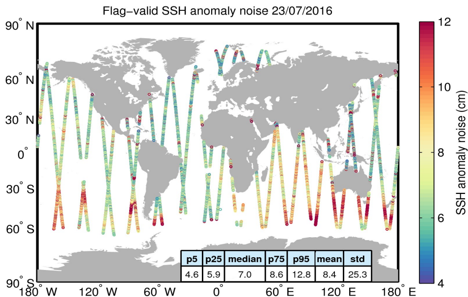
Figure 8. Geographical distribution of flag-valid 20-Hz SSH anomaly measurement noise over oceans and lakes for 23/07/2016. The statistical values shown in the table refer to the SSH anomaly noise and are calculated over all measurements shown in the figure.
