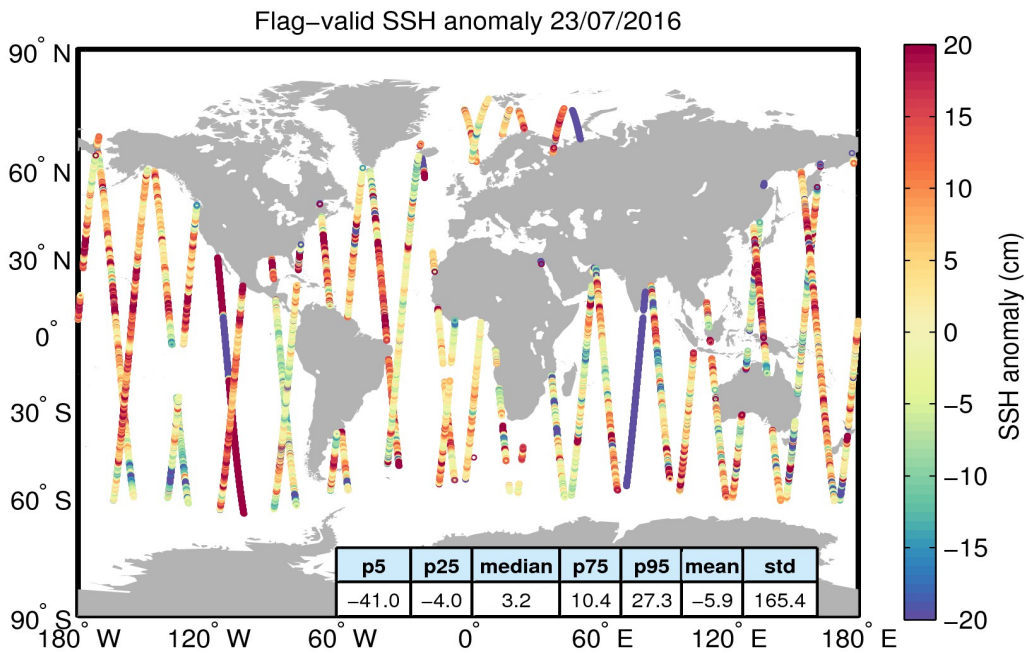
Figure 5. Geographical distribution of flag-valid 1-Hz SSH anomaly data over oceans and lakes for 23/07/2016. The statistical values shown in the table refer to the SSH anomaly in cm and are calculated over all measurements shown in the figure.
