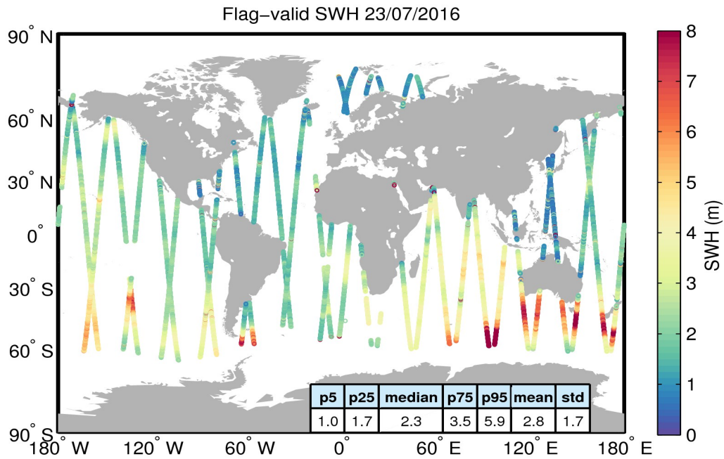
Figure 15. Geographical distribution of flag-valid SWH data over oceans and lakes for 23/07/2016. The statistical values shown in the table refer to the SWH in m and are calculated over all measurements shown in the figure.
