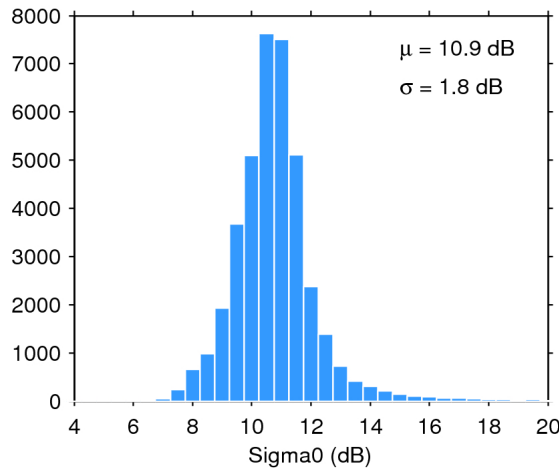
Figure 28. Histogram of science-valid sigma0 over oceans and lakes for 23/07/2016. The mean ( \mu ) and standard deviation ( \sigma ) are also shown. Note that values outside [4 20] dB are excluded from the histogram for the sake of readability but not from the computation of \mu and \sigma .
