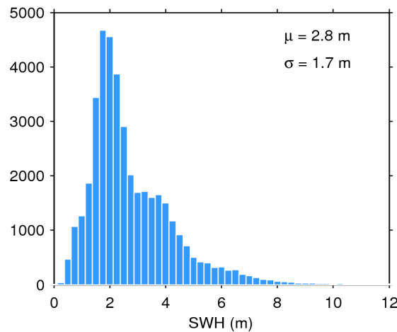
Figure 17. Histogram of flag-valid SWH over oceans and lakes for 23/07/2016. The mean ( \mu ) and standard deviation ( \sigma ) are also shown. Note that values larger than 12 m are excluded from the histogram for the sake of readability but not from the computation of \mu and \sigma .
