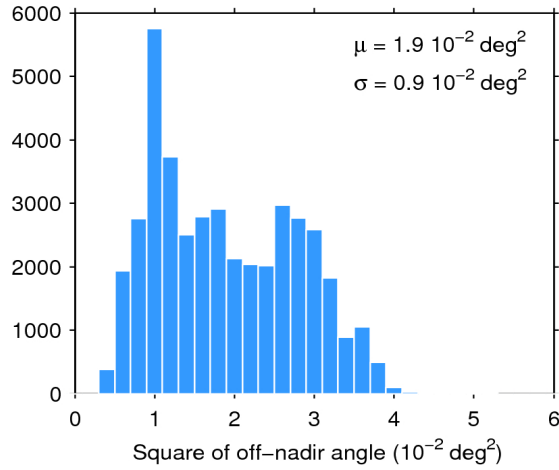
Figure 39. Histogram of flag-valid mispointing over oceans and lakes for 23/07/2016. The mean ( \mu ) and standard deviation ( \sigma ) are also shown. Note that values larger than 6 \cdot 10^{-2} \text{ deg}^2 are excluded from the histogram for the sake of readability but not from the computation of \mu and \sigma .
