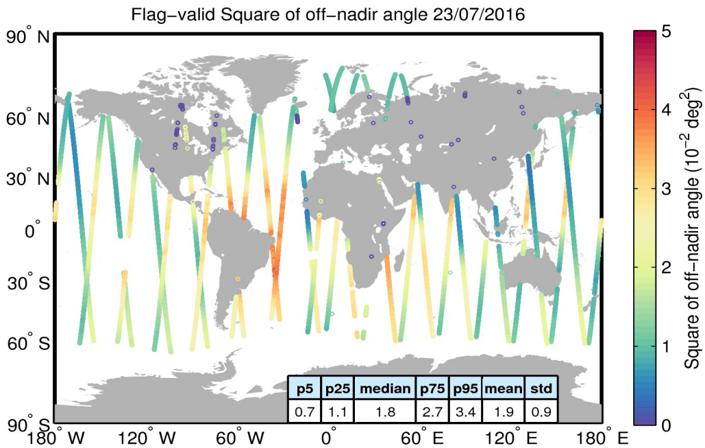
Figure 37. Geographical distribution of flag-valid mispointing data over oceans and lakes for 23/07/2016. The statistical values shown in the table refer to the mispointing in 10^{-2} deg 2 and are calculated over all measurements shown in the figure.
