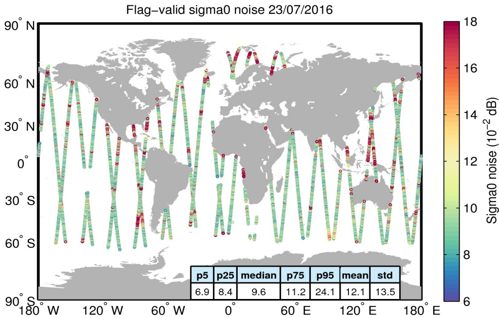
Figure 26. Geographical distribution of flag-valid 20-Hz sigma0 measurement noise over oceans and lakes for 23/07/2016. The statistical values shown in the table refer to the sigma0 noise and are calculated over all measurements shown in the figure.
