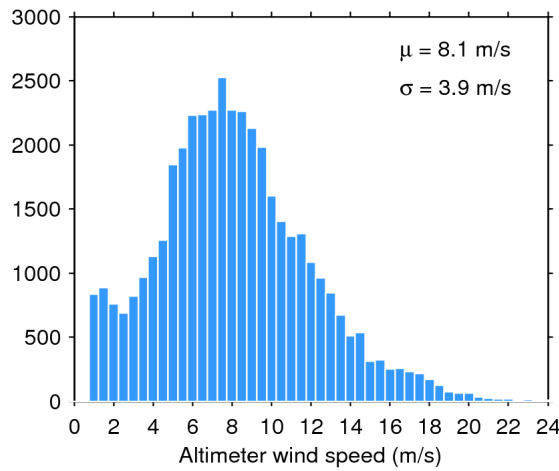
Figure 33. Histogram of flag-valid wind over oceans and lakes for 23/07/2016. The mean ( \mu ) and standard deviation ( \sigma ) are also shown. Note that values larger than 24 m/s are excluded from the histogram for the sake of readability but not from the computation of \mu and \sigma .
