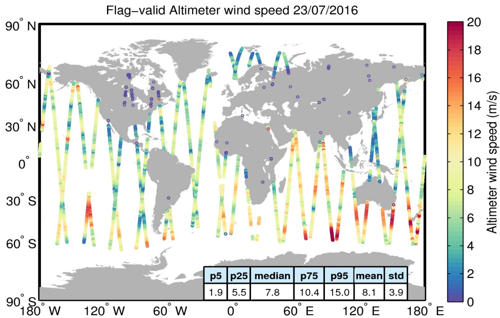
Figure 31. Geographical distribution of flag-valid wind data over oceans and lakes for 23/07/2016. The statistical values shown in the table refer to the wind in m/s and are calculated over all measurements shown in the figure.
