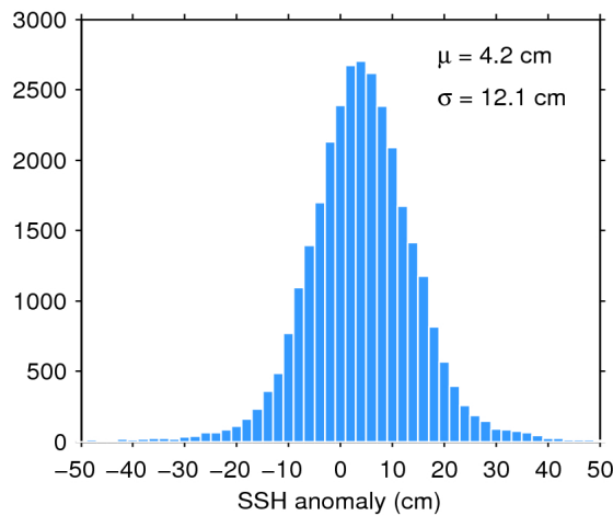
Figure 11. Histogram of science-valid SSH anomaly over oceans and lakes for 23/07/2016. The mean ( \mu ) and standard deviation ( \sigma ) are also shown. Note that values outside [-50 50] cm are excluded from the histogram for the sake of readability but not from the computation of \mu and \sigma .
