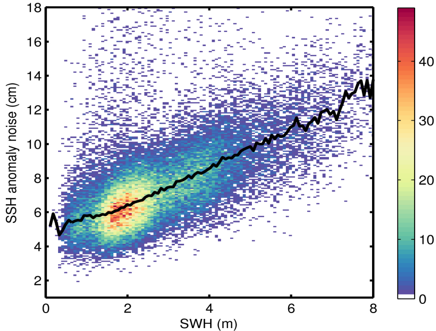
Figure 9. 2D histogram showing flag-valid SSH anomaly noise as a function of SWH for 23/07/2016. The black line denotes the median SSH anomaly noise as a function of SWH.
