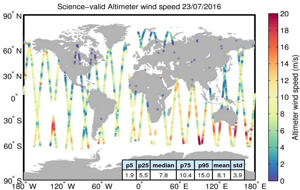
Figure 34. Geographical distribution of science-valid wind data over oceans and lakes for 23/07/2016. The statistical values shown in the table refer to the wind in m/s and are calculated over all measurements shown in the figure. Gray circles denote records that have been rejected based on the editing criteria described in Table 5.
