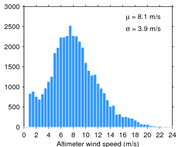
Figure 35. Histogram of science-valid wind over oceans and lakes for 23/07/2016. The mean ( \mu ) and standard deviation ( \sigma ) are also shown. Note that values larger than 24 m/s are excluded from the histogram for the sake of readability but not from the computation of \mu and \sigma .
