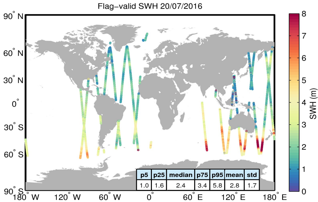
Figure 15. Geographical distribution of flag-valid SWH data over oceans and lakes for 20/07/2016. The statistical values shown in the table refer to the SWH in m and are calculated over all measurements shown in the figure.
