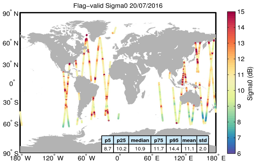
Figure 23. Geographical distribution of flag-valid sigma0 data over oceans and lakes for 20/07/2016. The statistical values shown in the table refer to the sigma0 in dB and are calculated over all measurements shown in the figure.
