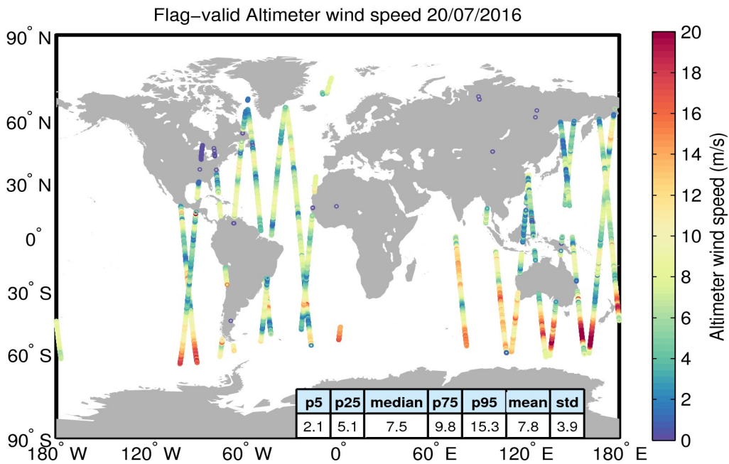
Figure 31. Geographical distribution of flag-valid wind data over oceans and lakes for 20/07/2016. The statistical values shown in the table refer to the wind in m/s and are calculated over all measurements shown in the figure.
