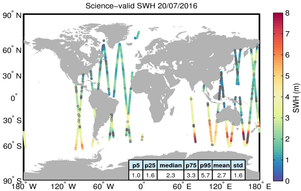
Figure 19. Geographical distribution of science-valid SWH data over oceans and lakes for 20/07/2016. The statistical values shown in the table refer to the SWH in m and are calculated over all measurements shown in the figure. Gray circles denote records that have been rejected based on the editing criteria described in Table 3.
