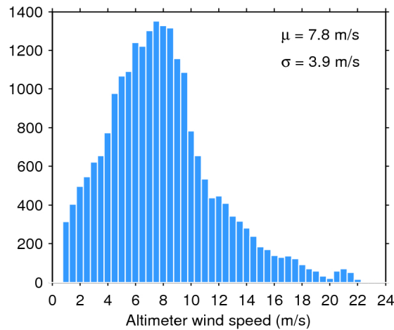
Figure 33. Histogram of flag-valid wind over oceans and lakes for 20/07/2016. The mean ( \mu ) and standard deviation ( \sigma ) are also shown. Note that values larger than 24 m/s are excluded from the histogram for the sake of readability but not from the computation of \mu and \sigma .
