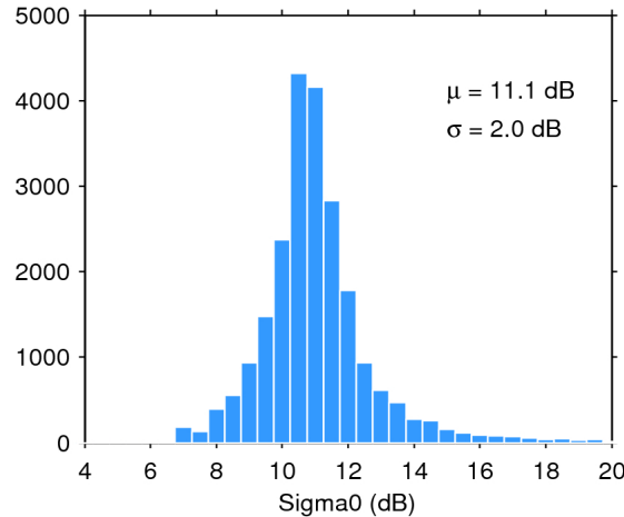
Figure 25. Histogram of flag-valid sigma0 over oceans and lakes for 20/07/2016. The mean ( \mu ) and standard deviation ( \sigma ) are also shown. Note that values outside [4 20] dB are excluded from the histogram for the sake of readability but not from the computation of \mu and \sigma .
