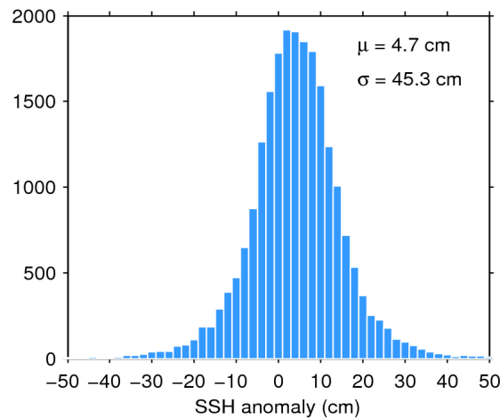
Figure 7. Histogram of flag-valid SSH anomaly over oceans and lakes for 20/07/2016. The mean ( \mu ) and standard deviation ( \sigma ) are also shown. Note that values outside [-50\ 50] cm are excluded from the histogram for the sake of readability but not from the computation of \mu and \sigma .
