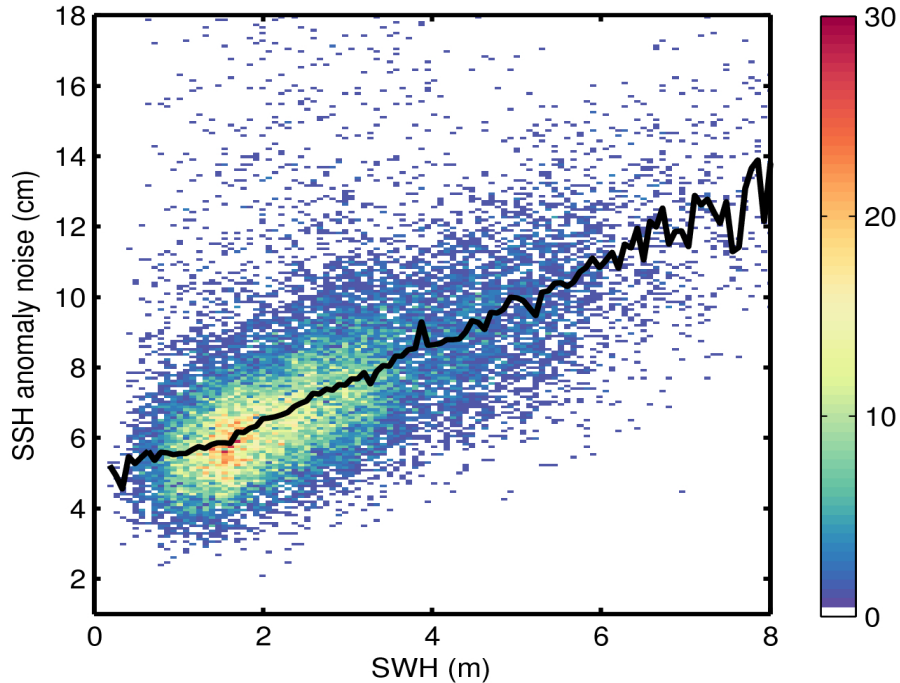
Figure 9. 2D histogram showing flag-valid SSH anomaly noise as a function of SWH for 20/07/2016. The black line denotes the median SSH anomaly noise as a function of SWH.
