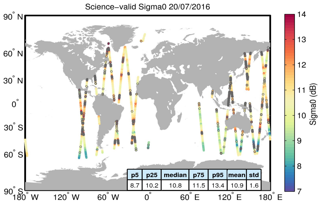
Figure 27. Geographical distribution of science-valid sigma0 data over oceans and lakes for 20/07/2016. The statistical values shown in the table refer to the sigma0 in dB and are calculated over all measurements shown in the figure. Gray circles denote records that have been rejected based on the editing criteria described in Table 4.
