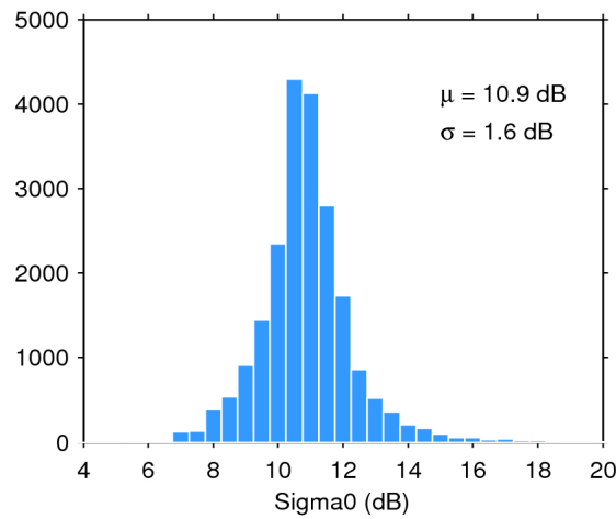
Figure 28. Histogram of science-valid sigma0 over oceans and lakes for 20/07/2016. The mean ( \mu ) and standard deviation ( \sigma ) are also shown. Note that values outside [4 20] dB are excluded from the histogram for the sake of readability but not from the computation of \mu and \sigma .
