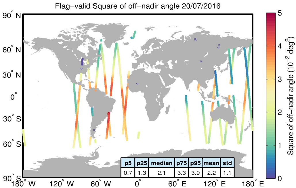
Figure 37. Geographical distribution of flag-valid mispointing data over oceans and lakes for 20/07/2016. The statistical values shown in the table refer to the mispointing in 10^{-2} \text{ deg}^2 and are calculated over all measurements shown in the figure.
