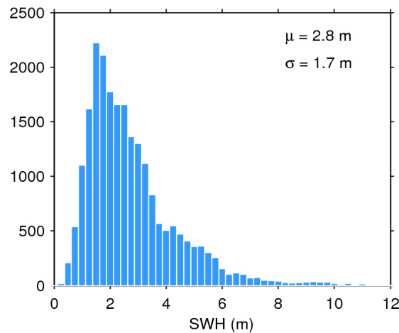
Figure 17. Histogram of flag-valid SWH over oceans and lakes for 20/07/2016. The mean ( \mu ) and standard deviation ( \sigma ) are also shown. Note that values larger than 12 m are excluded from the histogram for the sake of readability but not from the computation of \mu and \sigma .
