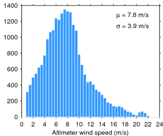
Figure 35. Histogram of science-valid wind over oceans and lakes for 20/07/2016. The mean ( \mu ) and standard deviation ( \sigma ) are also shown. Note that values larger than 24 m/s are excluded from the histogram for the sake of readability but not from the computation of \mu and \sigma .
