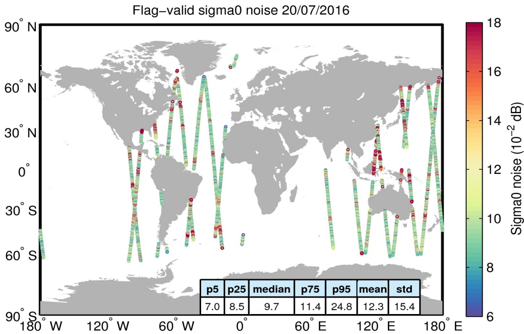
Figure 26. Geographical distribution of flag-valid 20-Hz sigma0 measurement noise over oceans and lakes for 20/07/2016. The statistical values shown in the table refer to the sigma0 noise and are calculated over all measurements shown in the figure.
