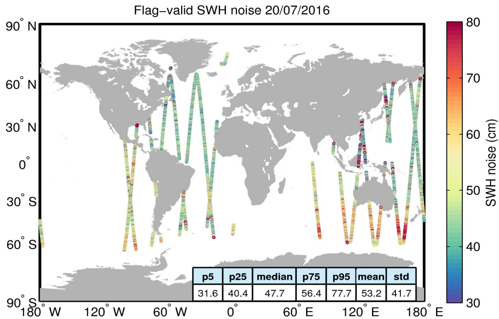
Figure 18. Geographical distribution of flag-valid 20-Hz SWH measurement noise over oceans and lakes for 20/07/2016. The statistical values shown in the table refer to the SWH noise and are calculated over all measurements shown in the figure.
