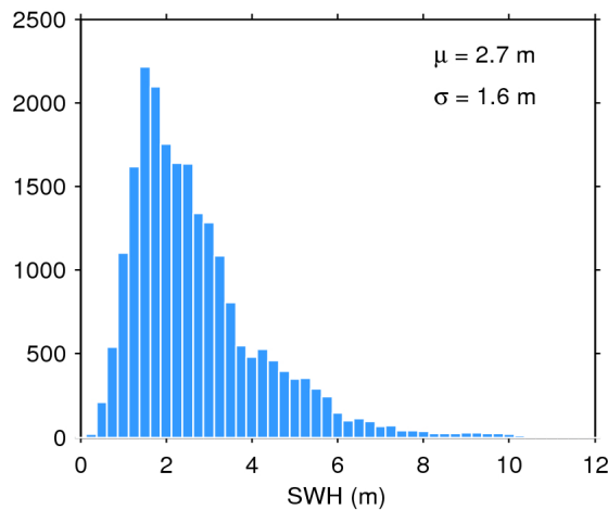
Figure 20. Histogram of science-valid SWH over oceans and lakes for 20/07/2016. The mean ( \mu ) and standard deviation ( \sigma ) are also shown. Note that values larger than 12 m are excluded from the histogram for the sake of readability but not from the computation of \mu and \sigma .
