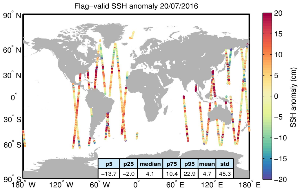
Figure 5. Geographical distribution of flag-valid 1-Hz SSH anomaly data over oceans and lakes for 20/07/2016. The statistical values shown in the table refer to the SSH anomaly in cm and are calculated over all measurements shown in the figure.
