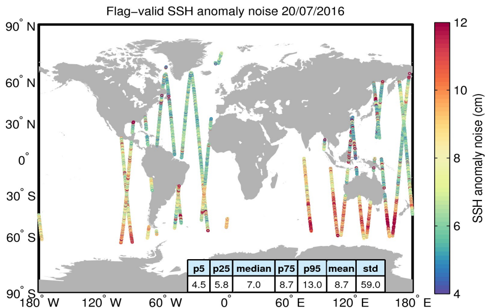
Figure 8. Geographical distribution of flag-valid 20-Hz SSH anomaly measurement noise over oceans and lakes for 20/07/2016. The statistical values shown in the table refer to the SSH anomaly noise and are calculated over all measurements shown in the figure.
