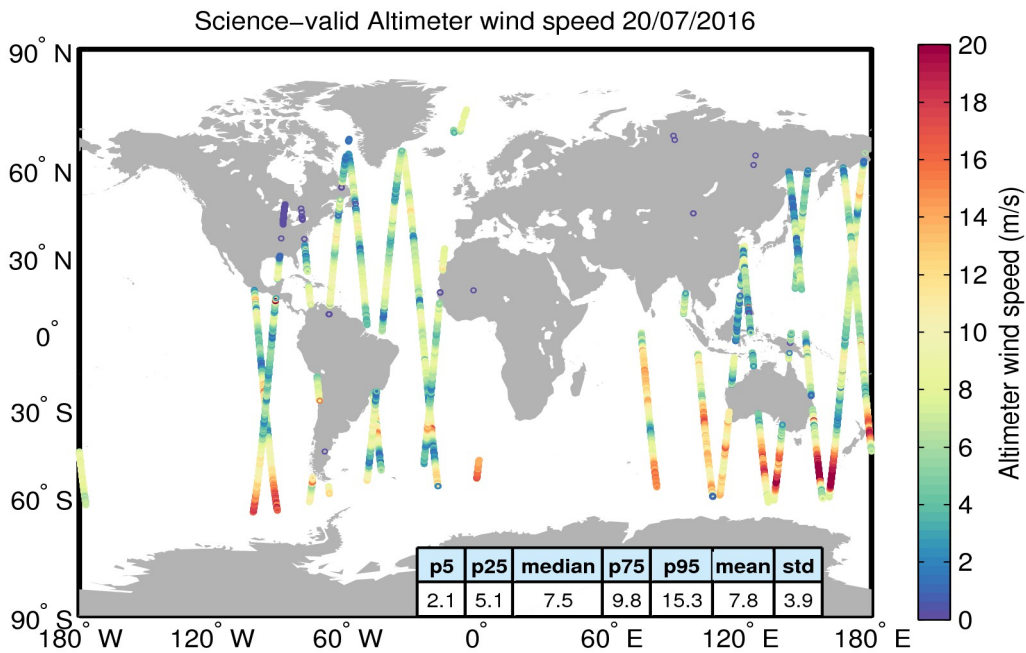
Figure 34. Geographical distribution of science-valid wind data over oceans and lakes for 20/07/2016. The statistical values shown in the table refer to the wind in m/s and are calculated over all measurements shown in the figure. Gray circles denote records that have been rejected based on the editing criteria described in Table 5.
