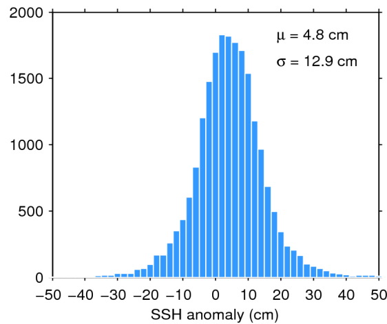
Figure 11. Histogram of science-valid SSH anomaly over oceans and lakes for 20/07/2016. The mean ( \mu ) and standard deviation ( \sigma ) are also shown. Note that values outside [-50 50] cm are excluded from the histogram for the sake of readability but not from the computation of \mu and \sigma .
