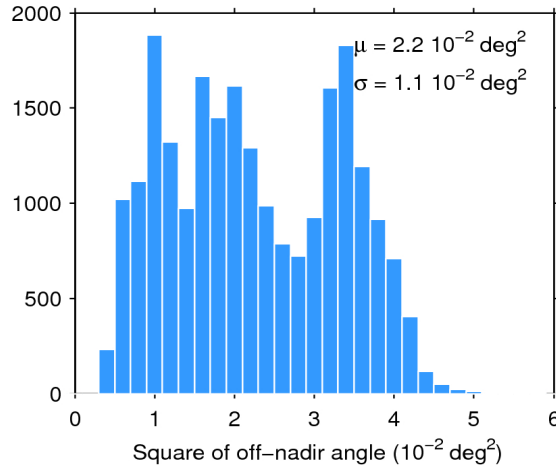
Figure 39. Histogram of flag-valid mispointing over oceans and lakes for 20/07/2016. The mean ( \mu ) and standard deviation ( \sigma ) are also shown. Note that values larger than 6 \cdot 10^{-2} \text{ deg}^2 are excluded from the histogram for the sake of readability but not from the computation of \mu and \sigma .
