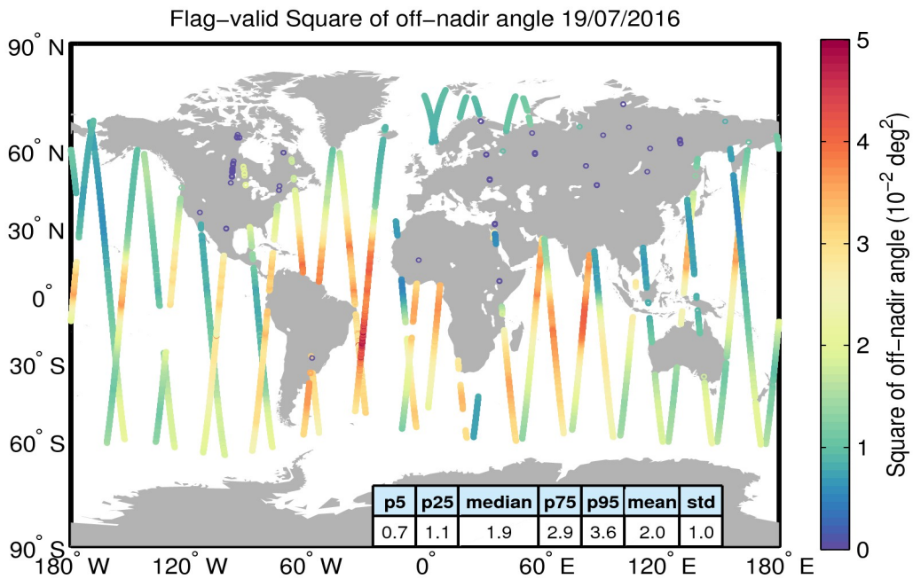
Figure 37. Geographical distribution of flag-valid mispointing data over oceans and lakes for 19/07/2016. The statistical values shown in the table refer to the mispointing in 10^{-2} deg 2 and are calculated over all measurements shown in the figure.
