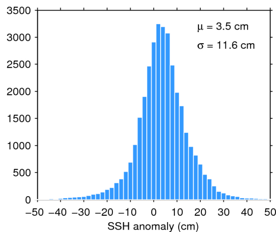
Figure 11. Histogram of science-valid SSH anomaly over oceans and lakes for 19/07/2016. The mean ( \mu ) and standard deviation ( \sigma ) are also shown. Note that values outside [-50 50] cm are excluded from the histogram for the sake of readability but not from the computation of \mu and \sigma .
