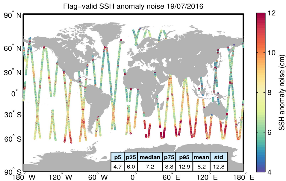
Figure 8. Geographical distribution of flag-valid 20-Hz SSH anomaly measurement noise over oceans and lakes for 19/07/2016. The statistical values shown in the table refer to the SSH anomaly noise and are calculated over all measurements shown in the figure.
