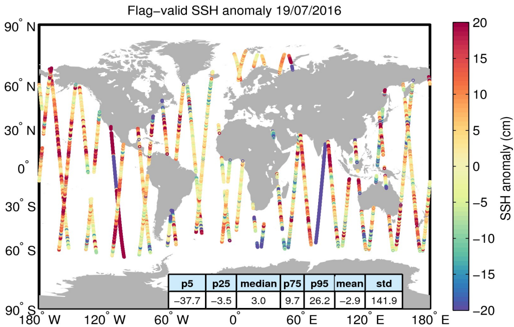
Figure 5. Geographical distribution of flag-valid 1-Hz SSH anomaly data over oceans and lakes for 19/07/2016. The statistical values shown in the table refer to the SSH anomaly in cm and are calculated over all measurements shown in the figure.
