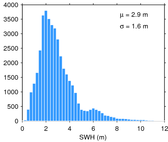
Figure 17. Histogram of flag-valid SWH over oceans and lakes for 19/07/2016. The mean ( \mu ) and standard deviation ( \sigma ) are also shown. Note that values larger than 12 m are excluded from the histogram for the sake of readability but not from the computation of \mu and \sigma .
