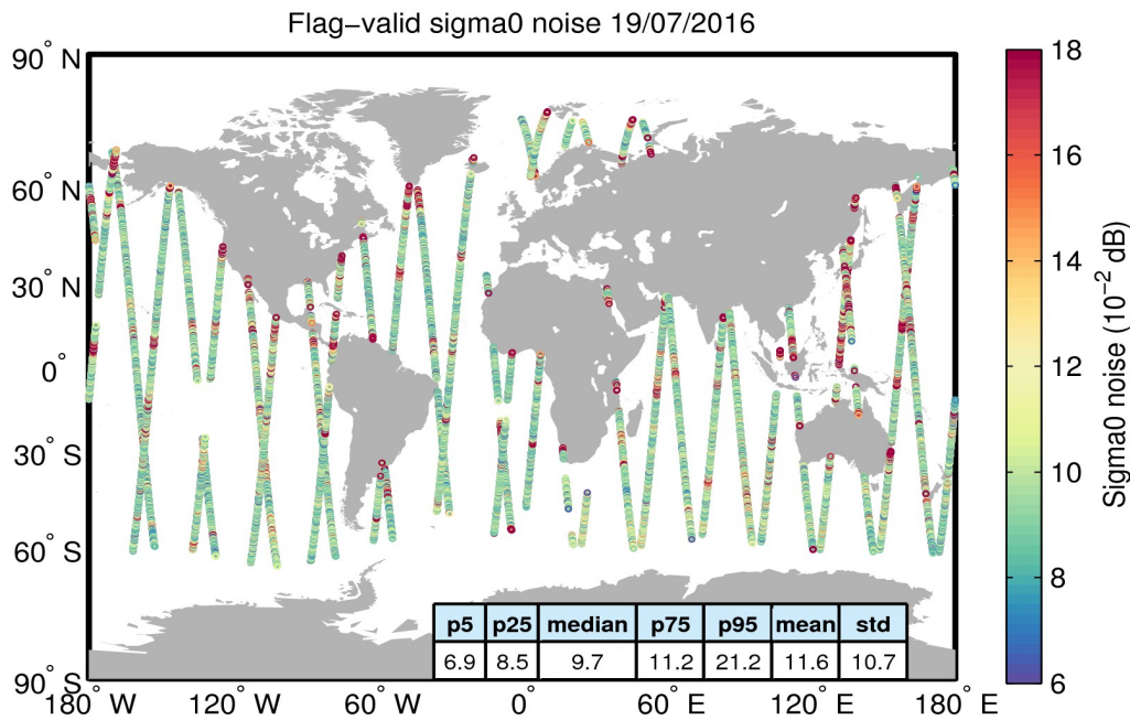
Figure 26. Geographical distribution of flag-valid 20-Hz sigma0 measurement noise over oceans and lakes for 19/07/2016. The statistical values shown in the table refer to the sigma0 noise and are calculated over all measurements shown in the figure.
