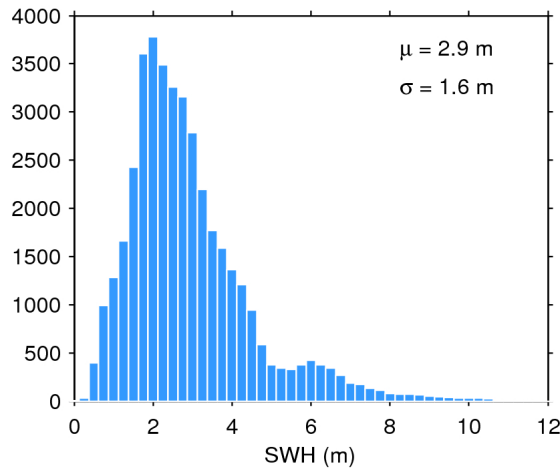
Figure 20. Histogram of science-valid SWH over oceans and lakes for 19/07/2016. The mean ( \mu ) and standard deviation ( \sigma ) are also shown. Note that values larger than 12 m are excluded from the histogram for the sake of readability but not from the computation of \mu and \sigma .
