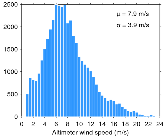
Figure 33. Histogram of flag-valid wind over oceans and lakes for 19/07/2016. The mean ( \mu ) and standard deviation ( \sigma ) are also shown. Note that values larger than 24 m/s are excluded from the histogram for the sake of readability but not from the computation of \mu and \sigma .
