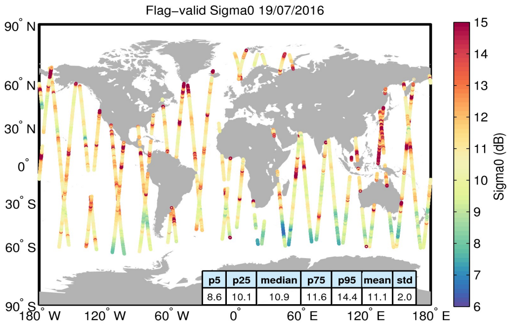
Figure 23. Geographical distribution of flag-valid sigma0 data over oceans and lakes for 19/07/2016. The statistical values shown in the table refer to the sigma0 in dB and are calculated over all measurements shown in the figure.
