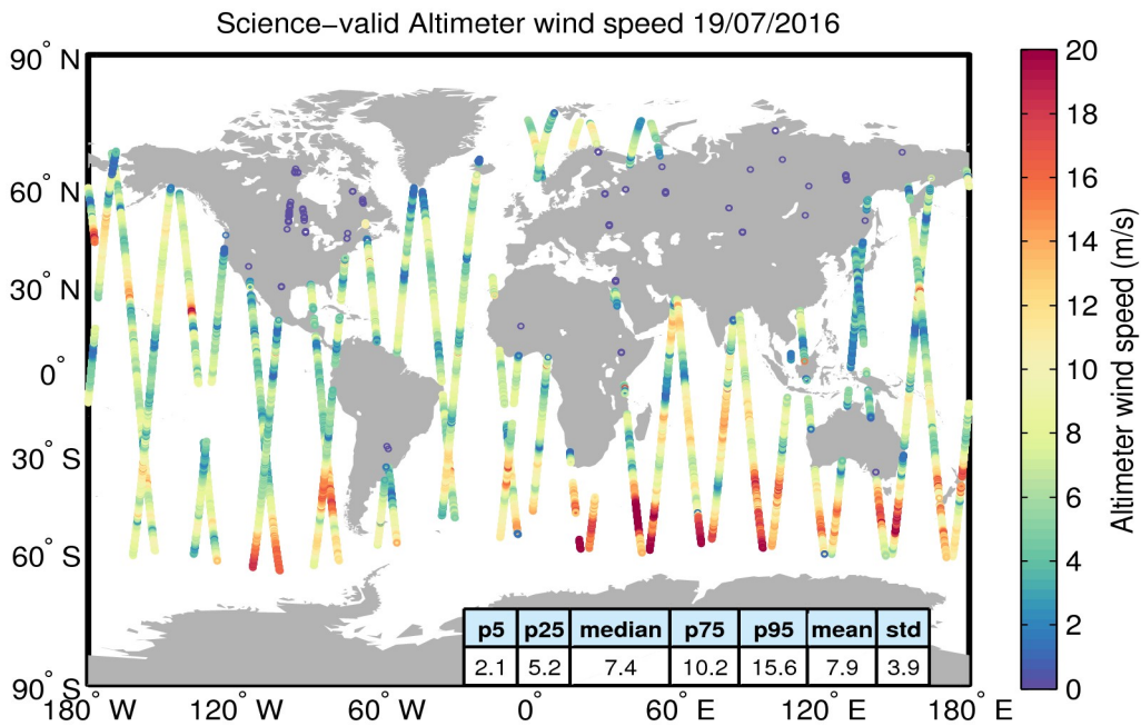
Figure 34. Geographical distribution of science-valid wind data over oceans and lakes for 19/07/2016. The statistical values shown in the table refer to the wind in m/s and are calculated over all measurements shown in the figure. Gray circles denote records that have been rejected based on the editing criteria described in Table 5.
