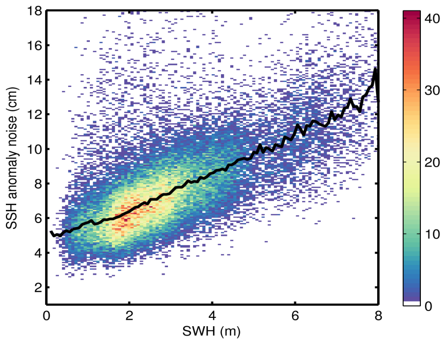
Figure 9. 2D histogram showing flag-valid SSH anomaly noise as a function of SWH for 19/07/2016. The black line denotes the median SSH anomaly noise as a function of SWH.
