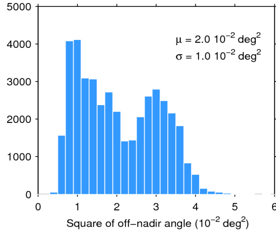
Figure 39. Histogram of flag-valid mispointing over oceans and lakes for 19/07/2016. The mean ( \mu ) and standard deviation ( \sigma ) are also shown. Note that values larger than 6 \cdot 10^{-2} \text{ deg}^2 are excluded from the histogram for the sake of readability but not from the computation of \mu and \sigma .
