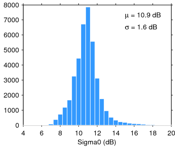
Figure 28. Histogram of science-valid sigma0 over oceans and lakes for 19/07/2016. The mean ( \mu ) and standard deviation ( \sigma ) are also shown. Note that values outside [4 20] dB are excluded from the histogram for the sake of readability but not from the computation of \mu and \sigma .
