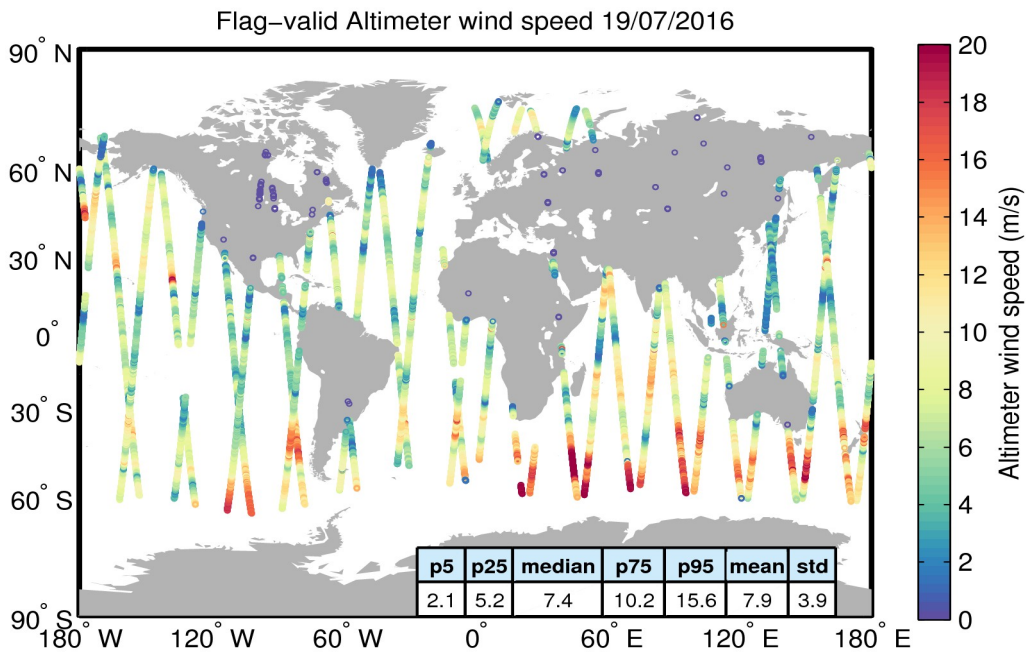
Figure 31. Geographical distribution of flag-valid wind data over oceans and lakes for 19/07/2016. The statistical values shown in the table refer to the wind in m/s and are calculated over all measurements shown in the figure.
