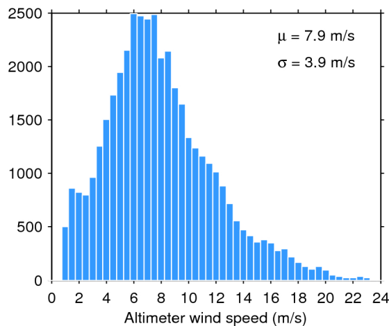
Figure 35. Histogram of science-valid wind over oceans and lakes for 19/07/2016. The mean ( \mu ) and standard deviation ( \sigma ) are also shown. Note that values larger than 24 m/s are excluded from the histogram for the sake of readability but not from the computation of \mu and \sigma .
