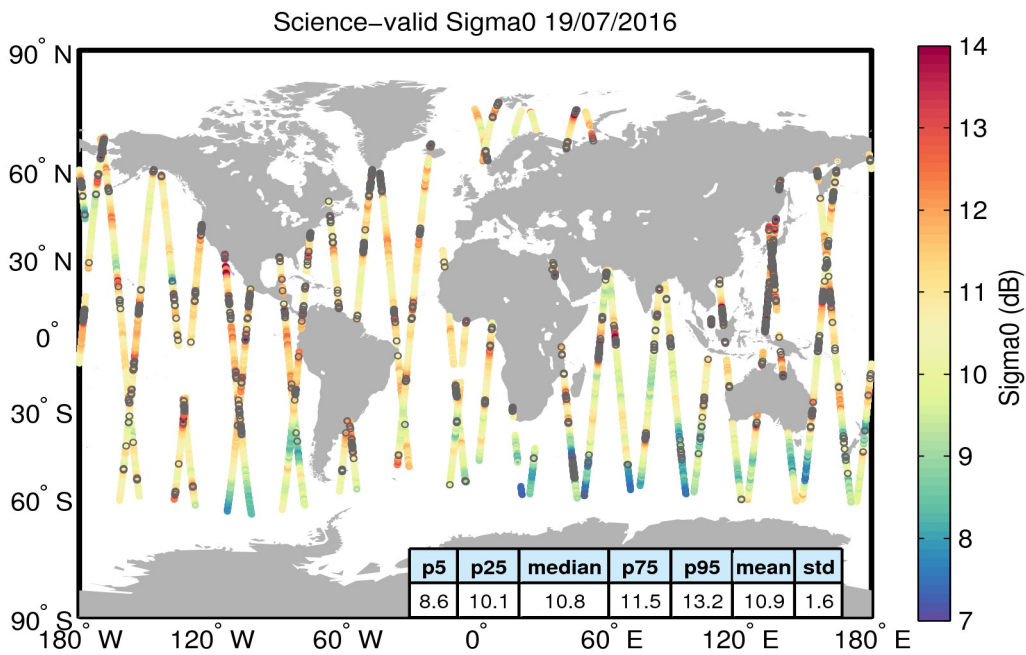
Figure 27. Geographical distribution of science-valid sigma0 data over oceans and lakes for 19/07/2016. The statistical values shown in the table refer to the sigma0 in dB and are calculated over all measurements shown in the figure. Gray circles denote records that have been rejected based on the editing criteria described in Table 4.
