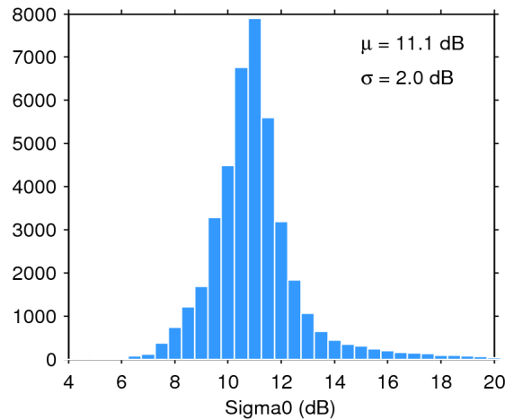
Figure 25. Histogram of flag-valid sigma0 over oceans and lakes for 19/07/2016. The mean ( \mu ) and standard deviation ( \sigma ) are also shown. Note that values outside [4 20] dB are excluded from the histogram for the sake of readability but not from the computation of \mu and \sigma .
