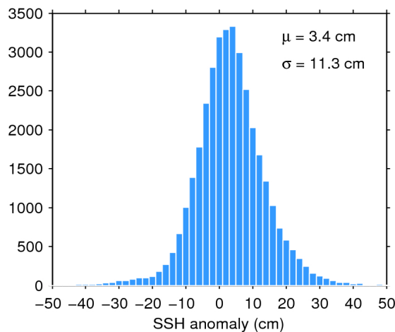
Figure 11. Histogram of science-valid SSH anomaly over oceans and lakes for 18/07/2016. The mean ( \mu ) and standard deviation ( \sigma ) are also shown. Note that values outside [-50 50] cm are excluded from the histogram for the sake of readability but not from the computation of \mu and \sigma .
