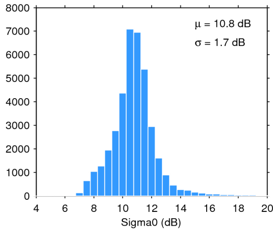
Figure 28. Histogram of science-valid sigma0 over oceans and lakes for 18/07/2016. The mean ( \mu ) and standard deviation ( \sigma ) are also shown. Note that values outside [4 20] dB are excluded from the histogram for the sake of readability but not from the computation of \mu and \sigma .
