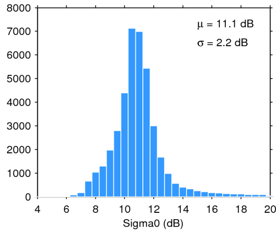
Figure 25. Histogram of flag-valid sigma0 over oceans and lakes for 18/07/2016. The mean ( \mu ) and standard deviation ( \sigma ) are also shown. Note that values outside [4 20] dB are excluded from the histogram for the sake of readability but not from the computation of \mu and \sigma .
