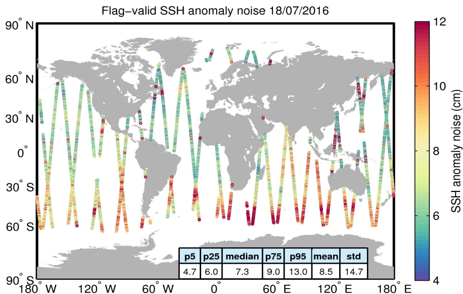
Figure 8. Geographical distribution of flag-valid 20-Hz SSH anomaly measurement noise over oceans and lakes for 18/07/2016. The statistical values shown in the table refer to the SSH anomaly noise and are calculated over all measurements shown in the figure.
