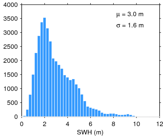
Figure 20. Histogram of science-valid SWH over oceans and lakes for 18/07/2016. The mean ( \mu ) and standard deviation ( \sigma ) are also shown. Note that values larger than 12 m are excluded from the histogram for the sake of readability but not from the computation of \mu and \sigma .
