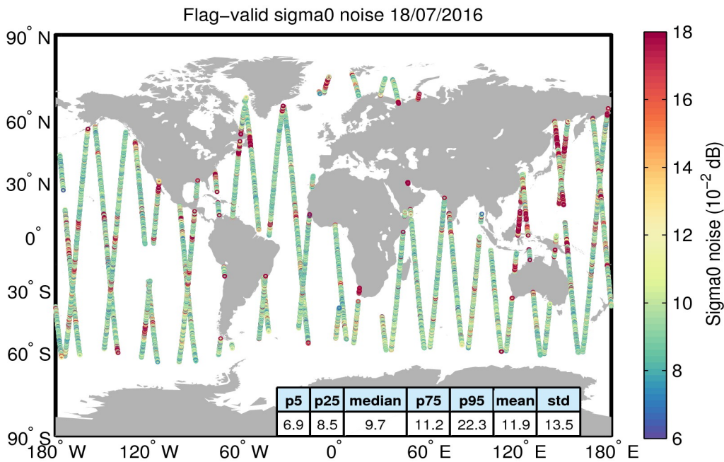
Figure 26. Geographical distribution of flag-valid 20-Hz sigma0 measurement noise over oceans and lakes for 18/07/2016. The statistical values shown in the table refer to the sigma0 noise and are calculated over all measurements shown in the figure.
