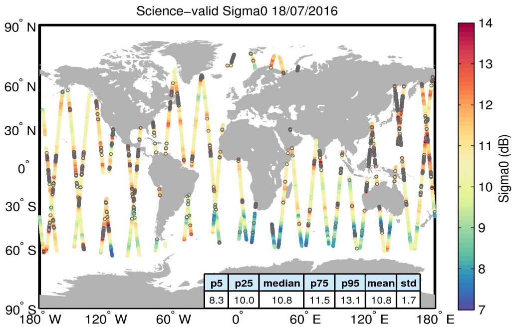
Figure 27. Geographical distribution of science-valid sigma0 data over oceans and lakes for 18/07/2016. The statistical values shown in the table refer to the sigma0 in dB and are calculated over all measurements shown in the figure. Gray circles denote records that have been rejected based on the editing criteria described in Table 4.
