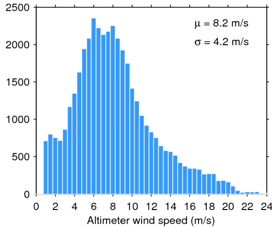
Figure 33. Histogram of flag-valid wind over oceans and lakes for 18/07/2016. The mean ( \mu ) and standard deviation ( \sigma ) are also shown. Note that values larger than 24 m/s are excluded from the histogram for the sake of readability but not from the computation of \mu and \sigma .
