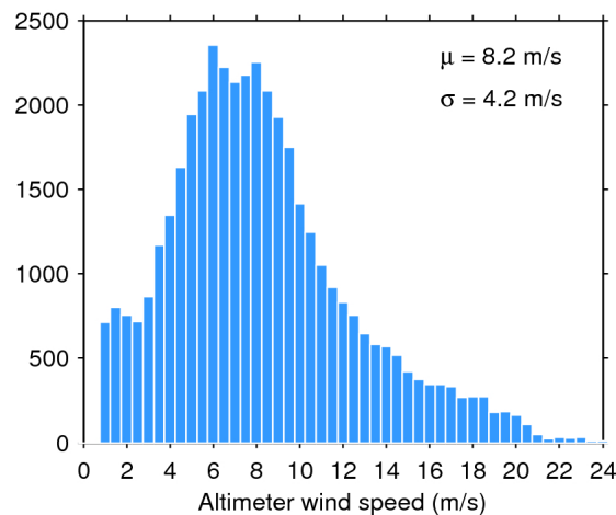
Figure 35. Histogram of science-valid wind over oceans and lakes for 18/07/2016. The mean ( \mu ) and standard deviation ( \sigma ) are also shown. Note that values larger than 24 m/s are excluded from the histogram for the sake of readability but not from the computation of \mu and \sigma .
