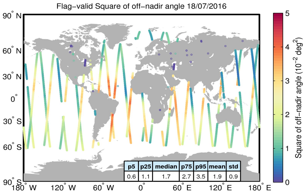
Figure 37. Geographical distribution of flag-valid mispointing data over oceans and lakes for 18/07/2016. The statistical values shown in the table refer to the mispointing in 10^{-2} \text{ deg}^2 and are calculated over all measurements shown in the figure.
