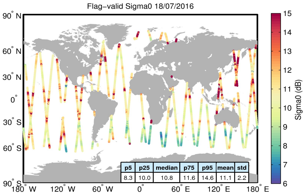
Figure 23. Geographical distribution of flag-valid sigma0 data over oceans and lakes for 18/07/2016. The statistical values shown in the table refer to the sigma0 in dB and are calculated over all measurements shown in the figure.
