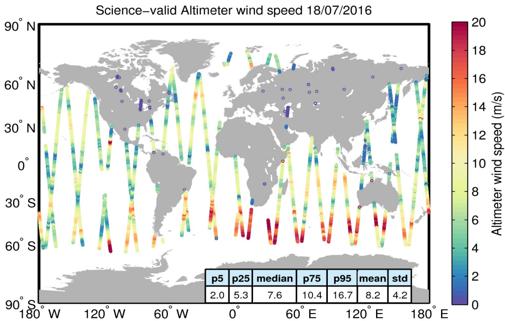
Figure 34. Geographical distribution of science-valid wind data over oceans and lakes for 18/07/2016. The statistical values shown in the table refer to the wind in m/s and are calculated over all measurements shown in the figure. Gray circles denote records that have been rejected based on the editing criteria described in Table 5.
