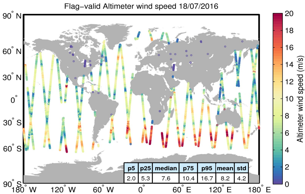
Figure 31. Geographical distribution of flag-valid wind data over oceans and lakes for 18/07/2016. The statistical values shown in the table refer to the wind in m/s and are calculated over all measurements shown in the figure.
