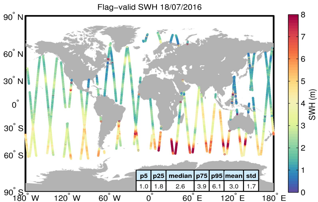
Figure 15. Geographical distribution of flag-valid SWH data over oceans and lakes for 18/07/2016. The statistical values shown in the table refer to the SWH in m and are calculated over all measurements shown in the figure.
