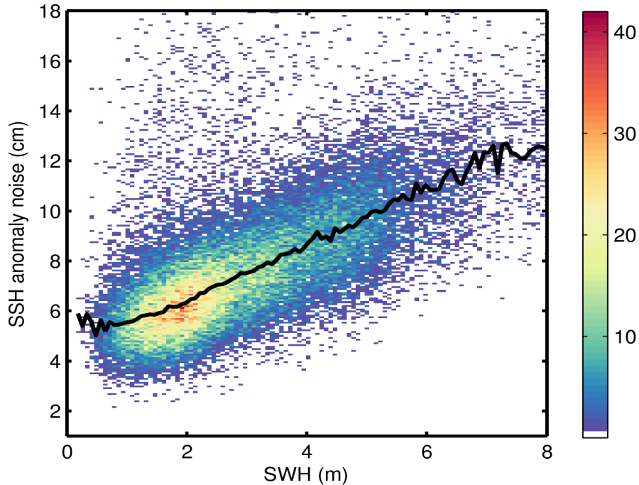
Figure 9. 2D histogram showing flag-valid SSH anomaly noise as a function of SWH for 18/07/2016. The black line denotes the median SSH anomaly noise as a function of SWH.
