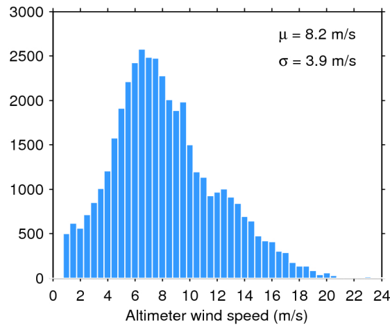
Figure 33. Histogram of flag-valid wind over oceans and lakes for 17/07/2016. The mean ( \mu ) and standard deviation ( \sigma ) are also shown. Note that values larger than 24 m/s are excluded from the histogram for the sake of readability but not from the computation of \mu and \sigma .
