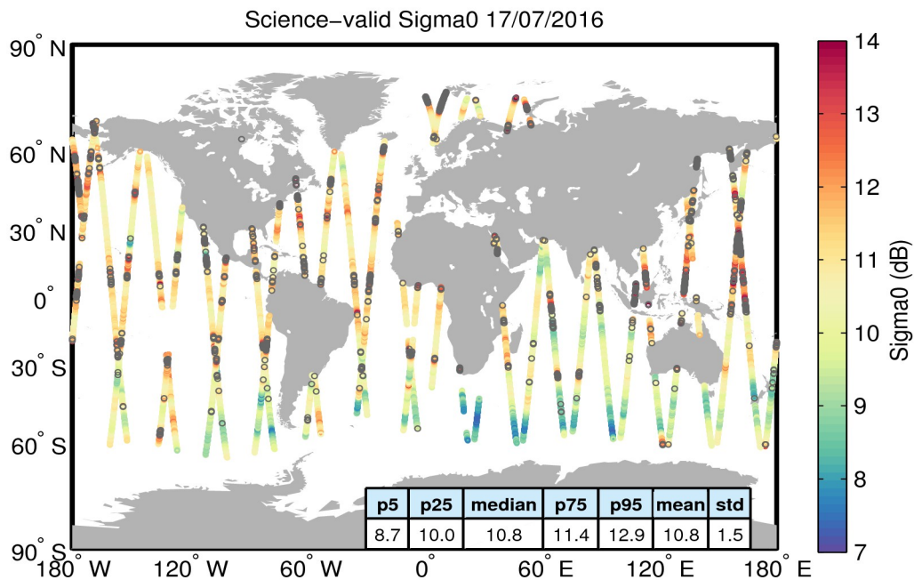
Figure 27. Geographical distribution of science-valid sigma0 data over oceans and lakes for 17/07/2016. The statistical values shown in the table refer to the sigma0 in dB and are calculated over all measurements shown in the figure. Gray circles denote records that have been rejected based on the editing criteria described in Table 4.
