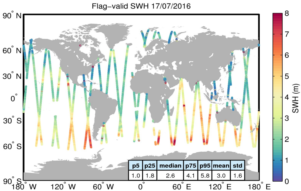
Figure 15. Geographical distribution of flag-valid SWH data over oceans and lakes for 17/07/2016. The statistical values shown in the table refer to the SWH in m and are calculated over all measurements shown in the figure.
