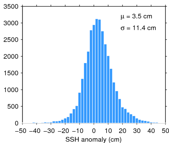
Figure 11. Histogram of science-valid SSH anomaly over oceans and lakes for 17/07/2016. The mean ( \mu ) and standard deviation ( \sigma ) are also shown. Note that values outside [-50 50] cm are excluded from the histogram for the sake of readability but not from the computation of \mu and \sigma .
