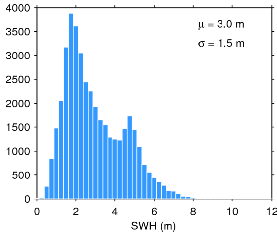
Figure 20. Histogram of science-valid SWH over oceans and lakes for 17/07/2016. The mean ( \mu ) and standard deviation ( \sigma ) are also shown. Note that values larger than 12 m are excluded from the histogram for the sake of readability but not from the computation of \mu and \sigma .
