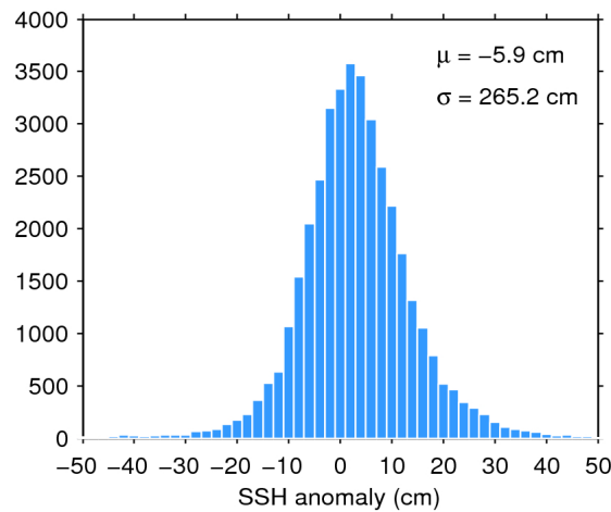
Figure 7. Histogram of flag-valid SSH anomaly over oceans and lakes for 17/07/2016. The mean ( \mu ) and standard deviation ( \sigma ) are also shown. Note that values outside [-50 50] cm are excluded from the histogram for the sake of readability but not from the computation of \mu and \sigma .
