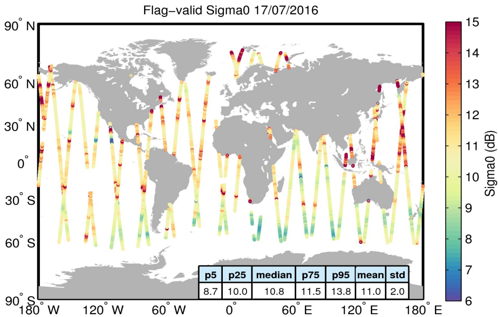
Figure 23. Geographical distribution of flag-valid sigma0 data over oceans and lakes for 17/07/2016. The statistical values shown in the table refer to the sigma0 in dB and are calculated over all measurements shown in the figure.
