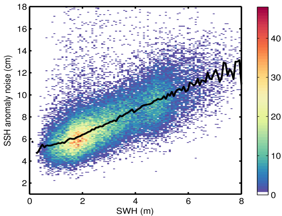
Figure 9. 2D histogram showing flag-valid SSH anomaly noise as a function of SWH for 17/07/2016. The black line denotes the median SSH anomaly noise as a function of SWH.
