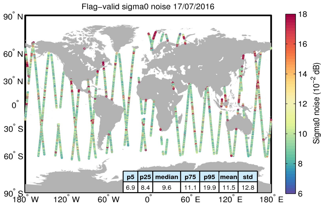
Figure 26. Geographical distribution of flag-valid 20-Hz sigma0 measurement noise over oceans and lakes for 17/07/2016. The statistical values shown in the table refer to the sigma0 noise and are calculated over all measurements shown in the figure.
