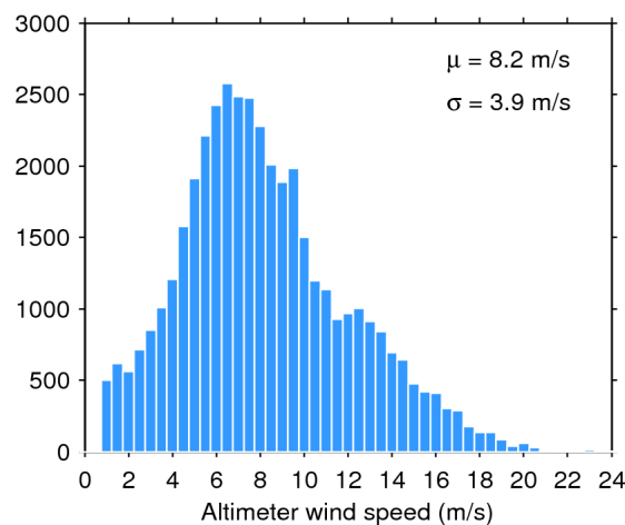
Figure 35. Histogram of science-valid wind over oceans and lakes for 17/07/2016. The mean ( \mu ) and standard deviation ( \sigma ) are also shown. Note that values larger than 24 m/s are excluded from the histogram for the sake of readability but not from the computation of \mu and \sigma .
