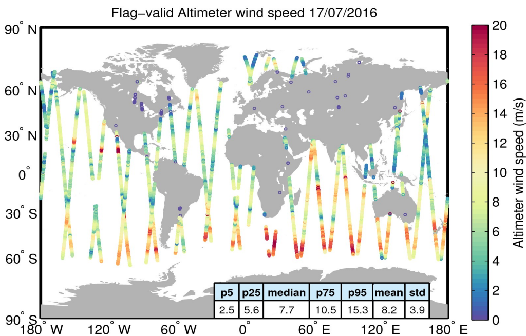
Figure 31. Geographical distribution of flag-valid wind data over oceans and lakes for 17/07/2016. The statistical values shown in the table refer to the wind in m/s and are calculated over all measurements shown in the figure.
