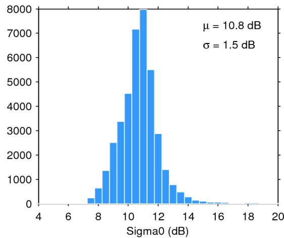
Figure 28. Histogram of science-valid sigma0 over oceans and lakes for 17/07/2016. The mean ( \mu ) and standard deviation ( \sigma ) are also shown. Note that values outside [4 20] dB are excluded from the histogram for the sake of readability but not from the computation of \mu and \sigma .
