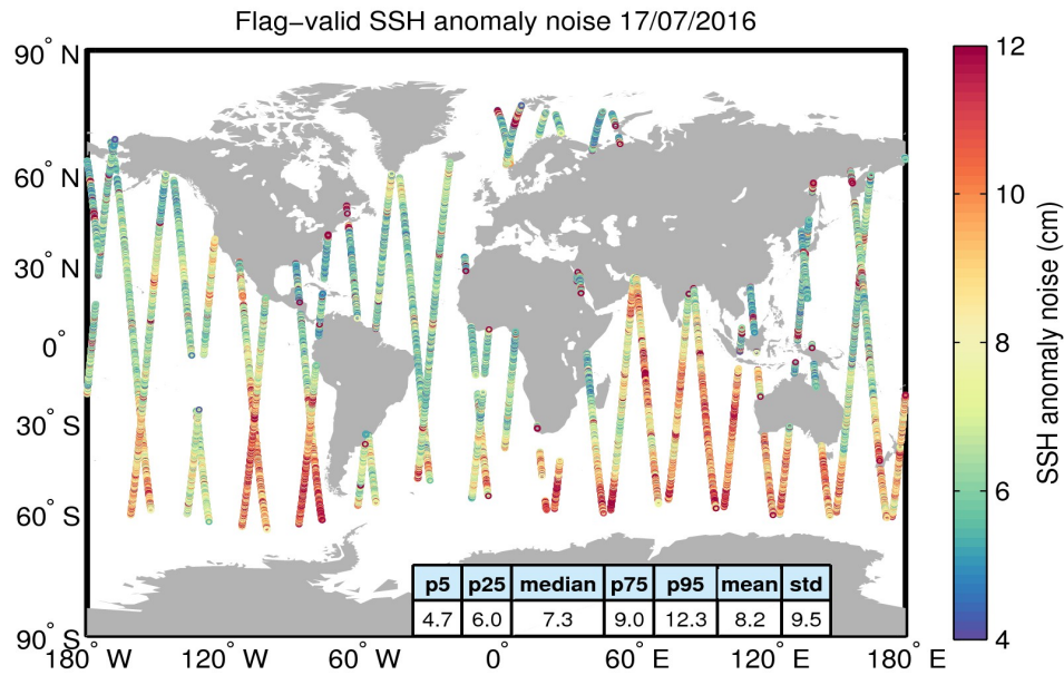
Figure 8. Geographical distribution of flag-valid 20-Hz SSH anomaly measurement noise over oceans and lakes for 17/07/2016. The statistical values shown in the table refer to the SSH anomaly noise and are calculated over all measurements shown in the figure.
