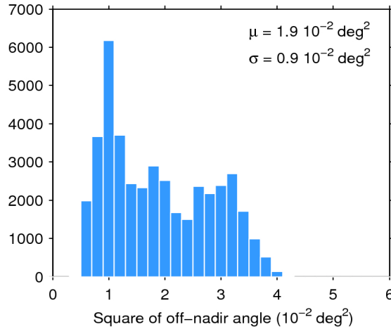
Figure 39. Histogram of flag-valid mispointing over oceans and lakes for 17/07/2016. The mean ( \mu ) and standard deviation ( \sigma ) are also shown. Note that values larger than 6 \cdot 10^{-2} \text{ deg}^2 are excluded from the histogram for the sake of readability but not from the computation of \mu and \sigma .
