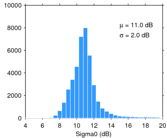
Figure 25. Histogram of flag-valid sigma0 over oceans and lakes for 17/07/2016. The mean ( \mu ) and standard deviation ( \sigma ) are also shown. Note that values outside [4 20] dB are excluded from the histogram for the sake of readability but not from the computation of \mu and \sigma .
