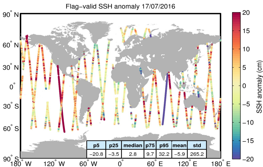
Figure 5. Geographical distribution of flag-valid 1-Hz SSH anomaly data over oceans and lakes for 17/07/2016. The statistical values shown in the table refer to the SSH anomaly in cm and are calculated over all measurements shown in the figure.
