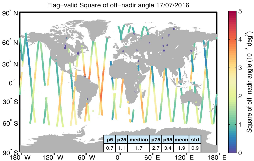
Figure 37. Geographical distribution of flag-valid mispointing data over oceans and lakes for 17/07/2016. The statistical values shown in the table refer to the mispointing in 10^{-2} deg 2 and are calculated over all measurements shown in the figure.
