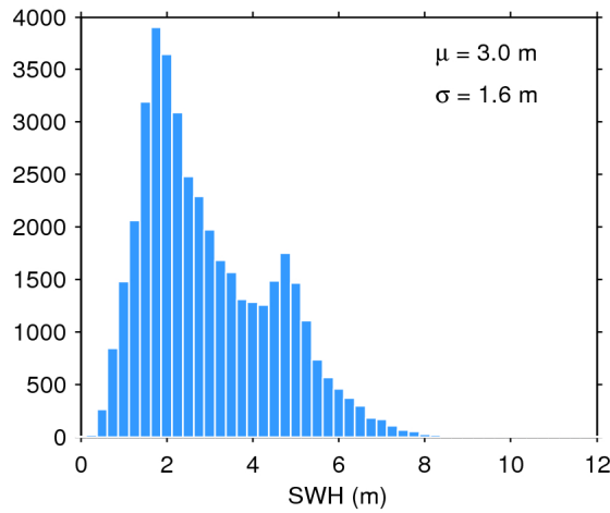
Figure 17. Histogram of flag-valid SWH over oceans and lakes for 17/07/2016. The mean ( \mu ) and standard deviation ( \sigma ) are also shown. Note that values larger than 12 m are excluded from the histogram for the sake of readability but not from the computation of \mu and \sigma .
