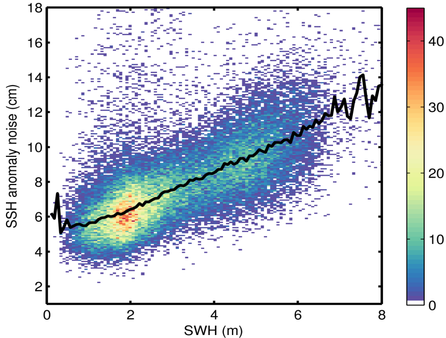
Figure 9. 2D histogram showing flag-valid SSH anomaly noise as a function of SWH for 16/07/2016. The black line denotes the median SSH anomaly noise as a function of SWH.
