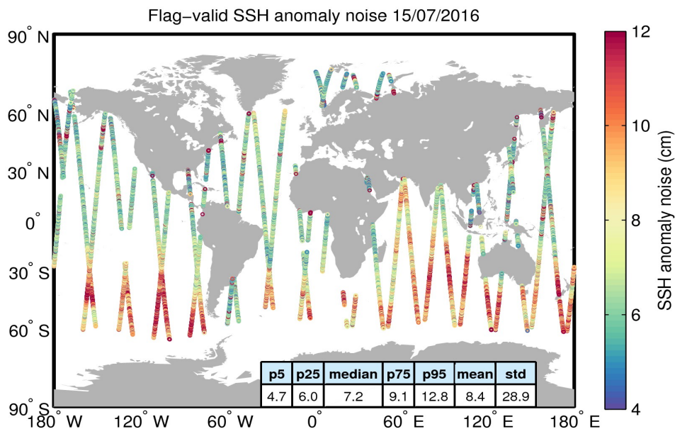
Figure 8. Geographical distribution of flag-valid 20-Hz SSH anomaly measurement noise over oceans and lakes for 15/07/2016. The statistical values shown in the table refer to the SSH anomaly noise and are calculated over all measurements shown in the figure.
