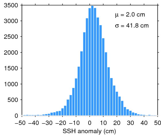
Figure 7. Histogram of flag-valid SSH anomaly over oceans and lakes for 15/07/2016. The mean ( \mu ) and standard deviation ( \sigma ) are also shown. Note that values outside [-50\ 50] cm are excluded from the histogram for the sake of readability but not from the computation of \mu and \sigma .
