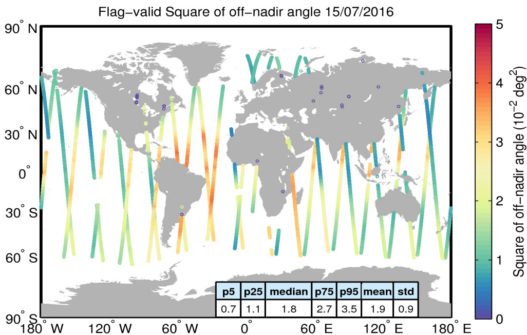
Figure 37. Geographical distribution of flag-valid mispointing data over oceans and lakes for 15/07/2016. The statistical values shown in the table refer to the mispointing in 10^{-2} deg 2 and are calculated over all measurements shown in the figure.
