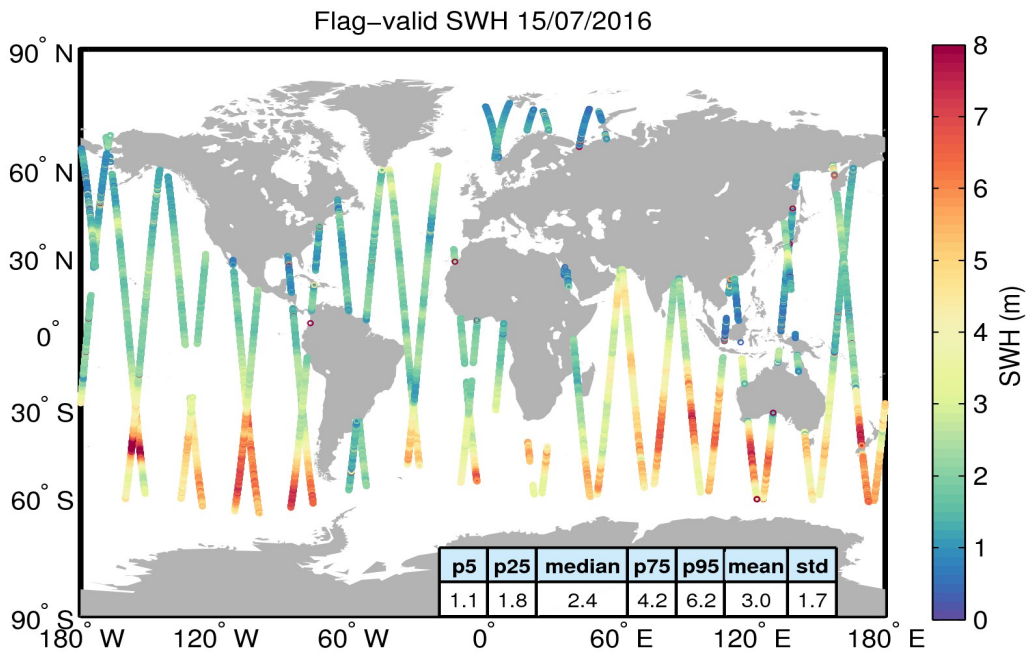
Figure 15. Geographical distribution of flag-valid SWH data over oceans and lakes for 15/07/2016. The statistical values shown in the table refer to the SWH in m and are calculated over all measurements shown in the figure.
