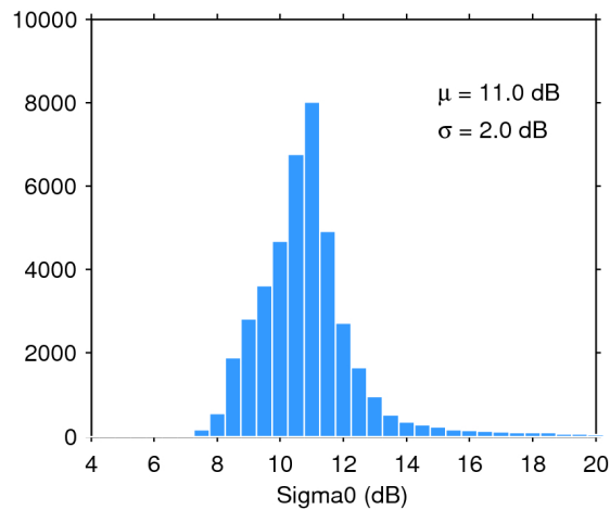
Figure 25. Histogram of flag-valid sigma0 over oceans and lakes for 15/07/2016. The mean ( \mu ) and standard deviation ( \sigma ) are also shown. Note that values outside [4 20] dB are excluded from the histogram for the sake of readability but not from the computation of \mu and \sigma .
