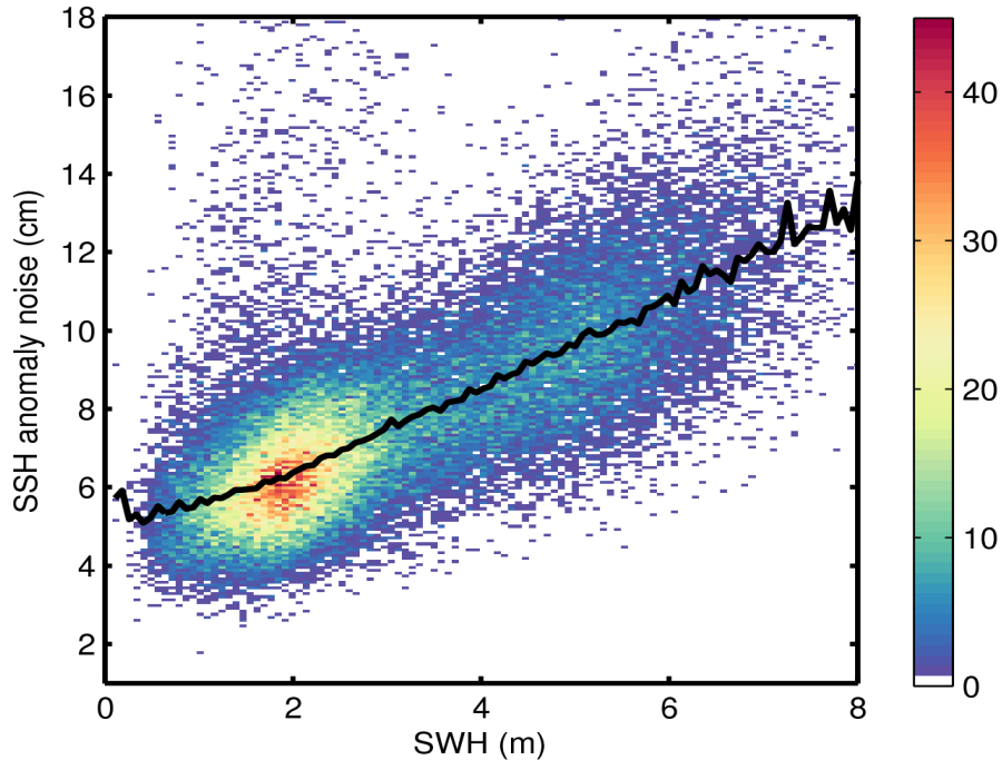
Figure 9. 2D histogram showing flag-valid SSH anomaly noise as a function of SWH for 15/07/2016. The black line denotes the median SSH anomaly noise as a function of SWH.
