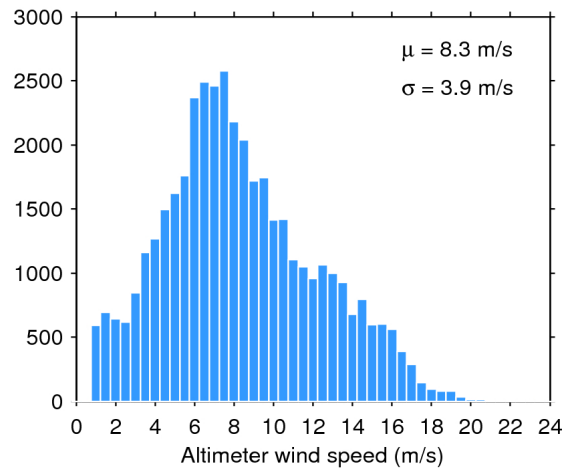
Figure 33. Histogram of flag-valid wind over oceans and lakes for 15/07/2016. The mean ( \mu ) and standard deviation ( \sigma ) are also shown. Note that values larger than 24 m/s are excluded from the histogram for the sake of readability but not from the computation of \mu and \sigma .
