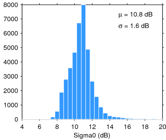
Figure 28. Histogram of science-valid sigma0 over oceans and lakes for 15/07/2016. The mean ( \mu ) and standard deviation ( \sigma ) are also shown. Note that values outside [4 20] dB are excluded from the histogram for the sake of readability but not from the computation of \mu and \sigma .
