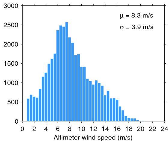
Figure 35. Histogram of science-valid wind over oceans and lakes for 15/07/2016. The mean ( \mu ) and standard deviation ( \sigma ) are also shown. Note that values larger than 24 m/s are excluded from the histogram for the sake of readability but not from the computation of \mu and \sigma .
