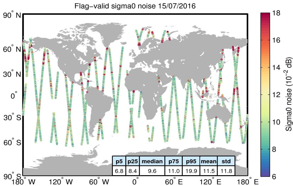
Figure 26. Geographical distribution of flag-valid 20-Hz sigma0 measurement noise over oceans and lakes for 15/07/2016. The statistical values shown in the table refer to the sigma0 noise and are calculated over all measurements shown in the figure.
