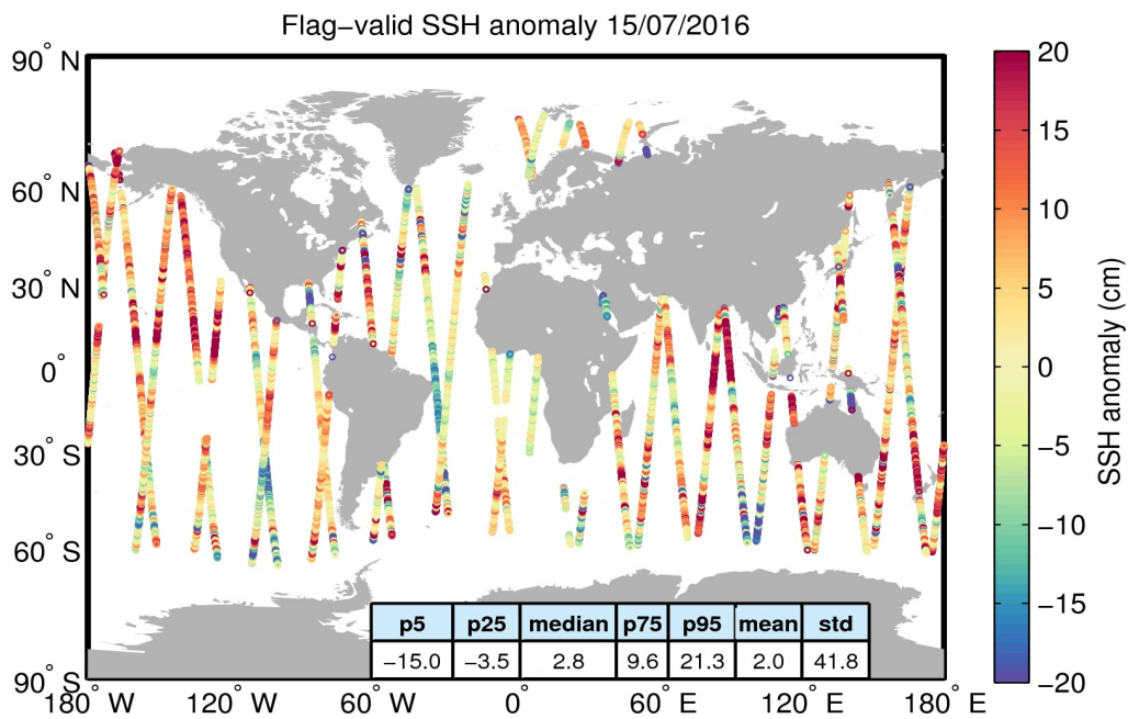
Figure 5. Geographical distribution of flag-valid 1-Hz SSH anomaly data over oceans and lakes for 15/07/2016. The statistical values shown in the table refer to the SSH anomaly in cm and are calculated over all measurements shown in the figure.
