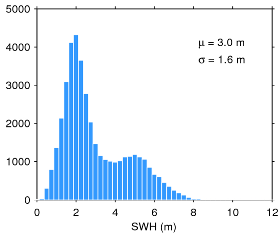
Figure 20. Histogram of science-valid SWH over oceans and lakes for 15/07/2016. The mean ( \mu ) and standard deviation ( \sigma ) are also shown. Note that values larger than 12 m are excluded from the histogram for the sake of readability but not from the computation of \mu and \sigma .
