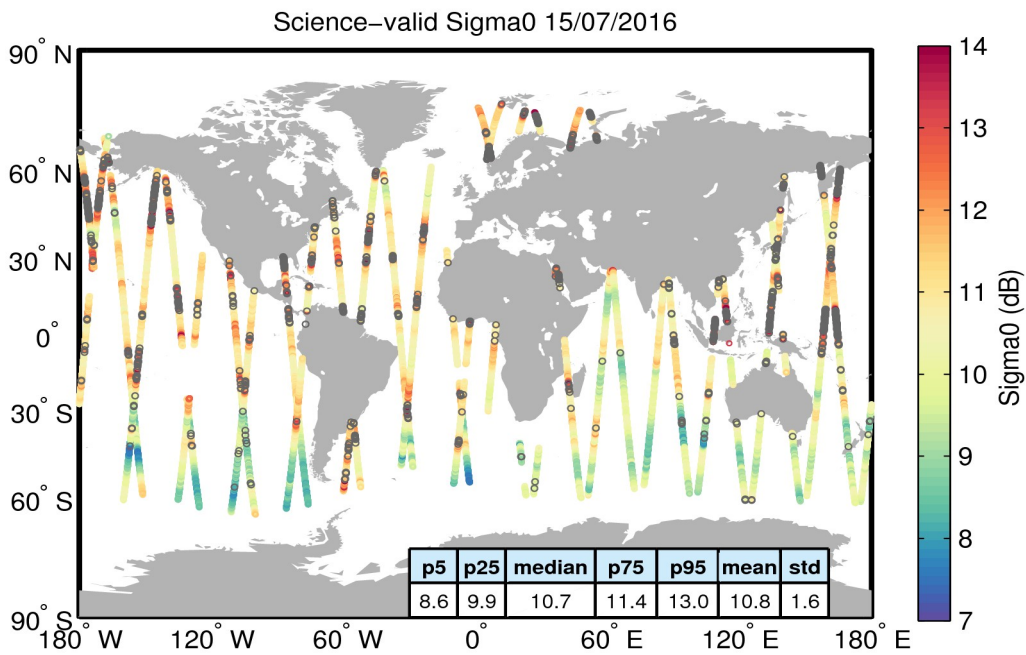
Figure 27. Geographical distribution of science-valid sigma0 data over oceans and lakes for 15/07/2016. The statistical values shown in the table refer to the sigma0 in dB and are calculated over all measurements shown in the figure. Gray circles denote records that have been rejected based on the editing criteria described in Table 4.
