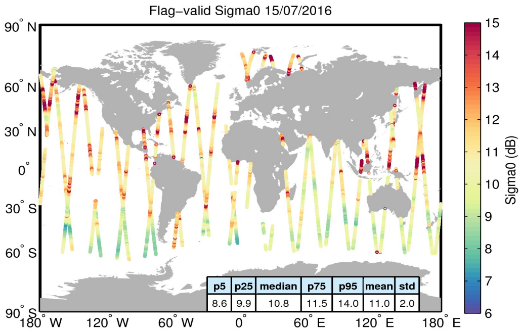
Figure 23. Geographical distribution of flag-valid sigma0 data over oceans and lakes for 15/07/2016. The statistical values shown in the table refer to the sigma0 in dB and are calculated over all measurements shown in the figure.
