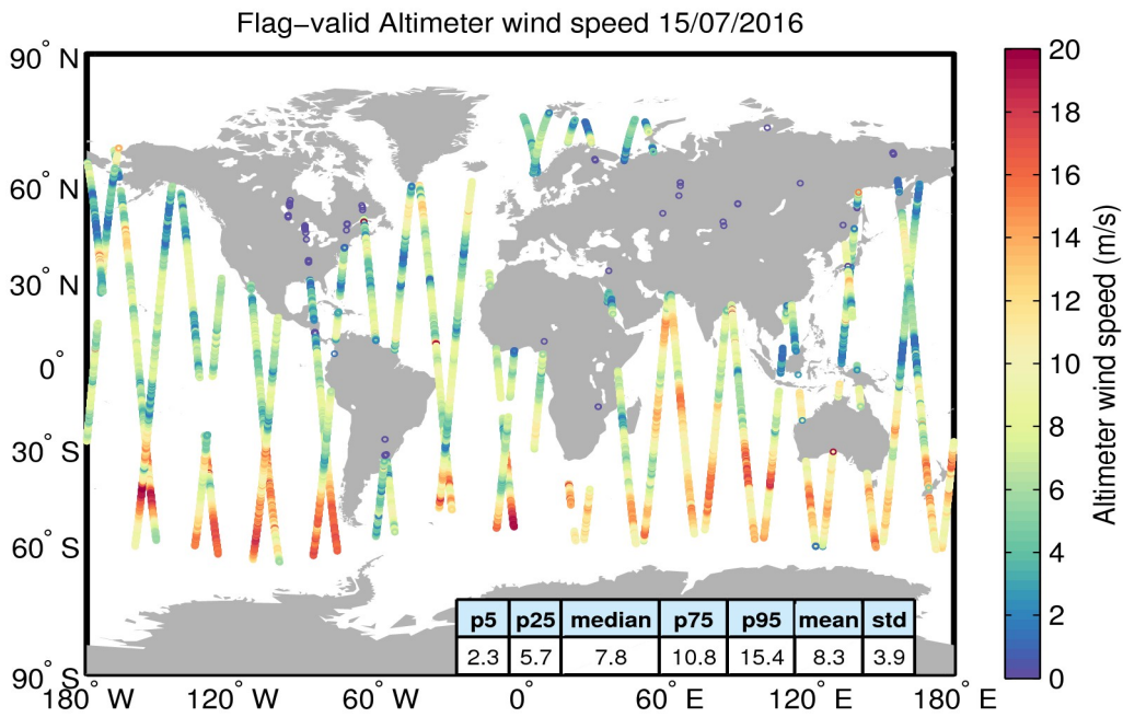
Figure 31. Geographical distribution of flag-valid wind data over oceans and lakes for 15/07/2016. The statistical values shown in the table refer to the wind in m/s and are calculated over all measurements shown in the figure.
