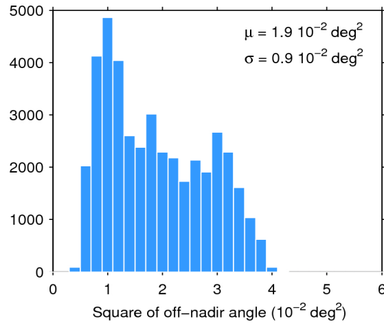
Figure 39. Histogram of flag-valid mispointing over oceans and lakes for 15/07/2016. The mean ( \mu ) and standard deviation ( \sigma ) are also shown. Note that values larger than 6 \cdot 10^{-2} \text{ deg}^2 are excluded from the histogram for the sake of readability but not from the computation of \mu and \sigma .
