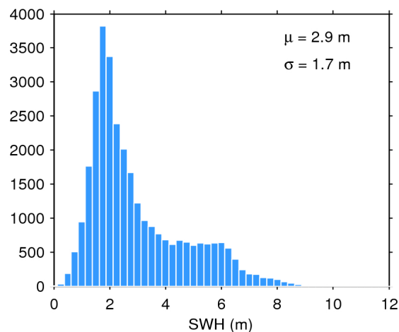
Figure 20. Histogram of science-valid SWH over oceans and lakes for 14/07/2016. The mean ( \mu ) and standard deviation ( \sigma ) are also shown. Note that values larger than 12 m are excluded from the histogram for the sake of readability but not from the computation of \mu and \sigma .
