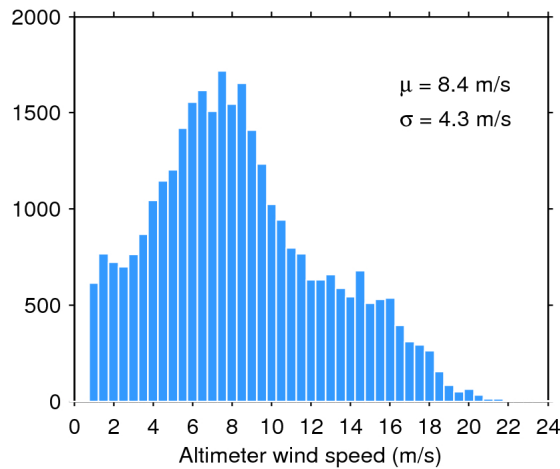
Figure 33. Histogram of flag-valid wind over oceans and lakes for 14/07/2016. The mean ( \mu ) and standard deviation ( \sigma ) are also shown. Note that values larger than 24 m/s are excluded from the histogram for the sake of readability but not from the computation of \mu and \sigma .
