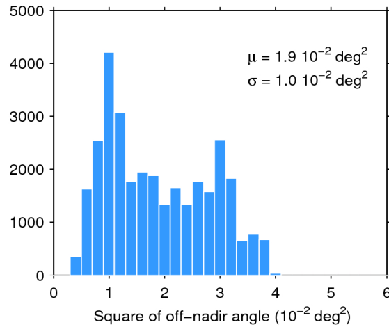
Figure 39. Histogram of flag-valid mispointing over oceans and lakes for 14/07/2016. The mean ( \mu ) and standard deviation ( \sigma ) are also shown. Note that values larger than 6 \cdot 10^{-2} \text{ deg}^2 are excluded from the histogram for the sake of readability but not from the computation of \mu and \sigma .
