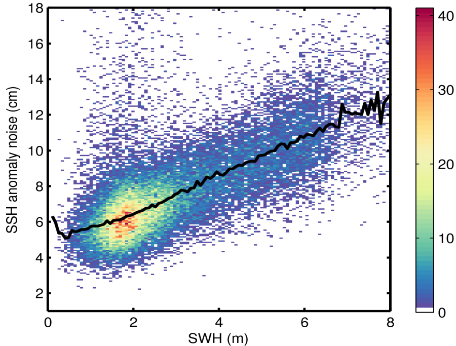
Figure 9. 2D histogram showing flag-valid SSH anomaly noise as a function of SWH for 14/07/2016. The black line denotes the median SSH anomaly noise as a function of SWH.
