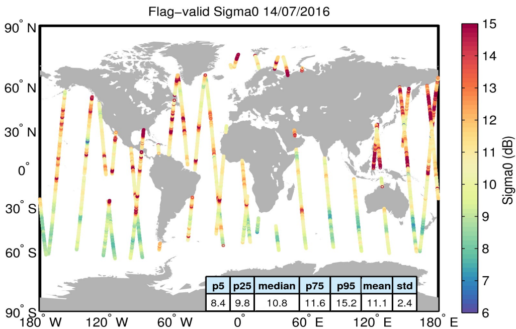
Figure 23. Geographical distribution of flag-valid sigma0 data over oceans and lakes for 14/07/2016. The statistical values shown in the table refer to the sigma0 in dB and are calculated over all measurements shown in the figure.
