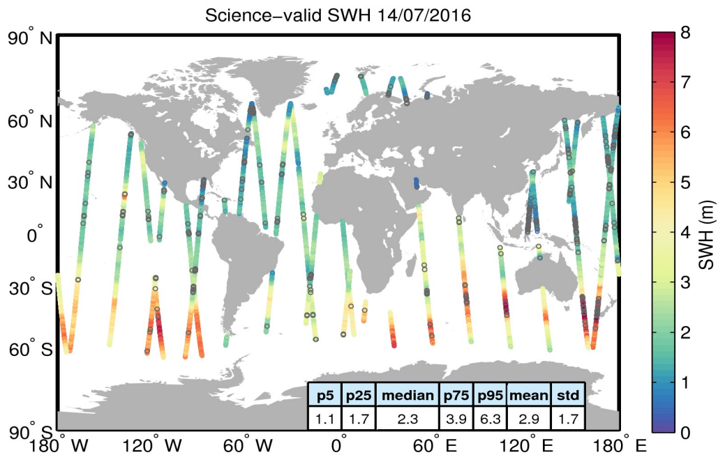
Figure 19. Geographical distribution of science-valid SWH data over oceans and lakes for 14/07/2016. The statistical values shown in the table refer to the SWH in m and are calculated over all measurements shown in the figure. Gray circles denote records that have been rejected based on the editing criteria described in Table 3.
