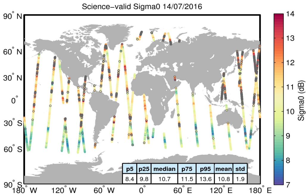
Figure 27. Geographical distribution of science-valid sigma0 data over oceans and lakes for 14/07/2016. The statistical values shown in the table refer to the sigma0 in dB and are calculated over all measurements shown in the figure. Gray circles denote records that have been rejected based on the editing criteria described in Table 4.
