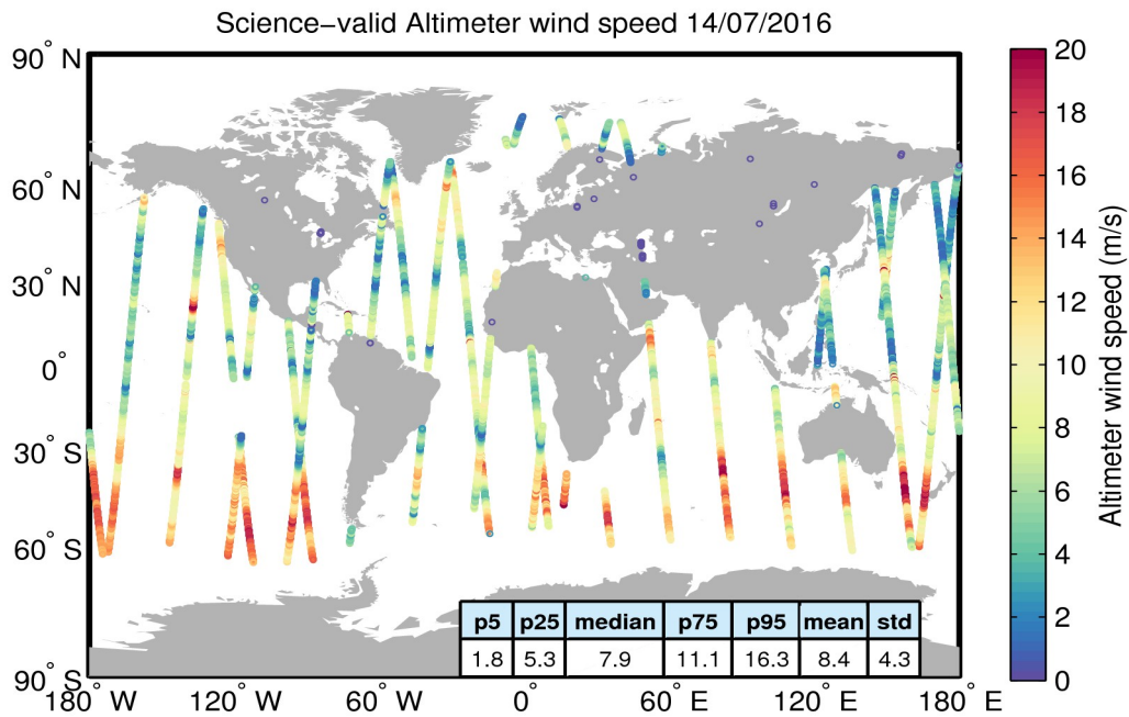
Figure 34. Geographical distribution of science-valid wind data over oceans and lakes for 14/07/2016. The statistical values shown in the table refer to the wind in m/s and are calculated over all measurements shown in the figure. Gray circles denote records that have been rejected based on the editing criteria described in Table 5.
