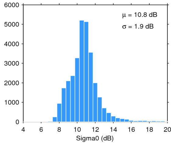
Figure 28. Histogram of science-valid sigma0 over oceans and lakes for 14/07/2016. The mean ( \mu ) and standard deviation ( \sigma ) are also shown. Note that values outside [4 20] dB are excluded from the histogram for the sake of readability but not from the computation of \mu and \sigma .
