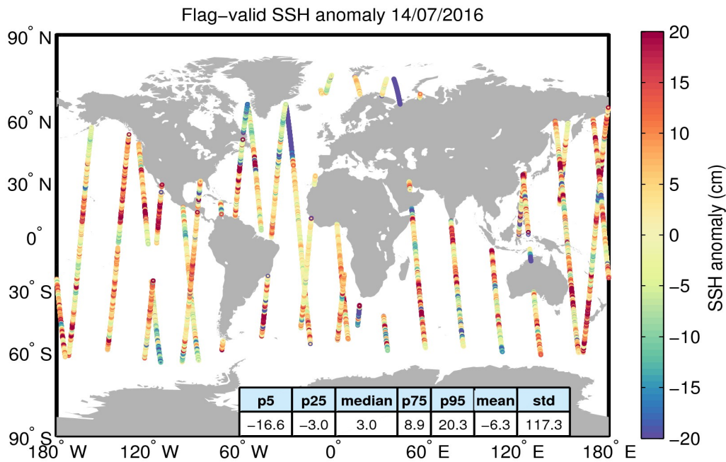
Figure 5. Geographical distribution of flag-valid 1-Hz SSH anomaly data over oceans and lakes for 14/07/2016. The statistical values shown in the table refer to the SSH anomaly in cm and are calculated over all measurements shown in the figure.
