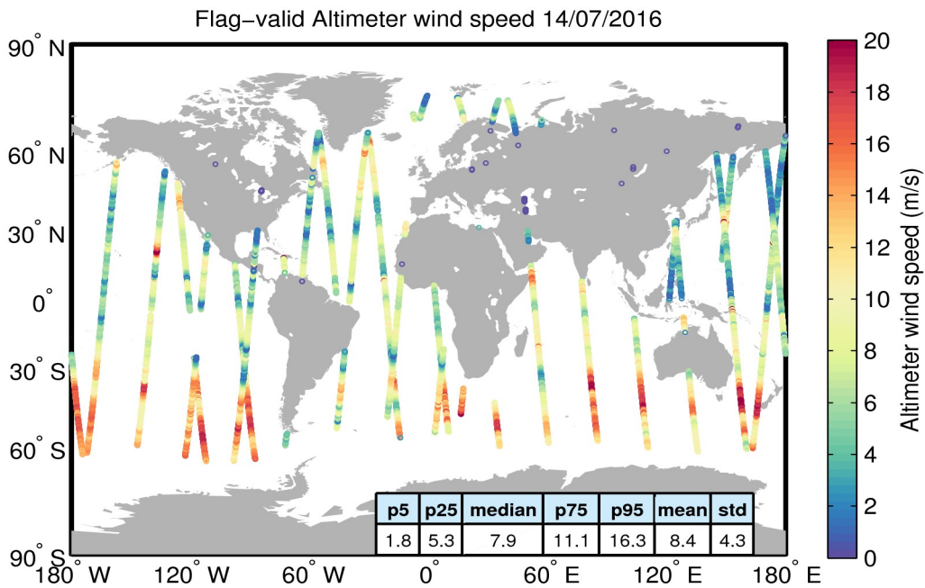
Figure 31. Geographical distribution of flag-valid wind data over oceans and lakes for 14/07/2016. The statistical values shown in the table refer to the wind in m/s and are calculated over all measurements shown in the figure.
