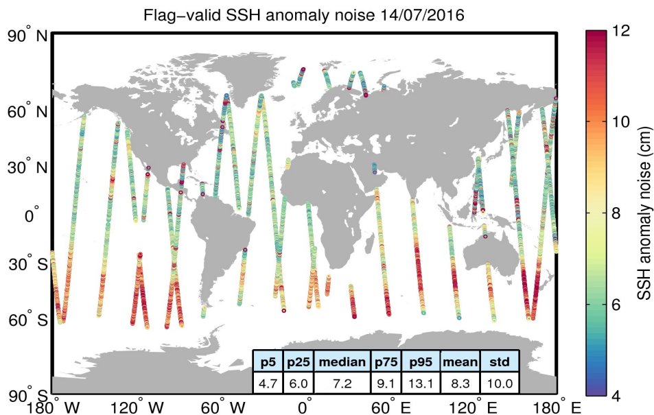
Figure 8. Geographical distribution of flag-valid 20-Hz SSH anomaly measurement noise over oceans and lakes for 14/07/2016. The statistical values shown in the table refer to the SSH anomaly noise and are calculated over all measurements shown in the figure.
