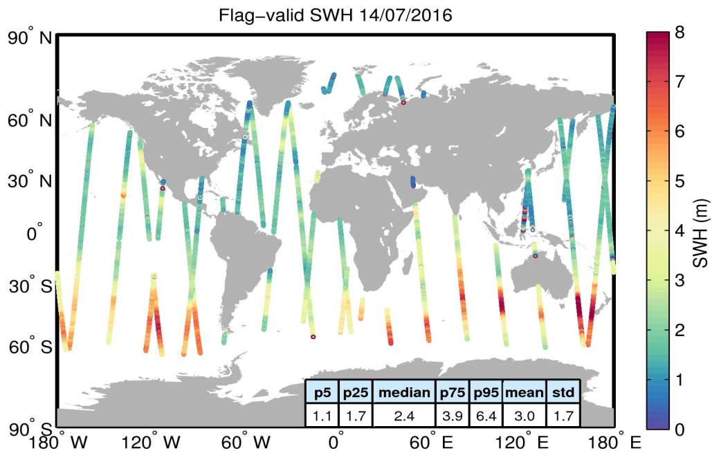
Figure 15. Geographical distribution of flag-valid SWH data over oceans and lakes for 14/07/2016. The statistical values shown in the table refer to the SWH in m and are calculated over all measurements shown in the figure.
