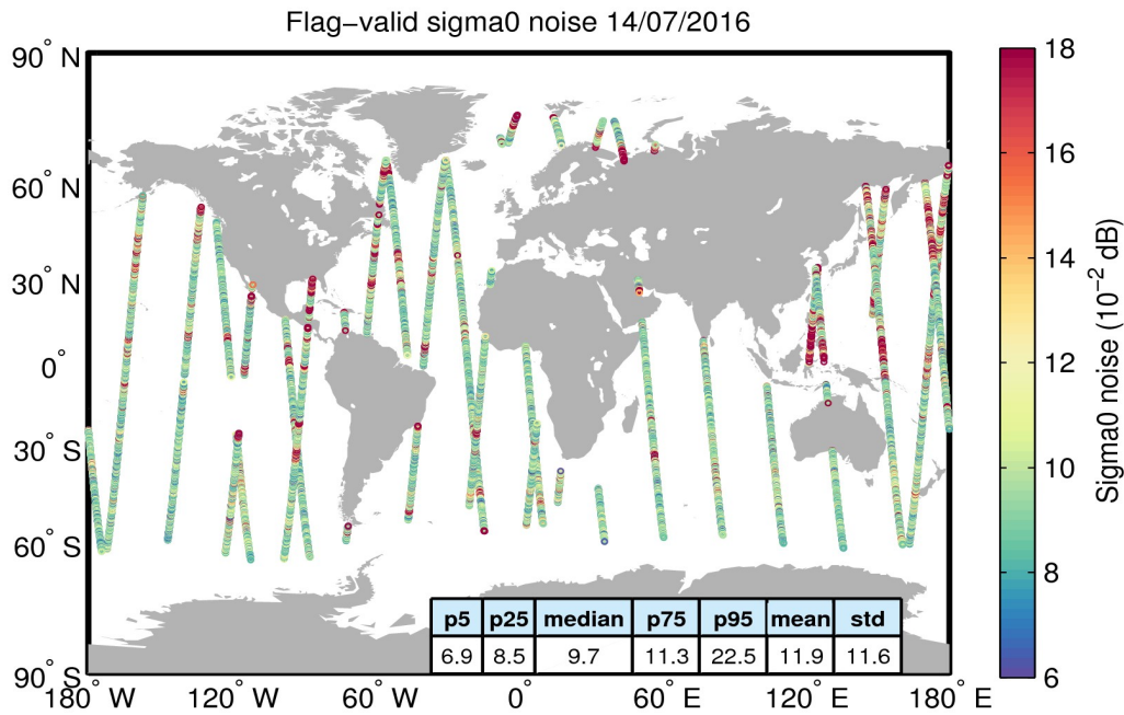
Figure 26. Geographical distribution of flag-valid 20-Hz sigma0 measurement noise over oceans and lakes for 14/07/2016. The statistical values shown in the table refer to the sigma0 noise and are calculated over all measurements shown in the figure.
