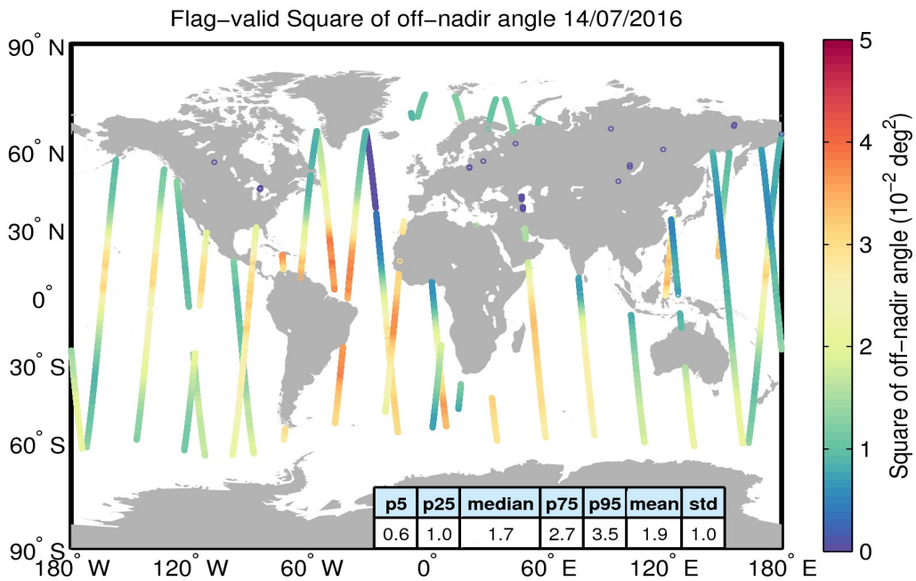
Figure 37. Geographical distribution of flag-valid mispointing data over oceans and lakes for 14/07/2016. The statistical values shown in the table refer to the mispointing in 10^{-2} deg 2 and are calculated over all measurements shown in the figure.
