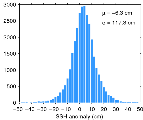
Figure 7. Histogram of flag-valid SSH anomaly over oceans and lakes for 14/07/2016. The mean ( \mu ) and standard deviation ( \sigma ) are also shown. Note that values outside [-50 50] cm are excluded from the histogram for the sake of readability but not from the computation of \mu and \sigma .
