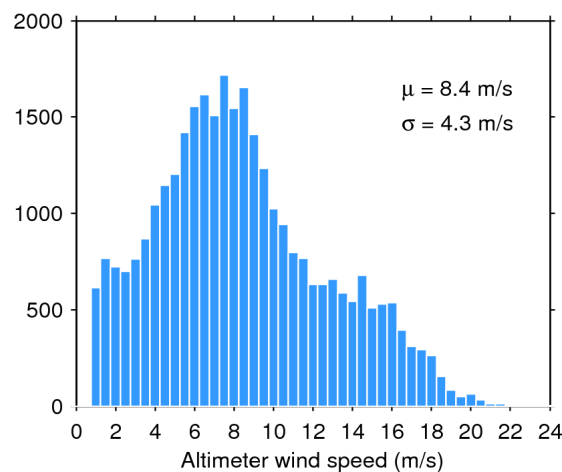
Figure 35. Histogram of science-valid wind over oceans and lakes for 14/07/2016. The mean ( \mu ) and standard deviation ( \sigma ) are also shown. Note that values larger than 24 m/s are excluded from the histogram for the sake of readability but not from the computation of \mu and \sigma .
