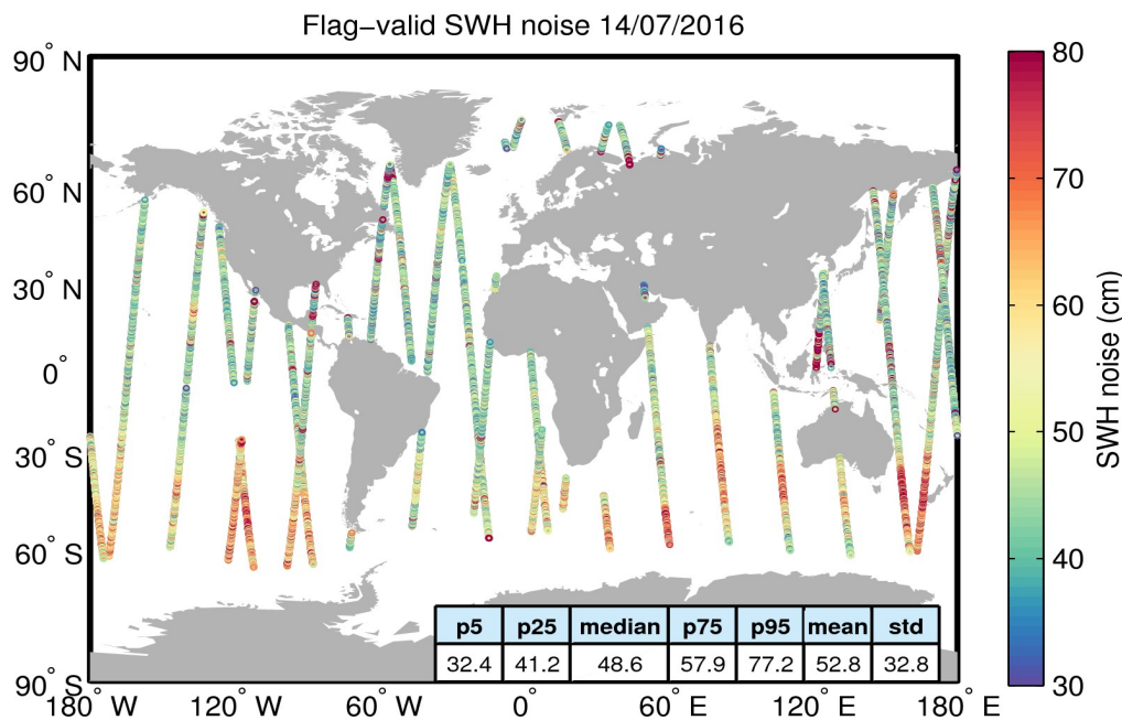
Figure 18. Geographical distribution of flag-valid 20-Hz SWH measurement noise over oceans and lakes for 14/07/2016. The statistical values shown in the table refer to the SWH noise and are calculated over all measurements shown in the figure.
