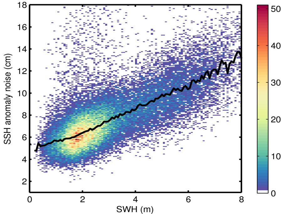
Figure 9. 2D histogram showing flag-valid SSH anomaly noise as a function of SWH for 13/07/2016. The black line denotes the median SSH anomaly noise as a function of SWH.
