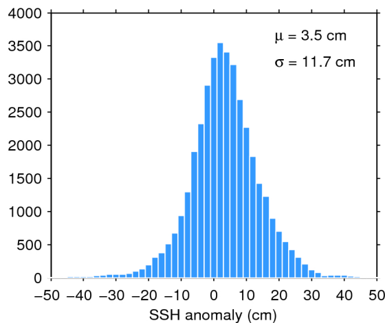
Figure 11. Histogram of science-valid SSH anomaly over oceans and lakes for 13/07/2016. The mean ( \mu ) and standard deviation ( \sigma ) are also shown. Note that values outside [-50 50] cm are excluded from the histogram for the sake of readability but not from the computation of \mu and \sigma .
