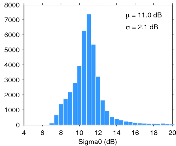
Figure 25. Histogram of flag-valid sigma0 over oceans and lakes for 13/07/2016. The mean ( \mu ) and standard deviation ( \sigma ) are also shown. Note that values outside [4 20] dB are excluded from the histogram for the sake of readability but not from the computation of \mu and \sigma .
