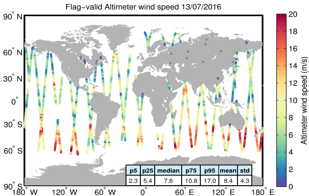
Figure 31. Geographical distribution of flag-valid wind data over oceans and lakes for 13/07/2016. The statistical values shown in the table refer to the wind in m/s and are calculated over all measurements shown in the figure.
