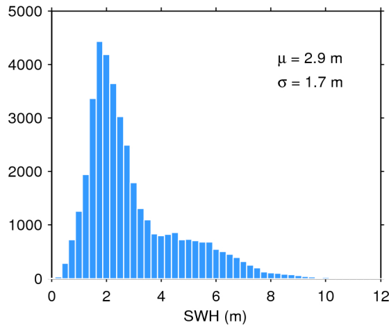
Figure 20. Histogram of science-valid SWH over oceans and lakes for 13/07/2016. The mean ( \mu ) and standard deviation ( \sigma ) are also shown. Note that values larger than 12 m are excluded from the histogram for the sake of readability but not from the computation of \mu and \sigma .
