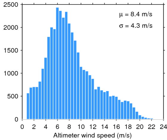
Figure 33. Histogram of flag-valid wind over oceans and lakes for 13/07/2016. The mean ( \mu ) and standard deviation ( \sigma ) are also shown. Note that values larger than 24 m/s are excluded from the histogram for the sake of readability but not from the computation of \mu and \sigma .
