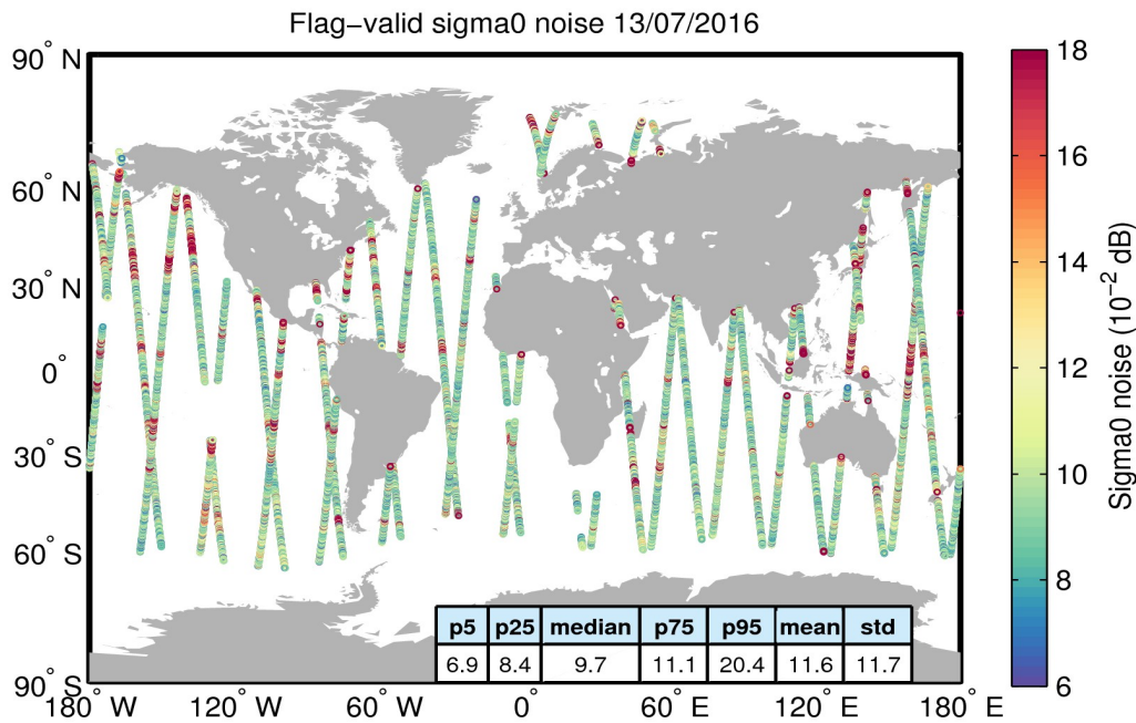
Figure 26. Geographical distribution of flag-valid 20-Hz sigma0 measurement noise over oceans and lakes for 13/07/2016. The statistical values shown in the table refer to the sigma0 noise and are calculated over all measurements shown in the figure.
