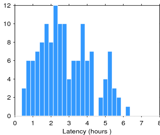
Figure 2. Histogram of the data latency for 13/07/2016. The y-axis denotes the number of files that are made available with a delay of x-hours with respect to the mean time of the records stored in the file.
