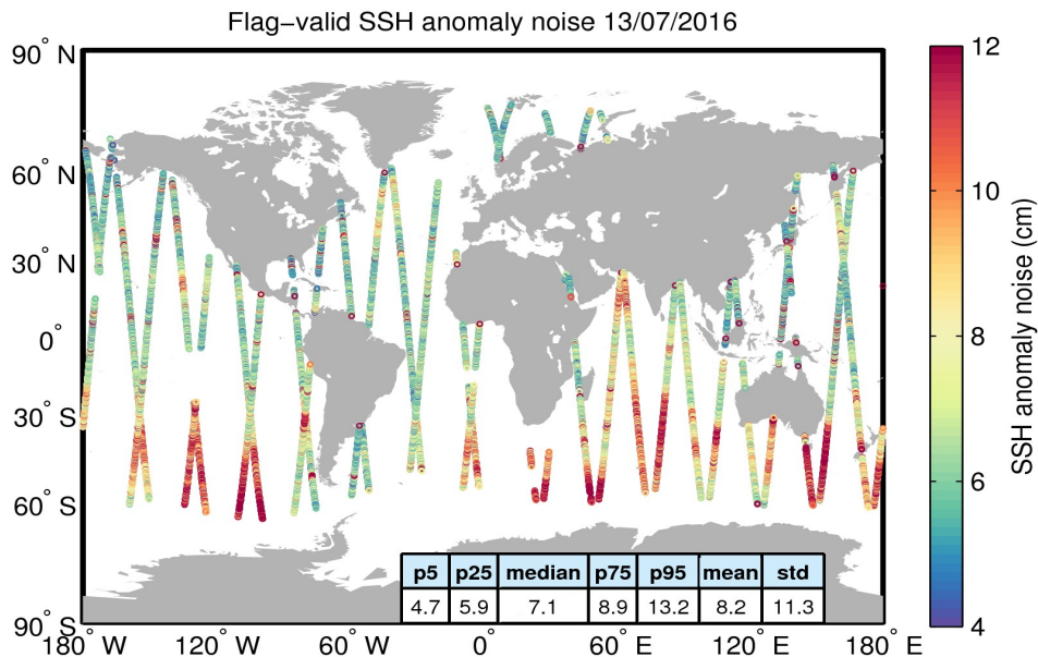
Figure 8. Geographical distribution of flag-valid 20-Hz SSH anomaly measurement noise over oceans and lakes for 13/07/2016. The statistical values shown in the table refer to the SSH anomaly noise and are calculated over all measurements shown in the figure.
