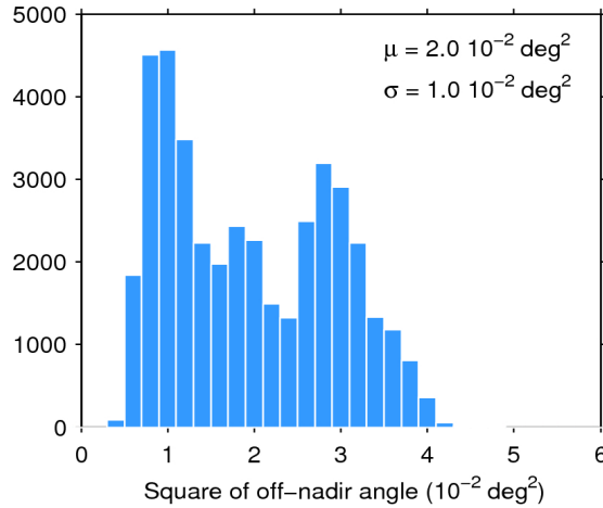
Figure 39. Histogram of flag-valid mispointing over oceans and lakes for 13/07/2016. The mean ( \mu ) and standard deviation ( \sigma ) are also shown. Note that values larger than 6 \cdot 10^{-2} \text{ deg}^2 are excluded from the histogram for the sake of readability but not from the computation of \mu and \sigma .
