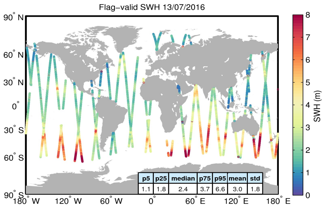
Figure 15. Geographical distribution of flag-valid SWH data over oceans and lakes for 13/07/2016. The statistical values shown in the table refer to the SWH in m and are calculated over all measurements shown in the figure.
