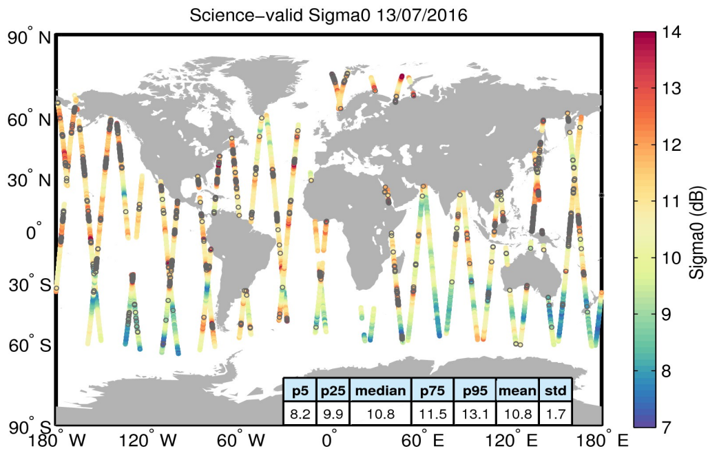
Figure 27. Geographical distribution of science-valid sigma0 data over oceans and lakes for 13/07/2016. The statistical values shown in the table refer to the sigma0 in dB and are calculated over all measurements shown in the figure. Gray circles denote records that have been rejected based on the editing criteria described in Table 4.
