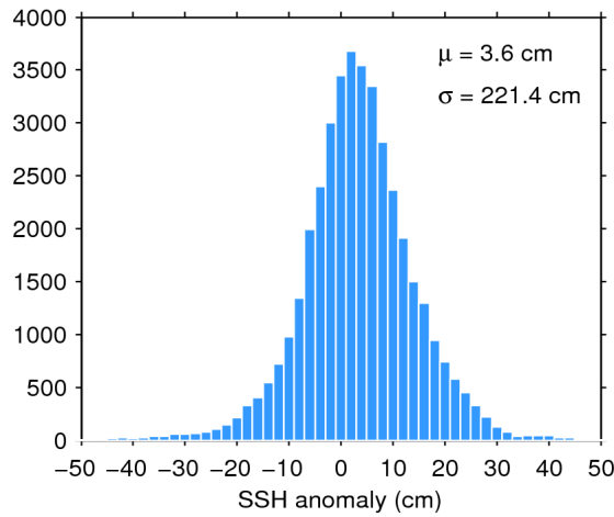
Figure 7. Histogram of flag-valid SSH anomaly over oceans and lakes for 13/07/2016. The mean ( \mu ) and standard deviation ( \sigma ) are also shown. Note that values outside [-50 50] cm are excluded from the histogram for the sake of readability but not from the computation of \mu and \sigma .
