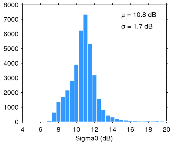
Figure 28. Histogram of science-valid sigma0 over oceans and lakes for 13/07/2016. The mean ( \mu ) and standard deviation ( \sigma ) are also shown. Note that values outside [4 20] dB are excluded from the histogram for the sake of readability but not from the computation of \mu and \sigma .
