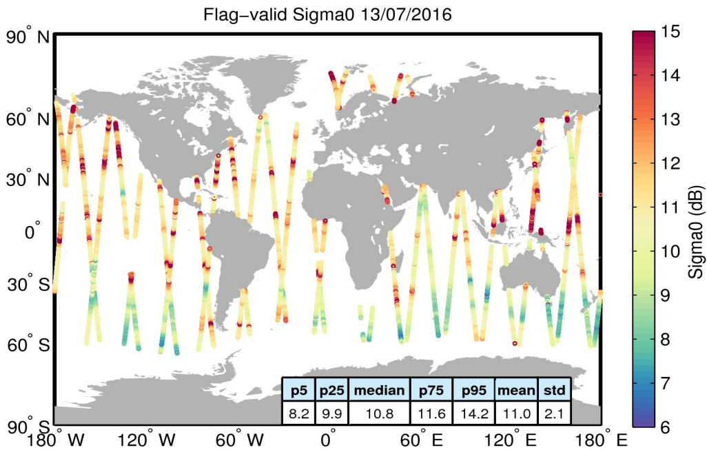
Figure 23. Geographical distribution of flag-valid sigma0 data over oceans and lakes for 13/07/2016. The statistical values shown in the table refer to the sigma0 in dB and are calculated over all measurements shown in the figure.
