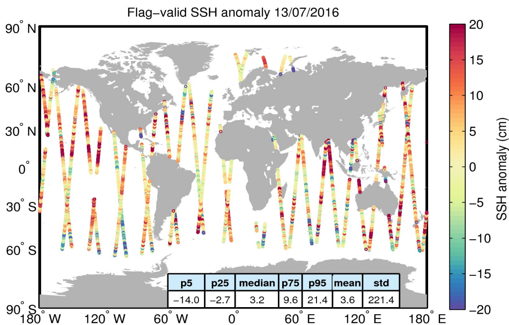
Figure 5. Geographical distribution of flag-valid 1-Hz SSH anomaly data over oceans and lakes for 13/07/2016. The statistical values shown in the table refer to the SSH anomaly in cm and are calculated over all measurements shown in the figure.
