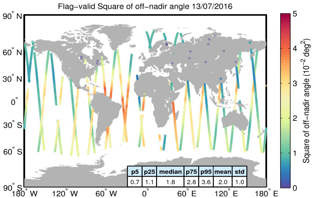
Figure 37. Geographical distribution of flag-valid mispointing data over oceans and lakes for 13/07/2016. The statistical values shown in the table refer to the mispointing in 10^{-2} deg 2 and are calculated over all measurements shown in the figure.
