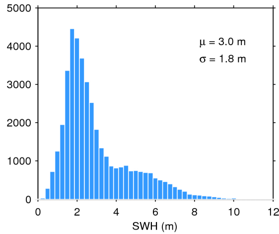
Figure 17. Histogram of flag-valid SWH over oceans and lakes for 13/07/2016. The mean ( \mu ) and standard deviation ( \sigma ) are also shown. Note that values larger than 12 m are excluded from the histogram for the sake of readability but not from the computation of \mu and \sigma .
