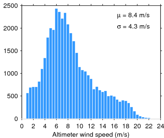
Figure 35. Histogram of science-valid wind over oceans and lakes for 13/07/2016. The mean ( \mu ) and standard deviation ( \sigma ) are also shown. Note that values larger than 24 m/s are excluded from the histogram for the sake of readability but not from the computation of \mu and \sigma .
