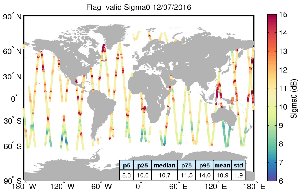
Figure 23. Geographical distribution of flag-valid sigma0 data over oceans and lakes for 12/07/2016. The statistical values shown in the table refer to the sigma0 in dB and are calculated over all measurements shown in the figure.
