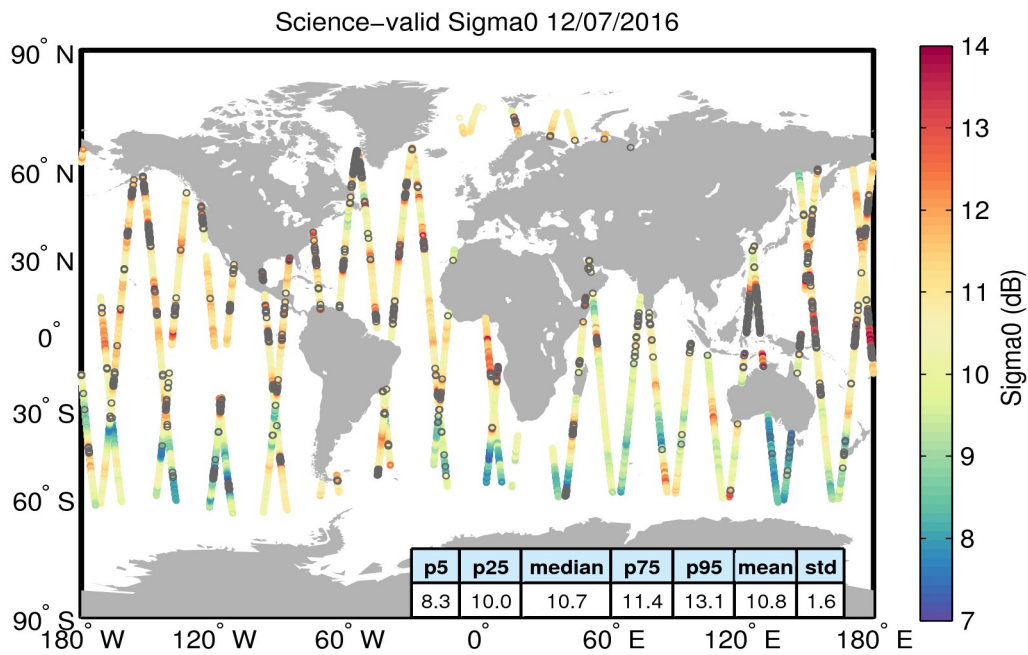
Figure 27. Geographical distribution of science-valid sigma0 data over oceans and lakes for 12/07/2016. The statistical values shown in the table refer to the sigma0 in dB and are calculated over all measurements shown in the figure. Gray circles denote records that have been rejected based on the editing criteria described in Table 4.
