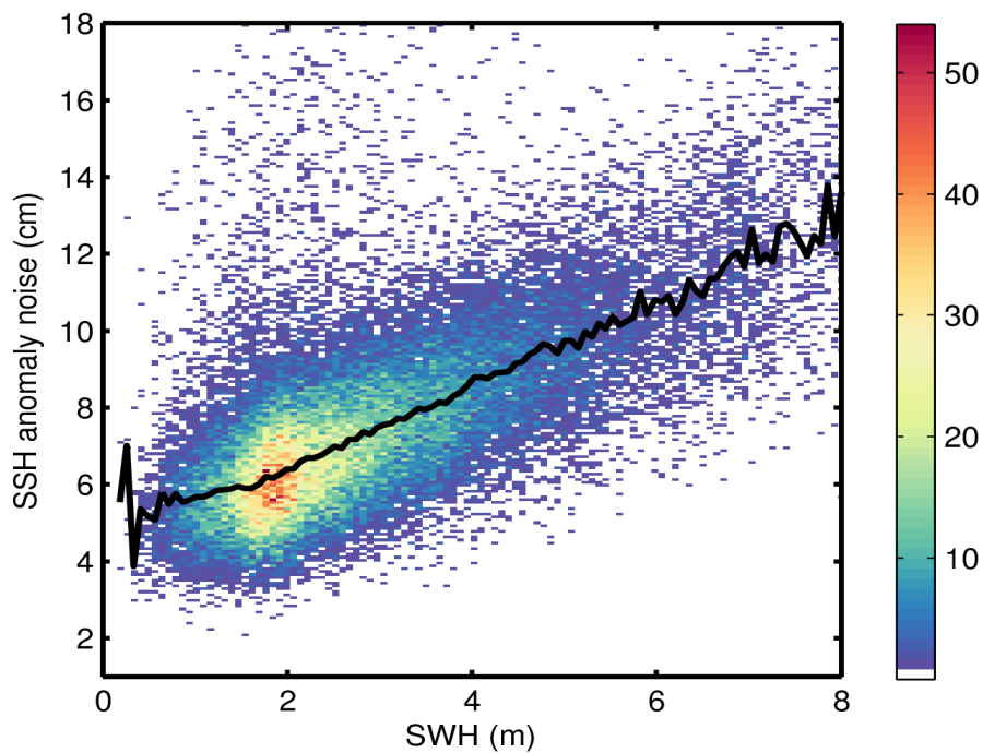
Figure 9. 2D histogram showing flag-valid SSH anomaly noise as a function of SWH for 12/07/2016. The black line denotes the median SSH anomaly noise as a function of SWH.
