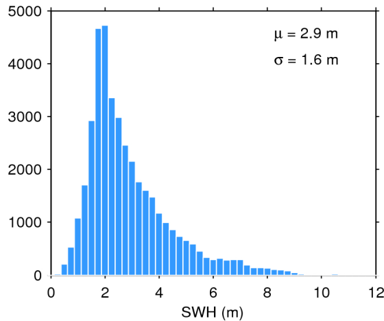
Figure 20. Histogram of science-valid SWH over oceans and lakes for 12/07/2016. The mean ( \mu ) and standard deviation ( \sigma ) are also shown. Note that values larger than 12 m are excluded from the histogram for the sake of readability but not from the computation of \mu and \sigma .
