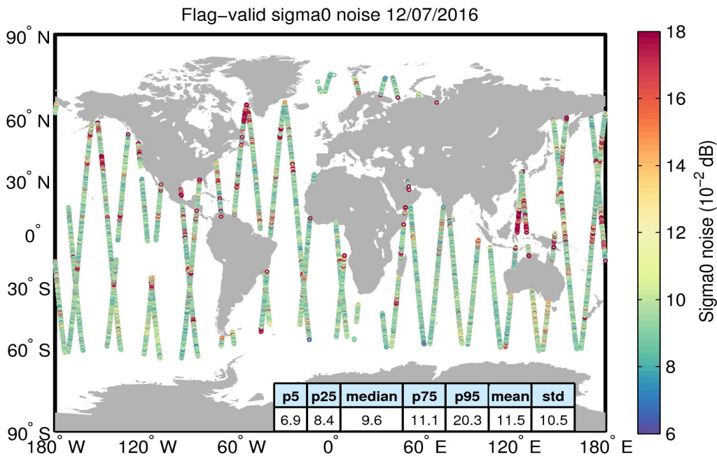
Figure 26. Geographical distribution of flag-valid 20-Hz sigma0 measurement noise over oceans and lakes for 12/07/2016. The statistical values shown in the table refer to the sigma0 noise and are calculated over all measurements shown in the figure.
