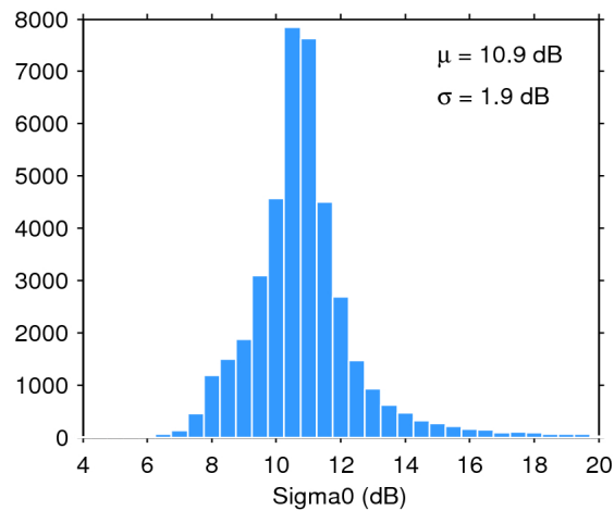
Figure 25. Histogram of flag-valid sigma0 over oceans and lakes for 12/07/2016. The mean ( \mu ) and standard deviation ( \sigma ) are also shown. Note that values outside [4 20] dB are excluded from the histogram for the sake of readability but not from the computation of \mu and \sigma .
