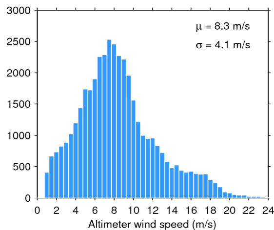
Figure 35. Histogram of science-valid wind over oceans and lakes for 12/07/2016. The mean ( \mu ) and standard deviation ( \sigma ) are also shown. Note that values larger than 24 m/s are excluded from the histogram for the sake of readability but not from the computation of \mu and \sigma .
