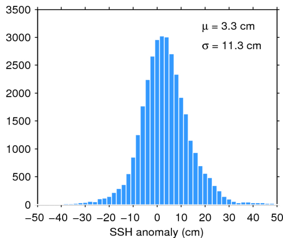
Figure 11. Histogram of science-valid SSH anomaly over oceans and lakes for 12/07/2016. The mean ( \mu ) and standard deviation ( \sigma ) are also shown. Note that values outside [-50 50] cm are excluded from the histogram for the sake of readability but not from the computation of \mu and \sigma .
