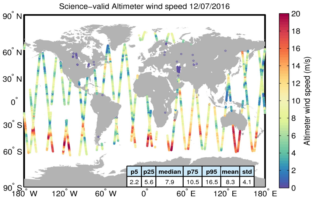
Figure 34. Geographical distribution of science-valid wind data over oceans and lakes for 12/07/2016. The statistical values shown in the table refer to the wind in m/s and are calculated over all measurements shown in the figure. Gray circles denote records that have been rejected based on the editing criteria described in Table 5.
