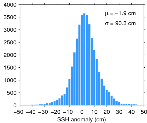
Figure 7. Histogram of flag-valid SSH anomaly over oceans and lakes for 12/07/2016. The mean ( \mu ) and standard deviation ( \sigma ) are also shown. Note that values outside [-50 50] cm are excluded from the histogram for the sake of readability but not from the computation of \mu and \sigma .
