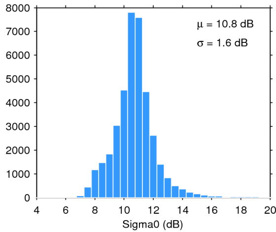
Figure 28. Histogram of science-valid sigma0 over oceans and lakes for 12/07/2016. The mean ( \mu ) and standard deviation ( \sigma ) are also shown. Note that values outside [4 20] dB are excluded from the histogram for the sake of readability but not from the computation of \mu and \sigma .
