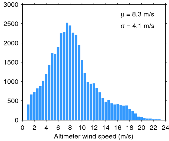
Figure 33. Histogram of flag-valid wind over oceans and lakes for 12/07/2016. The mean ( \mu ) and standard deviation ( \sigma ) are also shown. Note that values larger than 24 m/s are excluded from the histogram for the sake of readability but not from the computation of \mu and \sigma .
