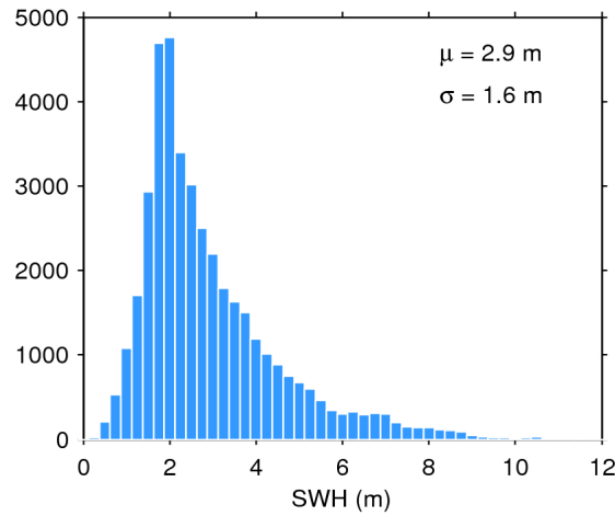
Figure 17. Histogram of flag-valid SWH over oceans and lakes for 12/07/2016. The mean ( \mu ) and standard deviation ( \sigma ) are also shown. Note that values larger than 12 m are excluded from the histogram for the sake of readability but not from the computation of \mu and \sigma .
