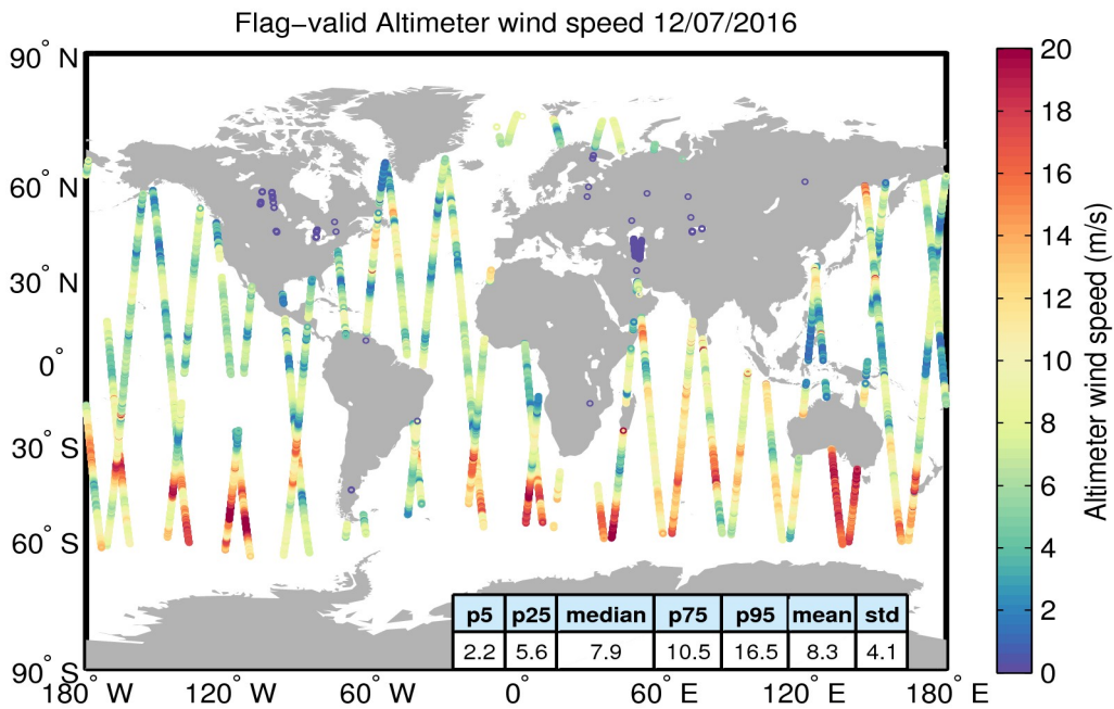
Figure 31. Geographical distribution of flag-valid wind data over oceans and lakes for 12/07/2016. The statistical values shown in the table refer to the wind in m/s and are calculated over all measurements shown in the figure.
