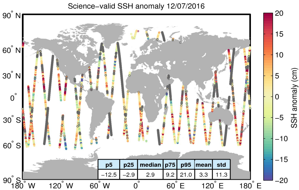
Figure 10. Geographical distribution of science-valid SSH anomaly data over oceans and lakes for 12/07/2016. The statistical values shown in the table refer to the SSH anomaly in cm and are calculated over all measurements shown in the figure. Gray circles denote records that have been rejected based on the editing criteria described in Table 2.
