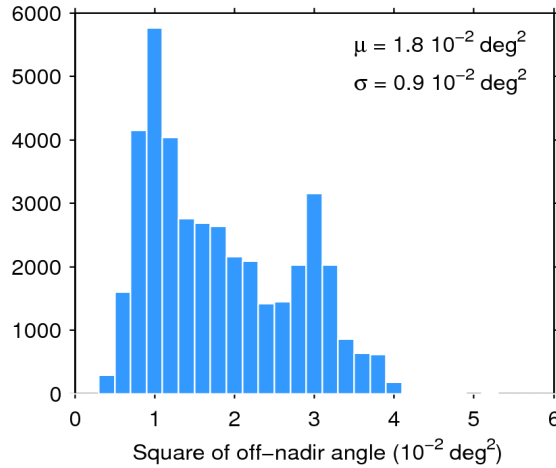
Figure 39. Histogram of flag-valid mispointing over oceans and lakes for 12/07/2016. The mean ( \mu ) and standard deviation ( \sigma ) are also shown. Note that values larger than 6 \cdot 10^{-2} \text{ deg}^2 are excluded from the histogram for the sake of readability but not from the computation of \mu and \sigma .
