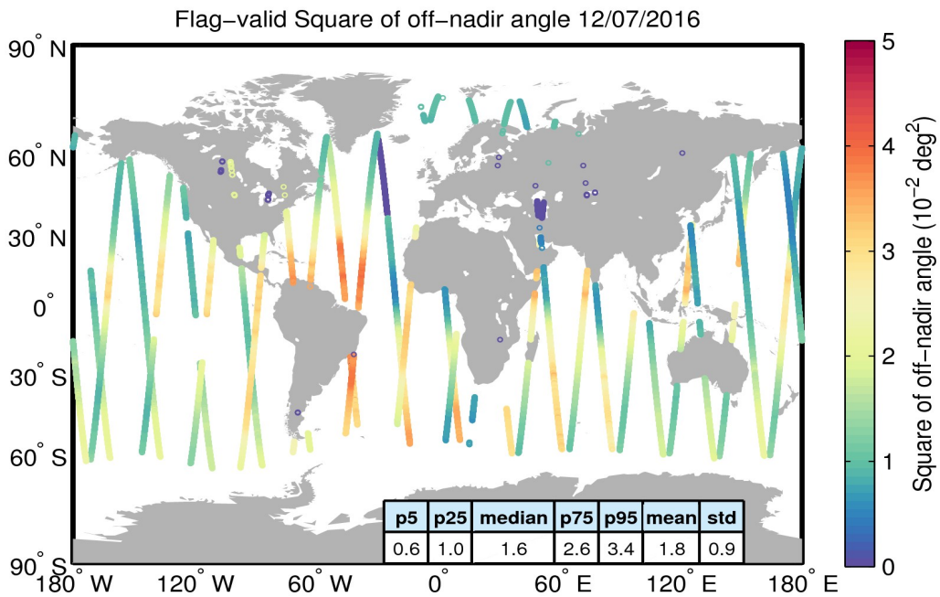
Figure 37. Geographical distribution of flag-valid mispointing data over oceans and lakes for 12/07/2016. The statistical values shown in the table refer to the mispointing in 10^{-2} deg 2 and are calculated over all measurements shown in the figure.
