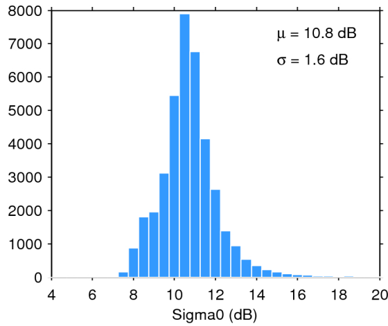
Figure 28. Histogram of science-valid sigma0 over oceans and lakes for 10/07/2016. The mean ( \mu ) and standard deviation ( \sigma ) are also shown. Note that values outside [4 20] dB are excluded from the histogram for the sake of readability but not from the computation of \mu and \sigma .
