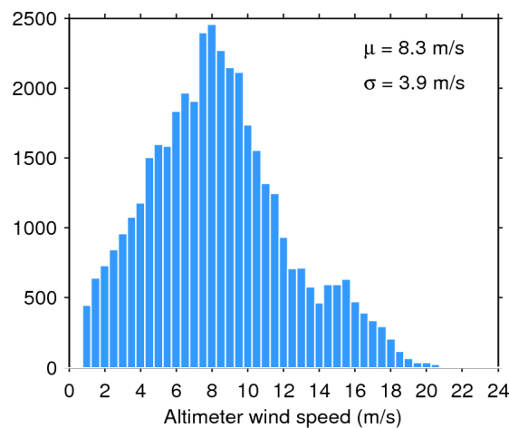
Figure 35. Histogram of science-valid wind over oceans and lakes for 10/07/2016. The mean ( \mu ) and standard deviation ( \sigma ) are also shown. Note that values larger than 24 m/s are excluded from the histogram for the sake of readability but not from the computation of \mu and \sigma .
