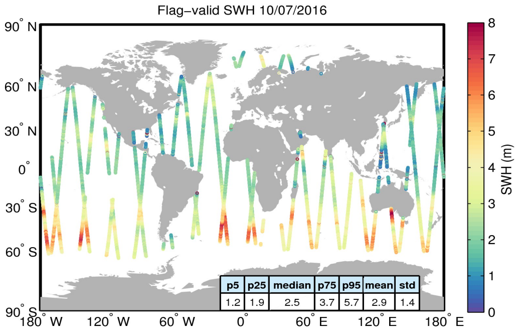
Figure 15. Geographical distribution of flag-valid SWH data over oceans and lakes for 10/07/2016. The statistical values shown in the table refer to the SWH in m and are calculated over all measurements shown in the figure.
