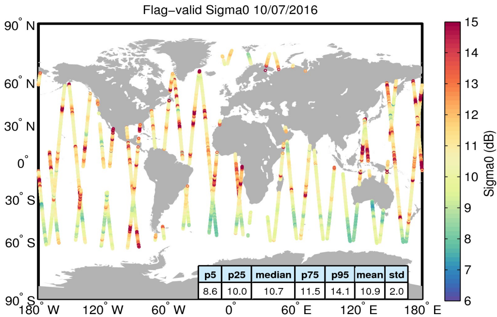
Figure 23. Geographical distribution of flag-valid sigma0 data over oceans and lakes for 10/07/2016. The statistical values shown in the table refer to the sigma0 in dB and are calculated over all measurements shown in the figure.
