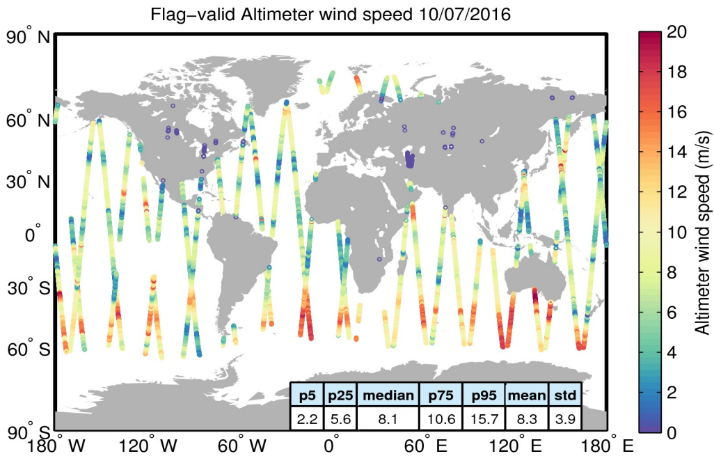
Figure 31. Geographical distribution of flag-valid wind data over oceans and lakes for 10/07/2016. The statistical values shown in the table refer to the wind in m/s and are calculated over all measurements shown in the figure.
