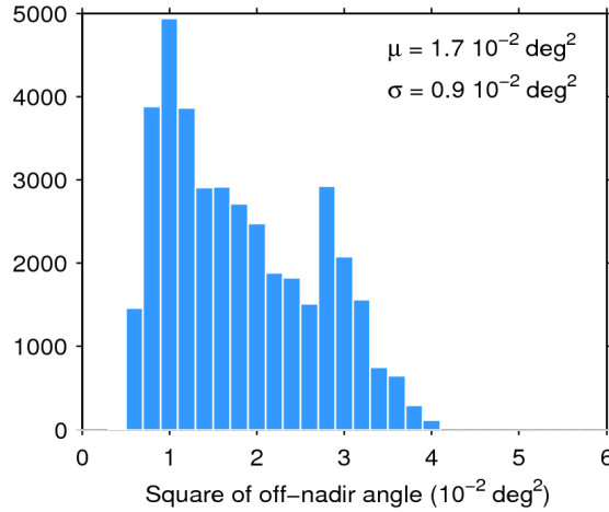
Figure 39. Histogram of flag-valid mispointing over oceans and lakes for 10/07/2016. The mean ( \mu ) and standard deviation ( \sigma ) are also shown. Note that values larger than 6 \cdot 10^{-2} \text{ deg}^2 are excluded from the histogram for the sake of readability but not from the computation of \mu and \sigma .
