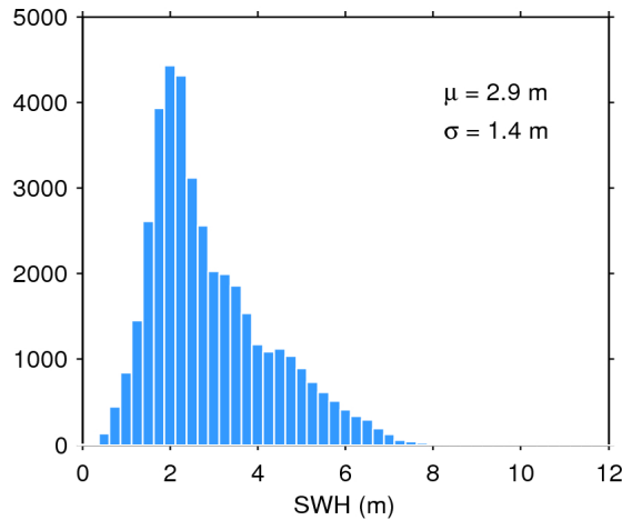
Figure 20. Histogram of science-valid SWH over oceans and lakes for 10/07/2016. The mean ( \mu ) and standard deviation ( \sigma ) are also shown. Note that values larger than 12 m are excluded from the histogram for the sake of readability but not from the computation of \mu and \sigma .
