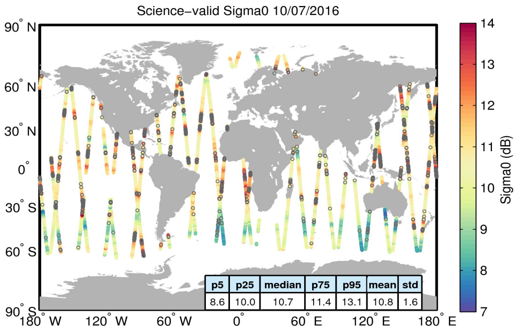
Figure 27. Geographical distribution of science-valid sigma0 data over oceans and lakes for 10/07/2016. The statistical values shown in the table refer to the sigma0 in dB and are calculated over all measurements shown in the figure. Gray circles denote records that have been rejected based on the editing criteria described in Table 4.
