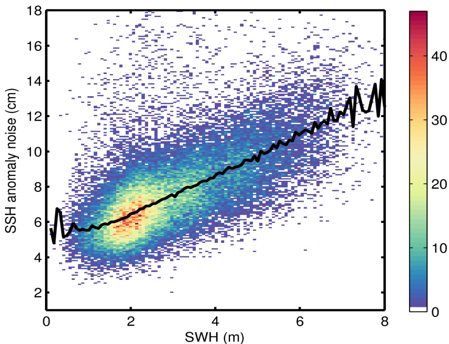
Figure 9. 2D histogram showing flag-valid SSH anomaly noise as a function of SWH for 10/07/2016. The black line denotes the median SSH anomaly noise as a function of SWH.
