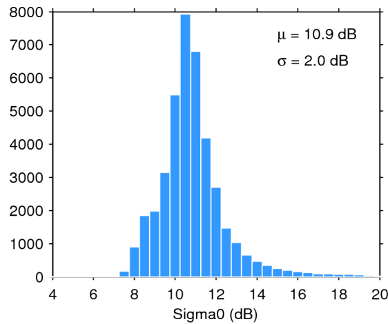
Figure 25. Histogram of flag-valid sigma0 over oceans and lakes for 10/07/2016. The mean ( \mu ) and standard deviation ( \sigma ) are also shown. Note that values outside [4 20] dB are excluded from the histogram for the sake of readability but not from the computation of \mu and \sigma .
