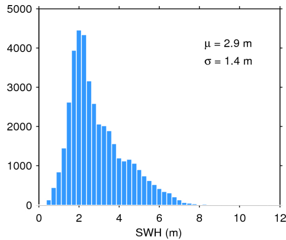
Figure 17. Histogram of flag-valid SWH over oceans and lakes for 10/07/2016. The mean ( \mu ) and standard deviation ( \sigma ) are also shown. Note that values larger than 12 m are excluded from the histogram for the sake of readability but not from the computation of \mu and \sigma .
