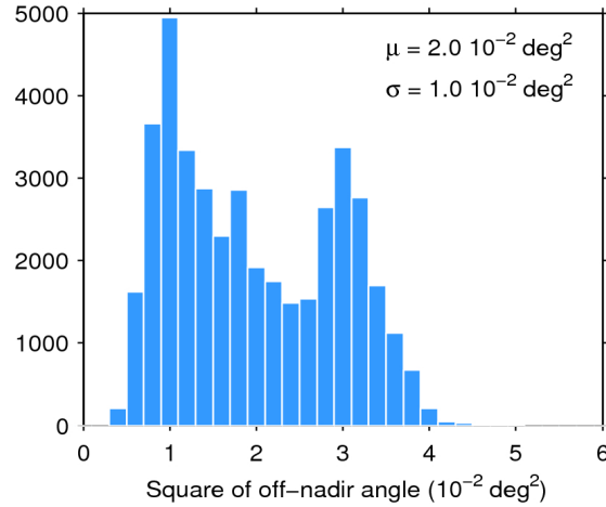
Figure 39. Histogram of flag-valid mispointing over oceans and lakes for 09/07/2016. The mean ( \mu ) and standard deviation ( \sigma ) are also shown. Note that values larger than 6 \cdot 10^{-2} \text{ deg}^2 are excluded from the histogram for the sake of readability but not from the computation of \mu and \sigma .
