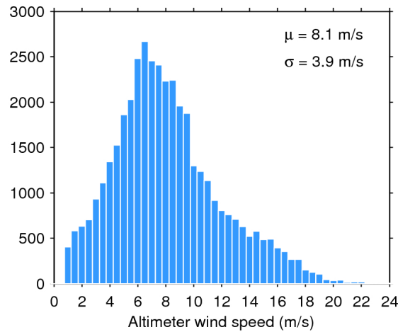
Figure 33. Histogram of flag-valid wind over oceans and lakes for 09/07/2016. The mean ( \mu ) and standard deviation ( \sigma ) are also shown. Note that values larger than 24 m/s are excluded from the histogram for the sake of readability but not from the computation of \mu and \sigma .
