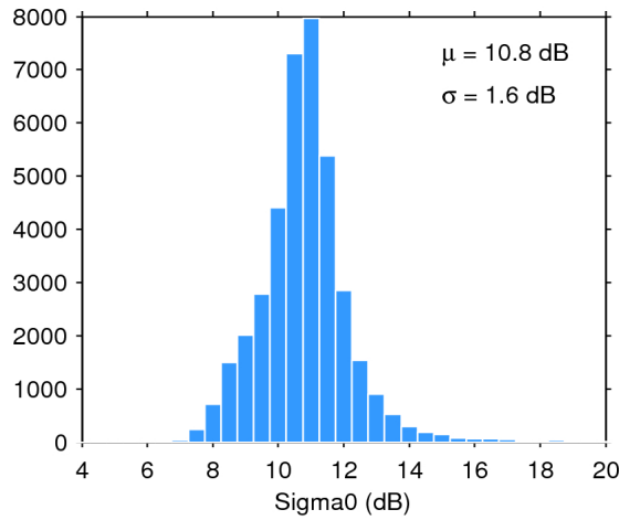
Figure 28. Histogram of science-valid sigma0 over oceans and lakes for 09/07/2016. The mean ( \mu ) and standard deviation ( \sigma ) are also shown. Note that values outside [4 20] dB are excluded from the histogram for the sake of readability but not from the computation of \mu and \sigma .
