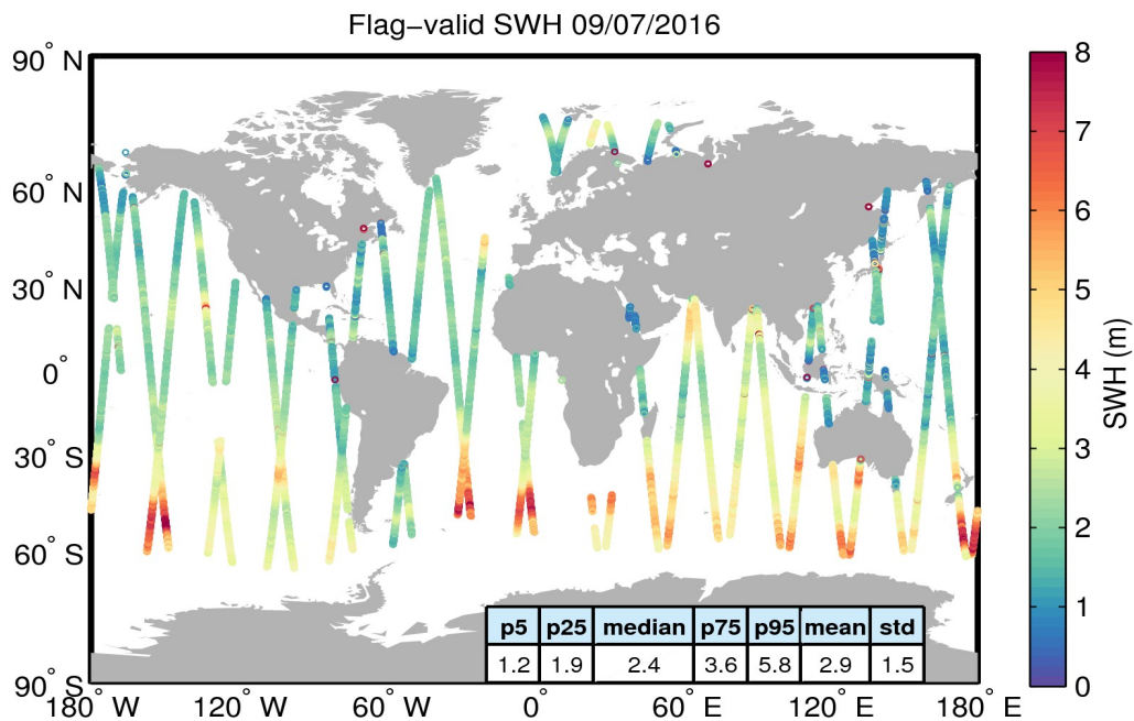
Figure 15. Geographical distribution of flag-valid SWH data over oceans and lakes for 09/07/2016. The statistical values shown in the table refer to the SWH in m and are calculated over all measurements shown in the figure.
