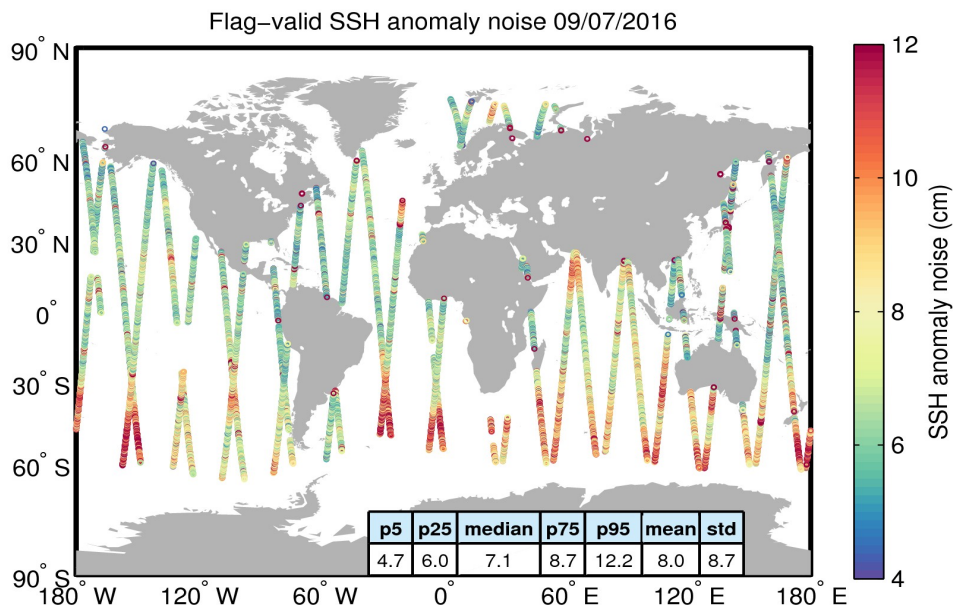
Figure 8. Geographical distribution of flag-valid 20-Hz SSH anomaly measurement noise over oceans and lakes for 09/07/2016. The statistical values shown in the table refer to the SSH anomaly noise and are calculated over all measurements shown in the figure.
