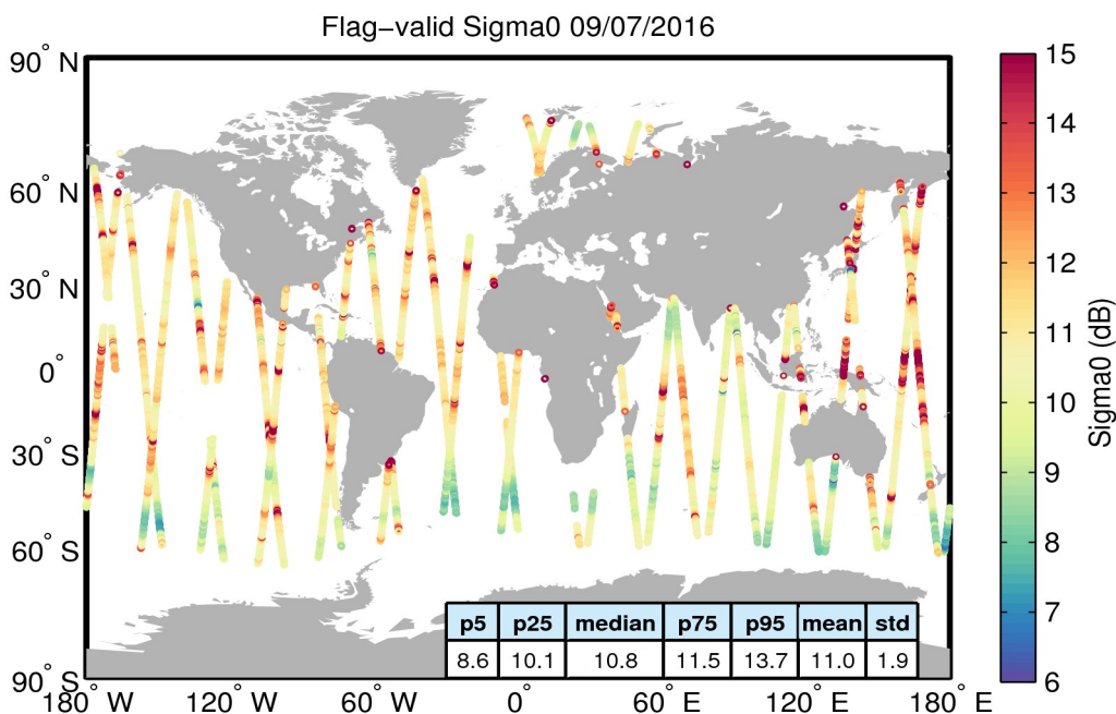
Figure 23. Geographical distribution of flag-valid sigma0 data over oceans and lakes for 09/07/2016. The statistical values shown in the table refer to the sigma0 in dB and are calculated over all measurements shown in the figure.
