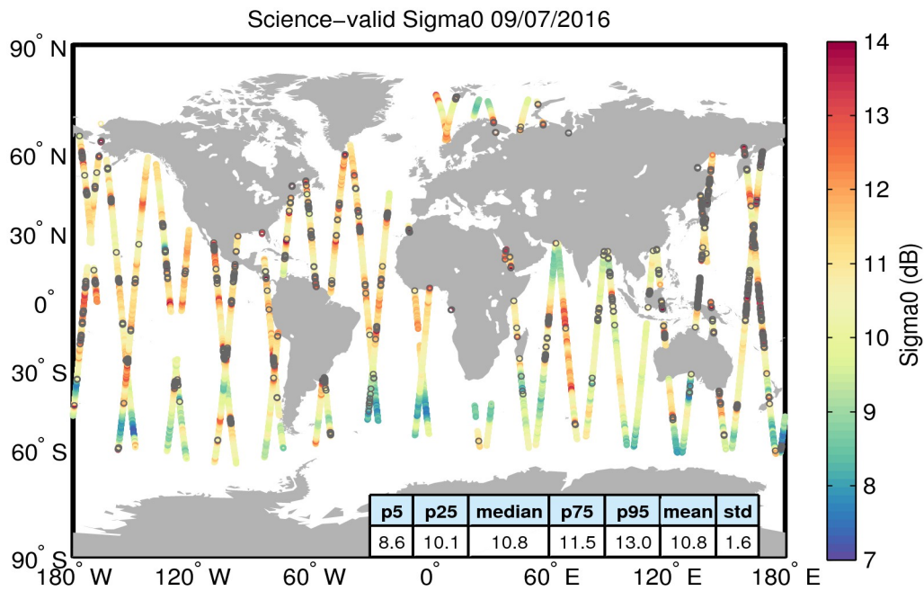
Figure 27. Geographical distribution of science-valid sigma0 data over oceans and lakes for 09/07/2016. The statistical values shown in the table refer to the sigma0 in dB and are calculated over all measurements shown in the figure. Gray circles denote records that have been rejected based on the editing criteria described in Table 4.
