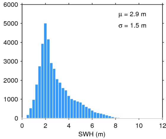
Figure 17. Histogram of flag-valid SWH over oceans and lakes for 09/07/2016. The mean ( \mu ) and standard deviation ( \sigma ) are also shown. Note that values larger than 12 m are excluded from the histogram for the sake of readability but not from the computation of \mu and \sigma .
