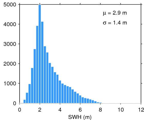
Figure 20. Histogram of science-valid SWH over oceans and lakes for 09/07/2016. The mean ( \mu ) and standard deviation ( \sigma ) are also shown. Note that values larger than 12 m are excluded from the histogram for the sake of readability but not from the computation of \mu and \sigma .
