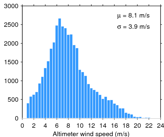
Figure 35. Histogram of science-valid wind over oceans and lakes for 09/07/2016. The mean ( \mu ) and standard deviation ( \sigma ) are also shown. Note that values larger than 24 m/s are excluded from the histogram for the sake of readability but not from the computation of \mu and \sigma .
