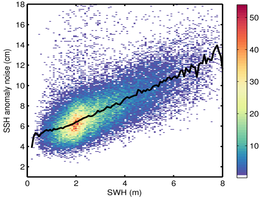
Figure 9. 2D histogram showing flag-valid SSH anomaly noise as a function of SWH for 09/07/2016. The black line denotes the median SSH anomaly noise as a function of SWH.
