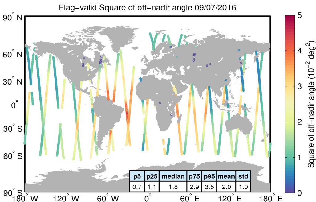
Figure 37. Geographical distribution of flag-valid mispointing data over oceans and lakes for 09/07/2016. The statistical values shown in the table refer to the mispointing in 10^{-2} deg 2 and are calculated over all measurements shown in the figure.
