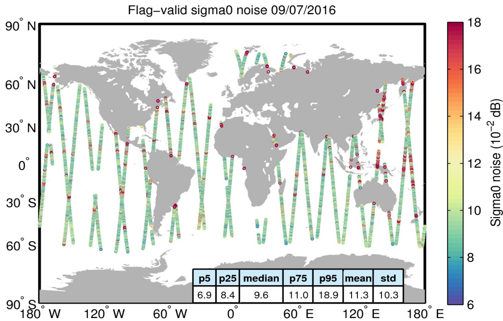
Figure 26. Geographical distribution of flag-valid 20-Hz sigma0 measurement noise over oceans and lakes for 09/07/2016. The statistical values shown in the table refer to the sigma0 noise and are calculated over all measurements shown in the figure.
