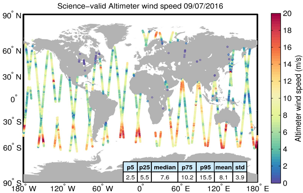
Figure 34. Geographical distribution of science-valid wind data over oceans and lakes for 09/07/2016. The statistical values shown in the table refer to the wind in m/s and are calculated over all measurements shown in the figure. Gray circles denote records that have been rejected based on the editing criteria described in Table 5.
