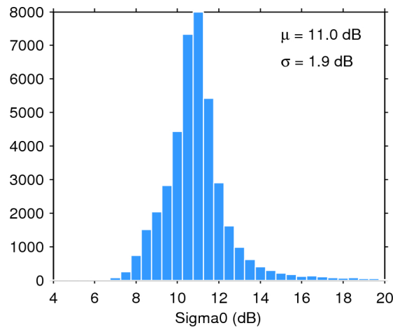
Figure 25. Histogram of flag-valid sigma0 over oceans and lakes for 09/07/2016. The mean ( \mu ) and standard deviation ( \sigma ) are also shown. Note that values outside [4 20] dB are excluded from the histogram for the sake of readability but not from the computation of \mu and \sigma .
