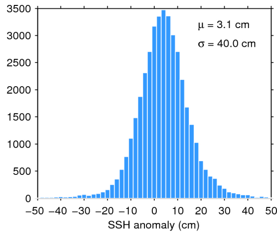
Figure 7. Histogram of flag-valid SSH anomaly over oceans and lakes for 09/07/2016. The mean ( \mu ) and standard deviation ( \sigma ) are also shown. Note that values outside [-50 50] cm are excluded from the histogram for the sake of readability but not from the computation of \mu and \sigma .
