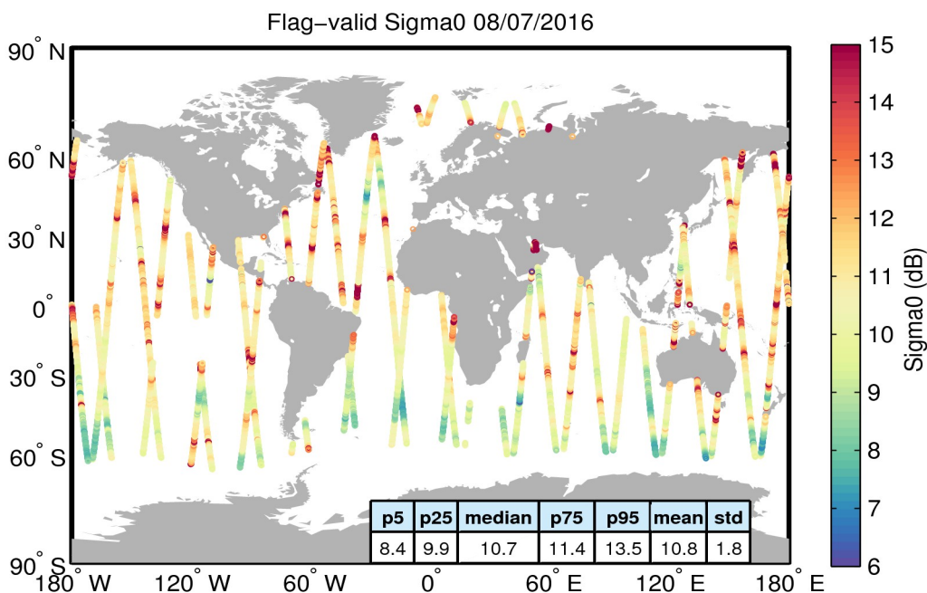
Figure 23. Geographical distribution of flag-valid sigma0 data over oceans and lakes for 08/07/2016. The statistical values shown in the table refer to the sigma0 in dB and are calculated over all measurements shown in the figure.
