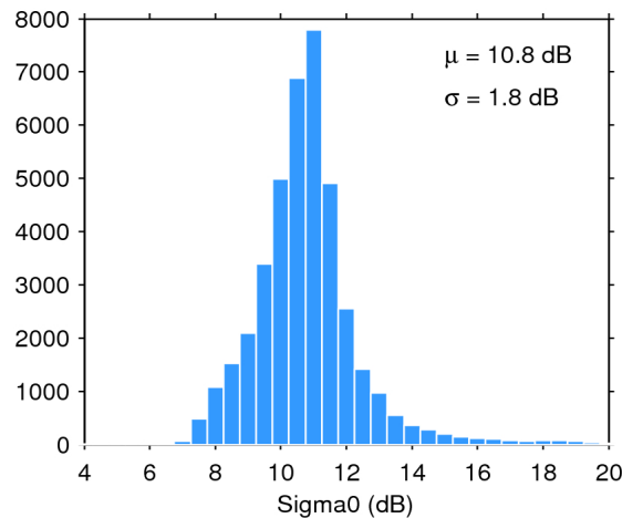
Figure 25. Histogram of flag-valid sigma0 over oceans and lakes for 08/07/2016. The mean ( \mu ) and standard deviation ( \sigma ) are also shown. Note that values outside [4 20] dB are excluded from the histogram for the sake of readability but not from the computation of \mu and \sigma .
