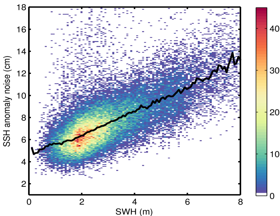
Figure 9. 2D histogram showing flag-valid SSH anomaly noise as a function of SWH for 08/07/2016. The black line denotes the median SSH anomaly noise as a function of SWH.
