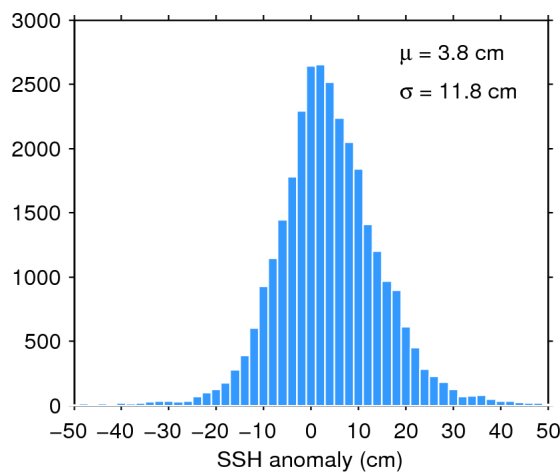
Figure 11. Histogram of science-valid SSH anomaly over oceans and lakes for 08/07/2016. The mean ( \mu ) and standard deviation ( \sigma ) are also shown. Note that values outside [-50 50] cm are excluded from the histogram for the sake of readability but not from the computation of \mu and \sigma .
