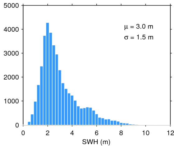
Figure 20. Histogram of science-valid SWH over oceans and lakes for 08/07/2016. The mean ( \mu ) and standard deviation ( \sigma ) are also shown. Note that values larger than 12 m are excluded from the histogram for the sake of readability but not from the computation of \mu and \sigma .
