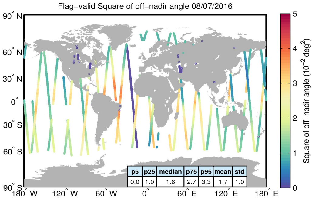
Figure 37. Geographical distribution of flag-valid mispointing data over oceans and lakes for 08/07/2016. The statistical values shown in the table refer to the mispointing in 10^{-2} \text{deg}^2 and are calculated over all measurements shown in the figure.
