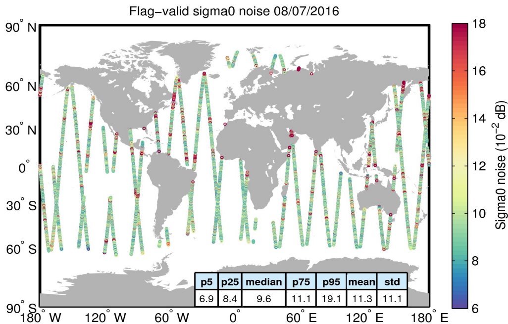
Figure 26. Geographical distribution of flag-valid 20-Hz sigma0 measurement noise over oceans and lakes for 08/07/2016. The statistical values shown in the table refer to the sigma0 noise and are calculated over all measurements shown in the figure.
