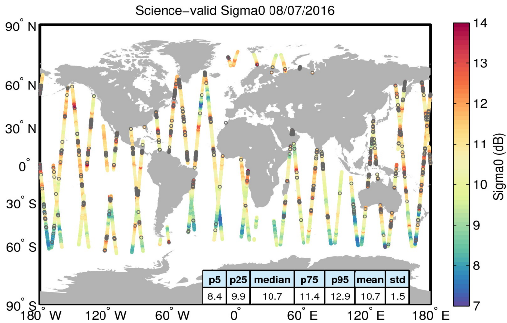
Figure 27. Geographical distribution of science-valid sigma0 data over oceans and lakes for 08/07/2016. The statistical values shown in the table refer to the sigma0 in dB and are calculated over all measurements shown in the figure. Gray circles denote records that have been rejected based on the editing criteria described in Table 4.
