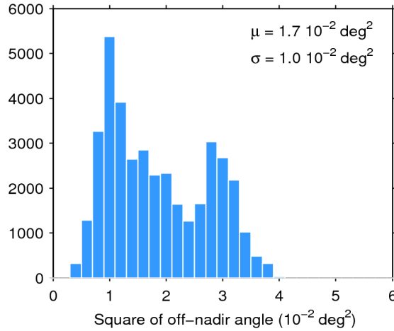
Figure 39. Histogram of flag-valid mispointing over oceans and lakes for 08/07/2016. The mean ( \mu ) and standard deviation ( \sigma ) are also shown. Note that values larger than 6 \cdot 10^{-2} \text{ deg}^2 are excluded from the histogram for the sake of readability but not from the computation of \mu and \sigma .
