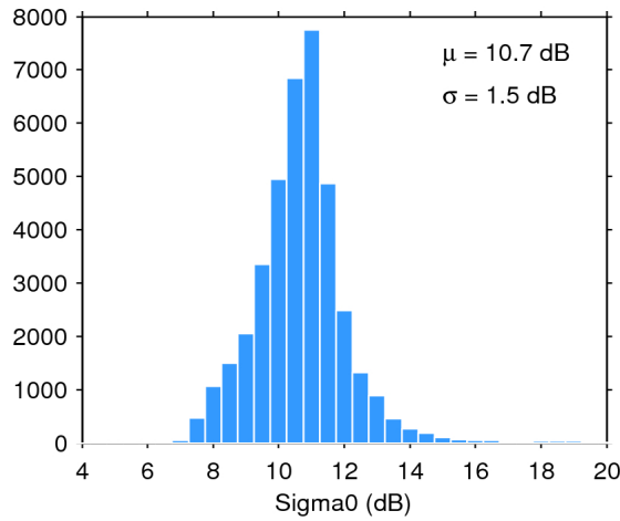
Figure 28. Histogram of science-valid sigma0 over oceans and lakes for 08/07/2016. The mean ( \mu ) and standard deviation ( \sigma ) are also shown. Note that values outside [4 20] dB are excluded from the histogram for the sake of readability but not from the computation of \mu and \sigma .
