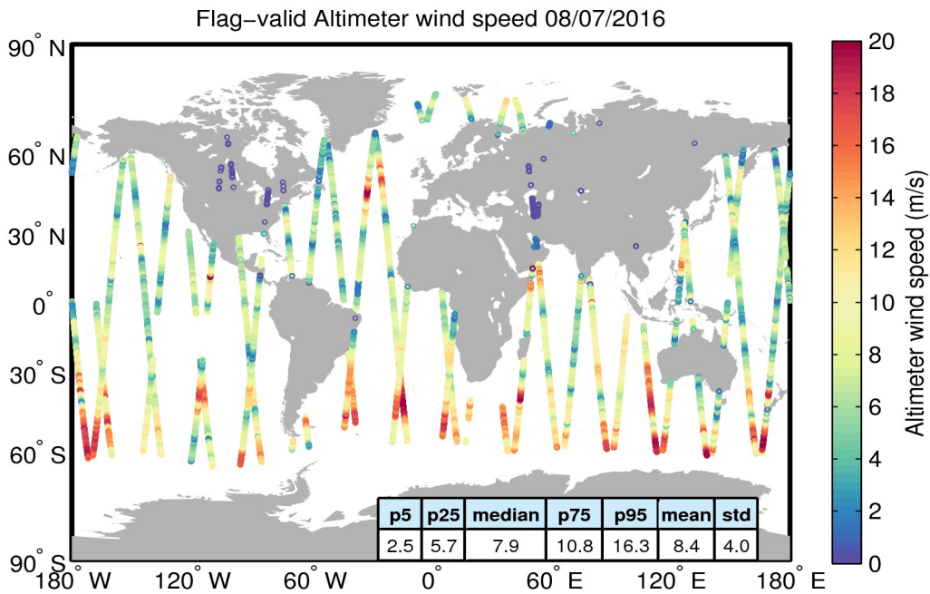
Figure 31. Geographical distribution of flag-valid wind data over oceans and lakes for 08/07/2016. The statistical values shown in the table refer to the wind in m/s and are calculated over all measurements shown in the figure.
