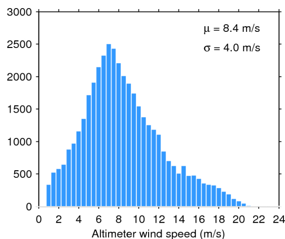
Figure 35. Histogram of science-valid wind over oceans and lakes for 08/07/2016. The mean ( \mu ) and standard deviation ( \sigma ) are also shown. Note that values larger than 24 m/s are excluded from the histogram for the sake of readability but not from the computation of \mu and \sigma .
