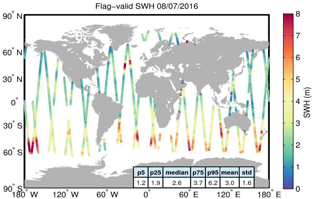
Figure 15. Geographical distribution of flag-valid SWH data over oceans and lakes for 08/07/2016. The statistical values shown in the table refer to the SWH in m and are calculated over all measurements shown in the figure.
