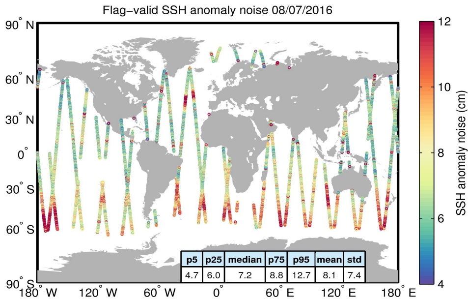
Figure 8. Geographical distribution of flag-valid 20-Hz SSH anomaly measurement noise over oceans and lakes for 08/07/2016. The statistical values shown in the table refer to the SSH anomaly noise and are calculated over all measurements shown in the figure.
