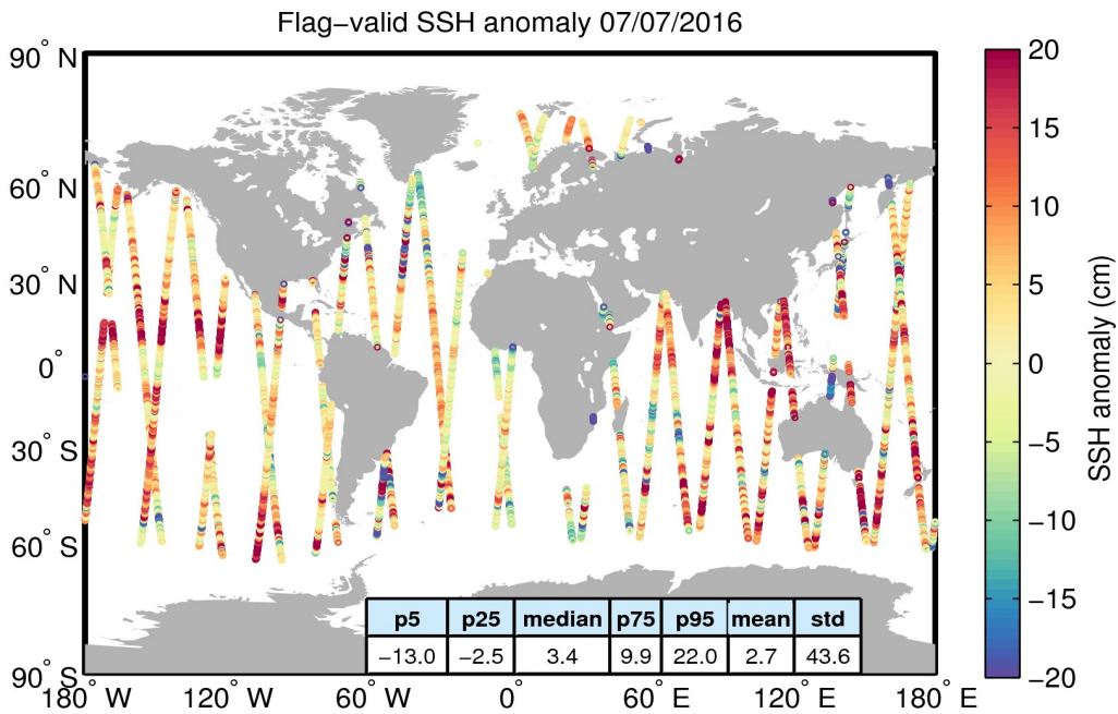
Figure 5. Geographical distribution of flag-valid 1-Hz SSH anomaly data over oceans and lakes for 07/07/2016. The statistical values shown in the table refer to the SSH anomaly in cm and are calculated over all measurements shown in the figure.
