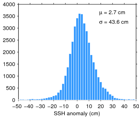
Figure 7. Histogram of flag-valid SSH anomaly over oceans and lakes for 07/07/2016. The mean ( \mu ) and standard deviation ( \sigma ) are also shown. Note that values outside [-50\ 50] cm are excluded from the histogram for the sake of readability but not from the computation of \mu and \sigma .
