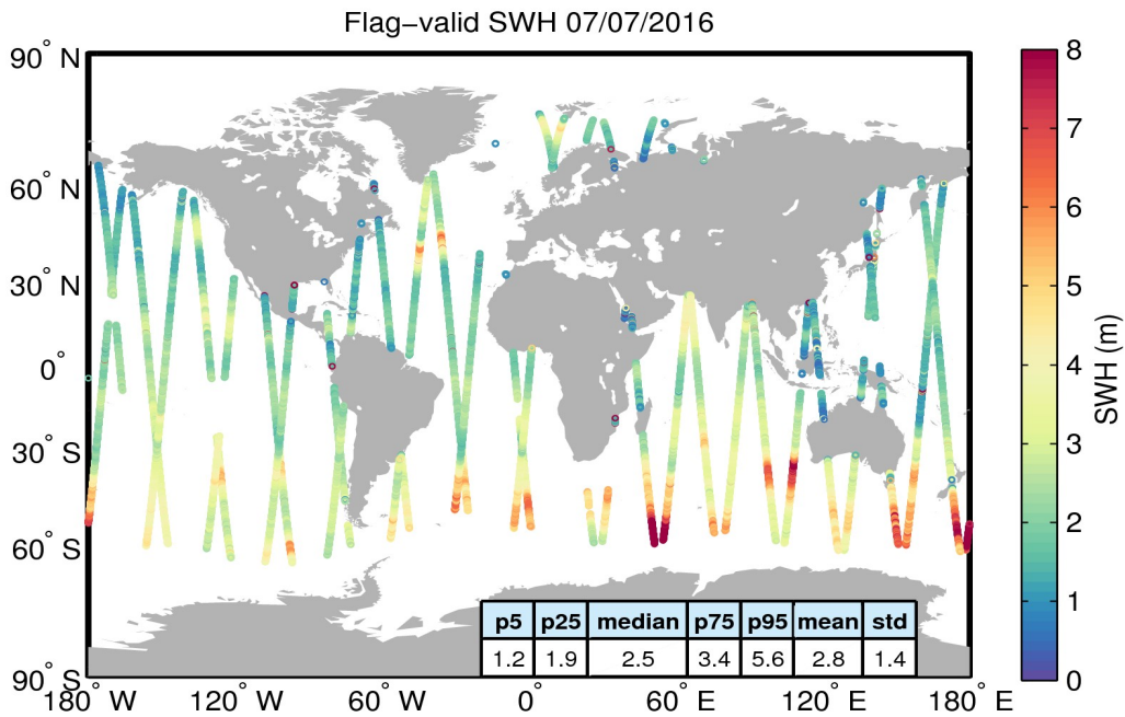
Figure 15. Geographical distribution of flag-valid SWH data over oceans and lakes for 07/07/2016. The statistical values shown in the table refer to the SWH in m and are calculated over all measurements shown in the figure.
