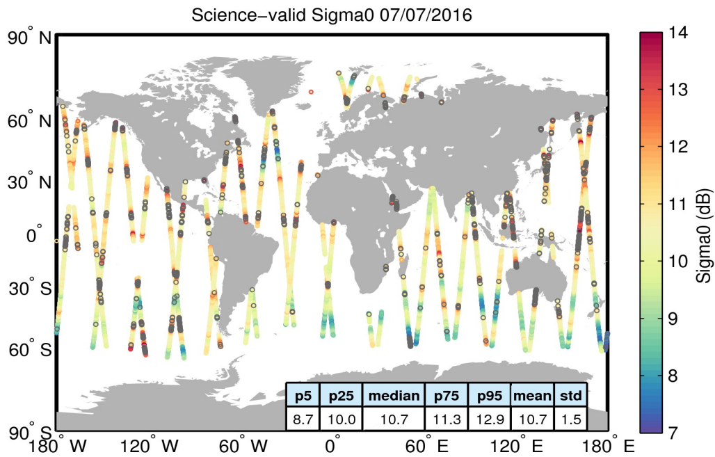
Figure 27. Geographical distribution of science-valid sigma0 data over oceans and lakes for 07/07/2016. The statistical values shown in the table refer to the sigma0 in dB and are calculated over all measurements shown in the figure. Gray circles denote records that have been rejected based on the editing criteria described in Table 4.
