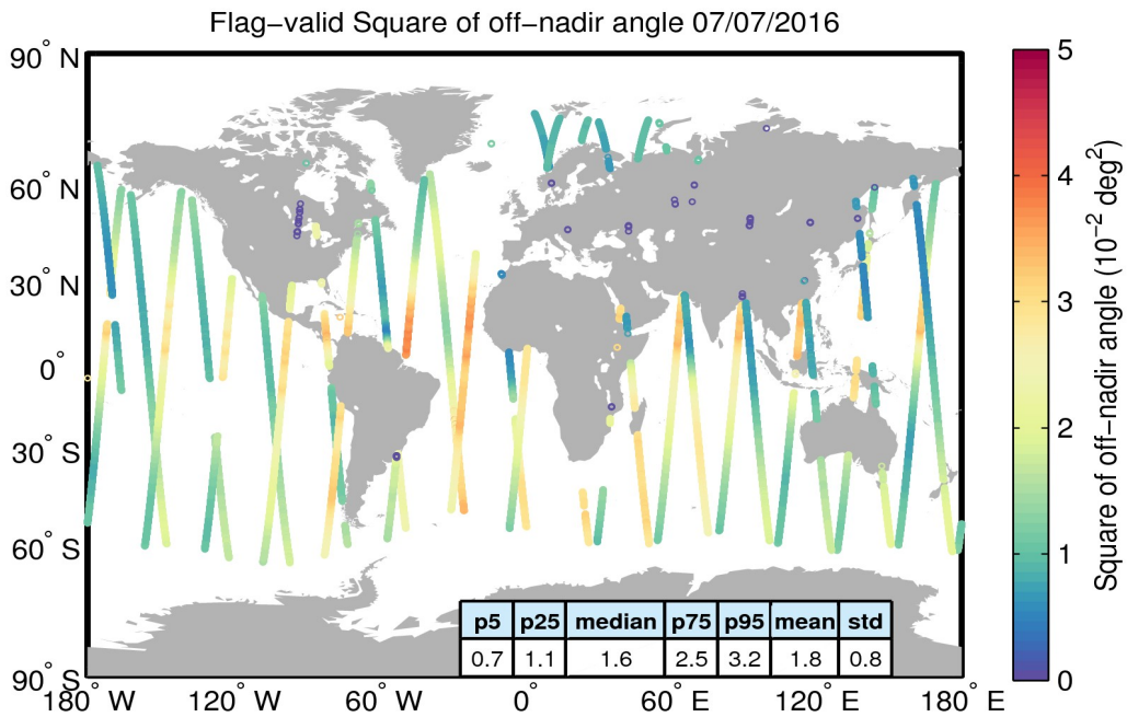
Figure 37. Geographical distribution of flag-valid mispointing data over oceans and lakes for 07/07/2016. The statistical values shown in the table refer to the mispointing in 10^{-2} deg 2 and are calculated over all measurements shown in the figure.
