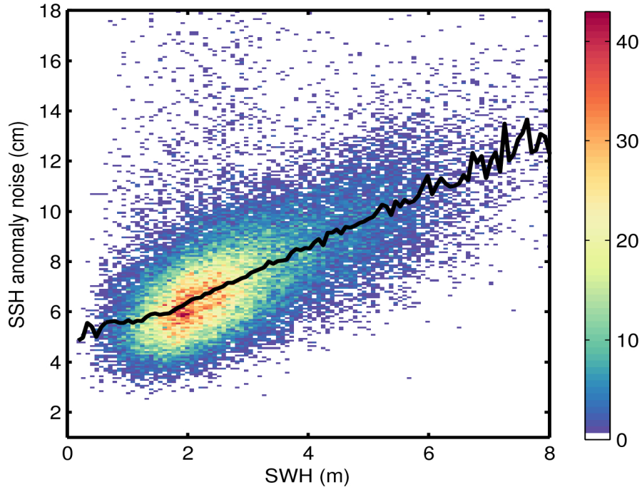
Figure 9. 2D histogram showing flag-valid SSH anomaly noise as a function of SWH for 07/07/2016. The black line denotes the median SSH anomaly noise as a function of SWH.
