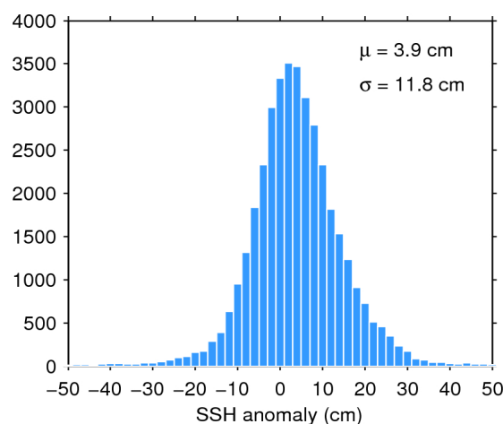
Figure 11. Histogram of science-valid SSH anomaly over oceans and lakes for 07/07/2016. The mean ( \mu ) and standard deviation ( \sigma ) are also shown. Note that values outside [-50 50] cm are excluded from the histogram for the sake of readability but not from the computation of \mu and \sigma .
