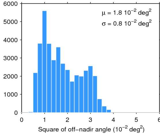
Figure 39. Histogram of flag-valid mispointing over oceans and lakes for 07/07/2016. The mean ( \mu ) and standard deviation ( \sigma ) are also shown. Note that values larger than 6 \cdot 10^{-2} \text{ deg}^2 are excluded from the histogram for the sake of readability but not from the computation of \mu and \sigma .
