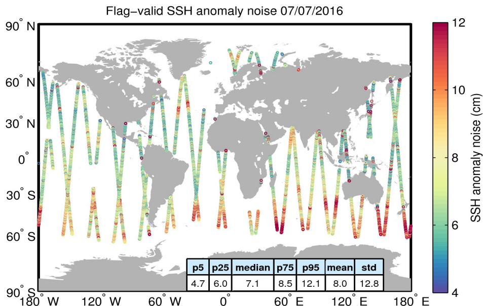
Figure 8. Geographical distribution of flag-valid 20-Hz SSH anomaly measurement noise over oceans and lakes for 07/07/2016. The statistical values shown in the table refer to the SSH anomaly noise and are calculated over all measurements shown in the figure.
