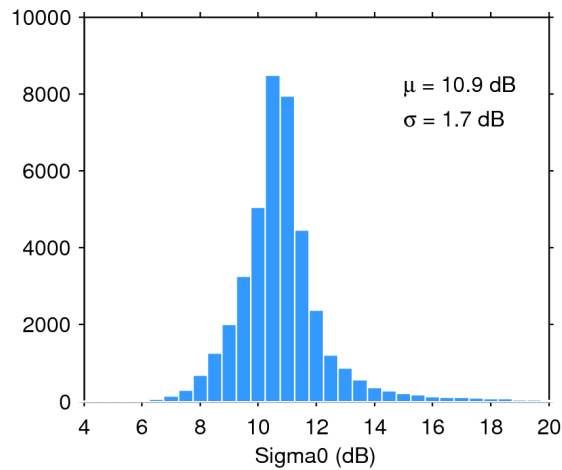
Figure 25. Histogram of flag-valid sigma0 over oceans and lakes for 07/07/2016. The mean ( \mu ) and standard deviation ( \sigma ) are also shown. Note that values outside [4 20] dB are excluded from the histogram for the sake of readability but not from the computation of \mu and \sigma .
