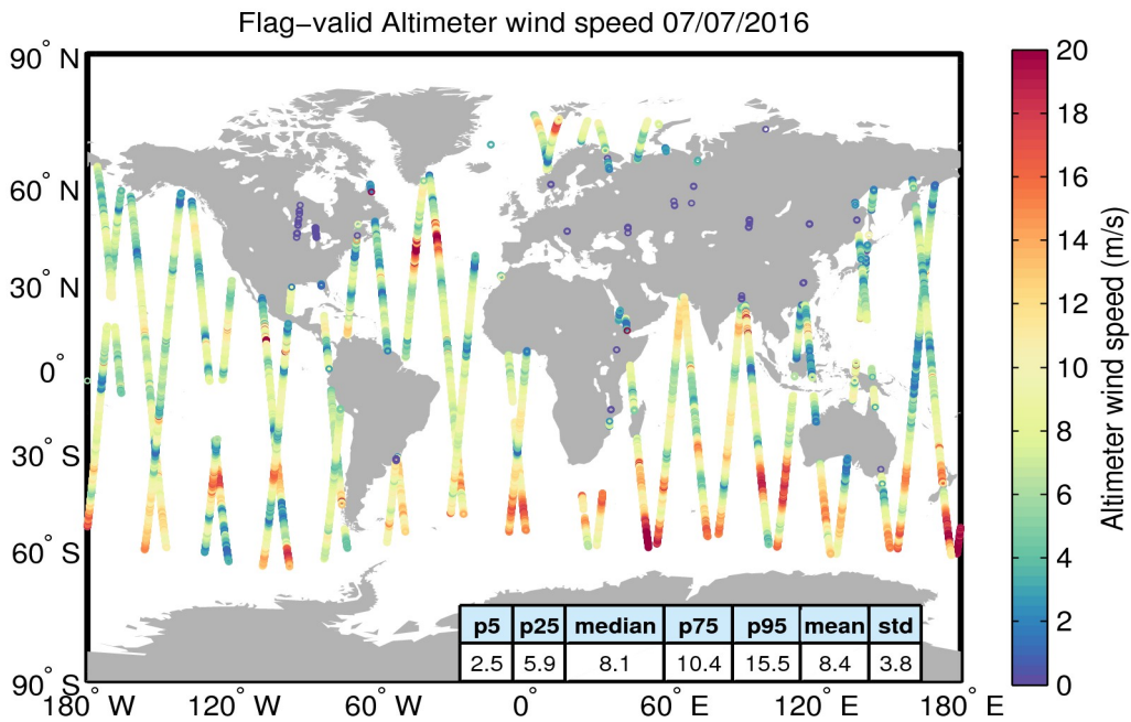
Figure 31. Geographical distribution of flag-valid wind data over oceans and lakes for 07/07/2016. The statistical values shown in the table refer to the wind in m/s and are calculated over all measurements shown in the figure.
