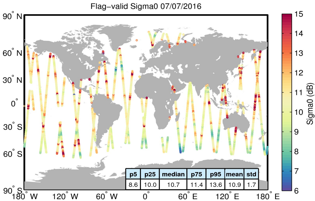
Figure 23. Geographical distribution of flag-valid sigma0 data over oceans and lakes for 07/07/2016. The statistical values shown in the table refer to the sigma0 in dB and are calculated over all measurements shown in the figure.
