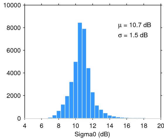
Figure 28. Histogram of science-valid sigma0 over oceans and lakes for 07/07/2016. The mean ( \mu ) and standard deviation ( \sigma ) are also shown. Note that values outside [4 20] dB are excluded from the histogram for the sake of readability but not from the computation of \mu and \sigma .
