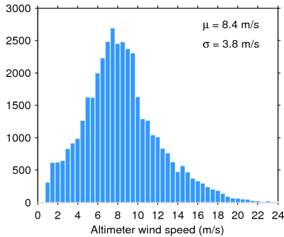
Figure 33. Histogram of flag-valid wind over oceans and lakes for 07/07/2016. The mean ( \mu ) and standard deviation ( \sigma ) are also shown. Note that values larger than 24 m/s are excluded from the histogram for the sake of readability but not from the computation of \mu and \sigma .
