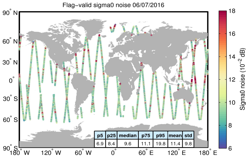
Figure 26. Geographical distribution of flag-valid 20-Hz sigma0 measurement noise over oceans and lakes for 06/07/2016. The statistical values shown in the table refer to the sigma0 noise and are calculated over all measurements shown in the figure.
