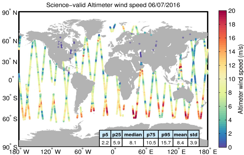
Figure 34. Geographical distribution of science-valid wind data over oceans and lakes for 06/07/2016. The statistical values shown in the table refer to the wind in m/s and are calculated over all measurements shown in the figure. Gray circles denote records that have been rejected based on the editing criteria described in Table 5.
