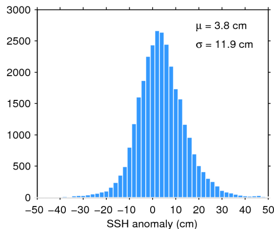
Figure 11. Histogram of science-valid SSH anomaly over oceans and lakes for 06/07/2016. The mean ( \mu ) and standard deviation ( \sigma ) are also shown. Note that values outside [-50 50] cm are excluded from the histogram for the sake of readability but not from the computation of \mu and \sigma .
