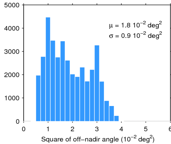
Figure 39. Histogram of flag-valid mispointing over oceans and lakes for 06/07/2016. The mean ( \mu ) and standard deviation ( \sigma ) are also shown. Note that values larger than 6 \cdot 10^{-2} \text{ deg}^2 are excluded from the histogram for the sake of readability but not from the computation of \mu and \sigma .
