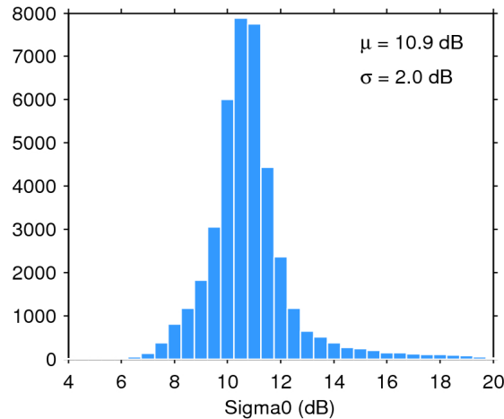
Figure 25. Histogram of flag-valid sigma0 over oceans and lakes for 06/07/2016. The mean ( \mu ) and standard deviation ( \sigma ) are also shown. Note that values outside [4 20] dB are excluded from the histogram for the sake of readability but not from the computation of \mu and \sigma .
