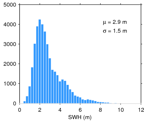
Figure 17. Histogram of flag-valid SWH over oceans and lakes for 06/07/2016. The mean ( \mu ) and standard deviation ( \sigma ) are also shown. Note that values larger than 12 m are excluded from the histogram for the sake of readability but not from the computation of \mu and \sigma .
