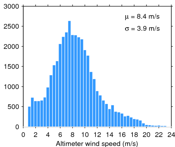
Figure 35. Histogram of science-valid wind over oceans and lakes for 06/07/2016. The mean ( \mu ) and standard deviation ( \sigma ) are also shown. Note that values larger than 24 m/s are excluded from the histogram for the sake of readability but not from the computation of \mu and \sigma .
