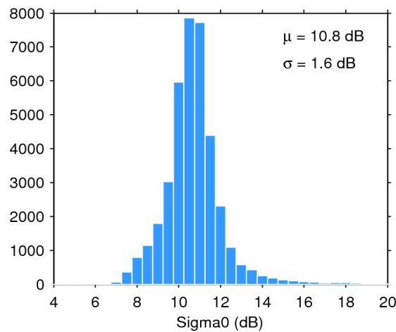
Figure 28. Histogram of science-valid sigma0 over oceans and lakes for 06/07/2016. The mean ( \mu ) and standard deviation ( \sigma ) are also shown. Note that values outside [4 20] dB are excluded from the histogram for the sake of readability but not from the computation of \mu and \sigma .
