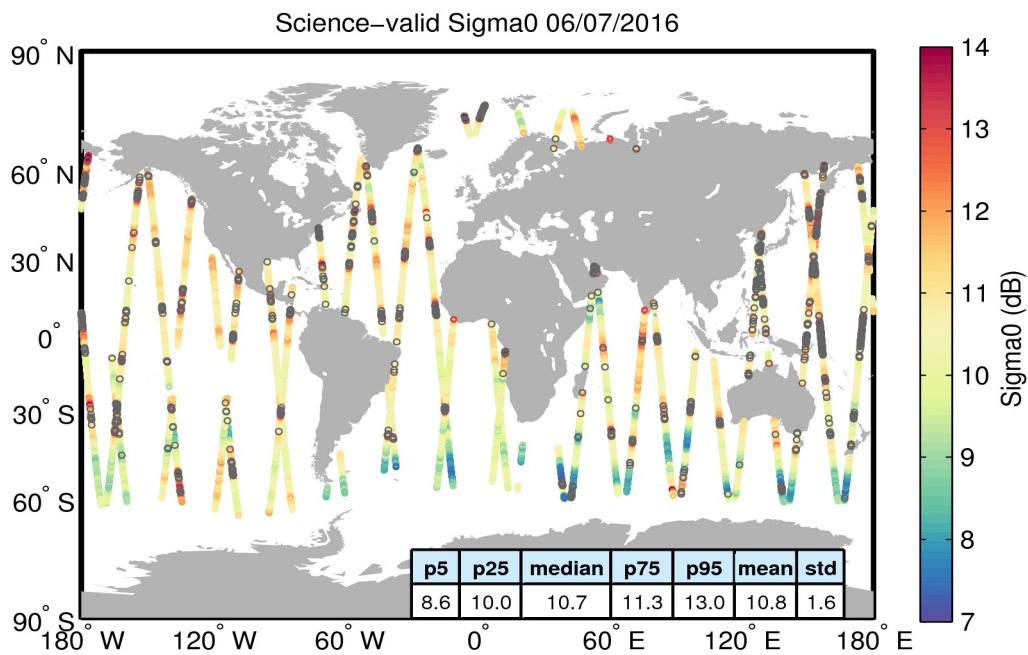
Figure 27. Geographical distribution of science-valid sigma0 data over oceans and lakes for 06/07/2016. The statistical values shown in the table refer to the sigma0 in dB and are calculated over all measurements shown in the figure. Gray circles denote records that have been rejected based on the editing criteria described in Table 4.
