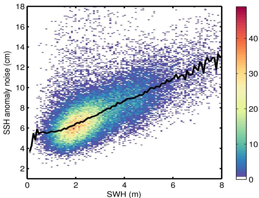
Figure 9. 2D histogram showing flag-valid SSH anomaly noise as a function of SWH for 06/07/2016. The black line denotes the median SSH anomaly noise as a function of SWH.
