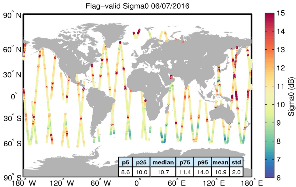
Figure 23. Geographical distribution of flag-valid sigma0 data over oceans and lakes for 06/07/2016. The statistical values shown in the table refer to the sigma0 in dB and are calculated over all measurements shown in the figure.
