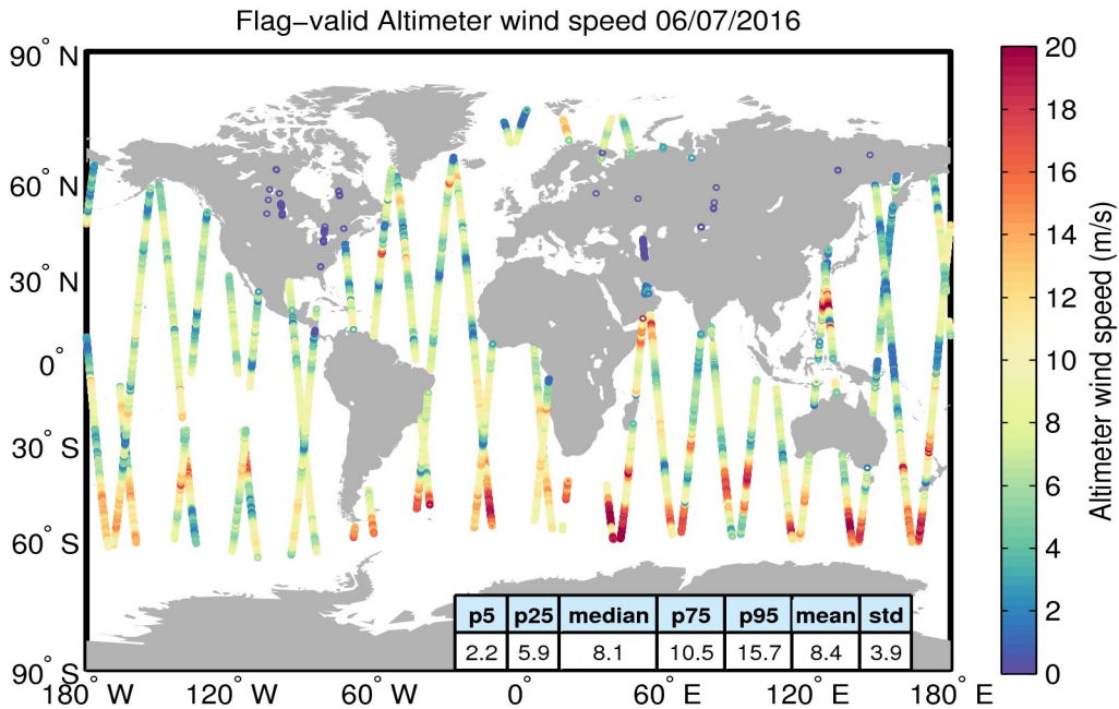
Figure 31. Geographical distribution of flag-valid wind data over oceans and lakes for 06/07/2016. The statistical values shown in the table refer to the wind in m/s and are calculated over all measurements shown in the figure.
