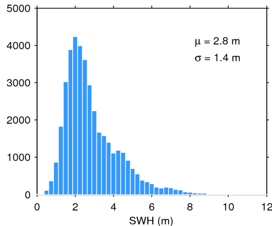
Figure 20. Histogram of science-valid SWH over oceans and lakes for 06/07/2016. The mean ( \mu ) and standard deviation ( \sigma ) are also shown. Note that values larger than 12 m are excluded from the histogram for the sake of readability but not from the computation of \mu and \sigma .
