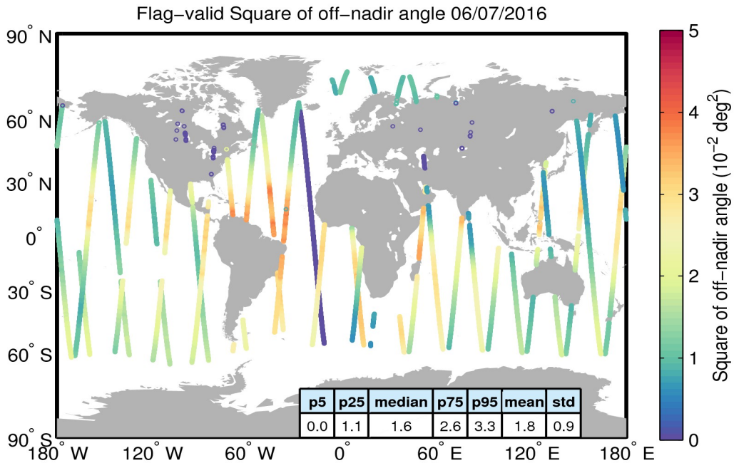
Figure 37. Geographical distribution of flag-valid mispointing data over oceans and lakes for 06/07/2016. The statistical values shown in the table refer to the mispointing in 10^{-2} \text{ deg}^2 and are calculated over all measurements shown in the figure.
