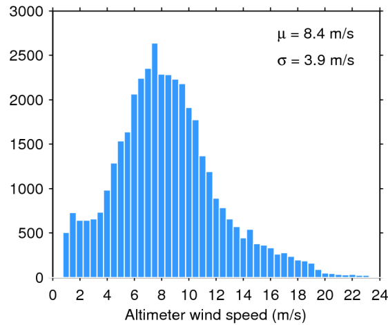
Figure 33. Histogram of flag-valid wind over oceans and lakes for 06/07/2016. The mean ( \mu ) and standard deviation ( \sigma ) are also shown. Note that values larger than 24 m/s are excluded from the histogram for the sake of readability but not from the computation of \mu and \sigma .
