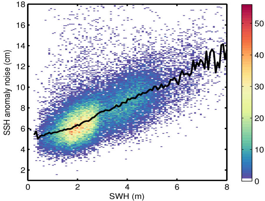
Figure 9. 2D histogram showing flag-valid SSH anomaly noise as a function of SWH for 05/07/2016. The black line denotes the median SSH anomaly noise as a function of SWH.
