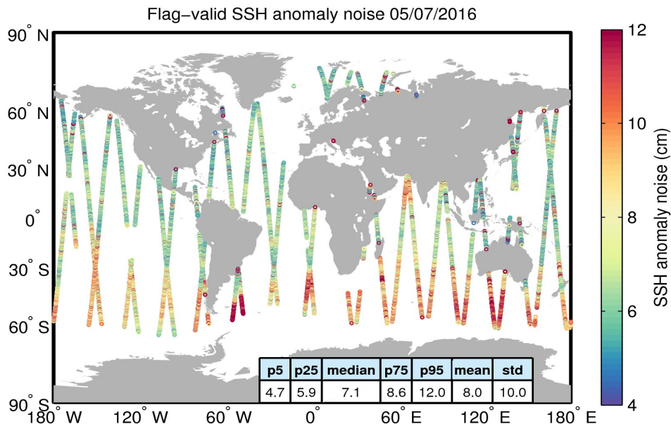
Figure 8. Geographical distribution of flag-valid 20-Hz SSH anomaly measurement noise over oceans and lakes for 05/07/2016. The statistical values shown in the table refer to the SSH anomaly noise and are calculated over all measurements shown in the figure.
