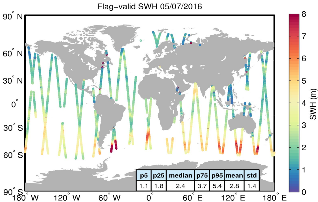
Figure 15. Geographical distribution of flag-valid SWH data over oceans and lakes for 05/07/2016. The statistical values shown in the table refer to the SWH in m and are calculated over all measurements shown in the figure.
