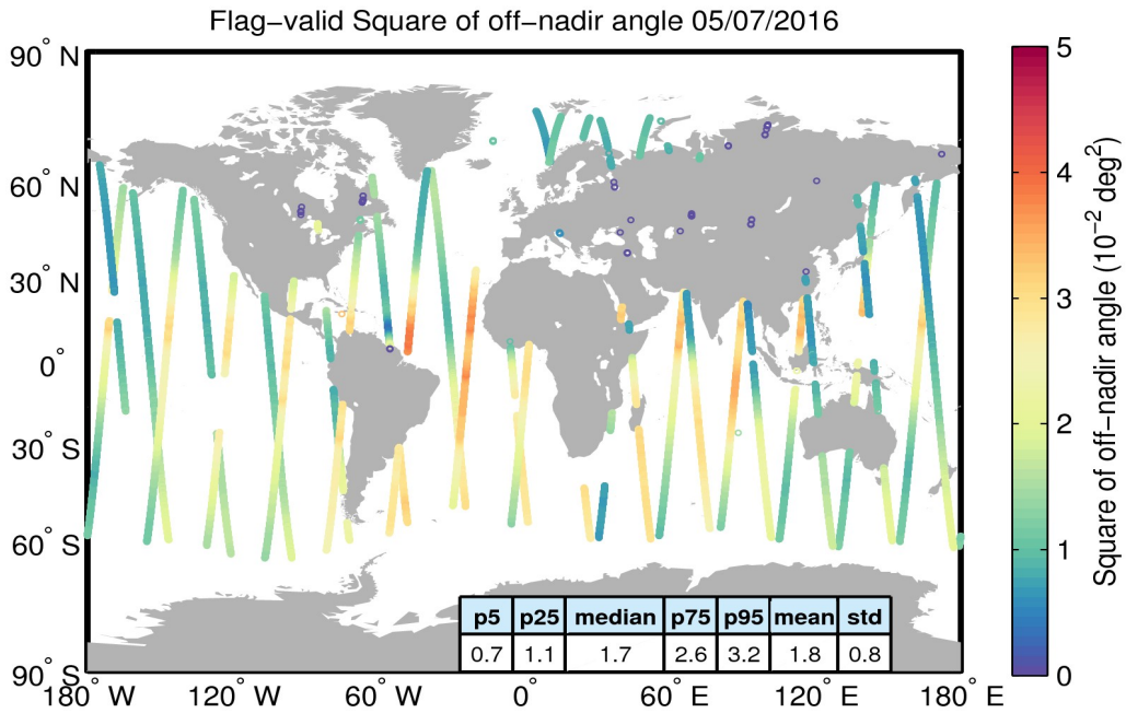
Figure 37. Geographical distribution of flag-valid mispointing data over oceans and lakes for 05/07/2016. The statistical values shown in the table refer to the mispointing in 10^{-2} deg 2 and are calculated over all measurements shown in the figure.
