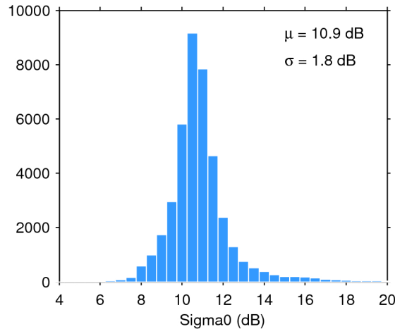
Figure 25. Histogram of flag-valid sigma0 over oceans and lakes for 05/07/2016. The mean ( \mu ) and standard deviation ( \sigma ) are also shown. Note that values outside [4 20] dB are excluded from the histogram for the sake of readability but not from the computation of \mu and \sigma .
