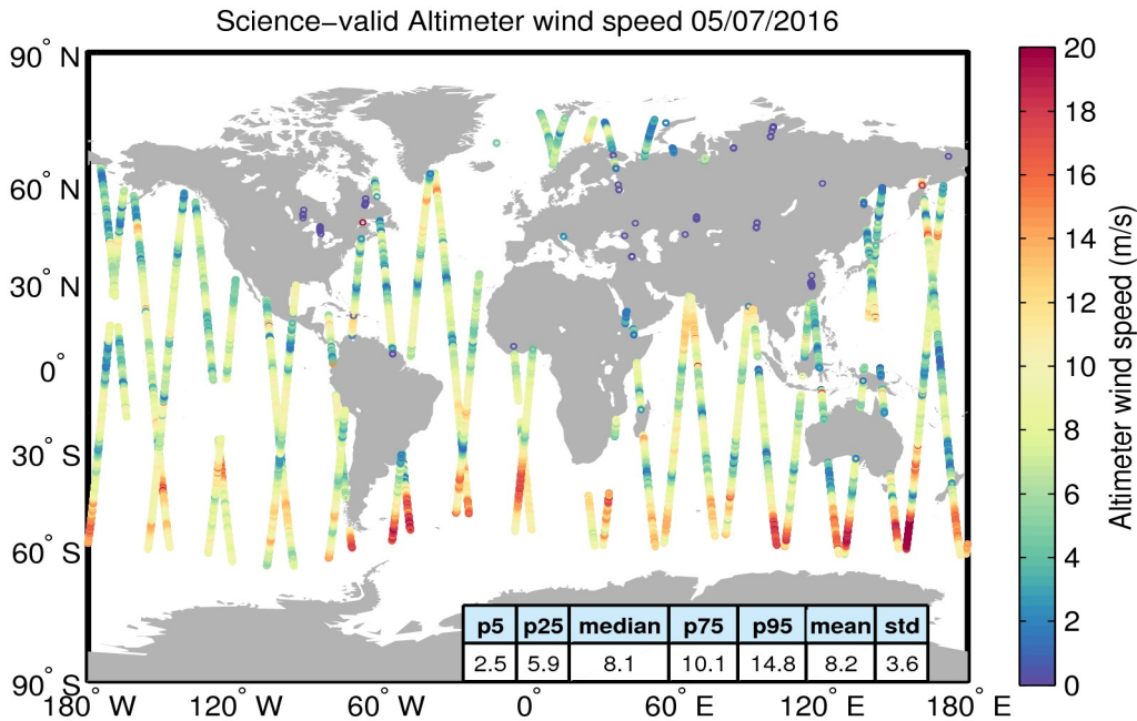
Figure 34. Geographical distribution of science-valid wind data over oceans and lakes for 05/07/2016. The statistical values shown in the table refer to the wind in m/s and are calculated over all measurements shown in the figure. Gray circles denote records that have been rejected based on the editing criteria described in Table 5.
