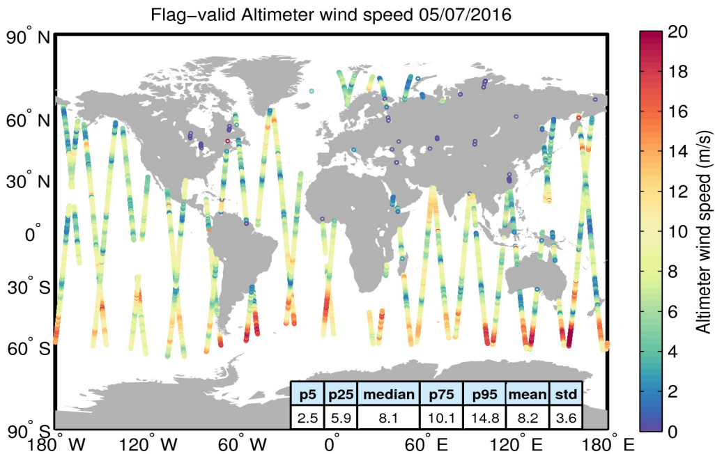
Figure 31. Geographical distribution of flag-valid wind data over oceans and lakes for 05/07/2016. The statistical values shown in the table refer to the wind in m/s and are calculated over all measurements shown in the figure.
