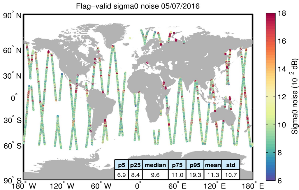
Figure 26. Geographical distribution of flag-valid 20-Hz sigma0 measurement noise over oceans and lakes for 05/07/2016. The statistical values shown in the table refer to the sigma0 noise and are calculated over all measurements shown in the figure.
