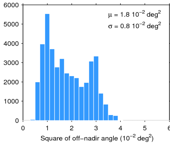
Figure 39. Histogram of flag-valid mispointing over oceans and lakes for 05/07/2016. The mean ( \mu ) and standard deviation ( \sigma ) are also shown. Note that values larger than 6 \cdot 10^{-2} \text{ deg}^2 are excluded from the histogram for the sake of readability but not from the computation of \mu and \sigma .
