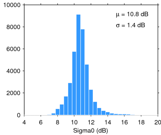
Figure 28. Histogram of science-valid sigma0 over oceans and lakes for 05/07/2016. The mean ( \mu ) and standard deviation ( \sigma ) are also shown. Note that values outside [4 20] dB are excluded from the histogram for the sake of readability but not from the computation of \mu and \sigma .
