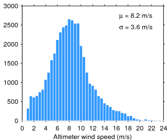
Figure 35. Histogram of science-valid wind over oceans and lakes for 05/07/2016. The mean ( \mu ) and standard deviation ( \sigma ) are also shown. Note that values larger than 24 m/s are excluded from the histogram for the sake of readability but not from the computation of \mu and \sigma .
