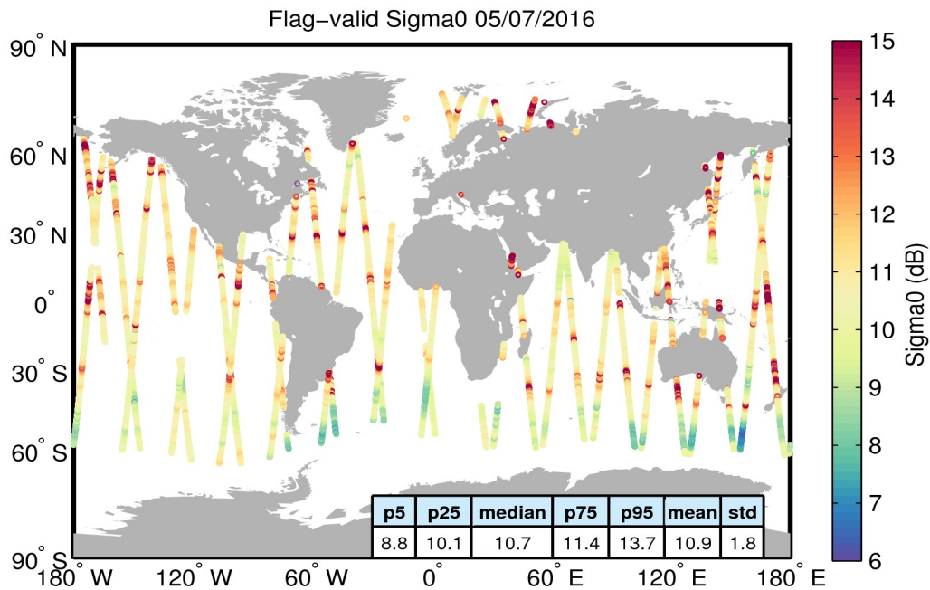
Figure 23. Geographical distribution of flag-valid sigma0 data over oceans and lakes for 05/07/2016. The statistical values shown in the table refer to the sigma0 in dB and are calculated over all measurements shown in the figure.
