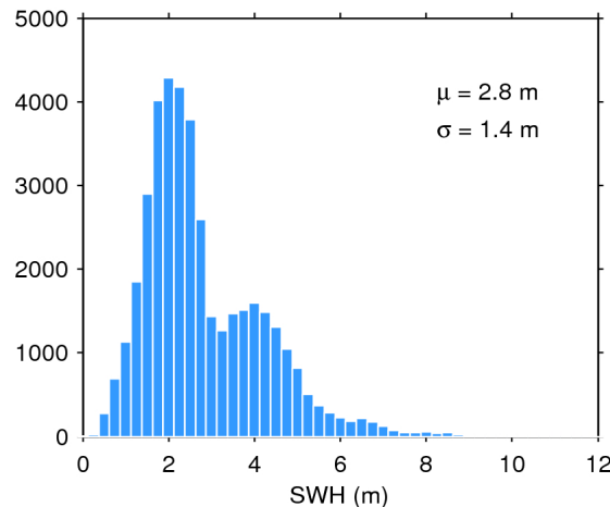
Figure 20. Histogram of science-valid SWH over oceans and lakes for 05/07/2016. The mean ( \mu ) and standard deviation ( \sigma ) are also shown. Note that values larger than 12 m are excluded from the histogram for the sake of readability but not from the computation of \mu and \sigma .
