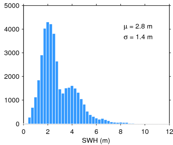
Figure 17. Histogram of flag-valid SWH over oceans and lakes for 05/07/2016. The mean ( \mu ) and standard deviation ( \sigma ) are also shown. Note that values larger than 12 m are excluded from the histogram for the sake of readability but not from the computation of \mu and \sigma .
