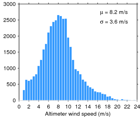
Figure 33. Histogram of flag-valid wind over oceans and lakes for 05/07/2016. The mean ( \mu ) and standard deviation ( \sigma ) are also shown. Note that values larger than 24 m/s are excluded from the histogram for the sake of readability but not from the computation of \mu and \sigma .
