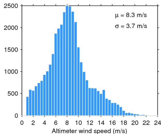
Figure 35. Histogram of science-valid wind over oceans and lakes for 04/07/2016. The mean ( \mu ) and standard deviation ( \sigma ) are also shown. Note that values larger than 24 m/s are excluded from the histogram for the sake of readability but not from the computation of \mu and \sigma .
