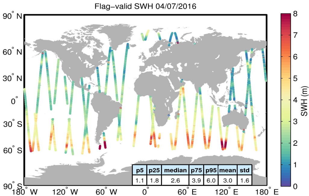
Figure 15. Geographical distribution of flag-valid SWH data over oceans and lakes for 04/07/2016. The statistical values shown in the table refer to the SWH in m and are calculated over all measurements shown in the figure.
