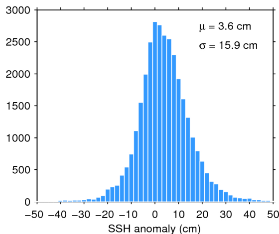
Figure 11. Histogram of science-valid SSH anomaly over oceans and lakes for 04/07/2016. The mean ( \mu ) and standard deviation ( \sigma ) are also shown. Note that values outside [-50 50] cm are excluded from the histogram for the sake of readability but not from the computation of \mu and \sigma .
