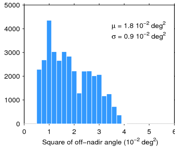
Figure 39. Histogram of flag-valid mispointing over oceans and lakes for 04/07/2016. The mean ( \mu ) and standard deviation ( \sigma ) are also shown. Note that values larger than 6 \cdot 10^{-2} \text{ deg}^2 are excluded from the histogram for the sake of readability but not from the computation of \mu and \sigma .
