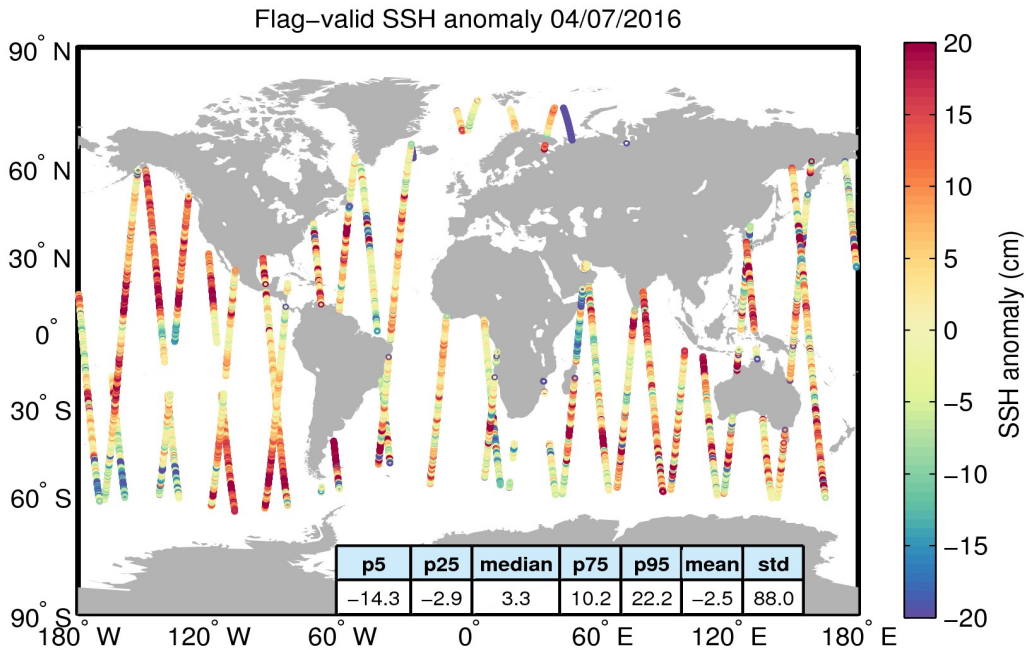
Figure 5. Geographical distribution of flag-valid 1-Hz SSH anomaly data over oceans and lakes for 04/07/2016. The statistical values shown in the table refer to the SSH anomaly in cm and are calculated over all measurements shown in the figure.
