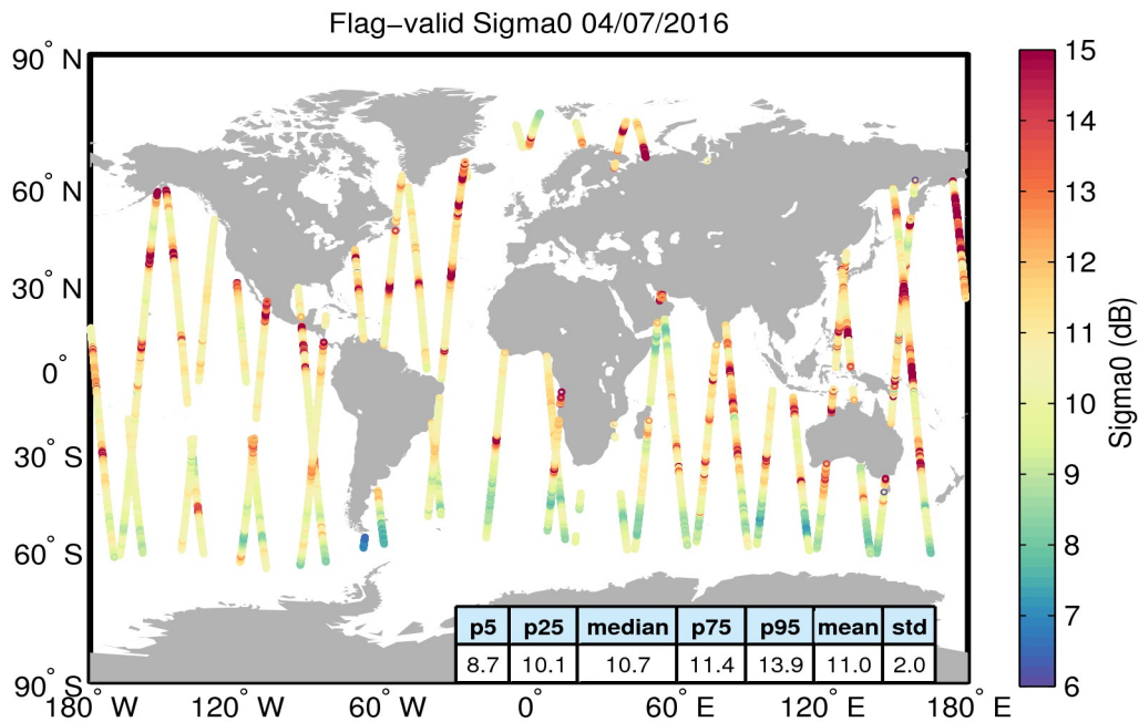
Figure 23. Geographical distribution of flag-valid sigma0 data over oceans and lakes for 04/07/2016. The statistical values shown in the table refer to the sigma0 in dB and are calculated over all measurements shown in the figure.
