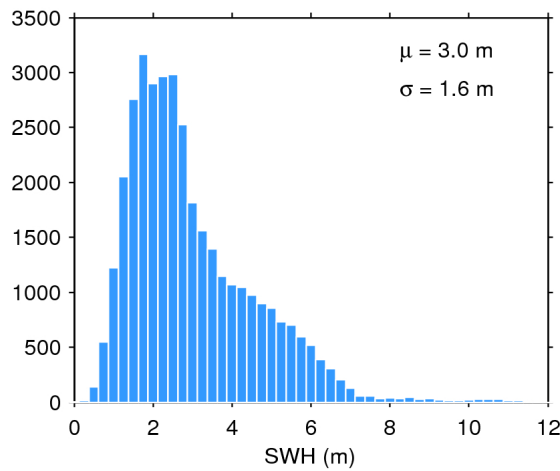
Figure 17. Histogram of flag-valid SWH over oceans and lakes for 04/07/2016. The mean ( \mu ) and standard deviation ( \sigma ) are also shown. Note that values larger than 12 m are excluded from the histogram for the sake of readability but not from the computation of \mu and \sigma .
