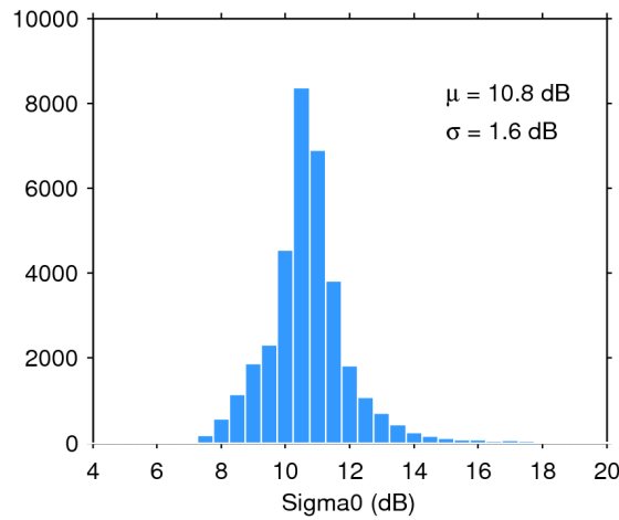
Figure 28. Histogram of science-valid sigma0 over oceans and lakes for 04/07/2016. The mean ( \mu ) and standard deviation ( \sigma ) are also shown. Note that values outside [4 20] dB are excluded from the histogram for the sake of readability but not from the computation of \mu and \sigma .
