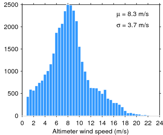
Figure 33. Histogram of flag-valid wind over oceans and lakes for 04/07/2016. The mean ( \mu ) and standard deviation ( \sigma ) are also shown. Note that values larger than 24 m/s are excluded from the histogram for the sake of readability but not from the computation of \mu and \sigma .
