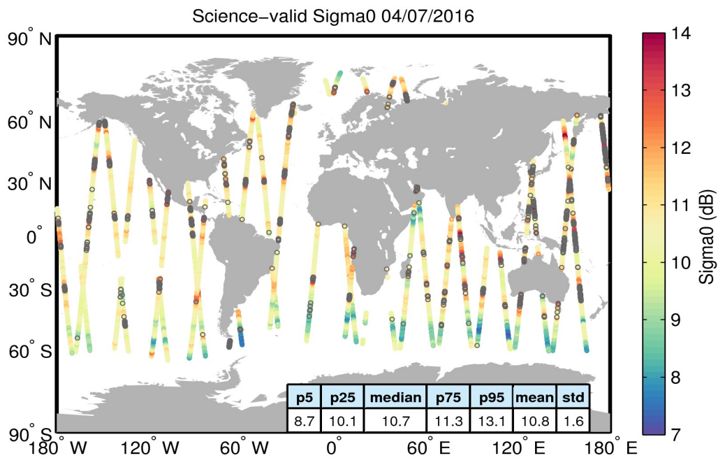
Figure 27. Geographical distribution of science-valid sigma0 data over oceans and lakes for 04/07/2016. The statistical values shown in the table refer to the sigma0 in dB and are calculated over all measurements shown in the figure. Gray circles denote records that have been rejected based on the editing criteria described in Table 4.
