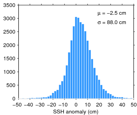
Figure 7. Histogram of flag-valid SSH anomaly over oceans and lakes for 04/07/2016. The mean ( \mu ) and standard deviation ( \sigma ) are also shown. Note that values outside [-50 50] cm are excluded from the histogram for the sake of readability but not from the computation of \mu and \sigma .
