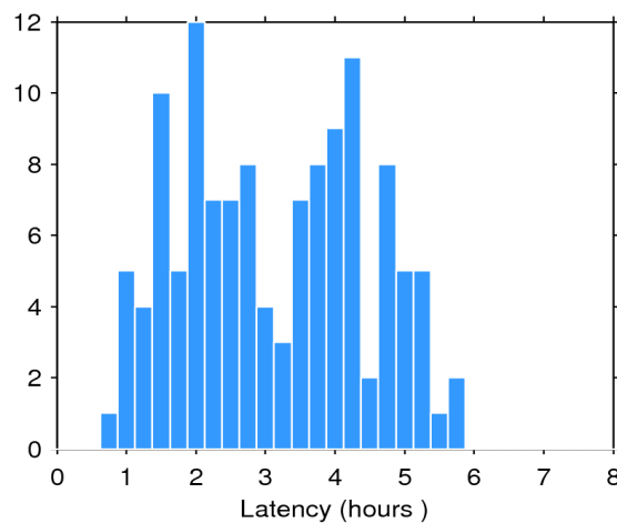
Figure 2. Histogram of the data latency for 04/07/2016. The y-axis denotes the number of files that are made available with a delay of x-hours with respect to the mean time of the records stored in the file.
