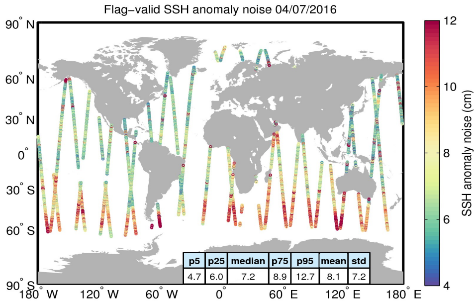
Figure 8. Geographical distribution of flag-valid 20-Hz SSH anomaly measurement noise over oceans and lakes for 04/07/2016. The statistical values shown in the table refer to the SSH anomaly noise and are calculated over all measurements shown in the figure.
