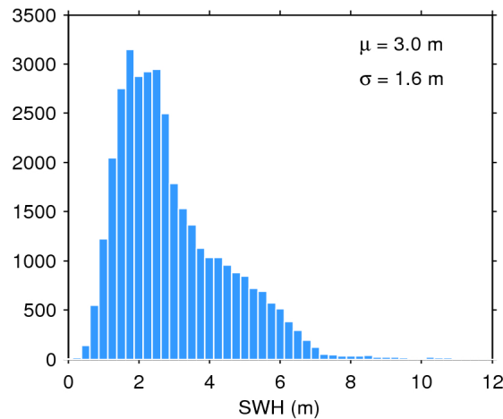
Figure 20. Histogram of science-valid SWH over oceans and lakes for 04/07/2016. The mean ( \mu ) and standard deviation ( \sigma ) are also shown. Note that values larger than 12 m are excluded from the histogram for the sake of readability but not from the computation of \mu and \sigma .
