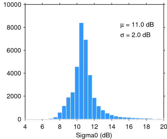
Figure 25. Histogram of flag-valid sigma0 over oceans and lakes for 04/07/2016. The mean ( \mu ) and standard deviation ( \sigma ) are also shown. Note that values outside [4 20] dB are excluded from the histogram for the sake of readability but not from the computation of \mu and \sigma .
