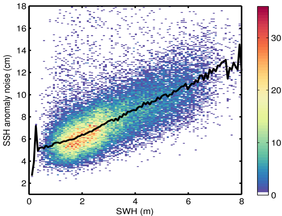
Figure 9. 2D histogram showing flag-valid SSH anomaly noise as a function of SWH for 04/07/2016. The black line denotes the median SSH anomaly noise as a function of SWH.
