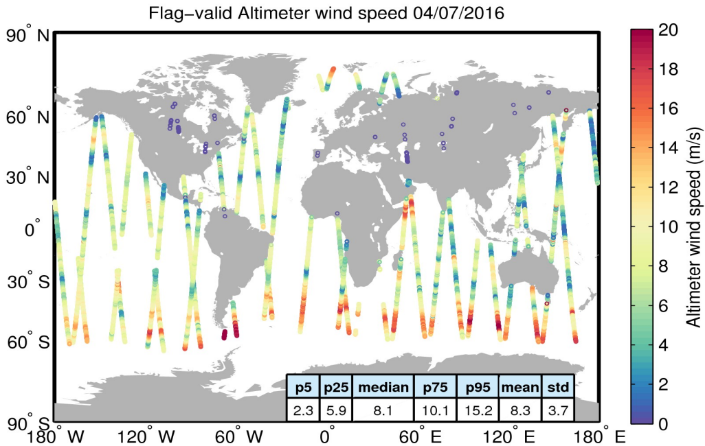
Figure 31. Geographical distribution of flag-valid wind data over oceans and lakes for 04/07/2016. The statistical values shown in the table refer to the wind in m/s and are calculated over all measurements shown in the figure.
