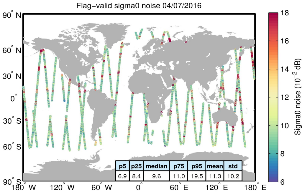
Figure 26. Geographical distribution of flag-valid 20-Hz sigma0 measurement noise over oceans and lakes for 04/07/2016. The statistical values shown in the table refer to the sigma0 noise and are calculated over all measurements shown in the figure.
