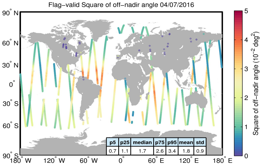
Figure 37. Geographical distribution of flag-valid mispointing data over oceans and lakes for 04/07/2016. The statistical values shown in the table refer to the mispointing in 10^{-2} deg 2 and are calculated over all measurements shown in the figure.
