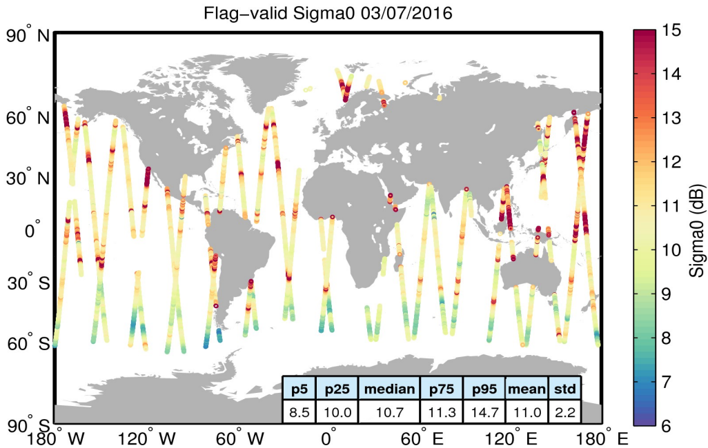
Figure 23. Geographical distribution of flag-valid sigma0 data over oceans and lakes for 03/07/2016. The statistical values shown in the table refer to the sigma0 in dB and are calculated over all measurements shown in the figure.
