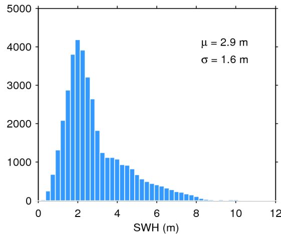
Figure 20. Histogram of science-valid SWH over oceans and lakes for 03/07/2016. The mean ( \mu ) and standard deviation ( \sigma ) are also shown. Note that values larger than 12 m are excluded from the histogram for the sake of readability but not from the computation of \mu and \sigma .
