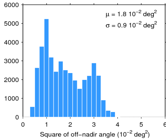
Figure 39. Histogram of flag-valid mispointing over oceans and lakes for 03/07/2016. The mean ( \mu ) and standard deviation ( \sigma ) are also shown. Note that values larger than 6 \cdot 10^{-2} \text{ deg}^2 are excluded from the histogram for the sake of readability but not from the computation of \mu and \sigma .
