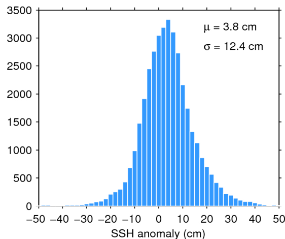
Figure 11. Histogram of science-valid SSH anomaly over oceans and lakes for 03/07/2016. The mean ( \mu ) and standard deviation ( \sigma ) are also shown. Note that values outside [-50 50] cm are excluded from the histogram for the sake of readability but not from the computation of \mu and \sigma .
