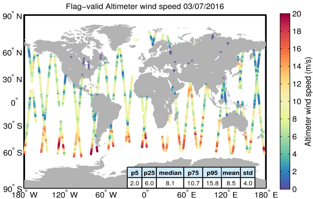
Figure 31. Geographical distribution of flag-valid wind data over oceans and lakes for 03/07/2016. The statistical values shown in the table refer to the wind in m/s and are calculated over all measurements shown in the figure.
