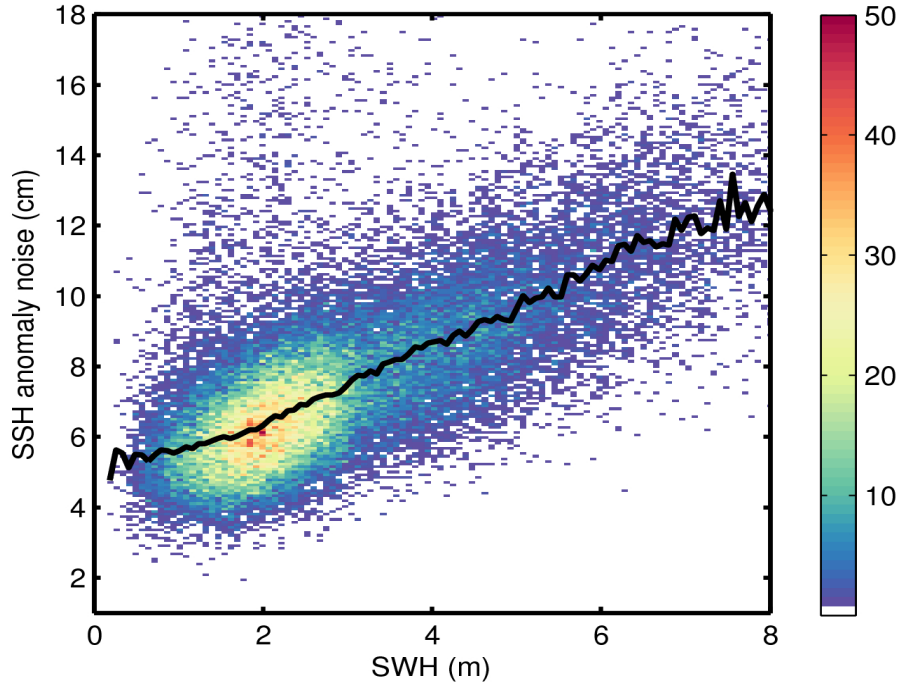
Figure 9. 2D histogram showing flag-valid SSH anomaly noise as a function of SWH for 03/07/2016. The black line denotes the median SSH anomaly noise as a function of SWH.
