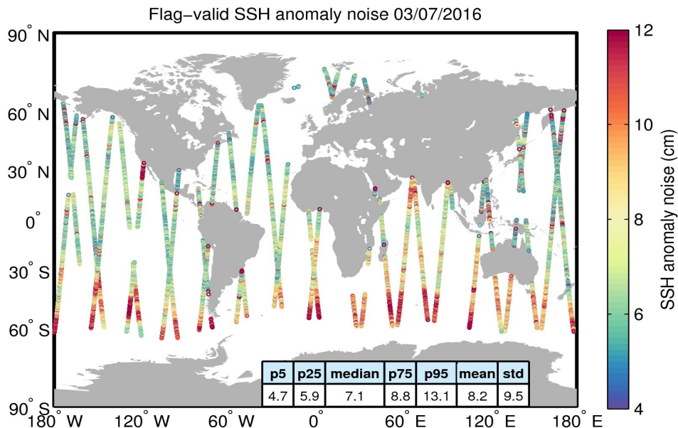
Figure 8. Geographical distribution of flag-valid 20-Hz SSH anomaly measurement noise over oceans and lakes for 03/07/2016. The statistical values shown in the table refer to the SSH anomaly noise and are calculated over all measurements shown in the figure.
