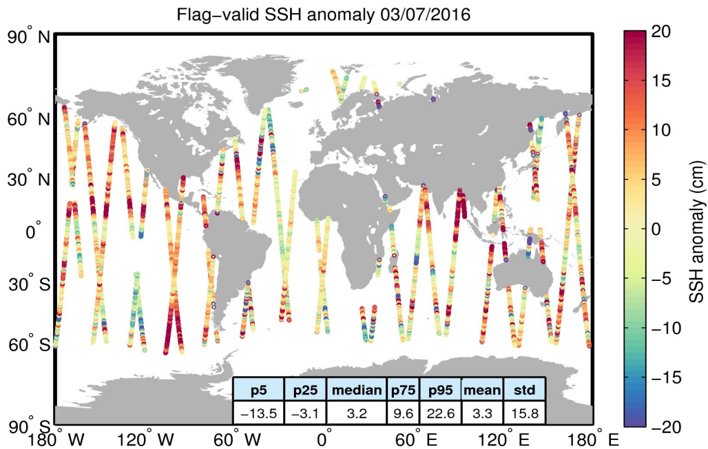
Figure 5. Geographical distribution of flag-valid 1-Hz SSH anomaly data over oceans and lakes for 03/07/2016. The statistical values shown in the table refer to the SSH anomaly in cm and are calculated over all measurements shown in the figure.
