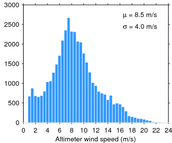
Figure 33. Histogram of flag-valid wind over oceans and lakes for 03/07/2016. The mean ( \mu ) and standard deviation ( \sigma ) are also shown. Note that values larger than 24 m/s are excluded from the histogram for the sake of readability but not from the computation of \mu and \sigma .
