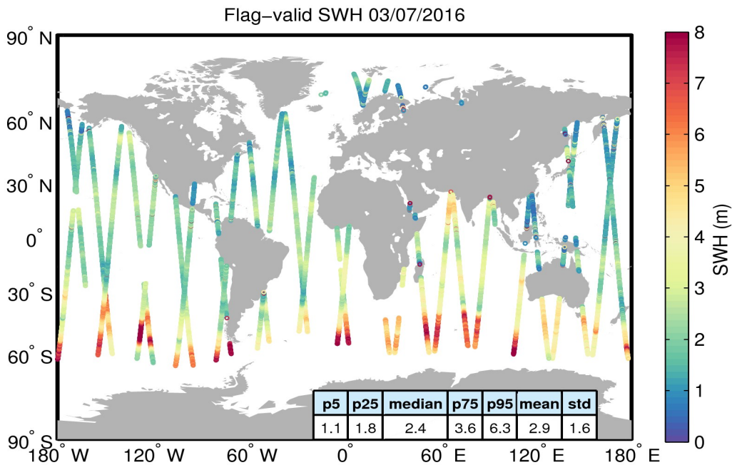
Figure 15. Geographical distribution of flag-valid SWH data over oceans and lakes for 03/07/2016. The statistical values shown in the table refer to the SWH in m and are calculated over all measurements shown in the figure.
