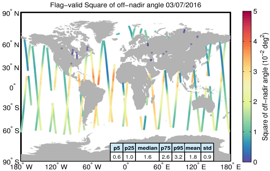
Figure 37. Geographical distribution of flag-valid mispointing data over oceans and lakes for 03/07/2016. The statistical values shown in the table refer to the mispointing in 10^{-2} \text{ deg}^2 and are calculated over all measurements shown in the figure.
