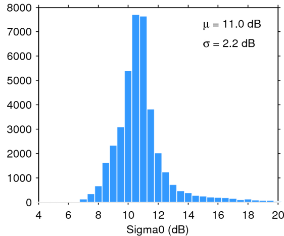
Figure 25. Histogram of flag-valid sigma0 over oceans and lakes for 03/07/2016. The mean ( \mu ) and standard deviation ( \sigma ) are also shown. Note that values outside [4 20] dB are excluded from the histogram for the sake of readability but not from the computation of \mu and \sigma .
