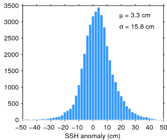
Figure 7. Histogram of flag-valid SSH anomaly over oceans and lakes for 03/07/2016. The mean ( \mu ) and standard deviation ( \sigma ) are also shown. Note that values outside [-50 50] cm are excluded from the histogram for the sake of readability but not from the computation of \mu and \sigma .
