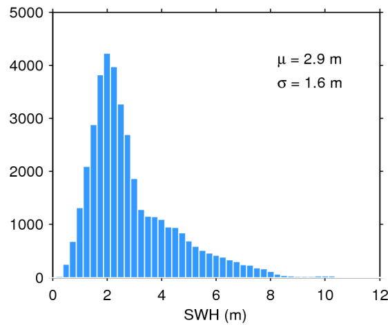
Figure 17. Histogram of flag-valid SWH over oceans and lakes for 03/07/2016. The mean ( \mu ) and standard deviation ( \sigma ) are also shown. Note that values larger than 12 m are excluded from the histogram for the sake of readability but not from the computation of \mu and \sigma .
