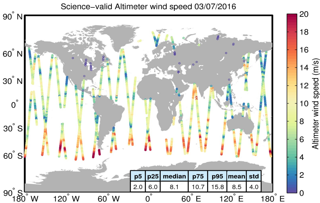
Figure 34. Geographical distribution of science-valid wind data over oceans and lakes for 03/07/2016. The statistical values shown in the table refer to the wind in m/s and are calculated over all measurements shown in the figure. Gray circles denote records that have been rejected based on the editing criteria described in Table 5.
