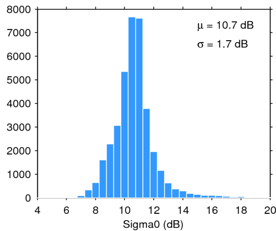
Figure 28. Histogram of science-valid sigma0 over oceans and lakes for 03/07/2016. The mean ( \mu ) and standard deviation ( \sigma ) are also shown. Note that values outside [4 20] dB are excluded from the histogram for the sake of readability but not from the computation of \mu and \sigma .
