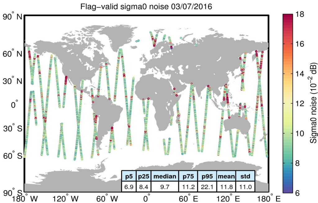
Figure 26. Geographical distribution of flag-valid 20-Hz sigma0 measurement noise over oceans and lakes for 03/07/2016. The statistical values shown in the table refer to the sigma0 noise and are calculated over all measurements shown in the figure.
