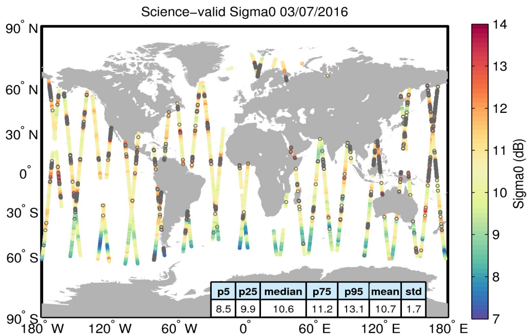
Figure 27. Geographical distribution of science-valid sigma0 data over oceans and lakes for 03/07/2016. The statistical values shown in the table refer to the sigma0 in dB and are calculated over all measurements shown in the figure. Gray circles denote records that have been rejected based on the editing criteria described in Table 4.
