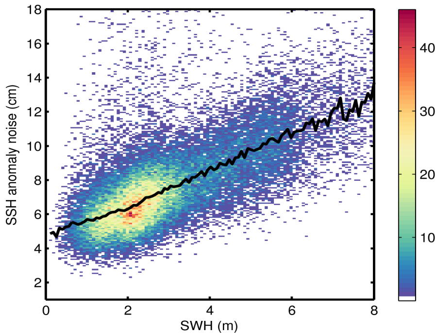
Figure 9. 2D histogram showing flag-valid SSH anomaly noise as a function of SWH for 02/07/2016. The black line denotes the median SSH anomaly noise as a function of SWH.
