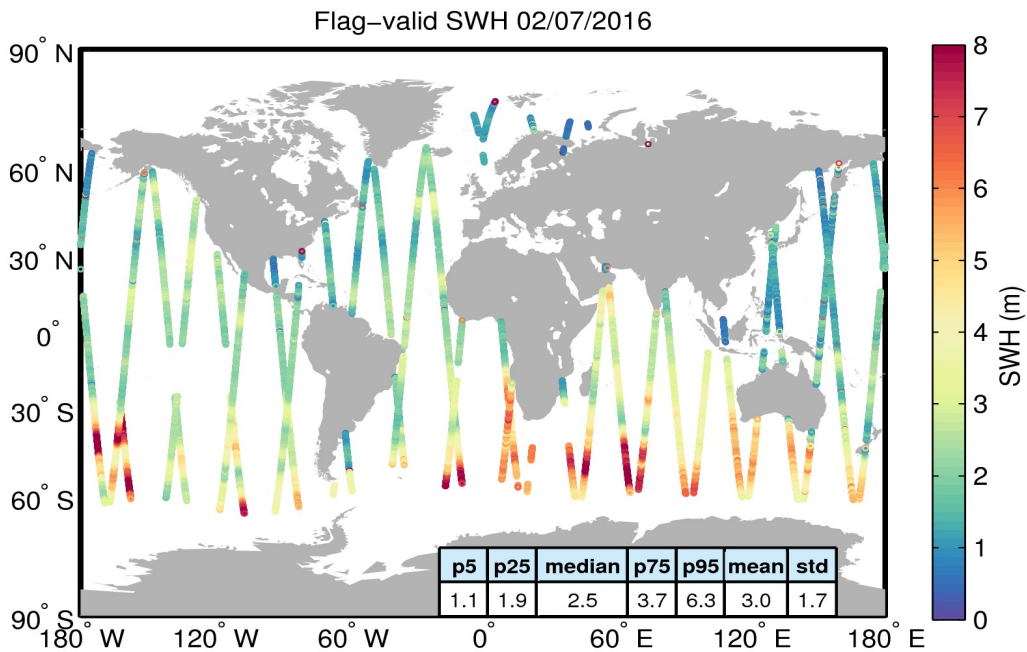
Figure 15. Geographical distribution of flag-valid SWH data over oceans and lakes for 02/07/2016. The statistical values shown in the table refer to the SWH in m and are calculated over all measurements shown in the figure.
