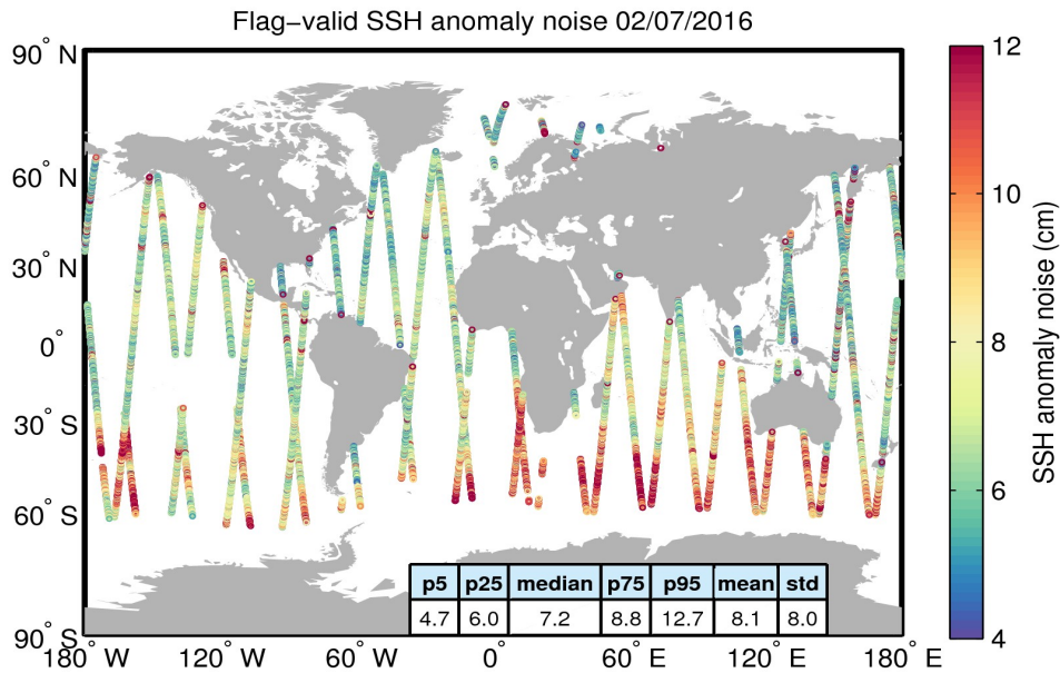
Figure 8. Geographical distribution of flag-valid 20-Hz SSH anomaly measurement noise over oceans and lakes for 02/07/2016. The statistical values shown in the table refer to the SSH anomaly noise and are calculated over all measurements shown in the figure.
