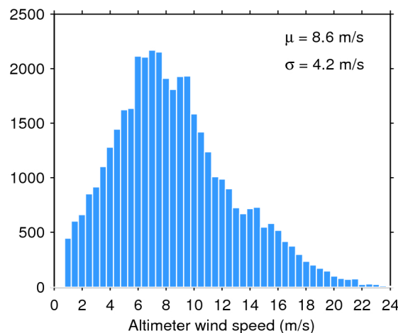
Figure 35. Histogram of science-valid wind over oceans and lakes for 02/07/2016. The mean ( \mu ) and standard deviation ( \sigma ) are also shown. Note that values larger than 24 m/s are excluded from the histogram for the sake of readability but not from the computation of \mu and \sigma .
