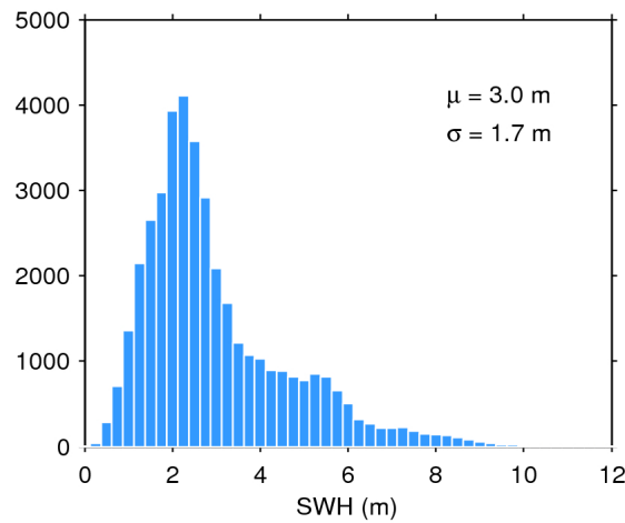
Figure 17. Histogram of flag-valid SWH over oceans and lakes for 02/07/2016. The mean ( \mu ) and standard deviation ( \sigma ) are also shown. Note that values larger than 12 m are excluded from the histogram for the sake of readability but not from the computation of \mu and \sigma .
