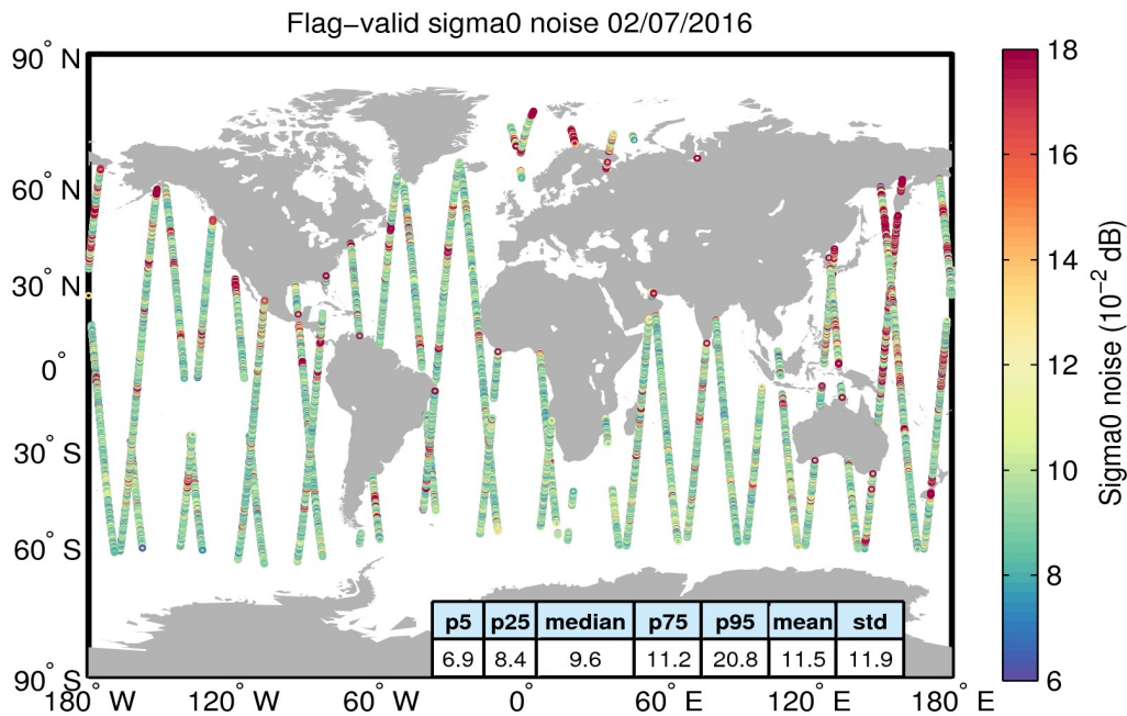
Figure 26. Geographical distribution of flag-valid 20-Hz sigma0 measurement noise over oceans and lakes for 02/07/2016. The statistical values shown in the table refer to the sigma0 noise and are calculated over all measurements shown in the figure.
