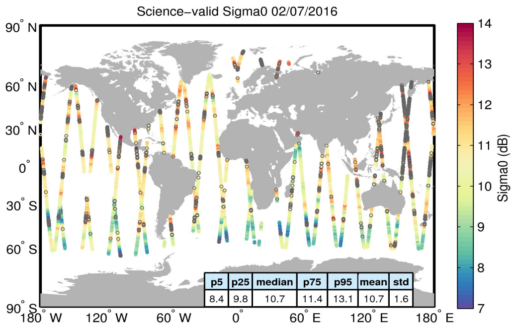
Figure 27. Geographical distribution of science-valid sigma0 data over oceans and lakes for 02/07/2016. The statistical values shown in the table refer to the sigma0 in dB and are calculated over all measurements shown in the figure. Gray circles denote records that have been rejected based on the editing criteria described in Table 4.
