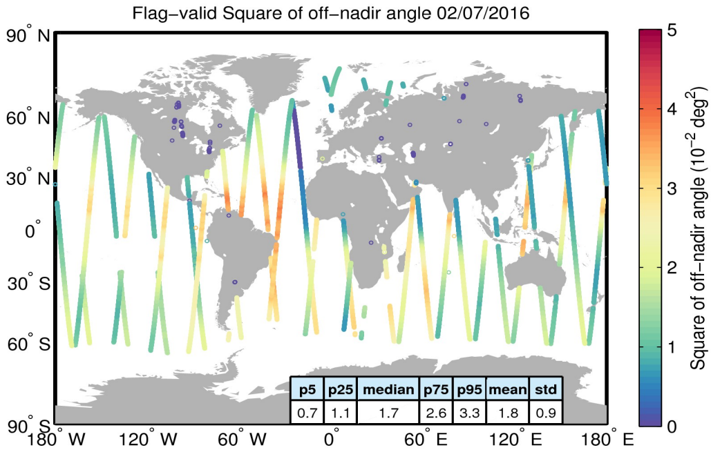
Figure 37. Geographical distribution of flag-valid mispointing data over oceans and lakes for 02/07/2016. The statistical values shown in the table refer to the mispointing in 10^{-2} \text{ deg}^2 and are calculated over all measurements shown in the figure.
