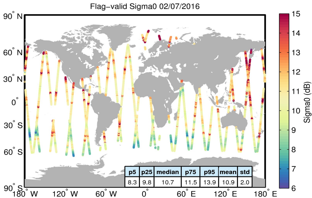
Figure 23. Geographical distribution of flag-valid sigma0 data over oceans and lakes for 02/07/2016. The statistical values shown in the table refer to the sigma0 in dB and are calculated over all measurements shown in the figure.
