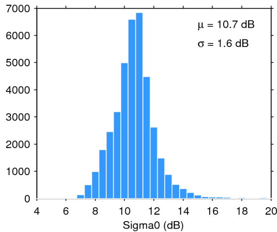
Figure 28. Histogram of science-valid sigma0 over oceans and lakes for 02/07/2016. The mean ( \mu ) and standard deviation ( \sigma ) are also shown. Note that values outside [4 20] dB are excluded from the histogram for the sake of readability but not from the computation of \mu and \sigma .
