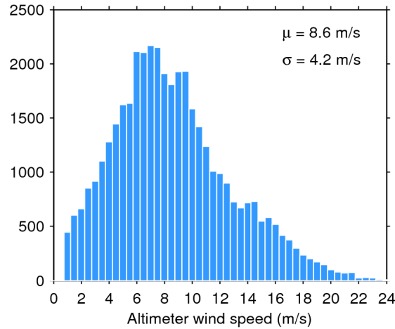
Figure 33. Histogram of flag-valid wind over oceans and lakes for 02/07/2016. The mean ( \mu ) and standard deviation ( \sigma ) are also shown. Note that values larger than 24 m/s are excluded from the histogram for the sake of readability but not from the computation of \mu and \sigma .
