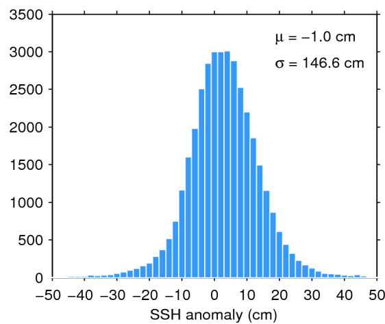
Figure 7. Histogram of flag-valid SSH anomaly over oceans and lakes for 02/07/2016. The mean ( \mu ) and standard deviation ( \sigma ) are also shown. Note that values outside [-50 50] cm are excluded from the histogram for the sake of readability but not from the computation of \mu and \sigma .
