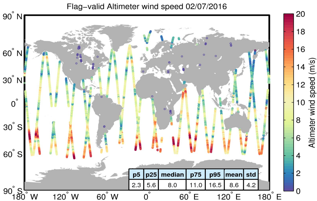
Figure 31. Geographical distribution of flag-valid wind data over oceans and lakes for 02/07/2016. The statistical values shown in the table refer to the wind in m/s and are calculated over all measurements shown in the figure.
