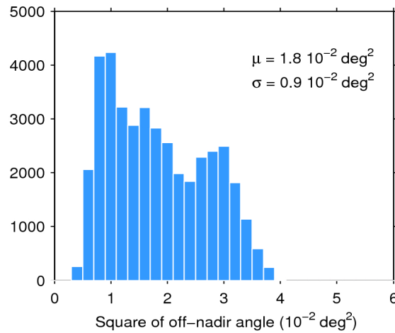
Figure 39. Histogram of flag-valid mispointing over oceans and lakes for 02/07/2016. The mean ( \mu ) and standard deviation ( \sigma ) are also shown. Note that values larger than 6 \cdot 10^{-2} \text{ deg}^2 are excluded from the histogram for the sake of readability but not from the computation of \mu and \sigma .
