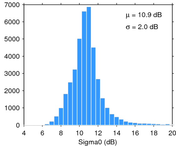
Figure 25. Histogram of flag-valid sigma0 over oceans and lakes for 02/07/2016. The mean ( \mu ) and standard deviation ( \sigma ) are also shown. Note that values outside [4 20] dB are excluded from the histogram for the sake of readability but not from the computation of \mu and \sigma .
