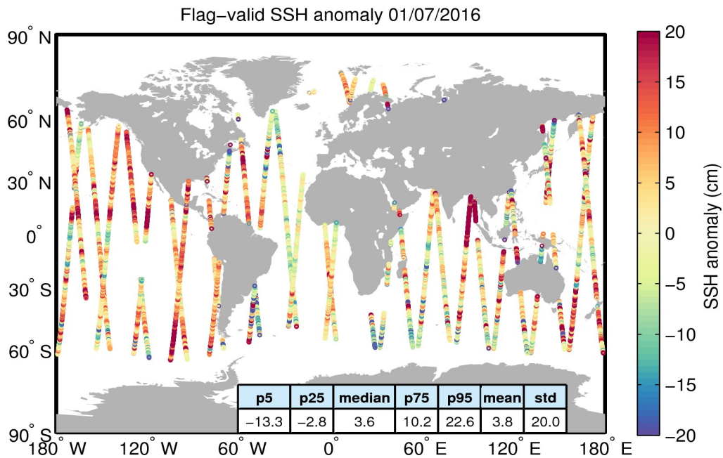
Figure 5. Geographical distribution of flag-valid 1-Hz SSH anomaly data over oceans and lakes for 01/07/2016. The statistical values shown in the table refer to the SSH anomaly in cm and are calculated over all measurements shown in the figure.
