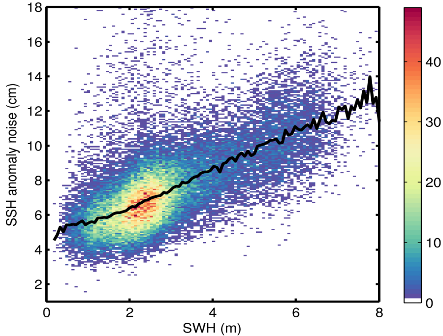
Figure 9. 2D histogram showing flag-valid SSH anomaly noise as a function of SWH for 01/07/2016. The black line denotes the median SSH anomaly noise as a function of SWH.
