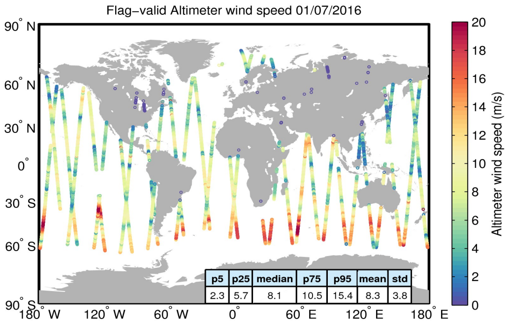
Figure 31. Geographical distribution of flag-valid wind data over oceans and lakes for 01/07/2016. The statistical values shown in the table refer to the wind in m/s and are calculated over all measurements shown in the figure.
