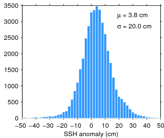
Figure 7. Histogram of flag-valid SSH anomaly over oceans and lakes for 01/07/2016. The mean ( \mu ) and standard deviation ( \sigma ) are also shown. Note that values outside [-50 50] cm are excluded from the histogram for the sake of readability but not from the computation of \mu and \sigma .
