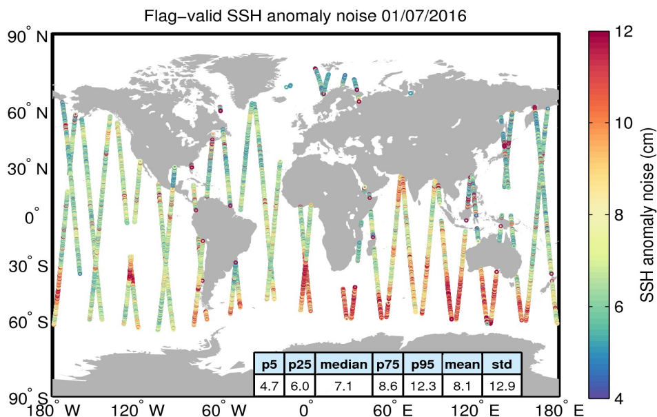
Figure 8. Geographical distribution of flag-valid 20-Hz SSH anomaly measurement noise over oceans and lakes for 01/07/2016. The statistical values shown in the table refer to the SSH anomaly noise and are calculated over all measurements shown in the figure.
