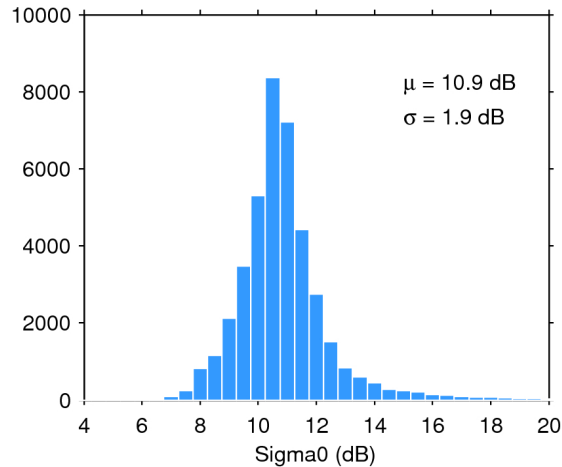
Figure 25. Histogram of flag-valid sigma0 over oceans and lakes for 01/07/2016. The mean ( \mu ) and standard deviation ( \sigma ) are also shown. Note that values outside [4 20] dB are excluded from the histogram for the sake of readability but not from the computation of \mu and \sigma .
