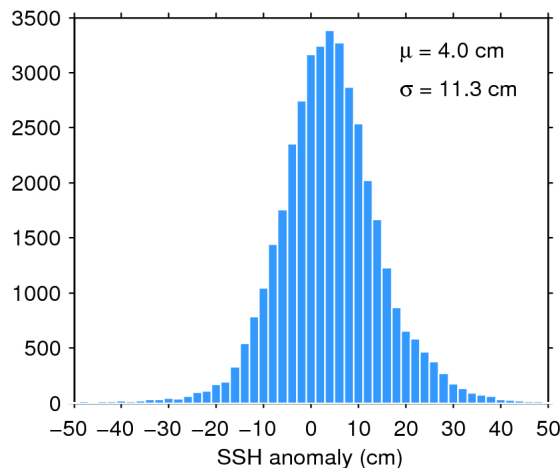
Figure 11. Histogram of science-valid SSH anomaly over oceans and lakes for 01/07/2016. The mean ( \mu ) and standard deviation ( \sigma ) are also shown. Note that values outside [-50 50] cm are excluded from the histogram for the sake of readability but not from the computation of \mu and \sigma .
