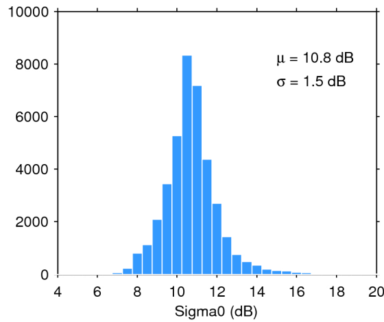
Figure 28. Histogram of science-valid sigma0 over oceans and lakes for 01/07/2016. The mean ( \mu ) and standard deviation ( \sigma ) are also shown. Note that values outside [4 20] dB are excluded from the histogram for the sake of readability but not from the computation of \mu and \sigma .
