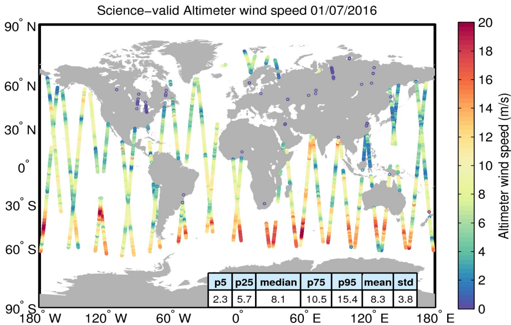
Figure 34. Geographical distribution of science-valid wind data over oceans and lakes for 01/07/2016. The statistical values shown in the table refer to the wind in m/s and are calculated over all measurements shown in the figure. Gray circles denote records that have been rejected based on the editing criteria described in Table 5.
