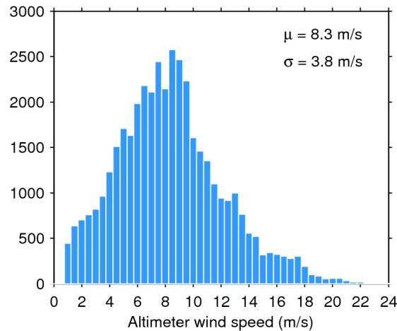
Figure 33. Histogram of flag-valid wind over oceans and lakes for 01/07/2016. The mean ( \mu ) and standard deviation ( \sigma ) are also shown. Note that values larger than 24 m/s are excluded from the histogram for the sake of readability but not from the computation of \mu and \sigma .
