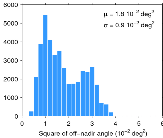
Figure 39. Histogram of flag-valid mispointing over oceans and lakes for 01/07/2016. The mean ( \mu ) and standard deviation ( \sigma ) are also shown. Note that values larger than 6 \cdot 10^{-2} \text{ deg}^2 are excluded from the histogram for the sake of readability but not from the computation of \mu and \sigma .
