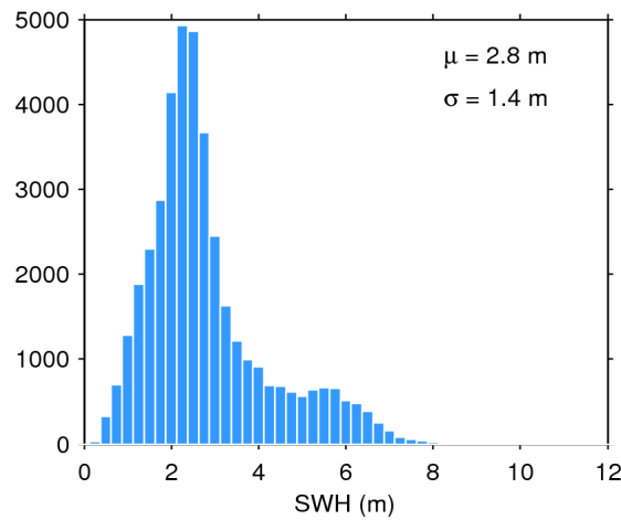
Figure 17. Histogram of flag-valid SWH over oceans and lakes for 01/07/2016. The mean ( \mu ) and standard deviation ( \sigma ) are also shown. Note that values larger than 12 m are excluded from the histogram for the sake of readability but not from the computation of \mu and \sigma .
