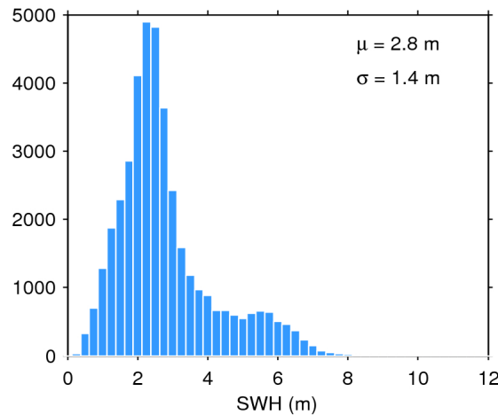
Figure 20. Histogram of science-valid SWH over oceans and lakes for 01/07/2016. The mean ( \mu ) and standard deviation ( \sigma ) are also shown. Note that values larger than 12 m are excluded from the histogram for the sake of readability but not from the computation of \mu and \sigma .
