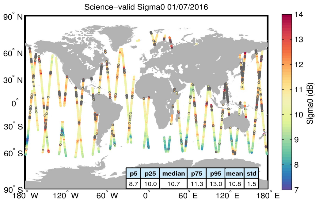
Figure 27. Geographical distribution of science-valid sigma0 data over oceans and lakes for 01/07/2016. The statistical values shown in the table refer to the sigma0 in dB and are calculated over all measurements shown in the figure. Gray circles denote records that have been rejected based on the editing criteria described in Table 4.
