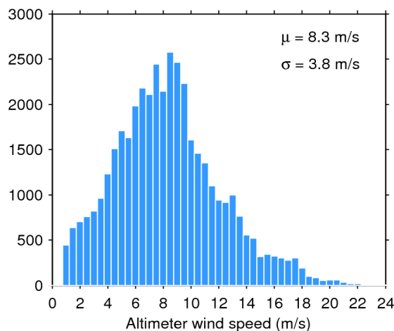
Figure 35. Histogram of science-valid wind over oceans and lakes for 01/07/2016. The mean ( \mu ) and standard deviation ( \sigma ) are also shown. Note that values larger than 24 m/s are excluded from the histogram for the sake of readability but not from the computation of \mu and \sigma .
