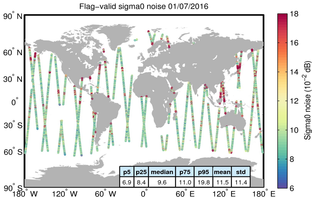
Figure 26. Geographical distribution of flag-valid 20-Hz sigma0 measurement noise over oceans and lakes for 01/07/2016. The statistical values shown in the table refer to the sigma0 noise and are calculated over all measurements shown in the figure.
