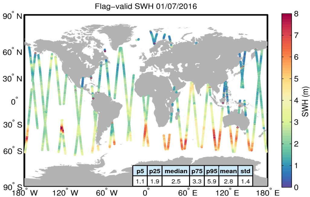
Figure 15. Geographical distribution of flag-valid SWH data over oceans and lakes for 01/07/2016. The statistical values shown in the table refer to the SWH in m and are calculated over all measurements shown in the figure.
