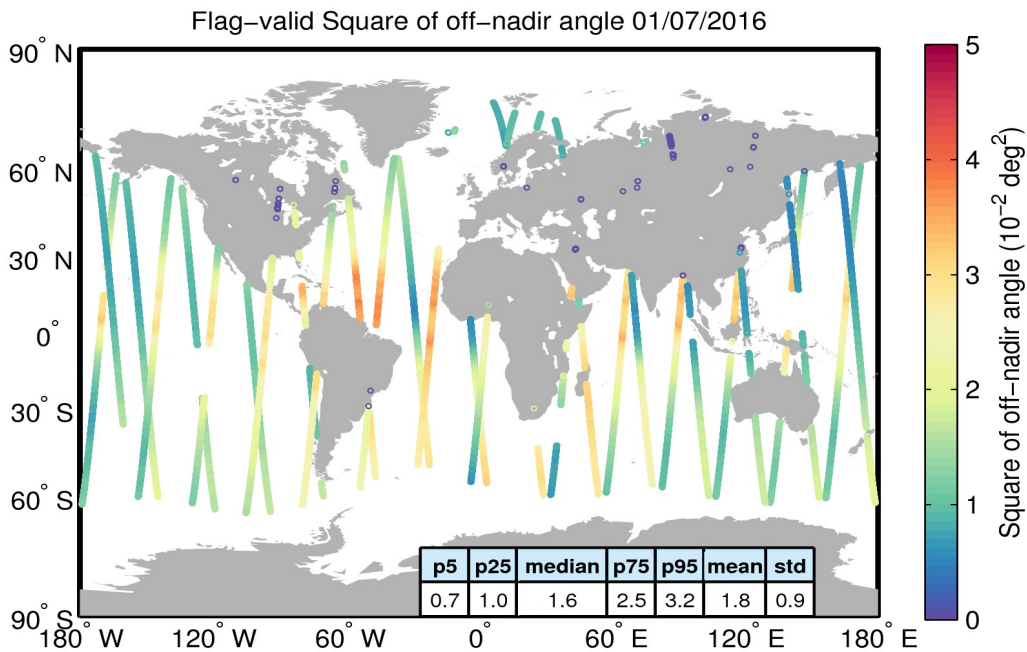
Figure 37. Geographical distribution of flag-valid mispointing data over oceans and lakes for 01/07/2016. The statistical values shown in the table refer to the mispointing in 10^{-2} \text{deg}^2 and are calculated over all measurements shown in the figure.
