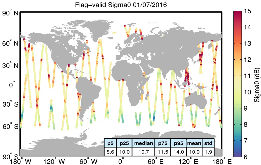
Figure 23. Geographical distribution of flag-valid sigma0 data over oceans and lakes for 01/07/2016. The statistical values shown in the table refer to the sigma0 in dB and are calculated over all measurements shown in the figure.
