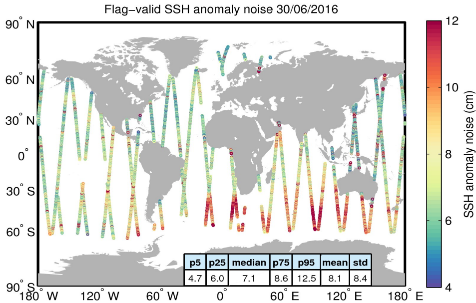
Figure 8. Geographical distribution of flag-valid 20-Hz SSH anomaly measurement noise over oceans and lakes for 30/06/2016. The statistical values shown in the table refer to the SSH anomaly noise and are calculated over all measurements shown in the figure.
