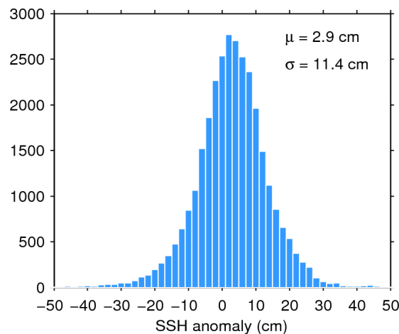
Figure 11. Histogram of science-valid SSH anomaly over oceans and lakes for 30/06/2016. The mean ( \mu ) and standard deviation ( \sigma ) are also shown. Note that values outside [-50 50] cm are excluded from the histogram for the sake of readability but not from the computation of \mu and \sigma .
