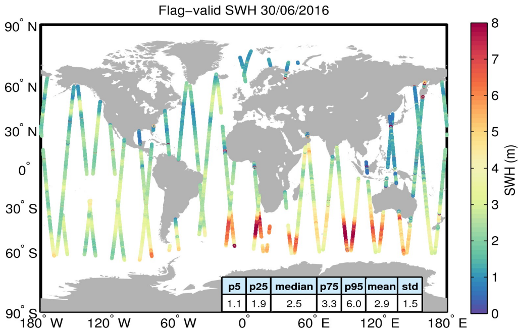
Figure 15. Geographical distribution of flag-valid SWH data over oceans and lakes for 30/06/2016. The statistical values shown in the table refer to the SWH in m and are calculated over all measurements shown in the figure.
