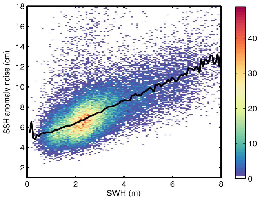
Figure 9. 2D histogram showing flag-valid SSH anomaly noise as a function of SWH for 30/06/2016. The black line denotes the median SSH anomaly noise as a function of SWH.
