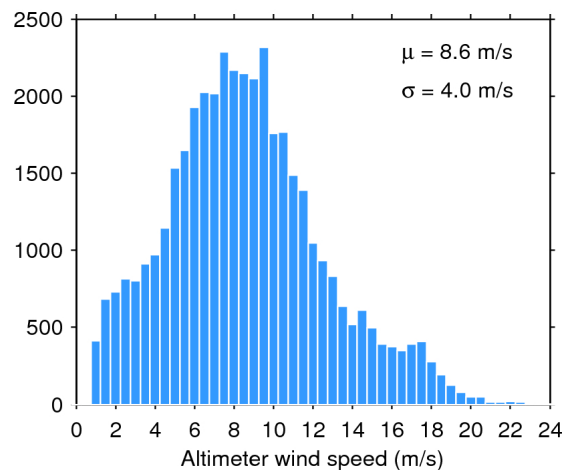
Figure 35. Histogram of science-valid wind over oceans and lakes for 30/06/2016. The mean ( \mu ) and standard deviation ( \sigma ) are also shown. Note that values larger than 24 m/s are excluded from the histogram for the sake of readability but not from the computation of \mu and \sigma .
