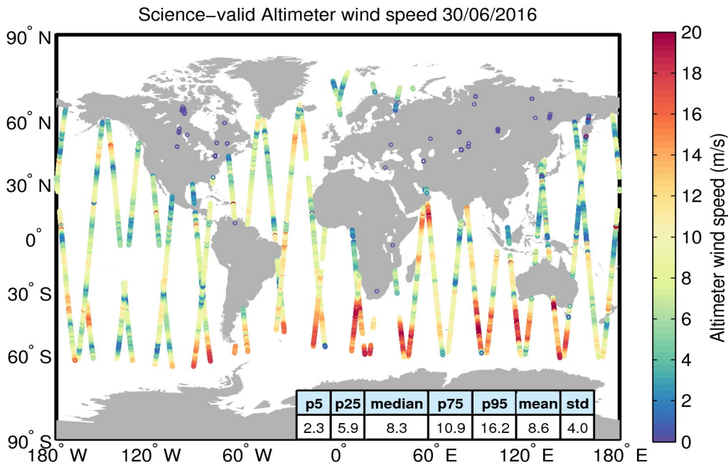
Figure 34. Geographical distribution of science-valid wind data over oceans and lakes for 30/06/2016. The statistical values shown in the table refer to the wind in m/s and are calculated over all measurements shown in the figure. Gray circles denote records that have been rejected based on the editing criteria described in Table 5.
