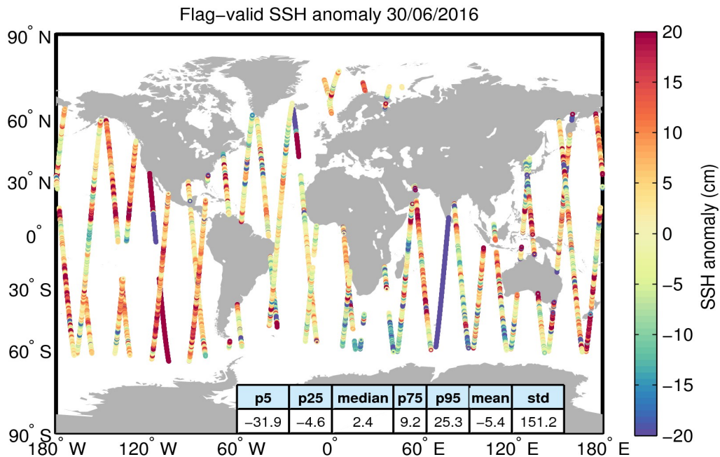
Figure 5. Geographical distribution of flag-valid 1-Hz SSH anomaly data over oceans and lakes for 30/06/2016. The statistical values shown in the table refer to the SSH anomaly in cm and are calculated over all measurements shown in the figure.
