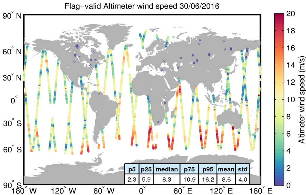
Figure 31. Geographical distribution of flag-valid wind data over oceans and lakes for 30/06/2016. The statistical values shown in the table refer to the wind in m/s and are calculated over all measurements shown in the figure.
