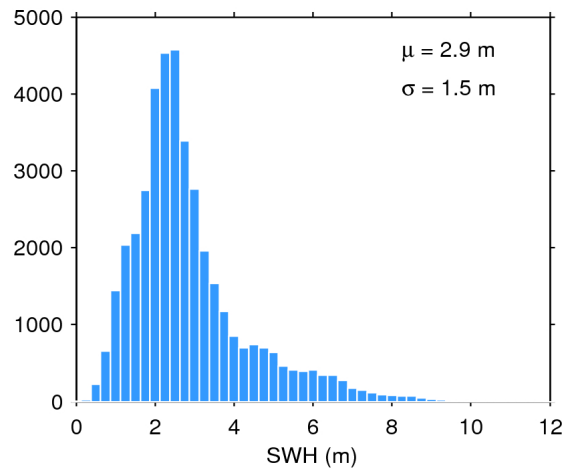
Figure 17. Histogram of flag-valid SWH over oceans and lakes for 30/06/2016. The mean ( \mu ) and standard deviation ( \sigma ) are also shown. Note that values larger than 12 m are excluded from the histogram for the sake of readability but not from the computation of \mu and \sigma .
