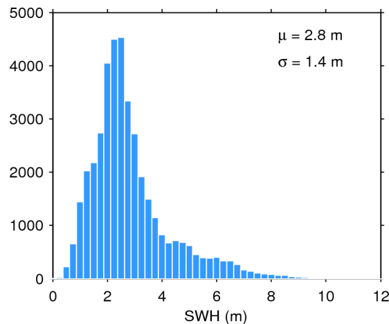
Figure 20. Histogram of science-valid SWH over oceans and lakes for 30/06/2016. The mean ( \mu ) and standard deviation ( \sigma ) are also shown. Note that values larger than 12 m are excluded from the histogram for the sake of readability but not from the computation of \mu and \sigma .
