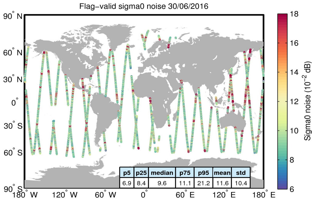
Figure 26. Geographical distribution of flag-valid 20-Hz sigma0 measurement noise over oceans and lakes for 30/06/2016. The statistical values shown in the table refer to the sigma0 noise and are calculated over all measurements shown in the figure.
