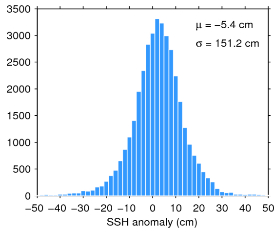
Figure 7. Histogram of flag-valid SSH anomaly over oceans and lakes for 30/06/2016. The mean ( \mu ) and standard deviation ( \sigma ) are also shown. Note that values outside [-50 50] cm are excluded from the histogram for the sake of readability but not from the computation of \mu and \sigma .
