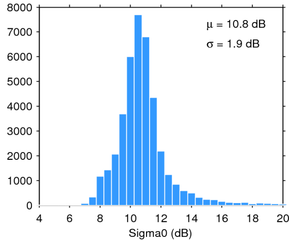
Figure 25. Histogram of flag-valid sigma0 over oceans and lakes for 30/06/2016. The mean ( \mu ) and standard deviation ( \sigma ) are also shown. Note that values outside [4 20] dB are excluded from the histogram for the sake of readability but not from the computation of \mu and \sigma .
