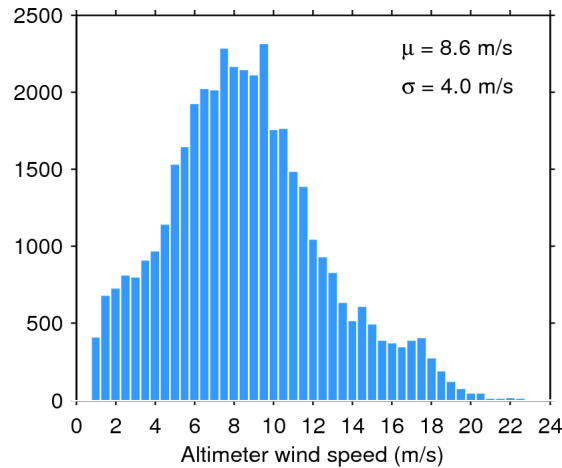
Figure 33. Histogram of flag-valid wind over oceans and lakes for 30/06/2016. The mean ( \mu ) and standard deviation ( \sigma ) are also shown. Note that values larger than 24 m/s are excluded from the histogram for the sake of readability but not from the computation of \mu and \sigma .
