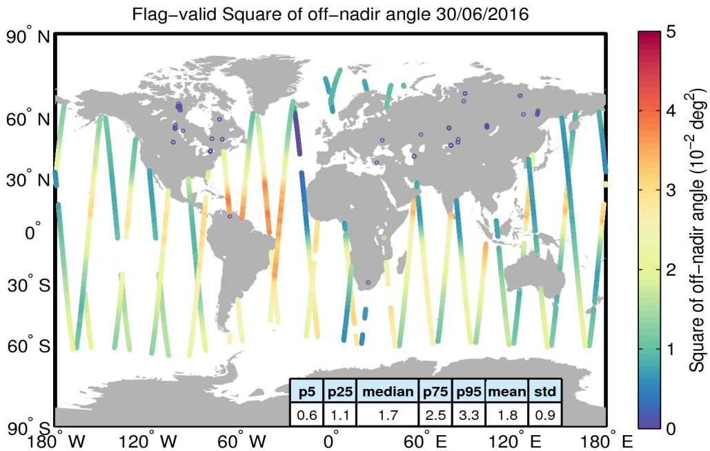
Figure 37. Geographical distribution of flag-valid mispointing data over oceans and lakes for 30/06/2016. The statistical values shown in the table refer to the mispointing in 10^{-2} deg 2 and are calculated over all measurements shown in the figure.
