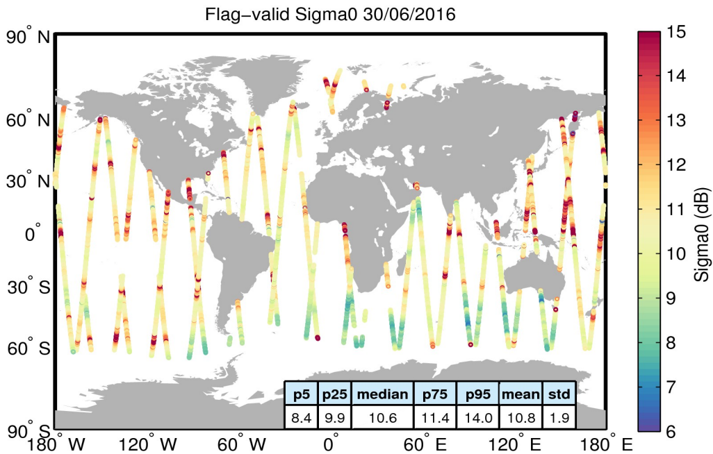
Figure 23. Geographical distribution of flag-valid sigma0 data over oceans and lakes for 30/06/2016. The statistical values shown in the table refer to the sigma0 in dB and are calculated over all measurements shown in the figure.
