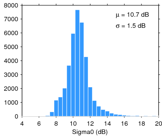
Figure 28. Histogram of science-valid sigma0 over oceans and lakes for 30/06/2016. The mean ( \mu ) and standard deviation ( \sigma ) are also shown. Note that values outside [4 20] dB are excluded from the histogram for the sake of readability but not from the computation of \mu and \sigma .
