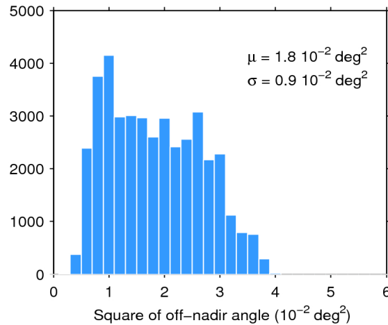
Figure 39. Histogram of flag-valid mispointing over oceans and lakes for 30/06/2016. The mean ( \mu ) and standard deviation ( \sigma ) are also shown. Note that values larger than 6 \cdot 10^{-2} \text{ deg}^2 are excluded from the histogram for the sake of readability but not from the computation of \mu and \sigma .
