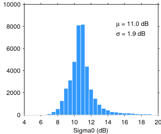
Figure 25. Histogram of flag-valid sigma0 over oceans and lakes for 28/06/2016. The mean ( \mu ) and standard deviation ( \sigma ) are also shown. Note that values outside [4 20] dB are excluded from the histogram for the sake of readability but not from the computation of \mu and \sigma .
