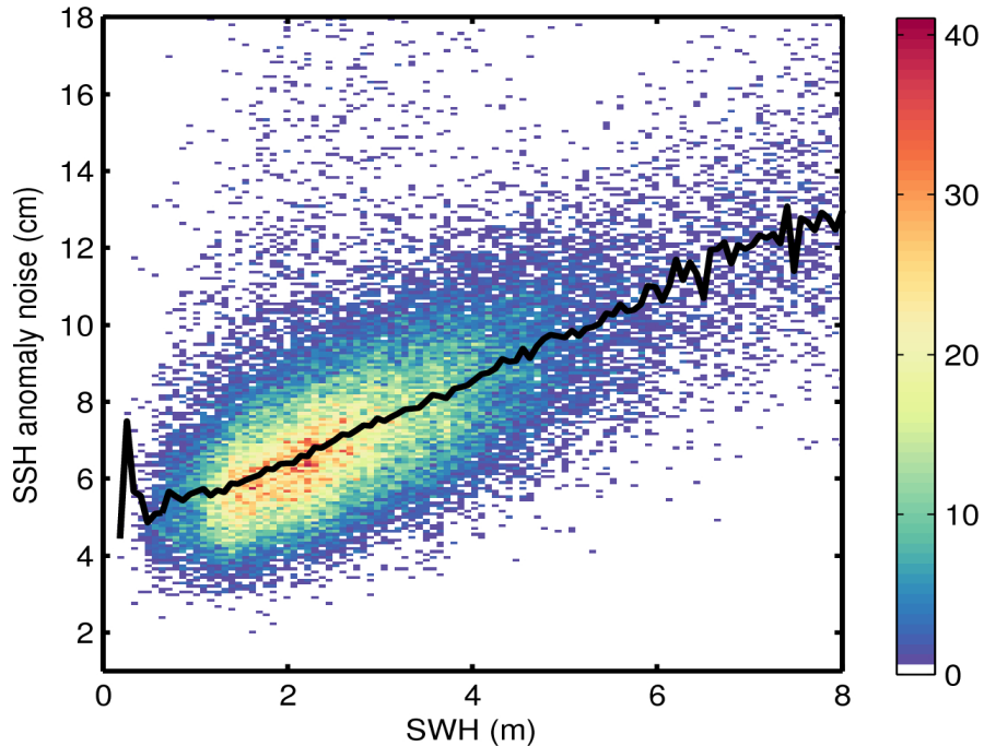
Figure 9. 2D histogram showing flag-valid SSH anomaly noise as a function of SWH for 28/06/2016. The black line denotes the median SSH anomaly noise as a function of SWH.
