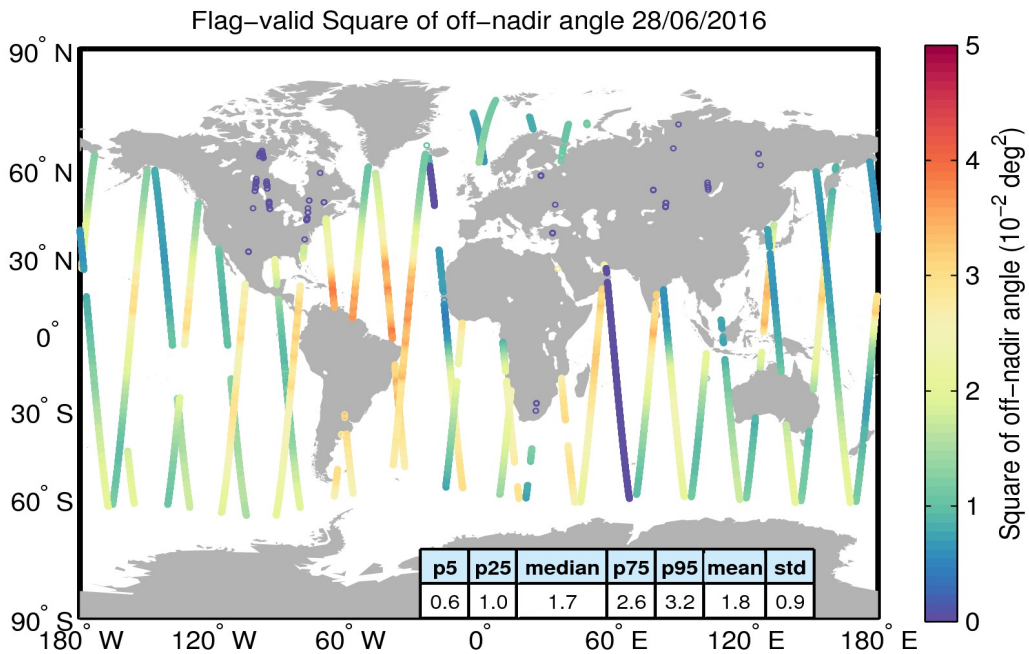
Figure 37. Geographical distribution of flag-valid mispointing data over oceans and lakes for 28/06/2016. The statistical values shown in the table refer to the mispointing in 10^{-2} deg 2 and are calculated over all measurements shown in the figure.
