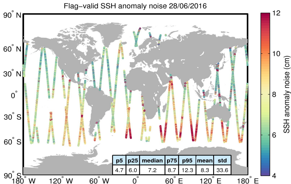
Figure 8. Geographical distribution of flag-valid 20-Hz SSH anomaly measurement noise over oceans and lakes for 28/06/2016. The statistical values shown in the table refer to the SSH anomaly noise and are calculated over all measurements shown in the figure.
