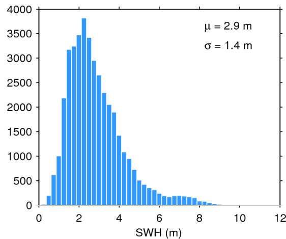
Figure 17. Histogram of flag-valid SWH over oceans and lakes for 28/06/2016. The mean ( \mu ) and standard deviation ( \sigma ) are also shown. Note that values larger than 12 m are excluded from the histogram for the sake of readability but not from the computation of \mu and \sigma .
