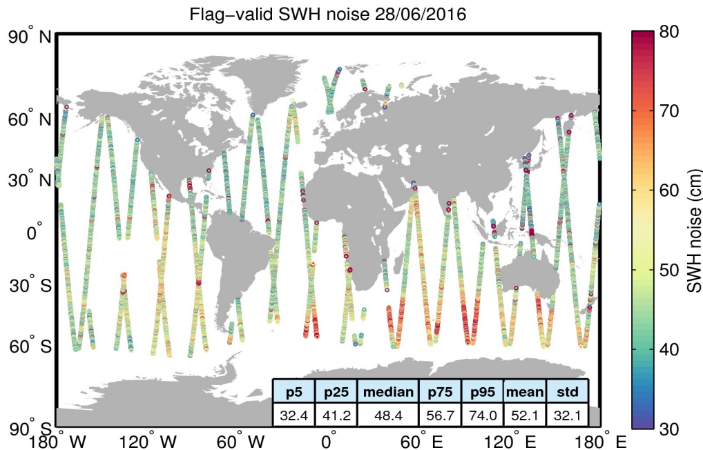
Figure 18. Geographical distribution of flag-valid 20-Hz SWH measurement noise over oceans and lakes for 28/06/2016. The statistical values shown in the table refer to the SWH noise and are calculated over all measurements shown in the figure.
