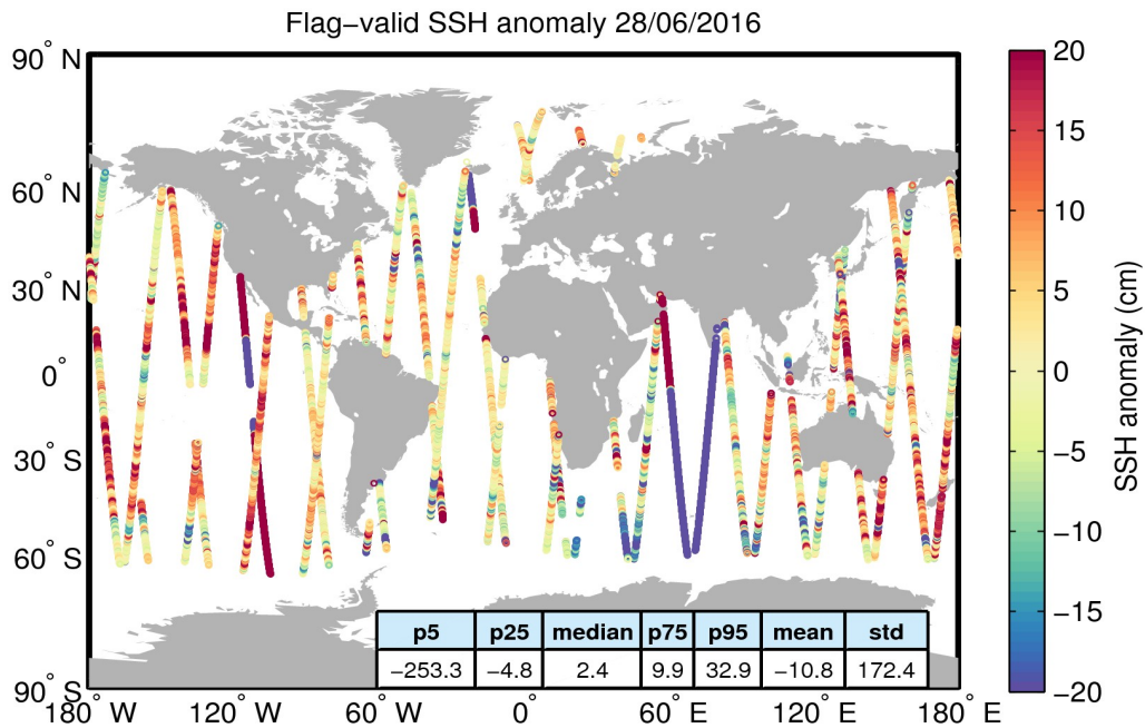
Figure 5. Geographical distribution of flag-valid 1-Hz SSH anomaly data over oceans and lakes for 28/06/2016. The statistical values shown in the table refer to the SSH anomaly in cm and are calculated over all measurements shown in the figure.
