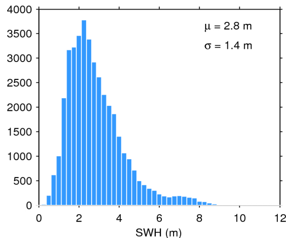
Figure 20. Histogram of science-valid SWH over oceans and lakes for 28/06/2016. The mean ( \mu ) and standard deviation ( \sigma ) are also shown. Note that values larger than 12 m are excluded from the histogram for the sake of readability but not from the computation of \mu and \sigma .
