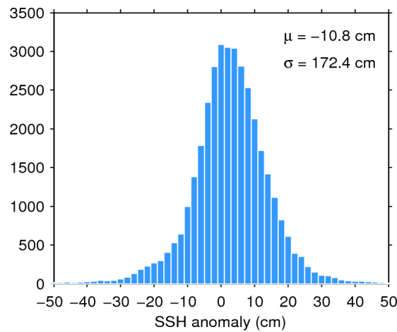
Figure 7. Histogram of flag-valid SSH anomaly over oceans and lakes for 28/06/2016. The mean ( \mu ) and standard deviation ( \sigma ) are also shown. Note that values outside [-50 50] cm are excluded from the histogram for the sake of readability but not from the computation of \mu and \sigma .
