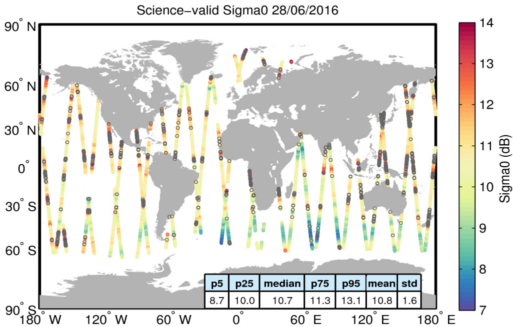
Figure 27. Geographical distribution of science-valid sigma0 data over oceans and lakes for 28/06/2016. The statistical values shown in the table refer to the sigma0 in dB and are calculated over all measurements shown in the figure. Gray circles denote records that have been rejected based on the editing criteria described in Table 4.
