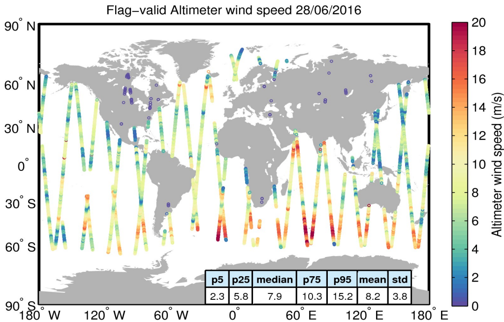
Figure 31. Geographical distribution of flag-valid wind data over oceans and lakes for 28/06/2016. The statistical values shown in the table refer to the wind in m/s and are calculated over all measurements shown in the figure.
