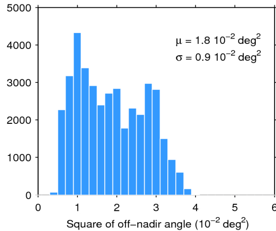
Figure 39. Histogram of flag-valid mispointing over oceans and lakes for 28/06/2016. The mean ( \mu ) and standard deviation ( \sigma ) are also shown. Note that values larger than 6 \cdot 10^{-2} \text{ deg}^2 are excluded from the histogram for the sake of readability but not from the computation of \mu and \sigma .
