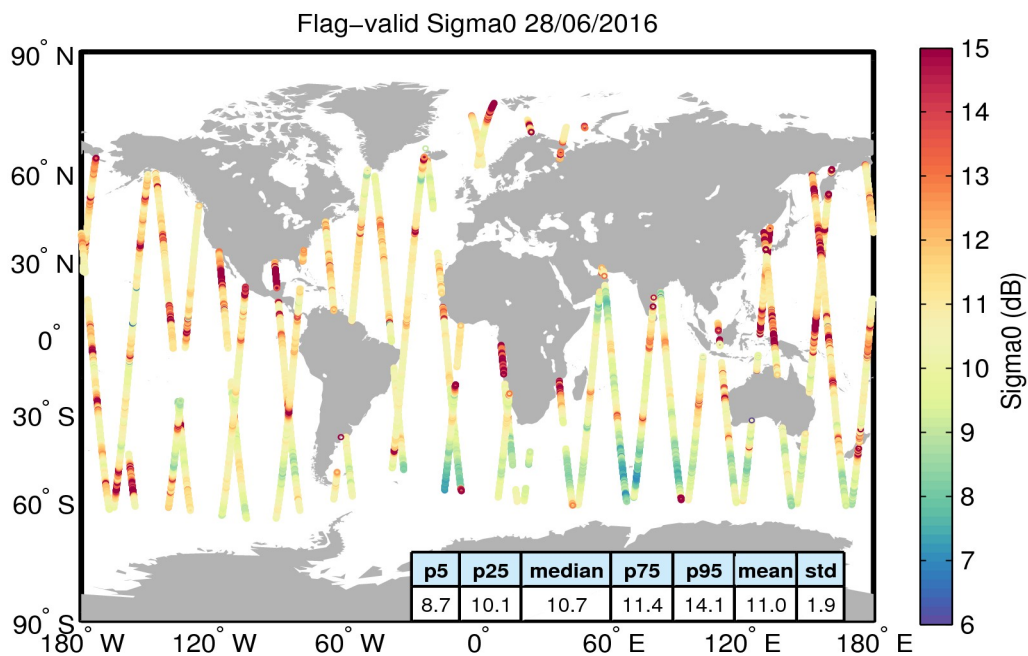
Figure 23. Geographical distribution of flag-valid sigma0 data over oceans and lakes for 28/06/2016. The statistical values shown in the table refer to the sigma0 in dB and are calculated over all measurements shown in the figure.
