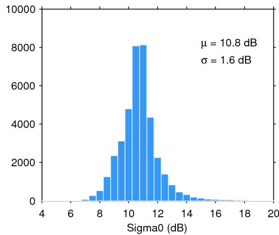
Figure 28. Histogram of science-valid sigma0 over oceans and lakes for 28/06/2016. The mean ( \mu ) and standard deviation ( \sigma ) are also shown. Note that values outside [4 20] dB are excluded from the histogram for the sake of readability but not from the computation of \mu and \sigma .
