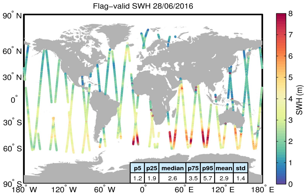
Figure 15. Geographical distribution of flag-valid SWH data over oceans and lakes for 28/06/2016. The statistical values shown in the table refer to the SWH in m and are calculated over all measurements shown in the figure.
