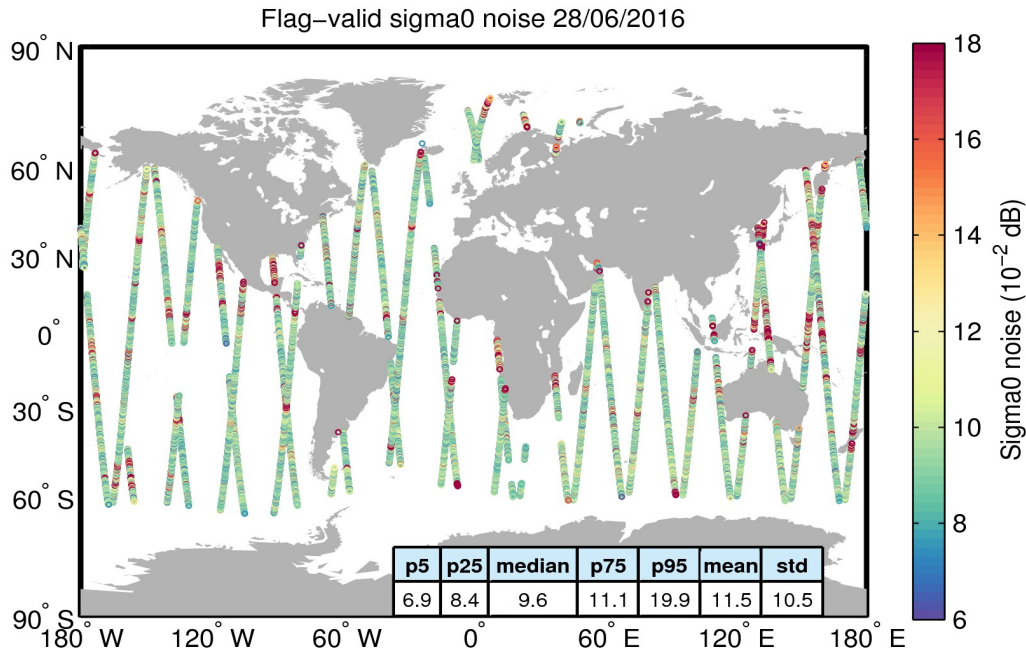
Figure 26. Geographical distribution of flag-valid 20-Hz sigma0 measurement noise over oceans and lakes for 28/06/2016. The statistical values shown in the table refer to the sigma0 noise and are calculated over all measurements shown in the figure.
