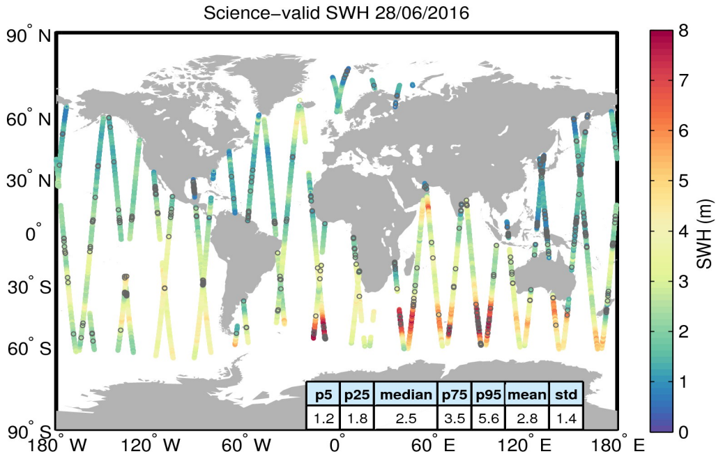
Figure 19. Geographical distribution of science-valid SWH data over oceans and lakes for 28/06/2016. The statistical values shown in the table refer to the SWH in m and are calculated over all measurements shown in the figure. Gray circles denote records that have been rejected based on the editing criteria described in Table 3.
