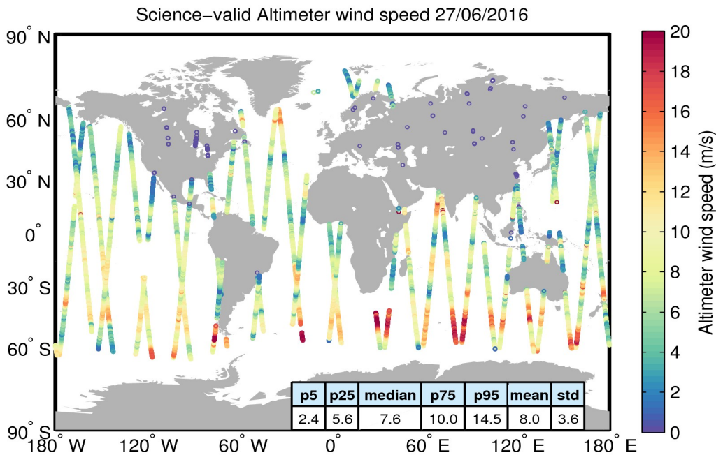
Figure 34. Geographical distribution of science-valid wind data over oceans and lakes for 27/06/2016. The statistical values shown in the table refer to the wind in m/s and are calculated over all measurements shown in the figure. Gray circles denote records that have been rejected based on the editing criteria described in Table 5.
