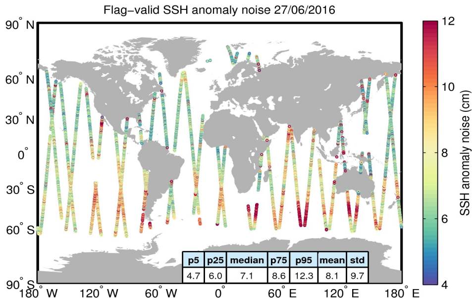
Figure 8. Geographical distribution of flag-valid 20-Hz SSH anomaly measurement noise over oceans and lakes for 27/06/2016. The statistical values shown in the table refer to the SSH anomaly noise and are calculated over all measurements shown in the figure.
