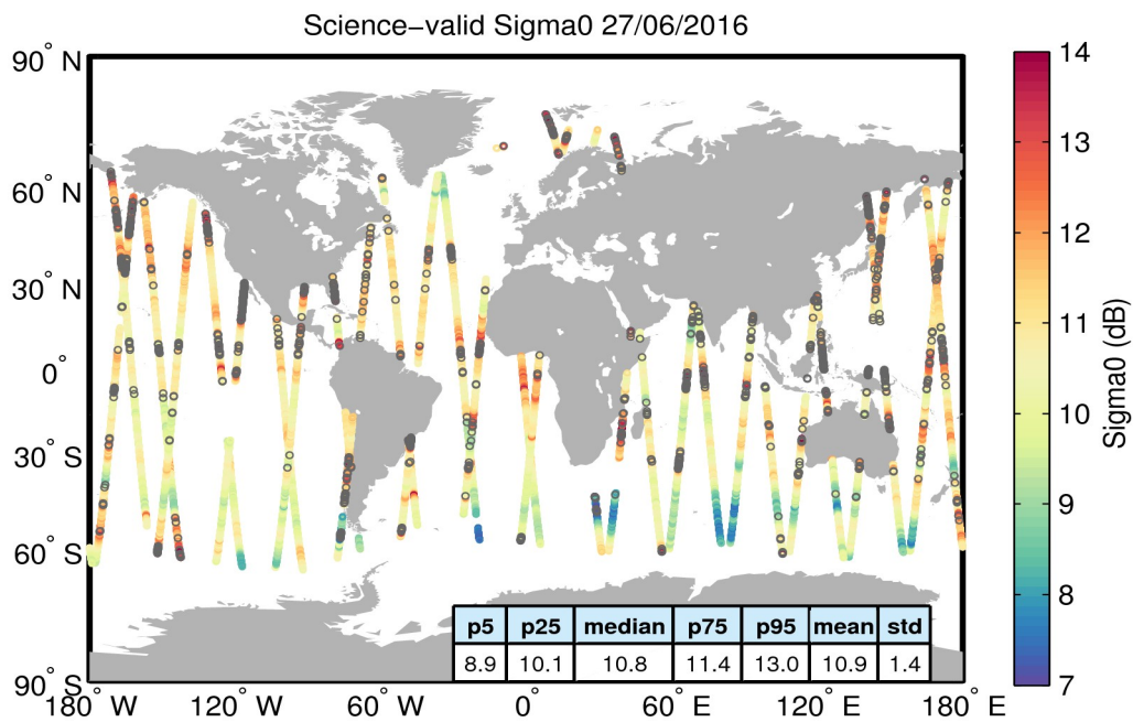
Figure 27. Geographical distribution of science-valid sigma0 data over oceans and lakes for 27/06/2016. The statistical values shown in the table refer to the sigma0 in dB and are calculated over all measurements shown in the figure. Gray circles denote records that have been rejected based on the editing criteria described in Table 4.
