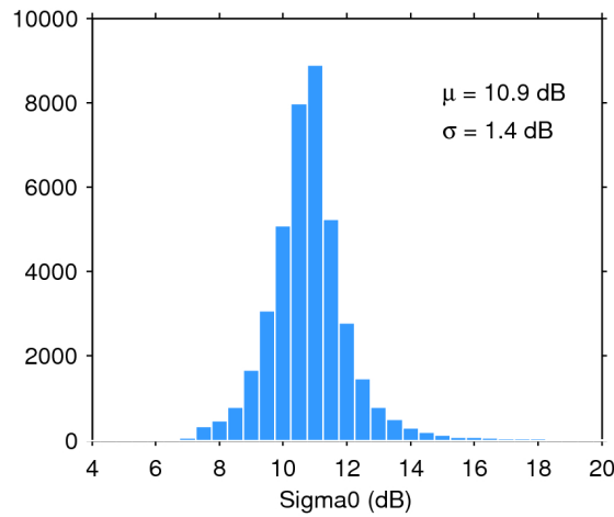
Figure 28. Histogram of science-valid sigma0 over oceans and lakes for 27/06/2016. The mean ( \mu ) and standard deviation ( \sigma ) are also shown. Note that values outside [4 20] dB are excluded from the histogram for the sake of readability but not from the computation of \mu and \sigma .
