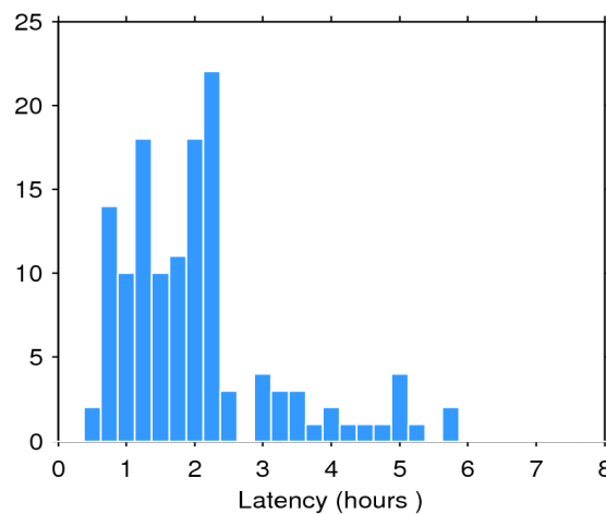
Figure 2. Histogram of the data latency for 27/06/2016. The y-axis denotes the number of files that are made available with a delay of x-hours with respect to the mean time of the records stored in the file.
