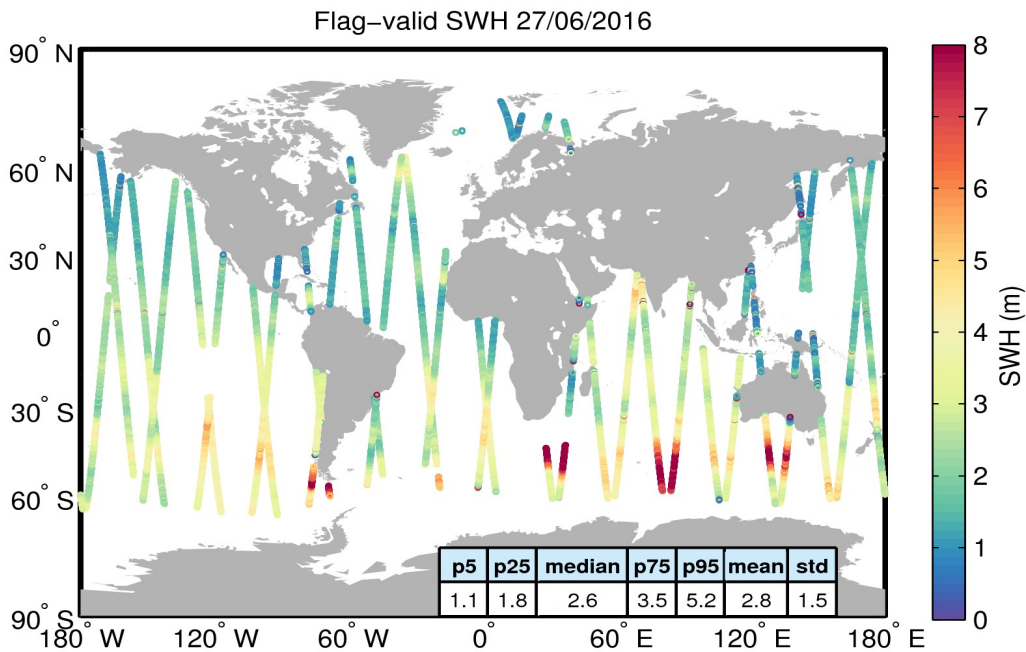
Figure 15. Geographical distribution of flag-valid SWH data over oceans and lakes for 27/06/2016. The statistical values shown in the table refer to the SWH in m and are calculated over all measurements shown in the figure.
