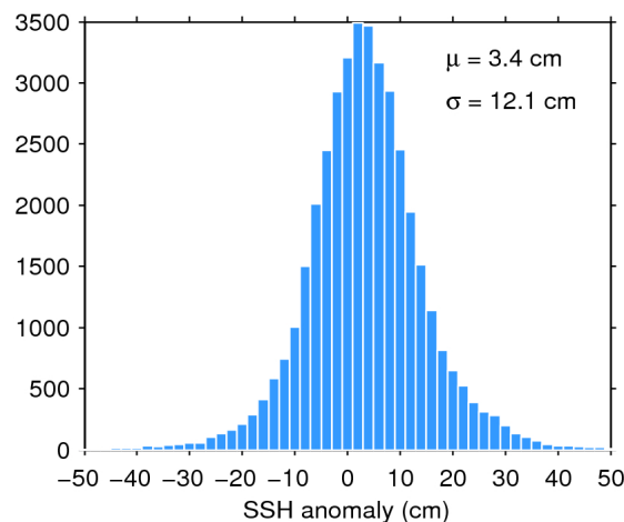
Figure 11. Histogram of science-valid SSH anomaly over oceans and lakes for 27/06/2016. The mean ( \mu ) and standard deviation ( \sigma ) are also shown. Note that values outside [-50 50] cm are excluded from the histogram for the sake of readability but not from the computation of \mu and \sigma .
