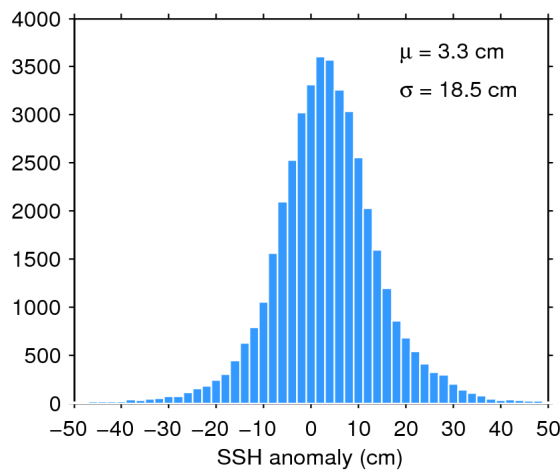
Figure 7. Histogram of flag-valid SSH anomaly over oceans and lakes for 27/06/2016. The mean ( \mu ) and standard deviation ( \sigma ) are also shown. Note that values outside [-50 50] cm are excluded from the histogram for the sake of readability but not from the computation of \mu and \sigma .
