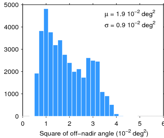
Figure 39. Histogram of flag-valid mispointing over oceans and lakes for 27/06/2016. The mean ( \mu ) and standard deviation ( \sigma ) are also shown. Note that values larger than 6 \cdot 10^{-2} \text{ deg}^2 are excluded from the histogram for the sake of readability but not from the computation of \mu and \sigma .
