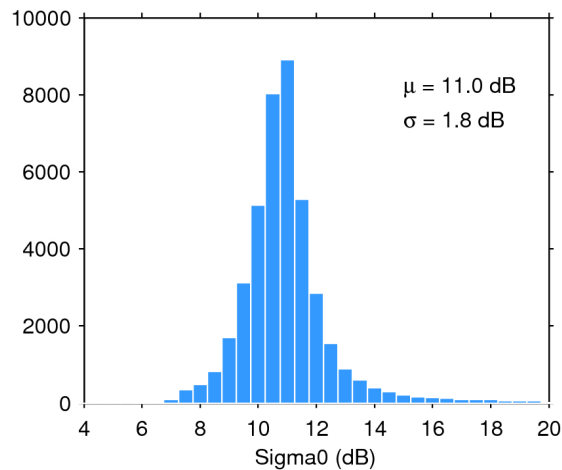
Figure 25. Histogram of flag-valid sigma0 over oceans and lakes for 27/06/2016. The mean ( \mu ) and standard deviation ( \sigma ) are also shown. Note that values outside [4 20] dB are excluded from the histogram for the sake of readability but not from the computation of \mu and \sigma .
