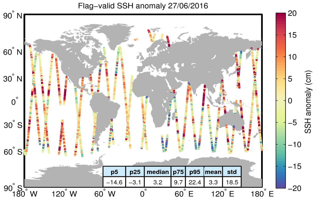
Figure 5. Geographical distribution of flag-valid 1-Hz SSH anomaly data over oceans and lakes for 27/06/2016. The statistical values shown in the table refer to the SSH anomaly in cm and are calculated over all measurements shown in the figure.
