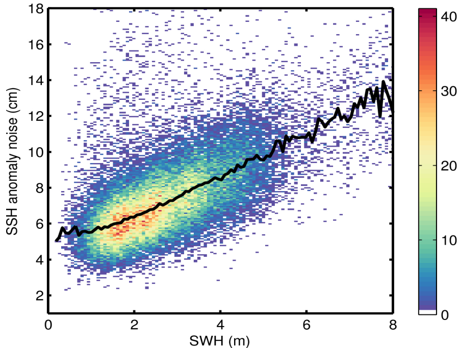
Figure 9. 2D histogram showing flag-valid SSH anomaly noise as a function of SWH for 27/06/2016. The black line denotes the median SSH anomaly noise as a function of SWH.
