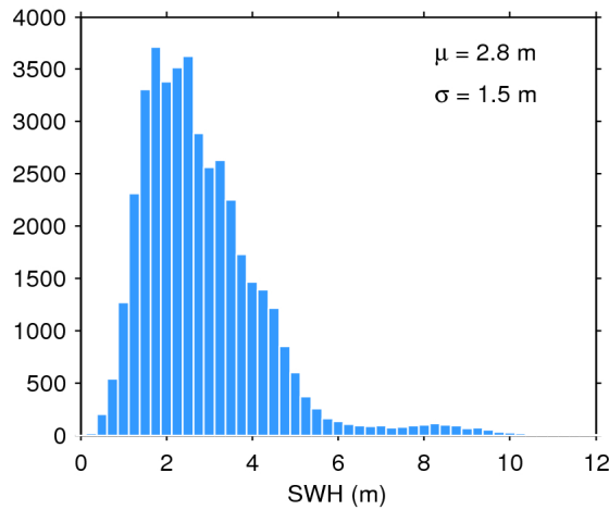
Figure 17. Histogram of flag-valid SWH over oceans and lakes for 27/06/2016. The mean ( \mu ) and standard deviation ( \sigma ) are also shown. Note that values larger than 12 m are excluded from the histogram for the sake of readability but not from the computation of \mu and \sigma .
