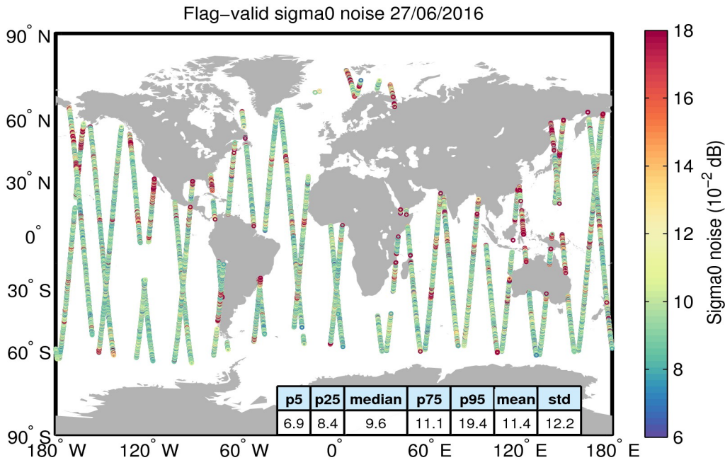
Figure 26. Geographical distribution of flag-valid 20-Hz sigma0 measurement noise over oceans and lakes for 27/06/2016. The statistical values shown in the table refer to the sigma0 noise and are calculated over all measurements shown in the figure.
