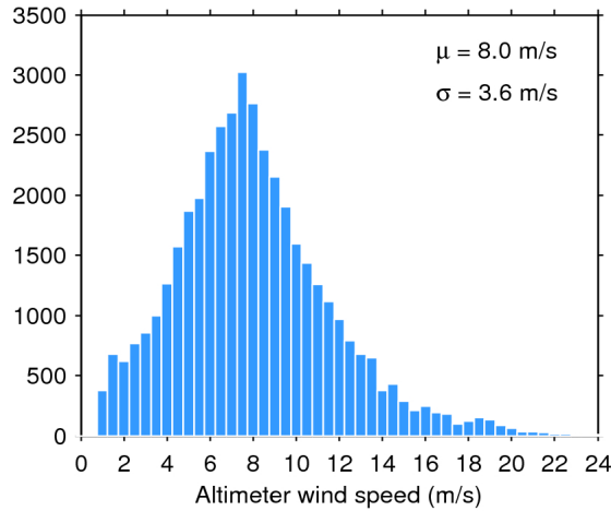
Figure 33. Histogram of flag-valid wind over oceans and lakes for 27/06/2016. The mean ( \mu ) and standard deviation ( \sigma ) are also shown. Note that values larger than 24 m/s are excluded from the histogram for the sake of readability but not from the computation of \mu and \sigma .
