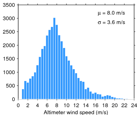
Figure 35. Histogram of science-valid wind over oceans and lakes for 27/06/2016. The mean ( \mu ) and standard deviation ( \sigma ) are also shown. Note that values larger than 24 m/s are excluded from the histogram for the sake of readability but not from the computation of \mu and \sigma .
