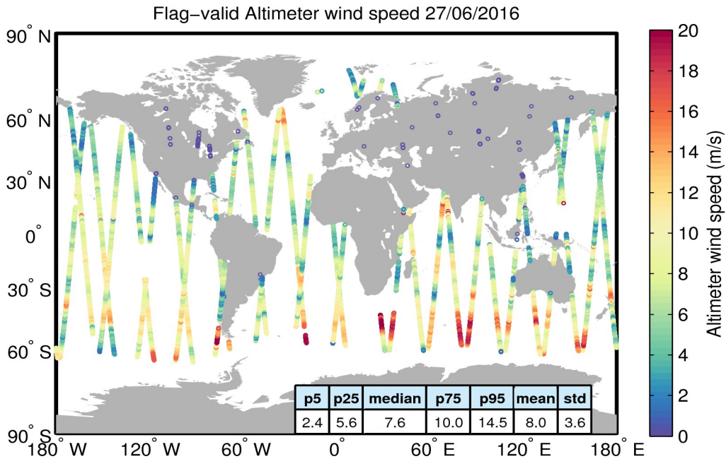
Figure 31. Geographical distribution of flag-valid wind data over oceans and lakes for 27/06/2016. The statistical values shown in the table refer to the wind in m/s and are calculated over all measurements shown in the figure.
