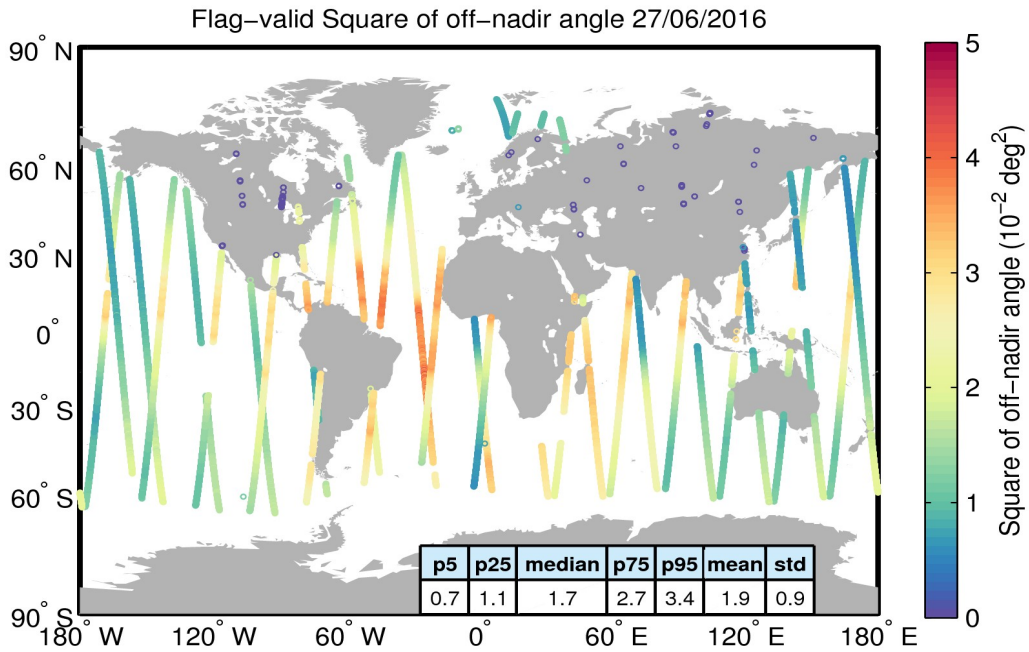
Figure 37. Geographical distribution of flag-valid mispointing data over oceans and lakes for 27/06/2016. The statistical values shown in the table refer to the mispointing in 10^{-2} deg 2 and are calculated over all measurements shown in the figure.
