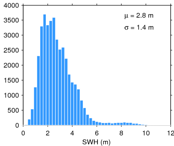
Figure 20. Histogram of science-valid SWH over oceans and lakes for 27/06/2016. The mean ( \mu ) and standard deviation ( \sigma ) are also shown. Note that values larger than 12 m are excluded from the histogram for the sake of readability but not from the computation of \mu and \sigma .
