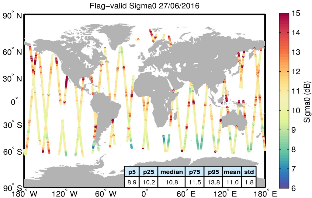
Figure 23. Geographical distribution of flag-valid sigma0 data over oceans and lakes for 27/06/2016. The statistical values shown in the table refer to the sigma0 in dB and are calculated over all measurements shown in the figure.
