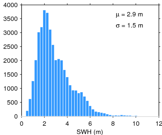
Figure 20. Histogram of science-valid SWH over oceans and lakes for 26/06/2016. The mean ( \mu ) and standard deviation ( \sigma ) are also shown. Note that values larger than 12 m are excluded from the histogram for the sake of readability but not from the computation of \mu and \sigma .
