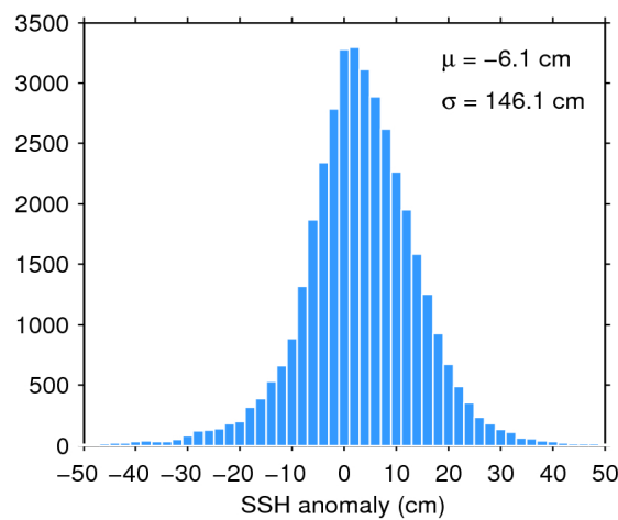
Figure 7. Histogram of flag-valid SSH anomaly over oceans and lakes for 26/06/2016. The mean ( \mu ) and standard deviation ( \sigma ) are also shown. Note that values outside [-50 50] cm are excluded from the histogram for the sake of readability but not from the computation of \mu and \sigma .
