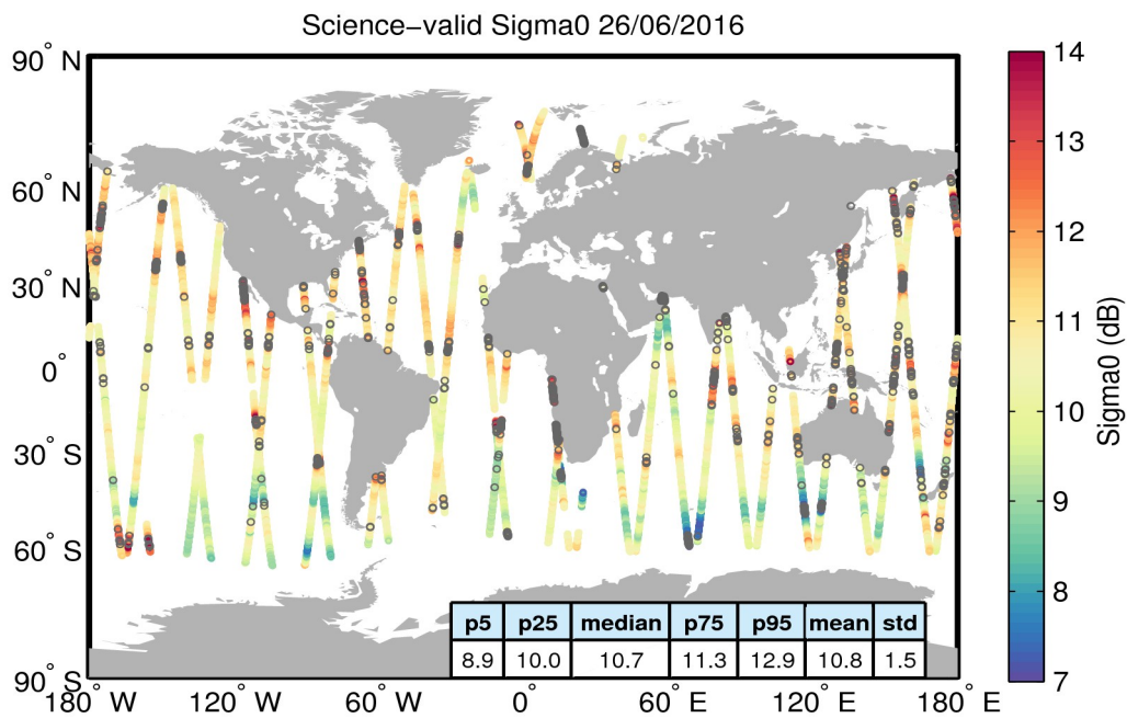
Figure 27. Geographical distribution of science-valid sigma0 data over oceans and lakes for 26/06/2016. The statistical values shown in the table refer to the sigma0 in dB and are calculated over all measurements shown in the figure. Gray circles denote records that have been rejected based on the editing criteria described in Table 4.
