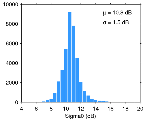
Figure 28. Histogram of science-valid sigma0 over oceans and lakes for 26/06/2016. The mean ( \mu ) and standard deviation ( \sigma ) are also shown. Note that values outside [4 20] dB are excluded from the histogram for the sake of readability but not from the computation of \mu and \sigma .
