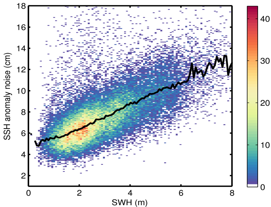
Figure 9. 2D histogram showing flag-valid SSH anomaly noise as a function of SWH for 26/06/2016. The black line denotes the median SSH anomaly noise as a function of SWH.
