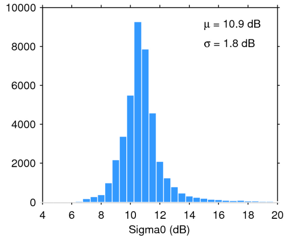
Figure 25. Histogram of flag-valid sigma0 over oceans and lakes for 26/06/2016. The mean ( \mu ) and standard deviation ( \sigma ) are also shown. Note that values outside [4 20] dB are excluded from the histogram for the sake of readability but not from the computation of \mu and \sigma .
