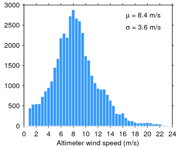
Figure 33. Histogram of flag-valid wind over oceans and lakes for 26/06/2016. The mean ( \mu ) and standard deviation ( \sigma ) are also shown. Note that values larger than 24 m/s are excluded from the histogram for the sake of readability but not from the computation of \mu and \sigma .
