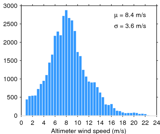
Figure 35. Histogram of science-valid wind over oceans and lakes for 26/06/2016. The mean ( \mu ) and standard deviation ( \sigma ) are also shown. Note that values larger than 24 m/s are excluded from the histogram for the sake of readability but not from the computation of \mu and \sigma .
