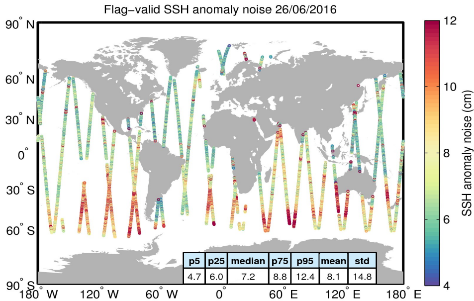
Figure 8. Geographical distribution of flag-valid 20-Hz SSH anomaly measurement noise over oceans and lakes for 26/06/2016. The statistical values shown in the table refer to the SSH anomaly noise and are calculated over all measurements shown in the figure.
