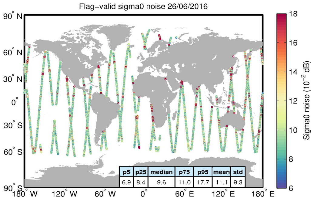
Figure 26. Geographical distribution of flag-valid 20-Hz sigma0 measurement noise over oceans and lakes for 26/06/2016. The statistical values shown in the table refer to the sigma0 noise and are calculated over all measurements shown in the figure.
