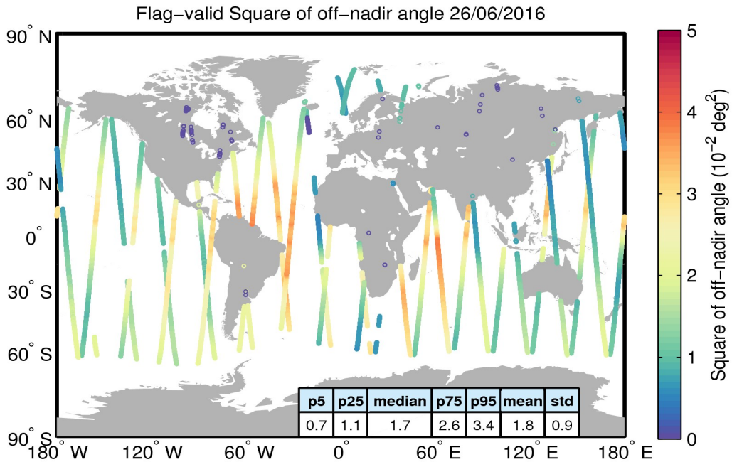
Figure 37. Geographical distribution of flag-valid mispointing data over oceans and lakes for 26/06/2016. The statistical values shown in the table refer to the mispointing in 10^{-2} deg 2 and are calculated over all measurements shown in the figure.
