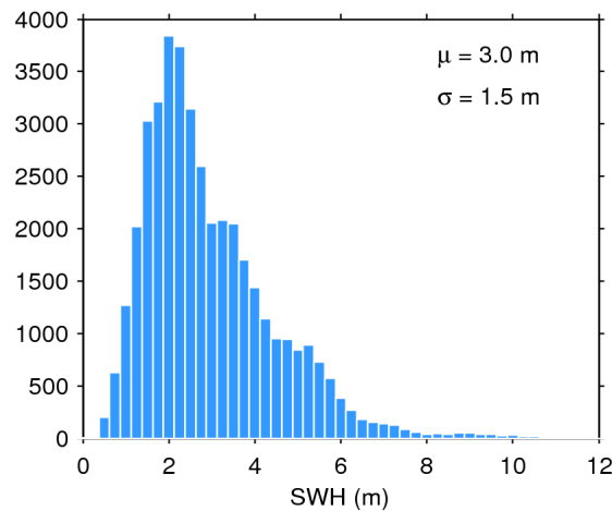
Figure 17. Histogram of flag-valid SWH over oceans and lakes for 26/06/2016. The mean ( \mu ) and standard deviation ( \sigma ) are also shown. Note that values larger than 12 m are excluded from the histogram for the sake of readability but not from the computation of \mu and \sigma .
