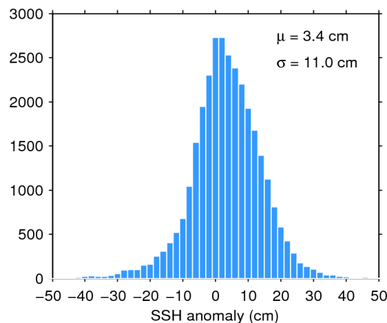
Figure 11. Histogram of science-valid SSH anomaly over oceans and lakes for 26/06/2016. The mean ( \mu ) and standard deviation ( \sigma ) are also shown. Note that values outside [-50 50] cm are excluded from the histogram for the sake of readability but not from the computation of \mu and \sigma .
