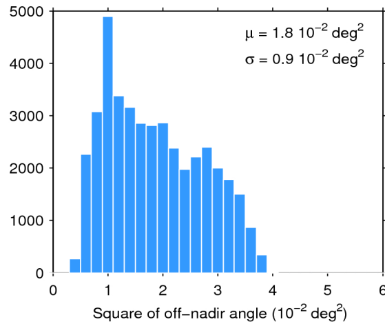
Figure 39. Histogram of flag-valid mispointing over oceans and lakes for 26/06/2016. The mean ( \mu ) and standard deviation ( \sigma ) are also shown. Note that values larger than 6 \cdot 10^{-2} \text{ deg}^2 are excluded from the histogram for the sake of readability but not from the computation of \mu and \sigma .
