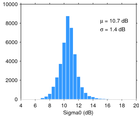
Figure 28. Histogram of science-valid sigma0 over oceans and lakes for 25/06/2016. The mean ( \mu ) and standard deviation ( \sigma ) are also shown. Note that values outside [4 20] dB are excluded from the histogram for the sake of readability but not from the computation of \mu and \sigma .
