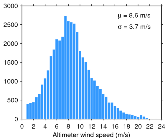
Figure 35. Histogram of science-valid wind over oceans and lakes for 25/06/2016. The mean ( \mu ) and standard deviation ( \sigma ) are also shown. Note that values larger than 24 m/s are excluded from the histogram for the sake of readability but not from the computation of \mu and \sigma .
