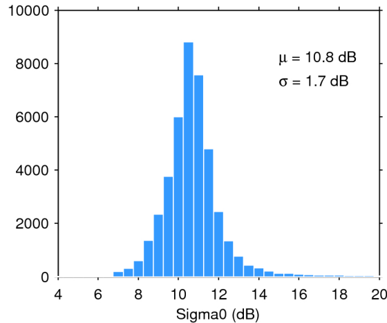
Figure 25. Histogram of flag-valid sigma0 over oceans and lakes for 25/06/2016. The mean ( \mu ) and standard deviation ( \sigma ) are also shown. Note that values outside [4 20] dB are excluded from the histogram for the sake of readability but not from the computation of \mu and \sigma .
