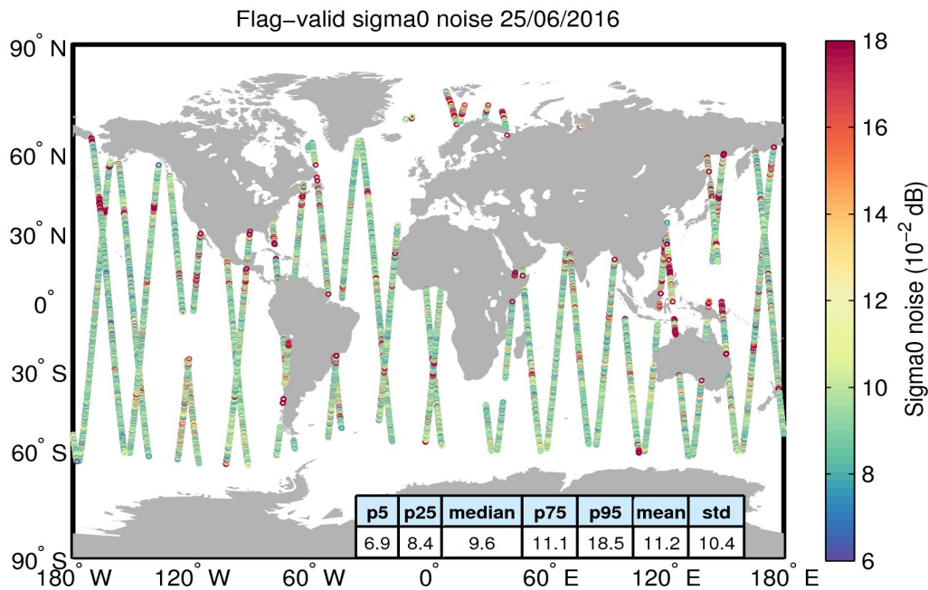
Figure 26. Geographical distribution of flag-valid 20-Hz sigma0 measurement noise over oceans and lakes for 25/06/2016. The statistical values shown in the table refer to the sigma0 noise and are calculated over all measurements shown in the figure.
