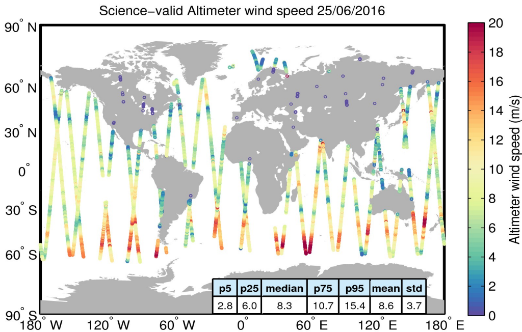
Figure 34. Geographical distribution of science-valid wind data over oceans and lakes for 25/06/2016. The statistical values shown in the table refer to the wind in m/s and are calculated over all measurements shown in the figure. Gray circles denote records that have been rejected based on the editing criteria described in Table 5.
