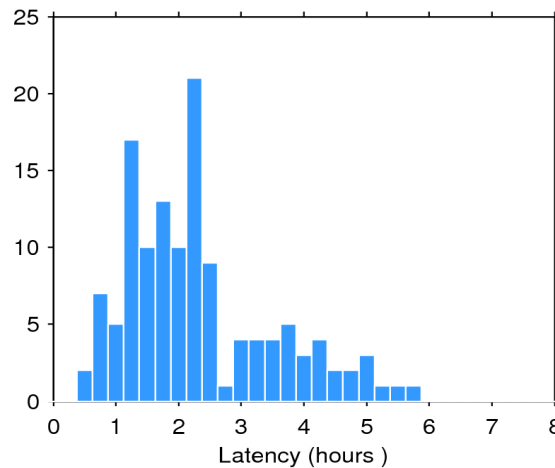
Figure 2. Histogram of the data latency for 25/06/2016. The y-axis denotes the number of files that are made available with a delay of x-hours with respect to the mean time of the records stored in the file.
