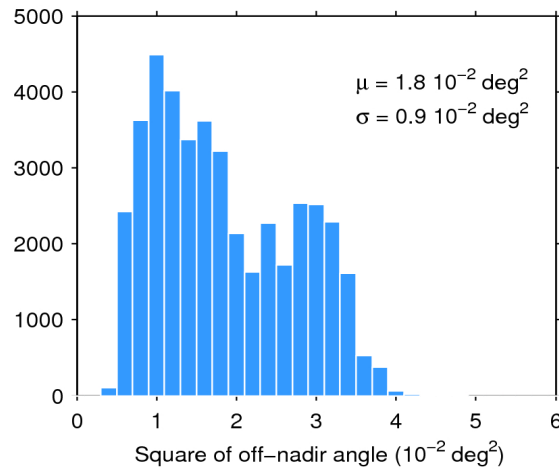
Figure 39. Histogram of flag-valid mispointing over oceans and lakes for 25/06/2016. The mean ( \mu ) and standard deviation ( \sigma ) are also shown. Note that values larger than 6 \cdot 10^{-2} \text{ deg}^2 are excluded from the histogram for the sake of readability but not from the computation of \mu and \sigma .
