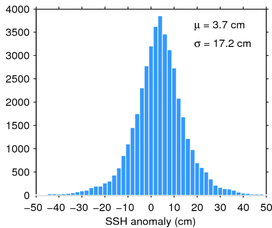
Figure 7. Histogram of flag-valid SSH anomaly over oceans and lakes for 25/06/2016. The mean ( \mu ) and standard deviation ( \sigma ) are also shown. Note that values outside [-50\ 50] cm are excluded from the histogram for the sake of readability but not from the computation of \mu and \sigma .
