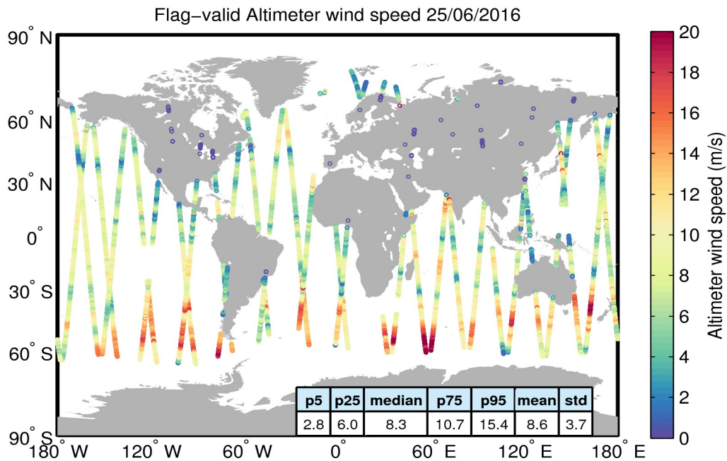
Figure 31. Geographical distribution of flag-valid wind data over oceans and lakes for 25/06/2016. The statistical values shown in the table refer to the wind in m/s and are calculated over all measurements shown in the figure.
