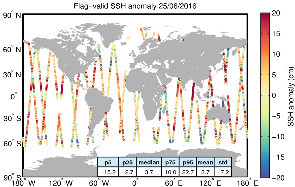
Figure 5. Geographical distribution of flag-valid 1-Hz SSH anomaly data over oceans and lakes for 25/06/2016. The statistical values shown in the table refer to the SSH anomaly in cm and are calculated over all measurements shown in the figure.
