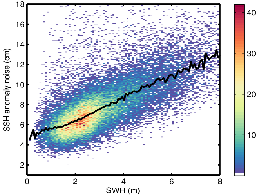
Figure 9. 2D histogram showing flag-valid SSH anomaly noise as a function of SWH for 25/06/2016. The black line denotes the median SSH anomaly noise as a function of SWH.
