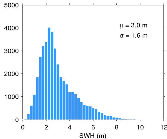
Figure 20. Histogram of science-valid SWH over oceans and lakes for 25/06/2016. The mean ( \mu ) and standard deviation ( \sigma ) are also shown. Note that values larger than 12 m are excluded from the histogram for the sake of readability but not from the computation of \mu and \sigma .
