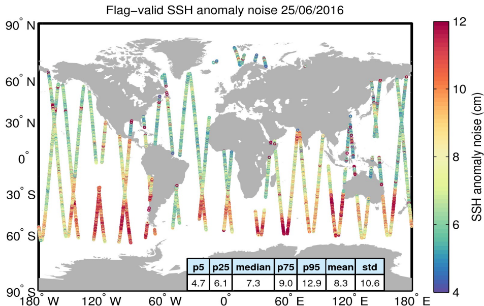
Figure 8. Geographical distribution of flag-valid 20-Hz SSH anomaly measurement noise over oceans and lakes for 25/06/2016. The statistical values shown in the table refer to the SSH anomaly noise and are calculated over all measurements shown in the figure.
