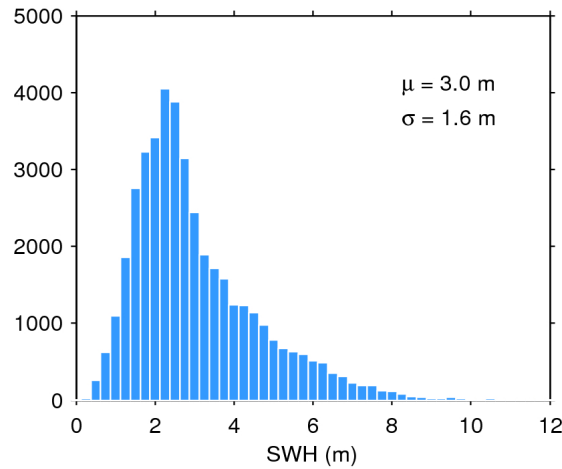
Figure 17. Histogram of flag-valid SWH over oceans and lakes for 25/06/2016. The mean ( \mu ) and standard deviation ( \sigma ) are also shown. Note that values larger than 12 m are excluded from the histogram for the sake of readability but not from the computation of \mu and \sigma .
