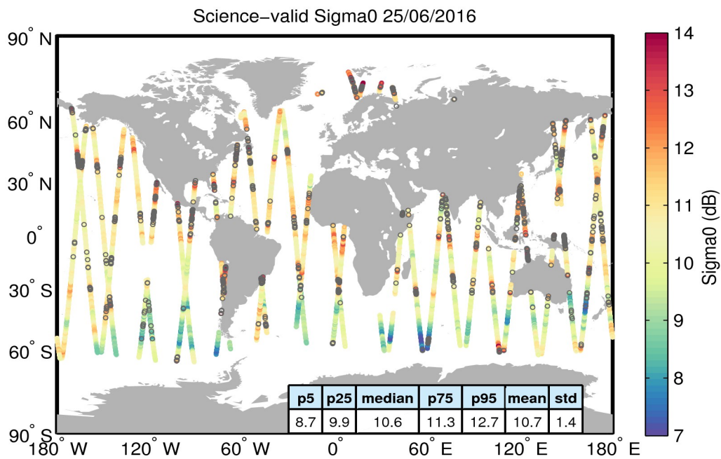
Figure 27. Geographical distribution of science-valid sigma0 data over oceans and lakes for 25/06/2016. The statistical values shown in the table refer to the sigma0 in dB and are calculated over all measurements shown in the figure. Gray circles denote records that have been rejected based on the editing criteria described in Table 4.
