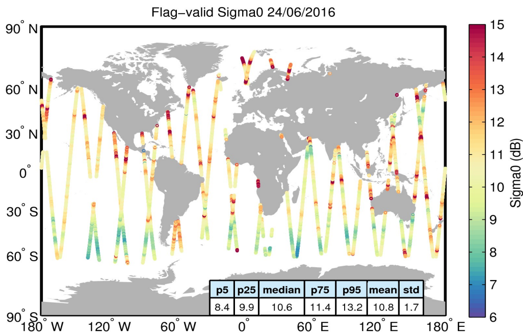
Figure 23. Geographical distribution of flag-valid sigma0 data over oceans and lakes for 24/06/2016. The statistical values shown in the table refer to the sigma0 in dB and are calculated over all measurements shown in the figure.
