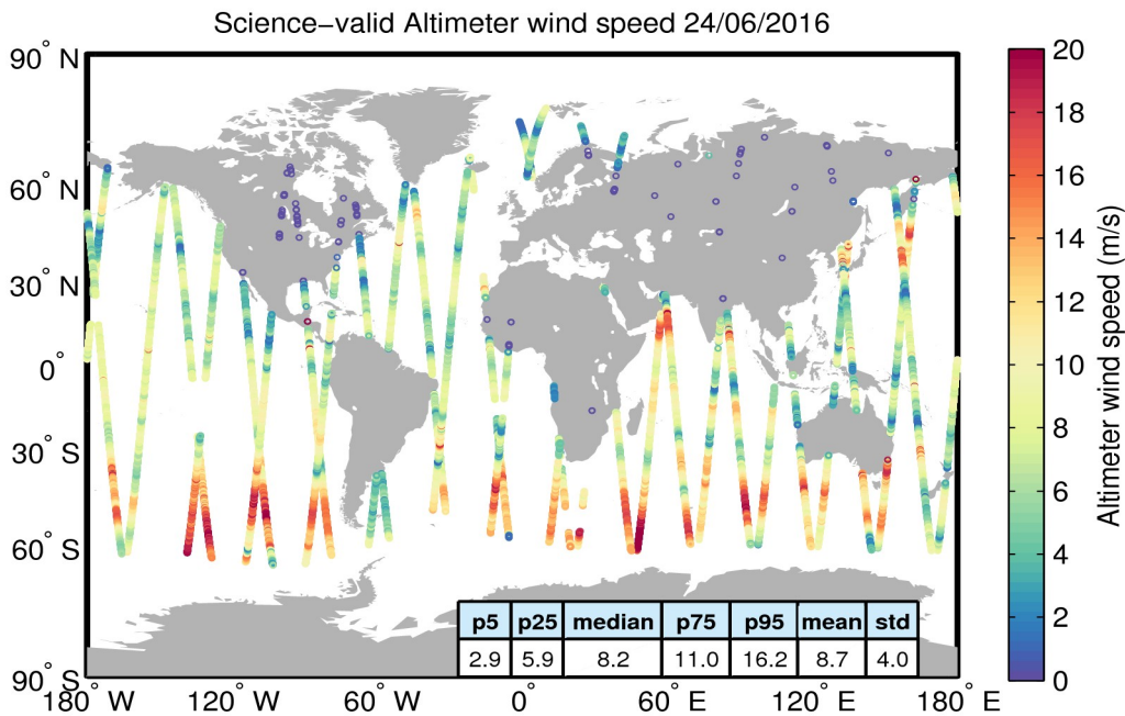
Figure 34. Geographical distribution of science-valid wind data over oceans and lakes for 24/06/2016. The statistical values shown in the table refer to the wind in m/s and are calculated over all measurements shown in the figure. Gray circles denote records that have been rejected based on the editing criteria described in Table 5.
