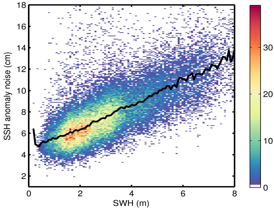
Figure 9. 2D histogram showing flag-valid SSH anomaly noise as a function of SWH for 24/06/2016. The black line denotes the median SSH anomaly noise as a function of SWH.
