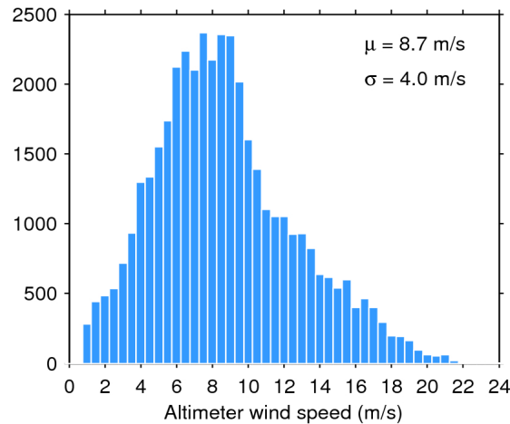
Figure 33. Histogram of flag-valid wind over oceans and lakes for 24/06/2016. The mean ( \mu ) and standard deviation ( \sigma ) are also shown. Note that values larger than 24 m/s are excluded from the histogram for the sake of readability but not from the computation of \mu and \sigma .
