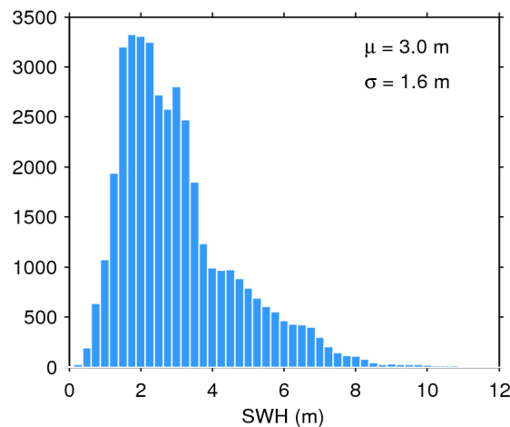
Figure 20. Histogram of science-valid SWH over oceans and lakes for 24/06/2016. The mean ( \mu ) and standard deviation ( \sigma ) are also shown. Note that values larger than 12 m are excluded from the histogram for the sake of readability but not from the computation of \mu and \sigma .
