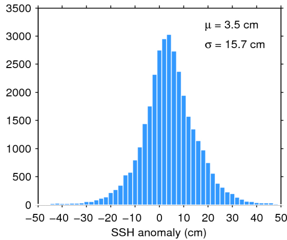
Figure 11. Histogram of science-valid SSH anomaly over oceans and lakes for 24/06/2016. The mean ( \mu ) and standard deviation ( \sigma ) are also shown. Note that values outside [-50 50] cm are excluded from the histogram for the sake of readability but not from the computation of \mu and \sigma .
