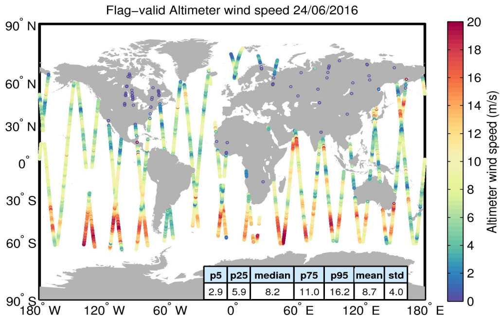
Figure 31. Geographical distribution of flag-valid wind data over oceans and lakes for 24/06/2016. The statistical values shown in the table refer to the wind in m/s and are calculated over all measurements shown in the figure.
