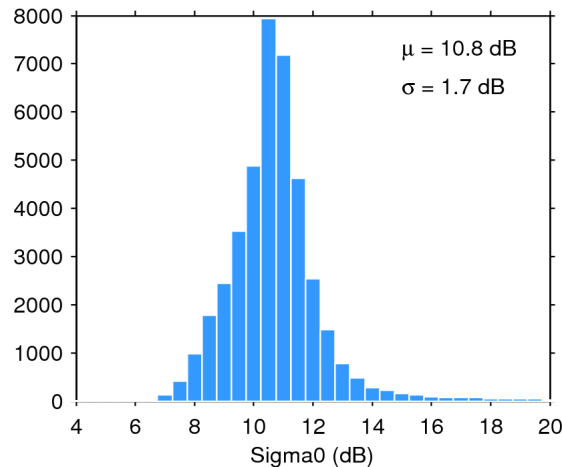
Figure 25. Histogram of flag-valid sigma0 over oceans and lakes for 24/06/2016. The mean ( \mu ) and standard deviation ( \sigma ) are also shown. Note that values outside [4 20] dB are excluded from the histogram for the sake of readability but not from the computation of \mu and \sigma .
