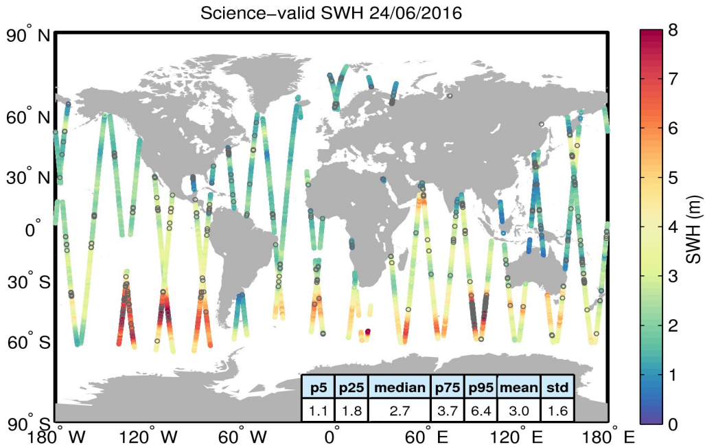
Figure 19. Geographical distribution of science-valid SWH data over oceans and lakes for 24/06/2016. The statistical values shown in the table refer to the SWH in m and are calculated over all measurements shown in the figure. Gray circles denote records that have been rejected based on the editing criteria described in Table 3.
