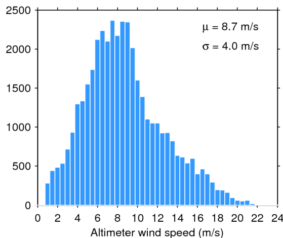
Figure 35. Histogram of science-valid wind over oceans and lakes for 24/06/2016. The mean ( \mu ) and standard deviation ( \sigma ) are also shown. Note that values larger than 24 m/s are excluded from the histogram for the sake of readability but not from the computation of \mu and \sigma .
