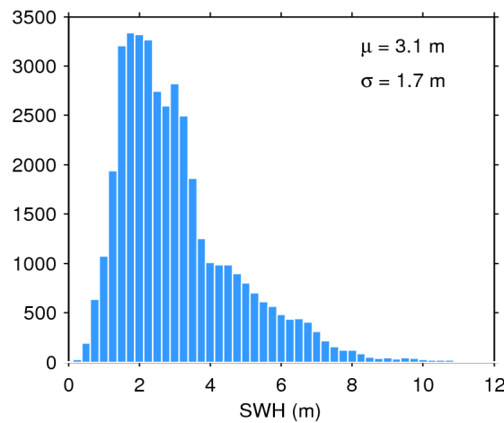
Figure 17. Histogram of flag-valid SWH over oceans and lakes for 24/06/2016. The mean ( \mu ) and standard deviation ( \sigma ) are also shown. Note that values larger than 12 m are excluded from the histogram for the sake of readability but not from the computation of \mu and \sigma .
