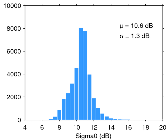
Figure 28. Histogram of science-valid sigma0 over oceans and lakes for 23/06/2016. The mean ( \mu ) and standard deviation ( \sigma ) are also shown. Note that values outside [4 20] dB are excluded from the histogram for the sake of readability but not from the computation of \mu and \sigma .
