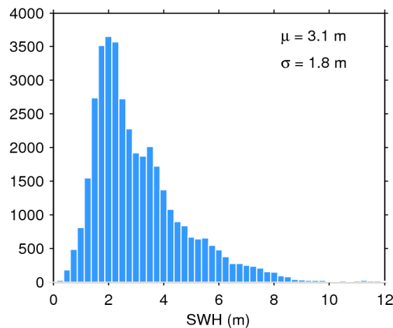
Figure 17. Histogram of flag-valid SWH over oceans and lakes for 23/06/2016. The mean ( \mu ) and standard deviation ( \sigma ) are also shown. Note that values larger than 12 m are excluded from the histogram for the sake of readability but not from the computation of \mu and \sigma .
