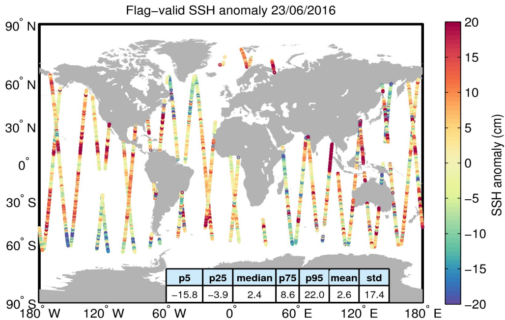
Figure 5. Geographical distribution of flag-valid 1-Hz SSH anomaly data over oceans and lakes for 23/06/2016. The statistical values shown in the table refer to the SSH anomaly in cm and are calculated over all measurements shown in the figure.
