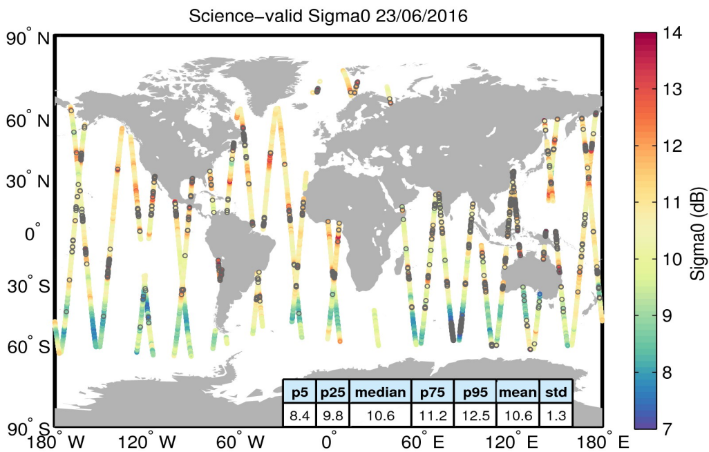
Figure 27. Geographical distribution of science-valid sigma0 data over oceans and lakes for 23/06/2016. The statistical values shown in the table refer to the sigma0 in dB and are calculated over all measurements shown in the figure. Gray circles denote records that have been rejected based on the editing criteria described in Table 4.
