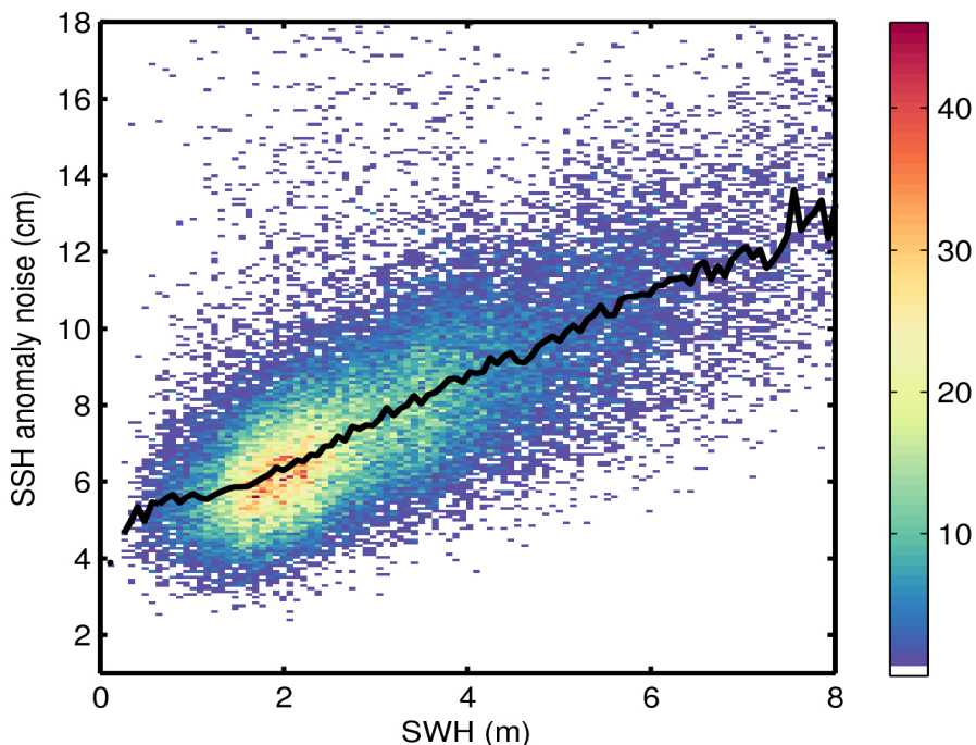
Figure 9. 2D histogram showing flag-valid SSH anomaly noise as a function of SWH for 23/06/2016. The black line denotes the median SSH anomaly noise as a function of SWH.
