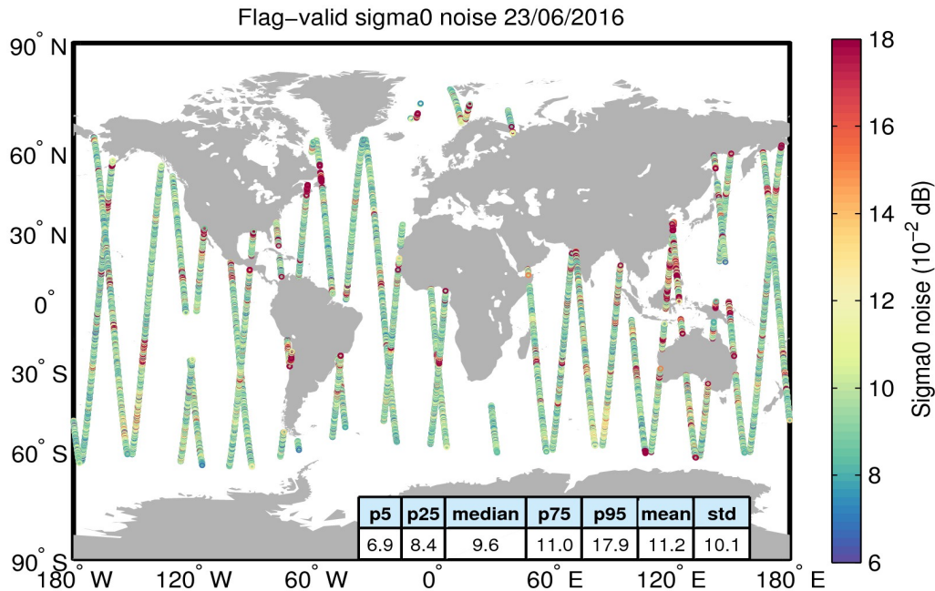
Figure 26. Geographical distribution of flag-valid 20-Hz sigma0 measurement noise over oceans and lakes for 23/06/2016. The statistical values shown in the table refer to the sigma0 noise and are calculated over all measurements shown in the figure.
