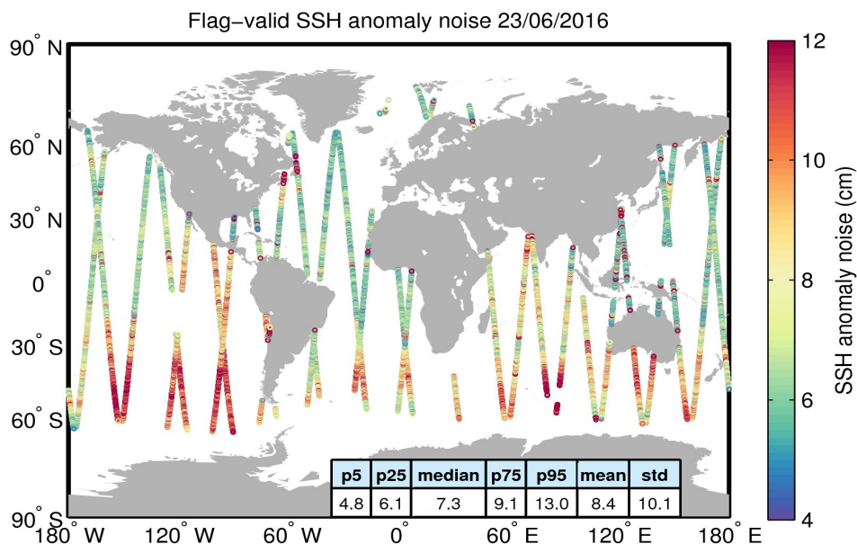
Figure 8. Geographical distribution of flag-valid 20-Hz SSH anomaly measurement noise over oceans and lakes for 23/06/2016. The statistical values shown in the table refer to the SSH anomaly noise and are calculated over all measurements shown in the figure.
