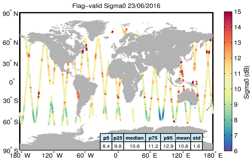
Figure 23. Geographical distribution of flag-valid sigma0 data over oceans and lakes for 23/06/2016. The statistical values shown in the table refer to the sigma0 in dB and are calculated over all measurements shown in the figure.
