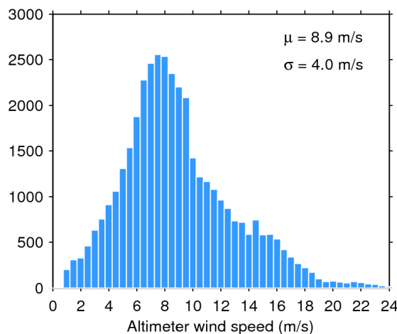
Figure 35. Histogram of science-valid wind over oceans and lakes for 23/06/2016. The mean ( \mu ) and standard deviation ( \sigma ) are also shown. Note that values larger than 24 m/s are excluded from the histogram for the sake of readability but not from the computation of \mu and \sigma .
