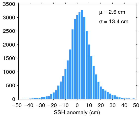
Figure 11. Histogram of science-valid SSH anomaly over oceans and lakes for 23/06/2016. The mean ( \mu ) and standard deviation ( \sigma ) are also shown. Note that values outside [-50 50] cm are excluded from the histogram for the sake of readability but not from the computation of \mu and \sigma .
