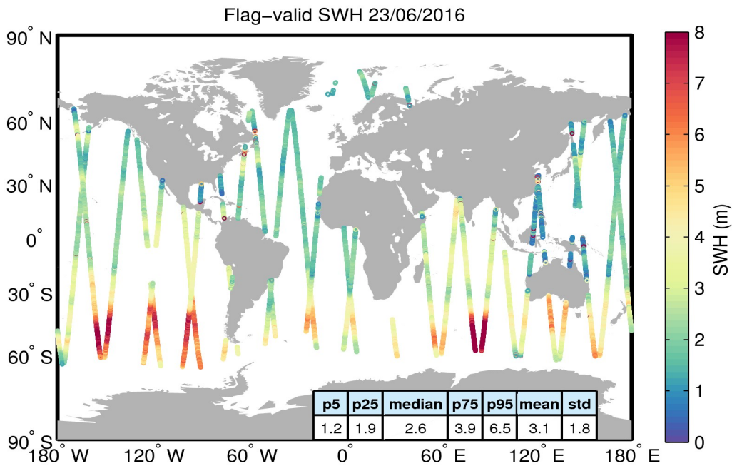
Figure 15. Geographical distribution of flag-valid SWH data over oceans and lakes for 23/06/2016. The statistical values shown in the table refer to the SWH in m and are calculated over all measurements shown in the figure.
