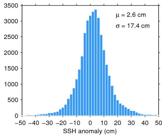
Figure 7. Histogram of flag-valid SSH anomaly over oceans and lakes for 23/06/2016. The mean ( \mu ) and standard deviation ( \sigma ) are also shown. Note that values outside [-50\ 50] cm are excluded from the histogram for the sake of readability but not from the computation of \mu and \sigma .
