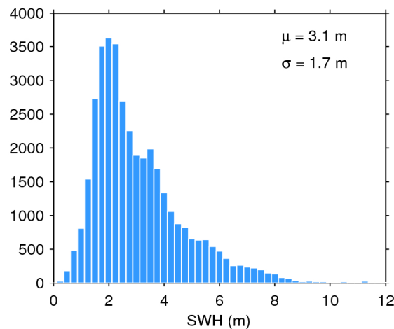
Figure 20. Histogram of science-valid SWH over oceans and lakes for 23/06/2016. The mean ( \mu ) and standard deviation ( \sigma ) are also shown. Note that values larger than 12 m are excluded from the histogram for the sake of readability but not from the computation of \mu and \sigma .
