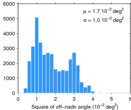
Figure 39. Histogram of flag-valid mispointing over oceans and lakes for 23/06/2016. The mean ( \mu ) and standard deviation ( \sigma ) are also shown. Note that values larger than 6 \cdot 10^{-2} \text{ deg}^2 are excluded from the histogram for the sake of readability but not from the computation of \mu and \sigma .
