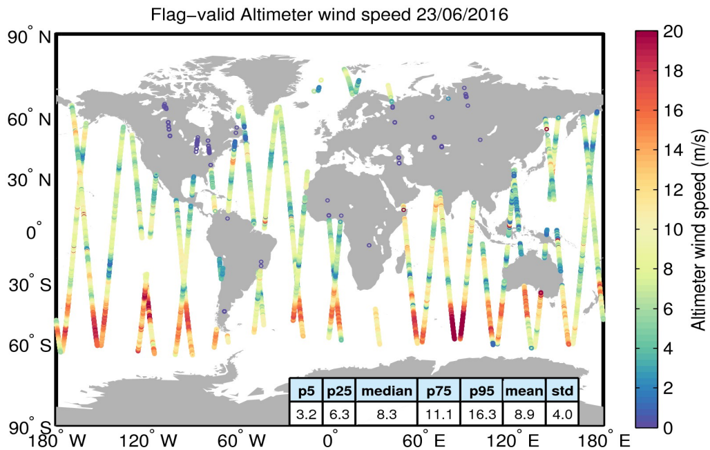
Figure 31. Geographical distribution of flag-valid wind data over oceans and lakes for 23/06/2016. The statistical values shown in the table refer to the wind in m/s and are calculated over all measurements shown in the figure.
