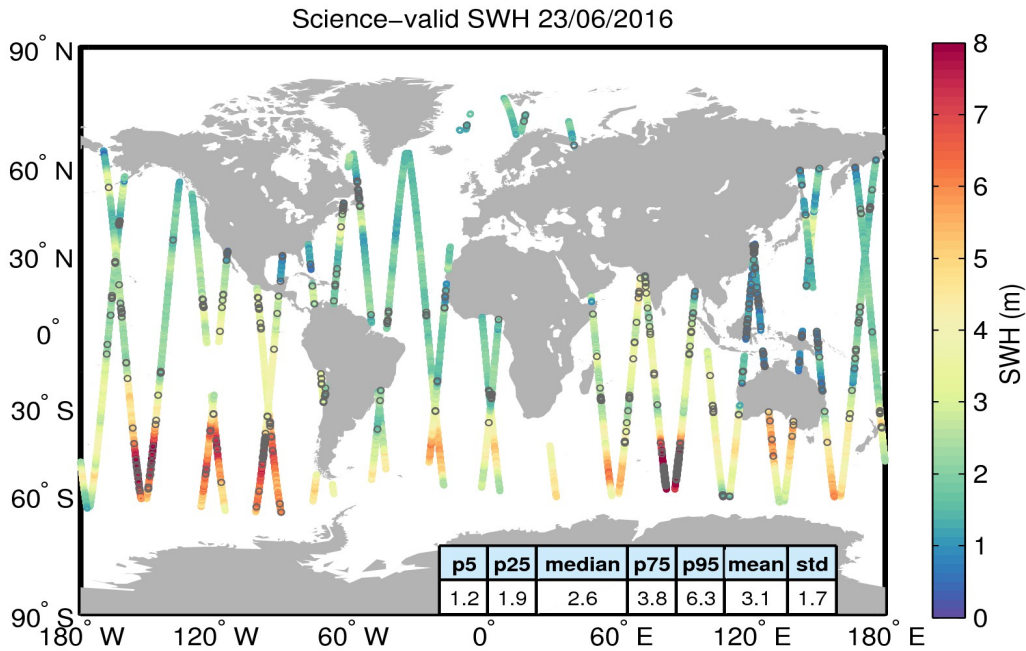
Figure 19. Geographical distribution of science-valid SWH data over oceans and lakes for 23/06/2016. The statistical values shown in the table refer to the SWH in m and are calculated over all measurements shown in the figure. Gray circles denote records that have been rejected based on the editing criteria described in Table 3.
