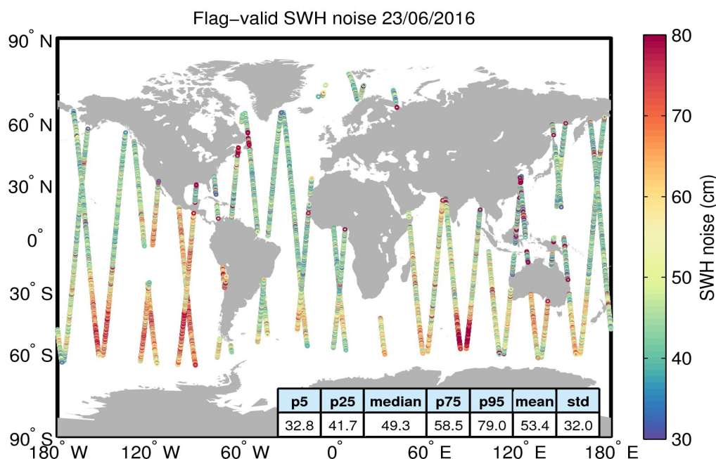
Figure 18. Geographical distribution of flag-valid 20-Hz SWH measurement noise over oceans and lakes for 23/06/2016. The statistical values shown in the figure refer to the SWH noise and are calculated over all measurements shown in the figure.
