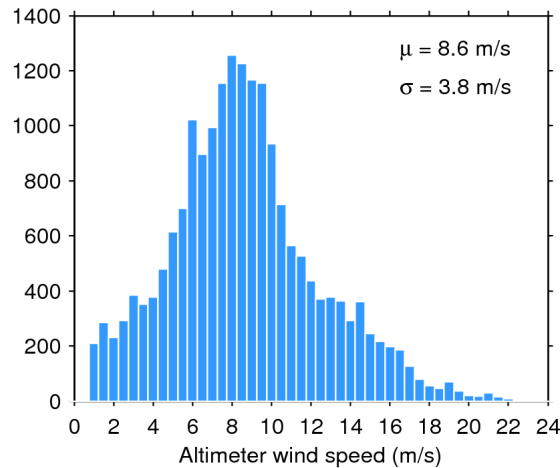
Figure 33. Histogram of flag-valid wind over oceans and lakes for 21/06/2016. The mean ( \mu ) and standard deviation ( \sigma ) are also shown. Note that values larger than 24 m/s are excluded from the histogram for the sake of readability but not from the computation of \mu and \sigma .
