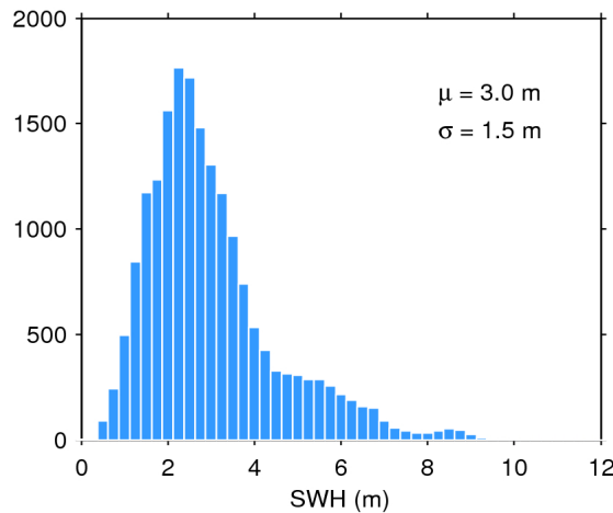
Figure 20. Histogram of science-valid SWH over oceans and lakes for 21/06/2016. The mean ( \mu ) and standard deviation ( \sigma ) are also shown. Note that values larger than 12 m are excluded from the histogram for the sake of readability but not from the computation of \mu and \sigma .
