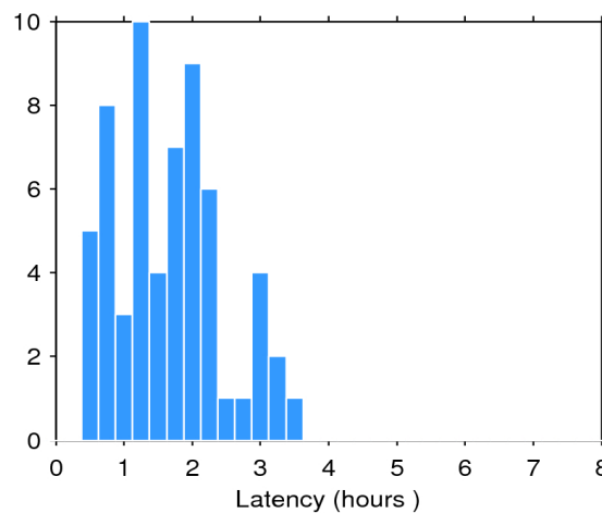
Figure 2. Histogram of the data latency for 21/06/2016. The y-axis denotes the number of files that are made available with a delay of x-hours with respect to the mean time of the records stored in the file.
