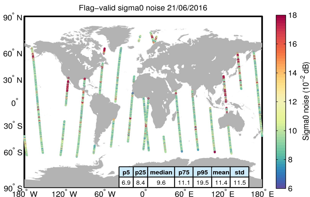
Figure 26. Geographical distribution of flag-valid 20-Hz sigma0 measurement noise over oceans and lakes for 21/06/2016. The statistical values shown in the table refer to the sigma0 noise and are calculated over all measurements shown in the figure.
