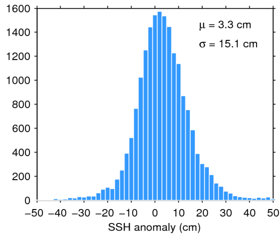
Figure 7. Histogram of flag-valid SSH anomaly over oceans and lakes for 21/06/2016. The mean ( \mu ) and standard deviation ( \sigma ) are also shown. Note that values outside [-50 50] cm are excluded from the histogram for the sake of readability but not from the computation of \mu and \sigma .
