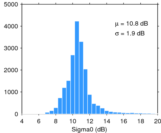
Figure 25. Histogram of flag-valid sigma0 over oceans and lakes for 21/06/2016. The mean ( \mu ) and standard deviation ( \sigma ) are also shown. Note that values outside [4 20] dB are excluded from the histogram for the sake of readability but not from the computation of \mu and \sigma .
