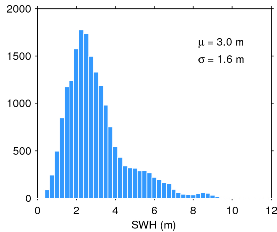
Figure 17. Histogram of flag-valid SWH over oceans and lakes for 21/06/2016. The mean ( \mu ) and standard deviation ( \sigma ) are also shown. Note that values larger than 12 m are excluded from the histogram for the sake of readability but not from the computation of \mu and \sigma .
