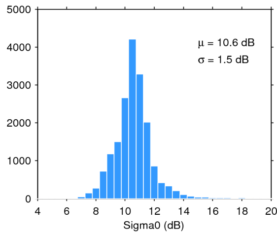
Figure 28. Histogram of science-valid sigma0 over oceans and lakes for 21/06/2016. The mean ( \mu ) and standard deviation ( \sigma ) are also shown. Note that values outside [4 20] dB are excluded from the histogram for the sake of readability but not from the computation of \mu and \sigma .
