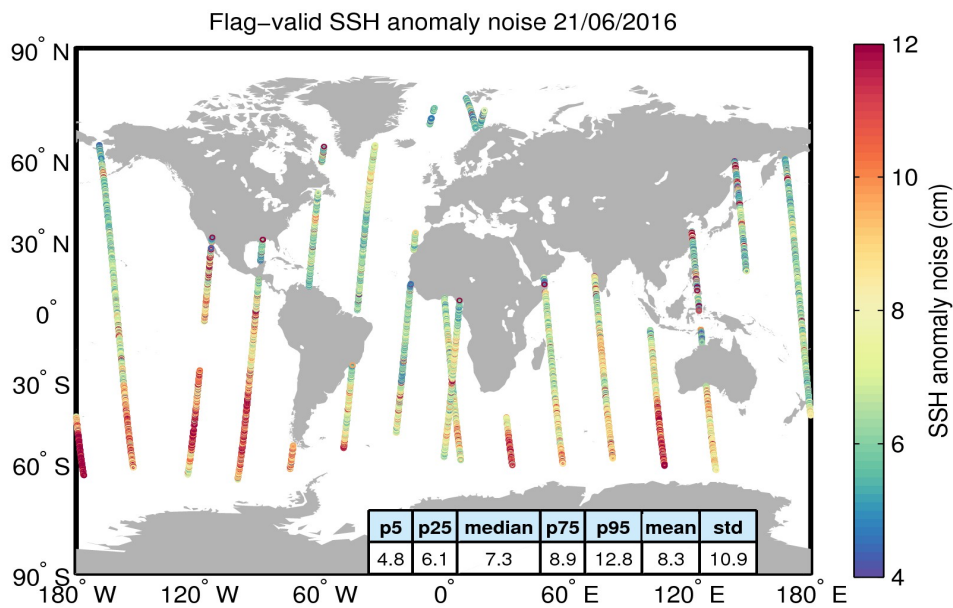
Figure 8. Geographical distribution of flag-valid 20-Hz SSH anomaly measurement noise over oceans and lakes for 21/06/2016. The statistical values shown in the table refer to the SSH anomaly noise and are calculated over all measurements shown in the figure.
