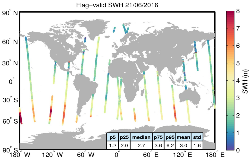
Figure 15. Geographical distribution of flag-valid SWH data over oceans and lakes for 21/06/2016. The statistical values shown in the table refer to the SWH in m and are calculated over all measurements shown in the figure.
