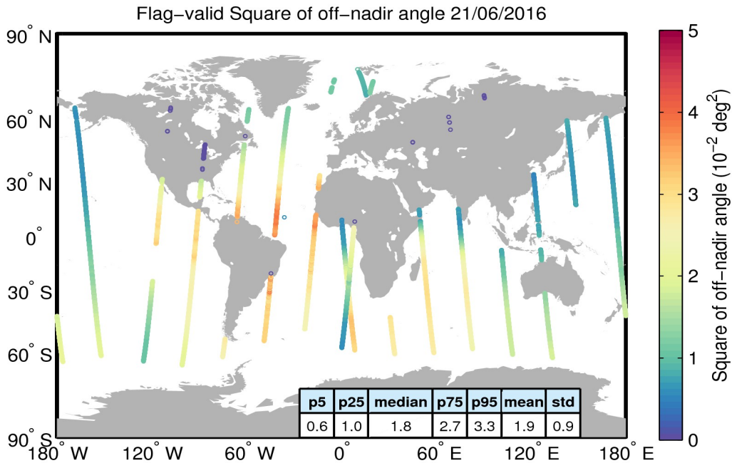
Figure 37. Geographical distribution of flag-valid mispointing data over oceans and lakes for 21/06/2016. The statistical values shown in the table refer to the mispointing in 10^{-2} \text{ deg}^2 and are calculated over all measurements shown in the figure.
