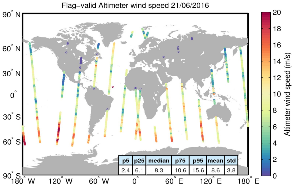
Figure 31. Geographical distribution of flag-valid wind data over oceans and lakes for 21/06/2016. The statistical values shown in the figure refer to the wind in m/s and are calculated over all measurements shown in the figure.
