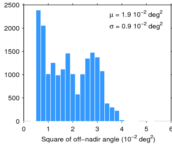
Figure 39. Histogram of flag-valid mispointing over oceans and lakes for 21/06/2016. The mean ( \mu ) and standard deviation ( \sigma ) are also shown. Note that values larger than 6 \cdot 10^{-2} \text{ deg}^2 are excluded from the histogram for the sake of readability but not from the computation of \mu and \sigma .
