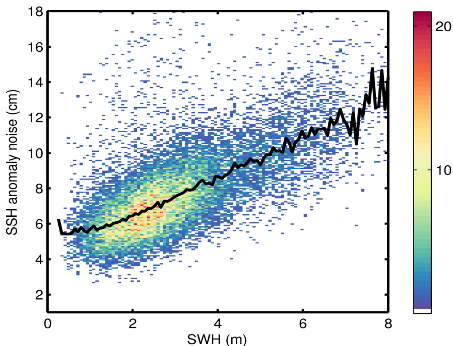
Figure 9. 2D histogram showing flag-valid SSH anomaly noise as a function of SWH for 21/06/2016. The black line denotes the median SSH anomaly noise as a function of SWH.
