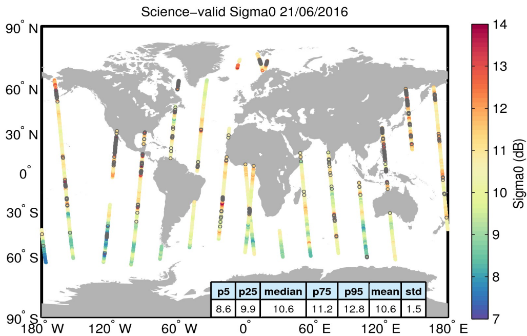
Figure 27. Geographical distribution of science-valid sigma0 data over oceans and lakes for 21/06/2016. The statistical values shown in the table refer to the sigma0 in dB and are calculated over all measurements shown in the figure. Gray circles denote records that have been rejected based on the editing criteria described in Table 4.
