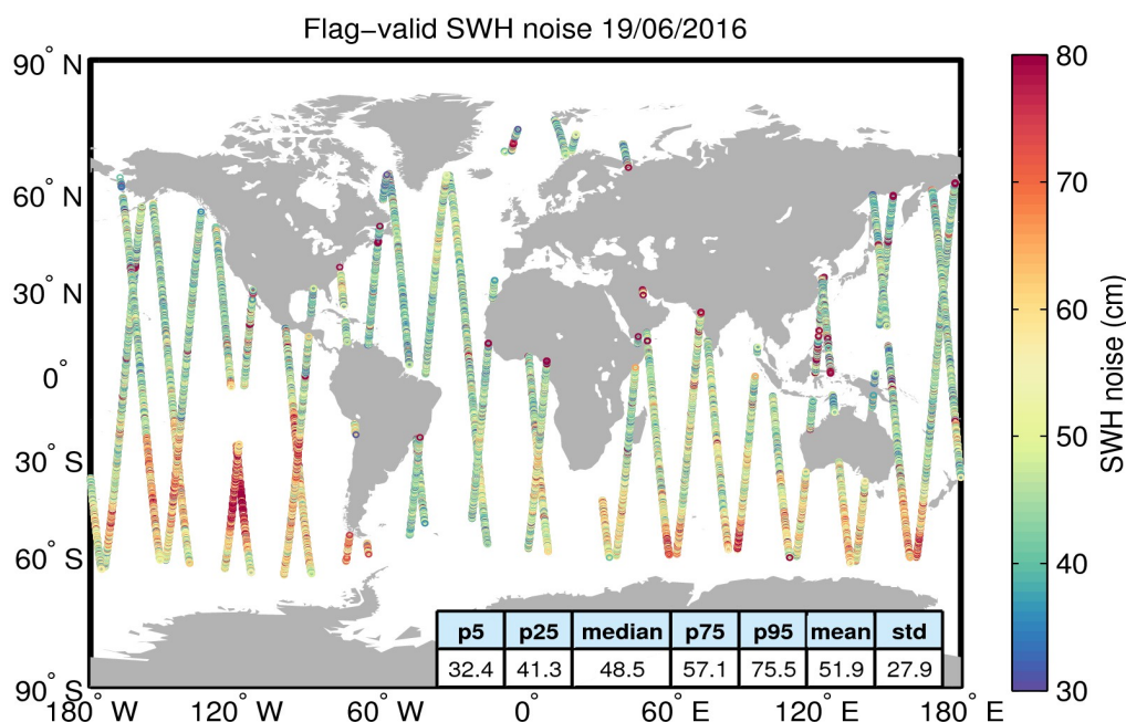
Figure 18. Geographical distribution of flag-valid 20-Hz SWH measurement noise over oceans and lakes for 19/06/2016. The statistical values shown in the figure refer to the SWH noise and are calculated over all measurements shown in the figure.
