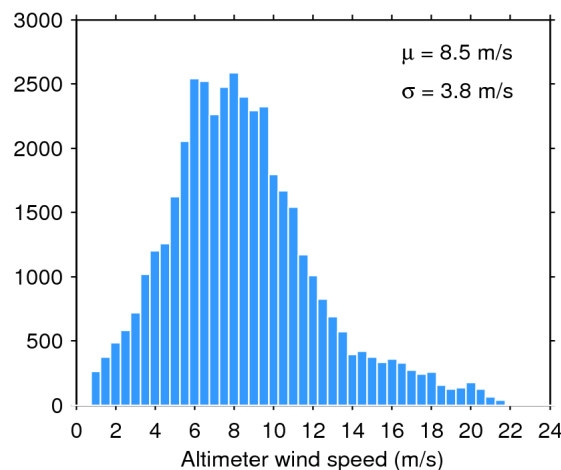
Figure 35. Histogram of science-valid wind over oceans and lakes for 19/06/2016. The mean ( \mu ) and standard deviation ( \sigma ) are also shown. Note that values larger than 24 m/s are excluded from the histogram for the sake of readability but not from the computation of \mu and \sigma .
