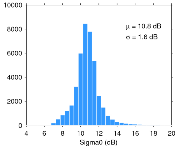
Figure 25. Histogram of flag-valid sigma0 over oceans and lakes for 19/06/2016. The mean ( \mu ) and standard deviation ( \sigma ) are also shown. Note that values outside [4 20] dB are excluded from the histogram for the sake of readability but not from the computation of \mu and \sigma .
