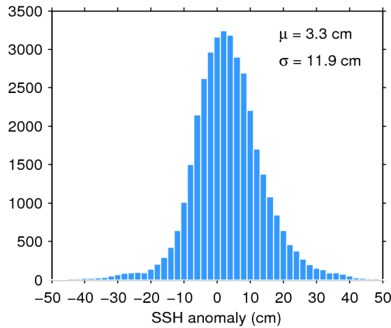
Figure 11. Histogram of science-valid SSH anomaly over oceans and lakes for 19/06/2016. The mean ( \mu ) and standard deviation ( \sigma ) are also shown. Note that values outside [-50 50] cm are excluded from the histogram for the sake of readability but not from the computation of \mu and \sigma .
