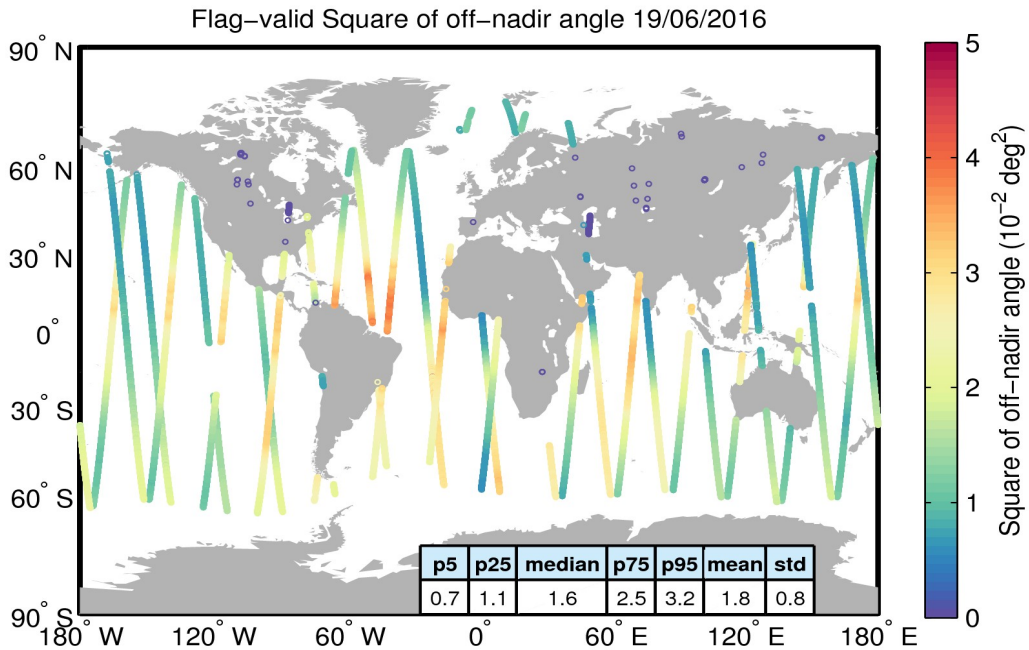
Figure 37. Geographical distribution of flag-valid mispointing data over oceans and lakes for 19/06/2016. The statistical values shown in the table refer to the mispointing in 10^{-2} \text{deg}^2 and are calculated over all measurements shown in the figure.
