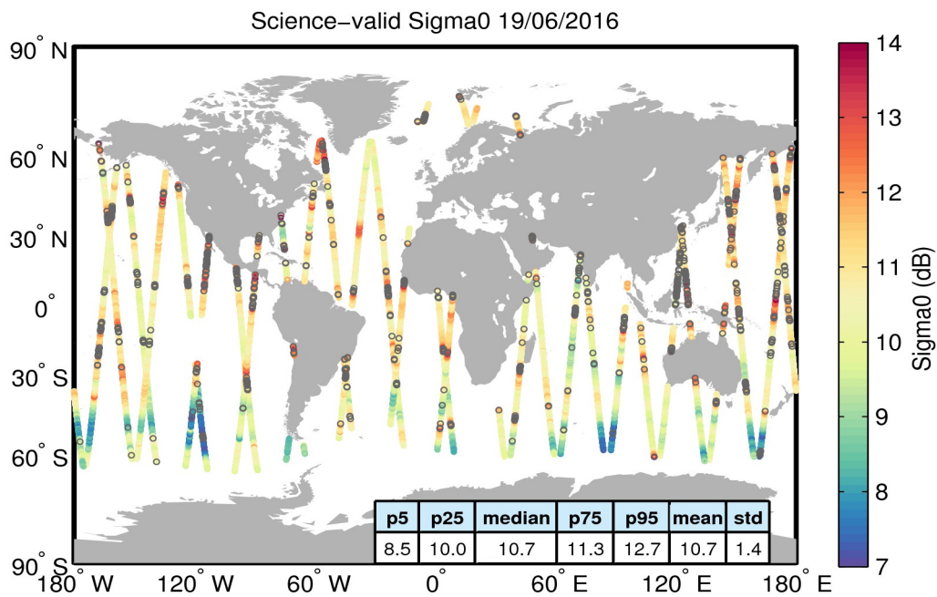
Figure 27. Geographical distribution of science-valid sigma0 data over oceans and lakes for 19/06/2016. The statistical values shown in the table refer to the sigma0 in dB and are calculated over all measurements shown in the figure. Gray circles denote records that have been rejected based on the editing criteria described in Table 4.
