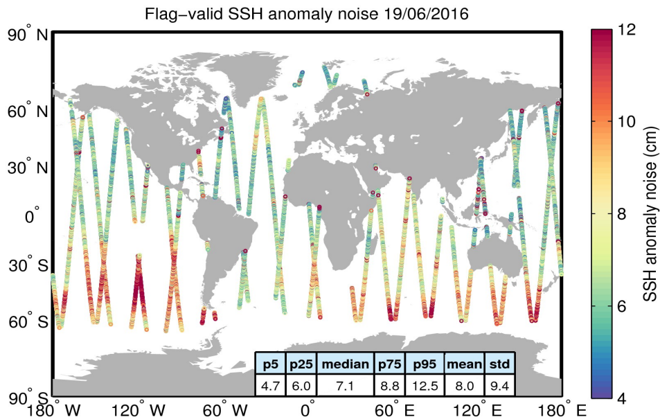
Figure 8. Geographical distribution of flag-valid 20-Hz SSH anomaly measurement noise over oceans and lakes for 19/06/2016. The statistical values shown in the table refer to the SSH anomaly noise and are calculated over all measurements shown in the figure.
