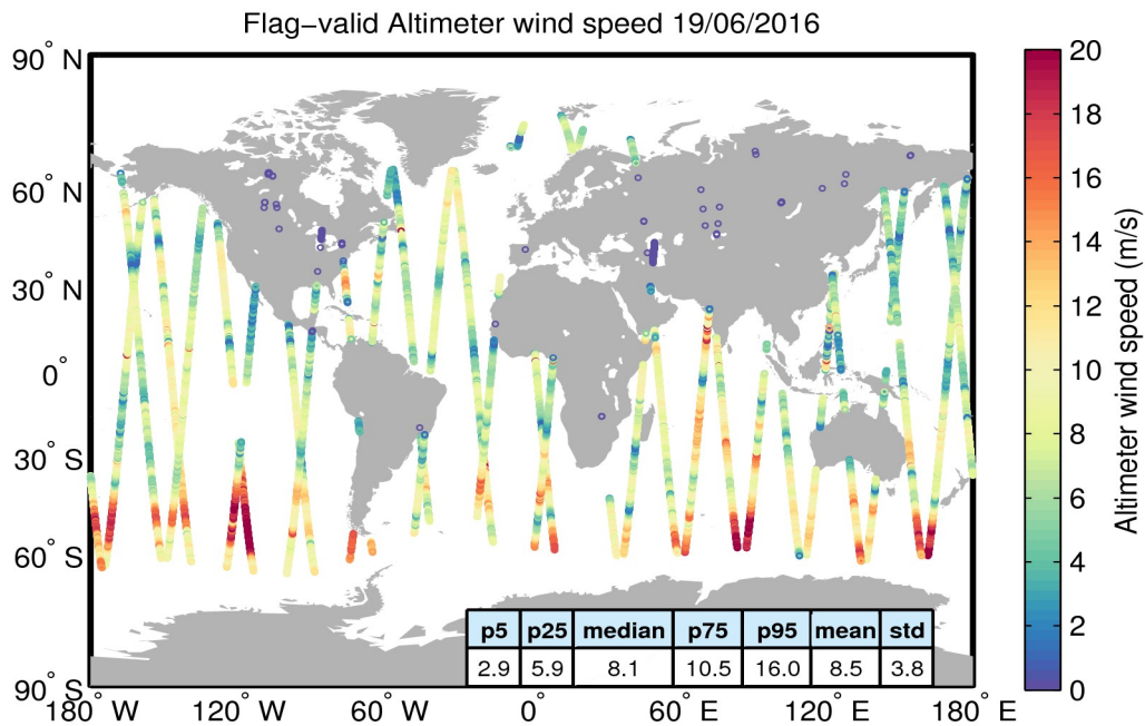
Figure 31. Geographical distribution of flag-valid wind data over oceans and lakes for 19/06/2016. The statistical values shown in the table refer to the wind in m/s and are calculated over all measurements shown in the figure.
