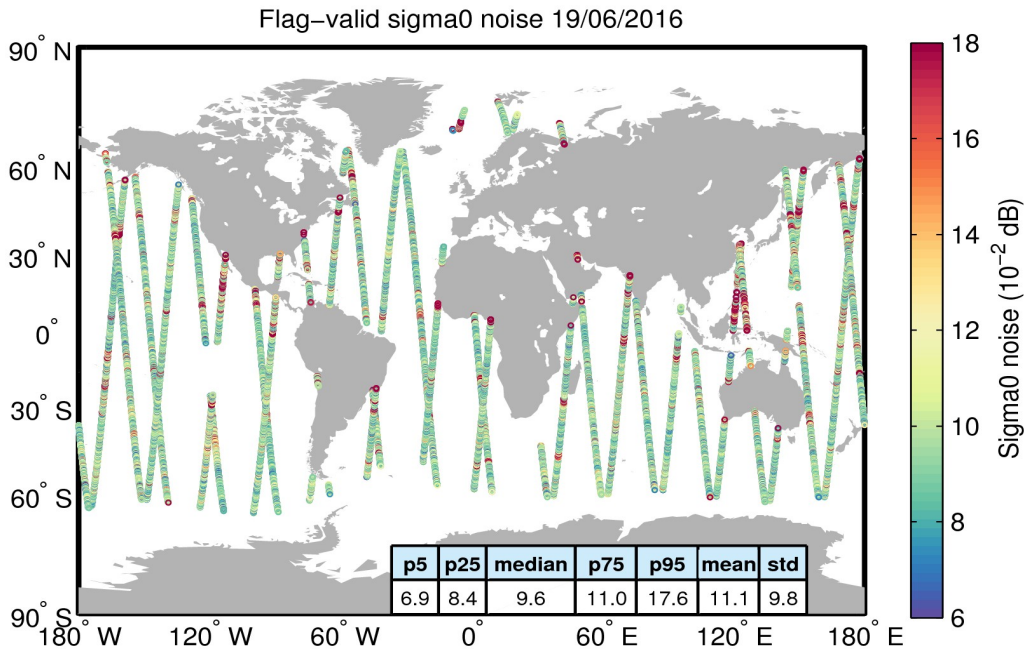
Figure 26. Geographical distribution of flag-valid 20-Hz sigma0 measurement noise over oceans and lakes for 19/06/2016. The statistical values shown in the table refer to the sigma0 noise and are calculated over all measurements shown in the figure.
