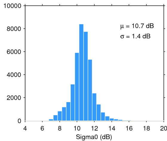
Figure 28. Histogram of science-valid sigma0 over oceans and lakes for 19/06/2016. The mean ( \mu ) and standard deviation ( \sigma ) are also shown. Note that values outside [4 20] dB are excluded from the histogram for the sake of readability but not from the computation of \mu and \sigma .
