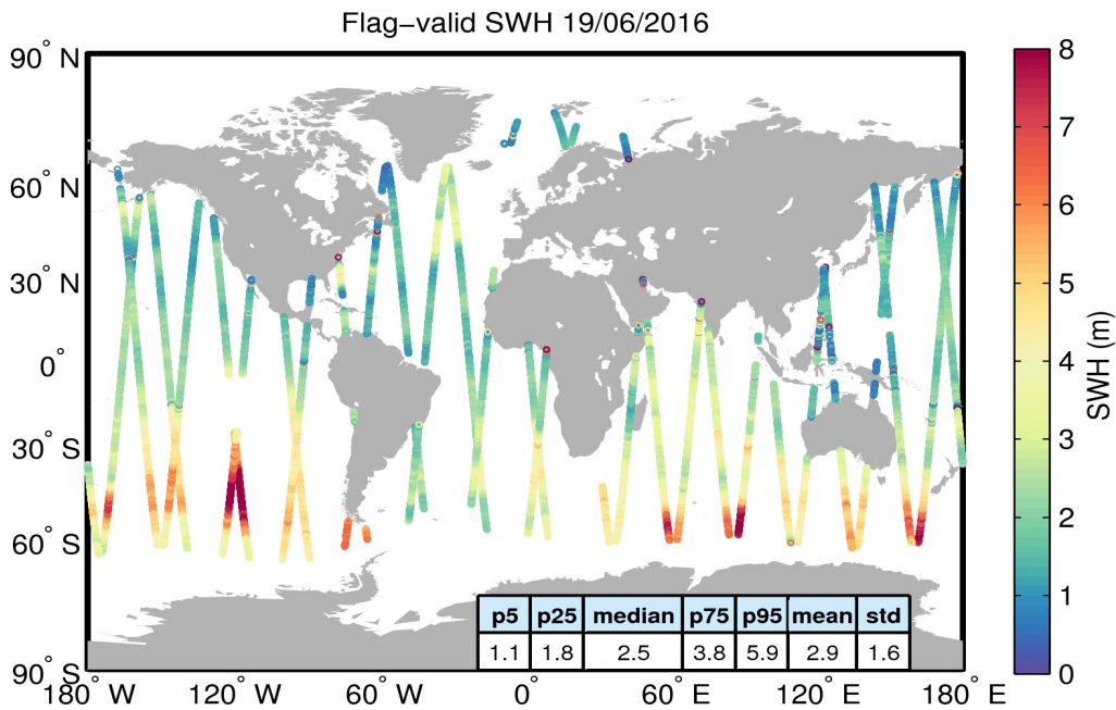
Figure 15. Geographical distribution of flag-valid SWH data over oceans and lakes for 19/06/2016. The statistical values shown in the table refer to the SWH in m and are calculated over all measurements shown in the figure.
