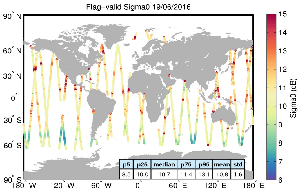
Figure 23. Geographical distribution of flag-valid sigma0 data over oceans and lakes for 19/06/2016. The statistical values shown in the table refer to the sigma0 in dB and are calculated over all measurements shown in the figure.
