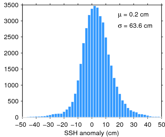
Figure 7. Histogram of flag-valid SSH anomaly over oceans and lakes for 19/06/2016. The mean ( \mu ) and standard deviation ( \sigma ) are also shown. Note that values outside [-50 \ 50] cm are excluded from the histogram for the sake of readability but not from the computation of \mu and \sigma .
