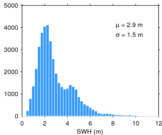
Figure 20. Histogram of science-valid SWH over oceans and lakes for 19/06/2016. The mean ( \mu ) and standard deviation ( \sigma ) are also shown. Note that values larger than 12 m are excluded from the histogram for the sake of readability but not from the computation of \mu and \sigma .
