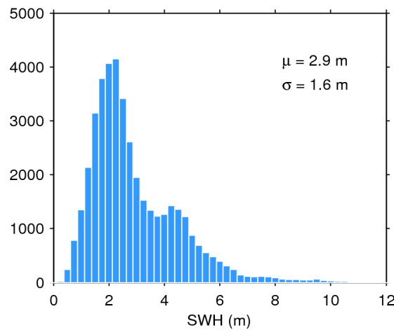
Figure 17. Histogram of flag-valid SWH over oceans and lakes for 19/06/2016. The mean ( \mu ) and standard deviation ( \sigma ) are also shown. Note that values larger than 12 m are excluded from the histogram for the sake of readability but not from the computation of \mu and \sigma .
