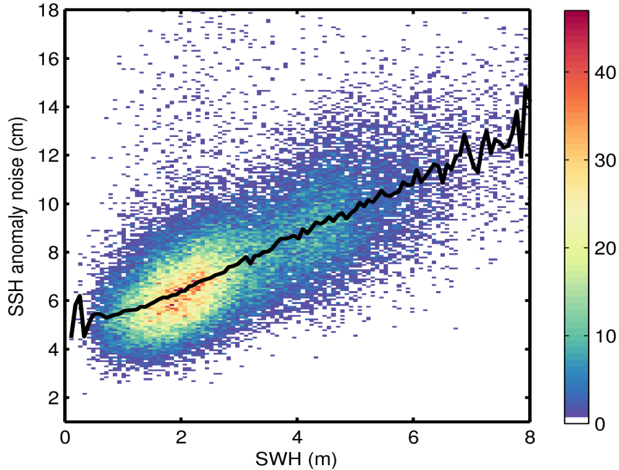
Figure 9. 2D histogram showing flag-valid SSH anomaly noise as a function of SWH for 19/06/2016. The black line denotes the median SSH anomaly noise as a function of SWH.
