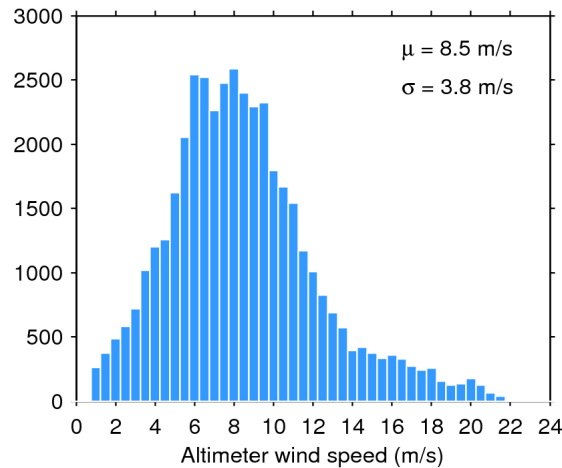
Figure 33. Histogram of flag-valid wind over oceans and lakes for 19/06/2016. The mean ( \mu ) and standard deviation ( \sigma ) are also shown. Note that values larger than 24 m/s are excluded from the histogram for the sake of readability but not from the computation of \mu and \sigma .
