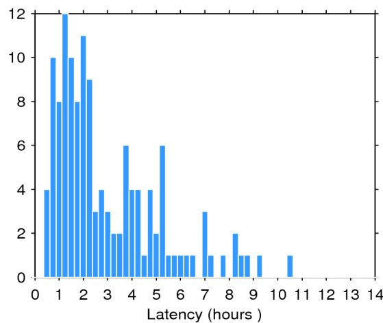
Figure 2. Histogram of the data latency for 19/06/2016. The y-axis denotes the number of files that are made available with a delay of x-hours with respect to the mean time of the records stored in the file.
