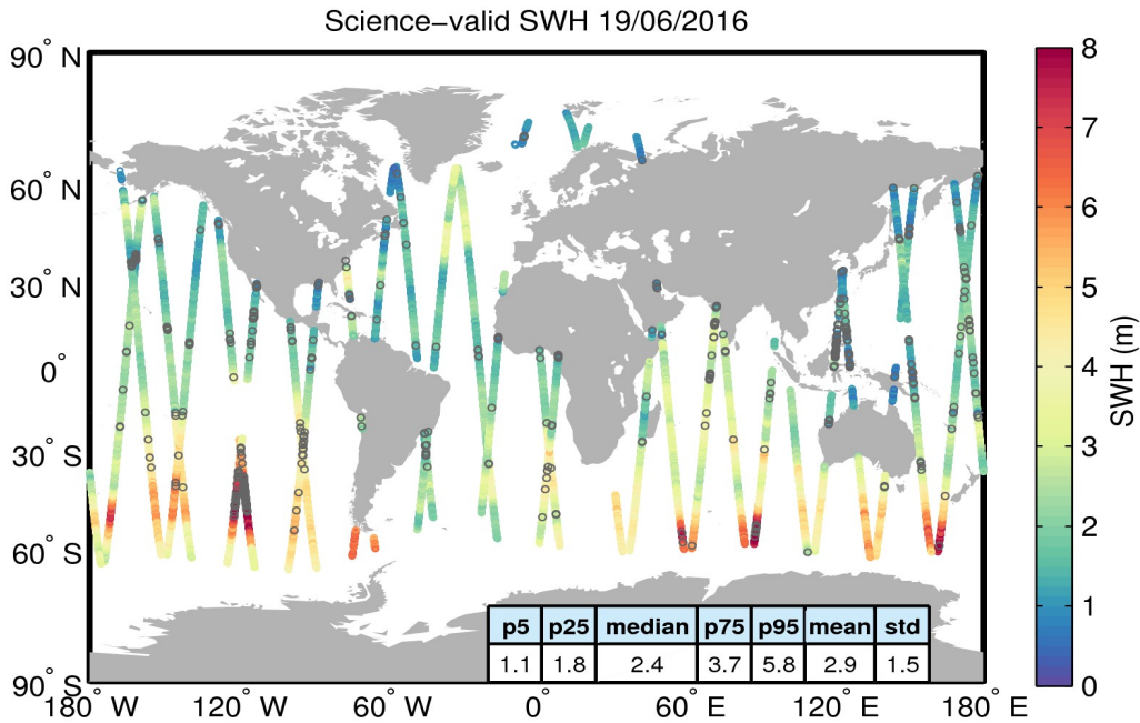
Figure 19. Geographical distribution of science-valid SWH data over oceans and lakes for 19/06/2016. The statistical values shown in the table refer to the SWH in m and are calculated over all measurements shown in the figure. Gray circles denote records that have been rejected based on the editing criteria described in Table 3.
