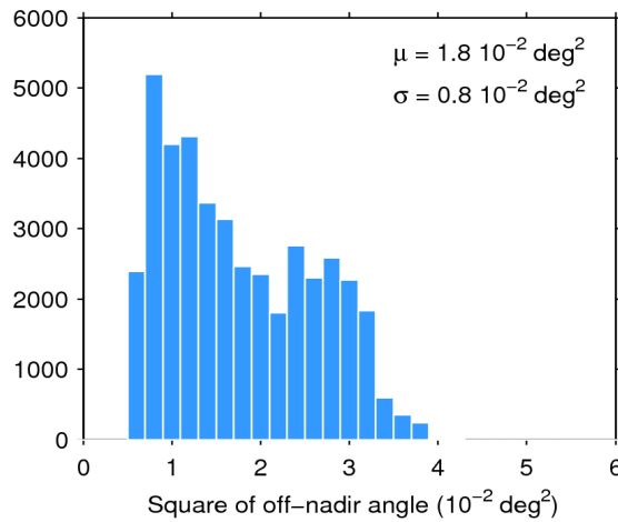
Figure 39. Histogram of flag-valid mispointing over oceans and lakes for 19/06/2016. The mean ( \mu ) and standard deviation ( \sigma ) are also shown. Note that values larger than 6 \cdot 10^{-2} \text{ deg}^2 are excluded from the histogram for the sake of readability but not from the computation of \mu and \sigma .
