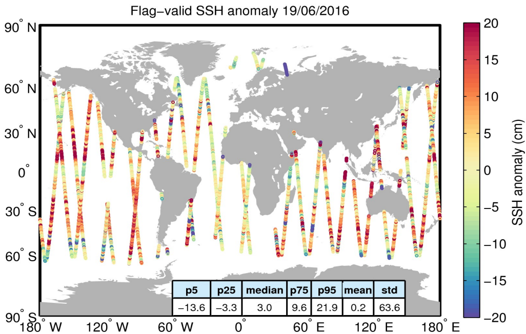
Figure 5. Geographical distribution of flag-valid 1-Hz SSH anomaly data over oceans and lakes for 19/06/2016. The statistical values shown in the table refer to the SSH anomaly in cm and are calculated over all measurements shown in the figure.
