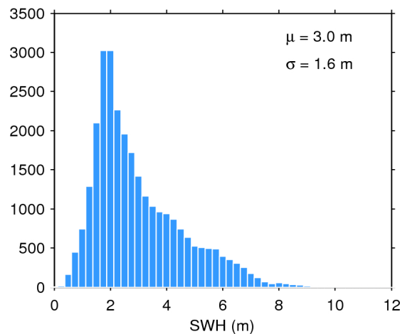
Figure 20. Histogram of science-valid SWH over oceans and lakes for 18/06/2016. The mean ( \mu ) and standard deviation ( \sigma ) are also shown. Note that values larger than 12 m are excluded from the histogram for the sake of readability but not from the computation of \mu and \sigma .
