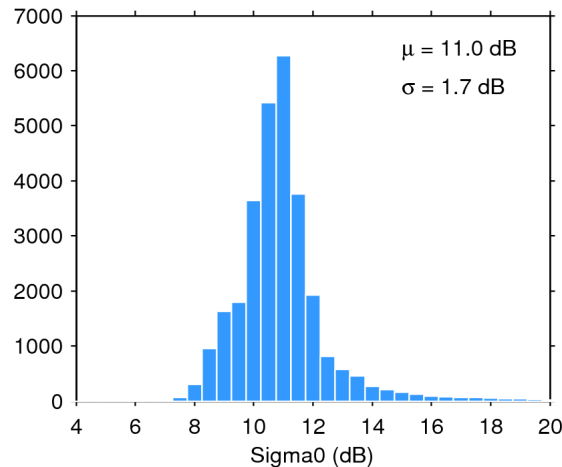
Figure 25. Histogram of flag-valid sigma0 over oceans and lakes for 18/06/2016. The mean ( \mu ) and standard deviation ( \sigma ) are also shown. Note that values outside [4 20] dB are excluded from the histogram for the sake of readability but not from the computation of \mu and \sigma .
