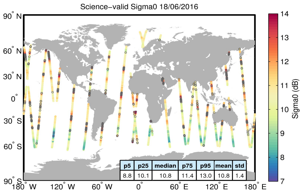
Figure 27. Geographical distribution of science-valid sigma0 data over oceans and lakes for 18/06/2016. The statistical values shown in the table refer to the sigma0 in dB and are calculated over all measurements shown in the figure. Gray circles denote records that have been rejected based on the editing criteria described in Table 4.
