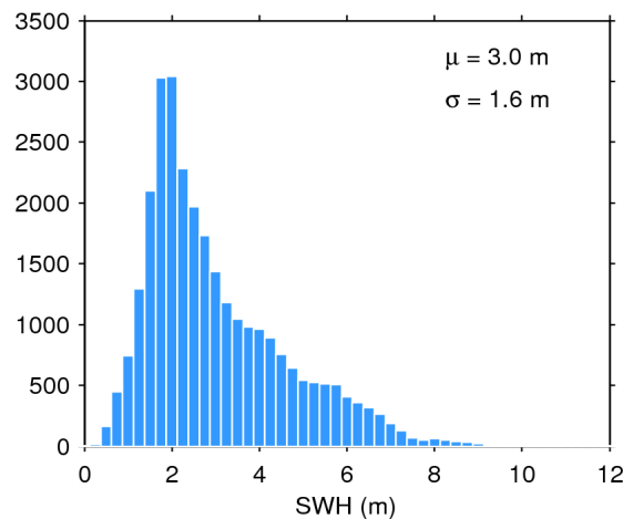
Figure 17. Histogram of flag-valid SWH over oceans and lakes for 18/06/2016. The mean ( \mu ) and standard deviation ( \sigma ) are also shown. Note that values larger than 12 m are excluded from the histogram for the sake of readability but not from the computation of \mu and \sigma .
