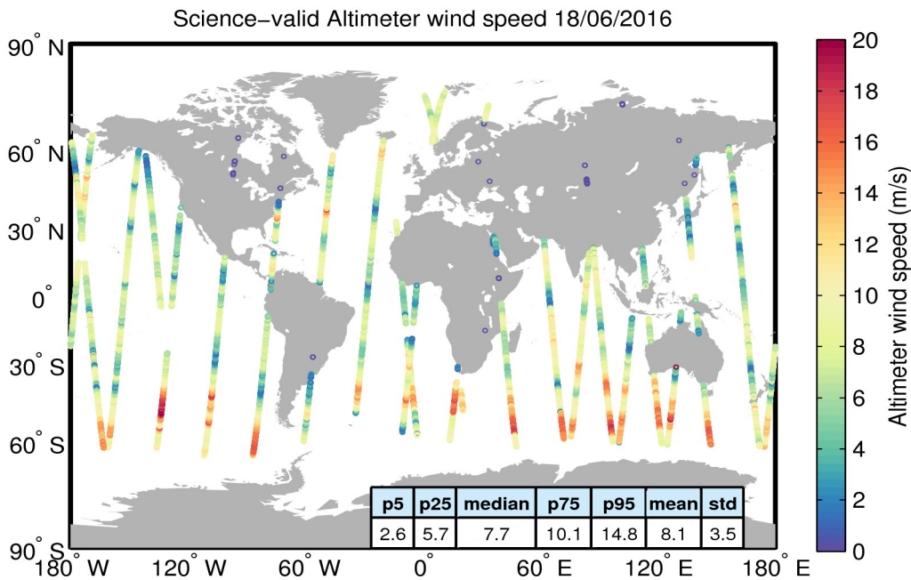
Figure 34. Geographical distribution of science-valid wind data over oceans and lakes for 18/06/2016. The statistical values shown in the table refer to the wind in m/s and are calculated over all measurements shown in the figure. Gray circles denote records that have been rejected based on the editing criteria described in Table 5.
