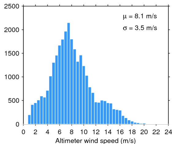
Figure 35. Histogram of science-valid wind over oceans and lakes for 18/06/2016. The mean ( \mu ) and standard deviation ( \sigma ) are also shown. Note that values larger than 24 m/s are excluded from the histogram for the sake of readability but not from the computation of \mu and \sigma .
