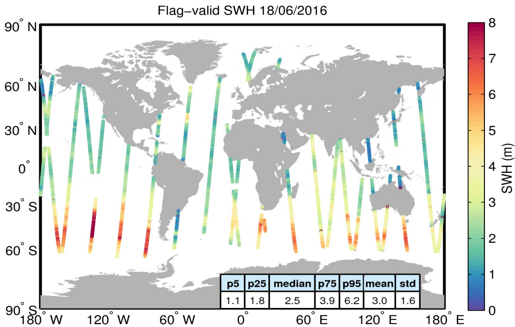
Figure 15. Geographical distribution of flag-valid SWH data over oceans and lakes for 18/06/2016. The statistical values shown in the table refer to the SWH in m and are calculated over all measurements shown in the figure.
