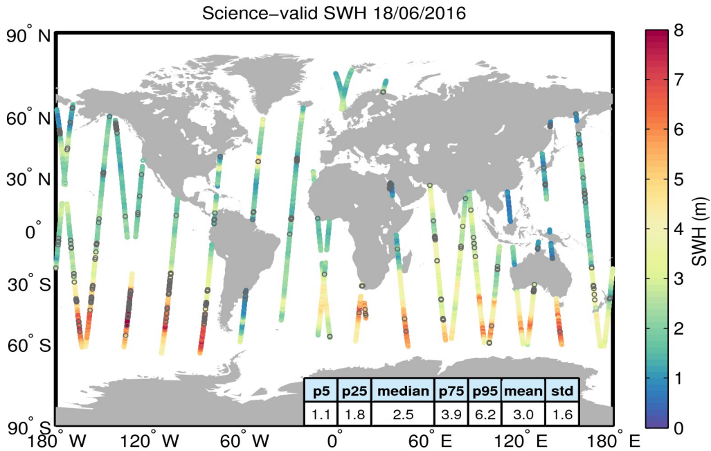
Figure 19. Geographical distribution of science-valid SWH data over oceans and lakes for 18/06/2016. The statistical values shown in the table refer to the SWH in m and are calculated over all measurements shown in the figure. Gray circles denote records that have been rejected based on the editing criteria described in Table 3.
