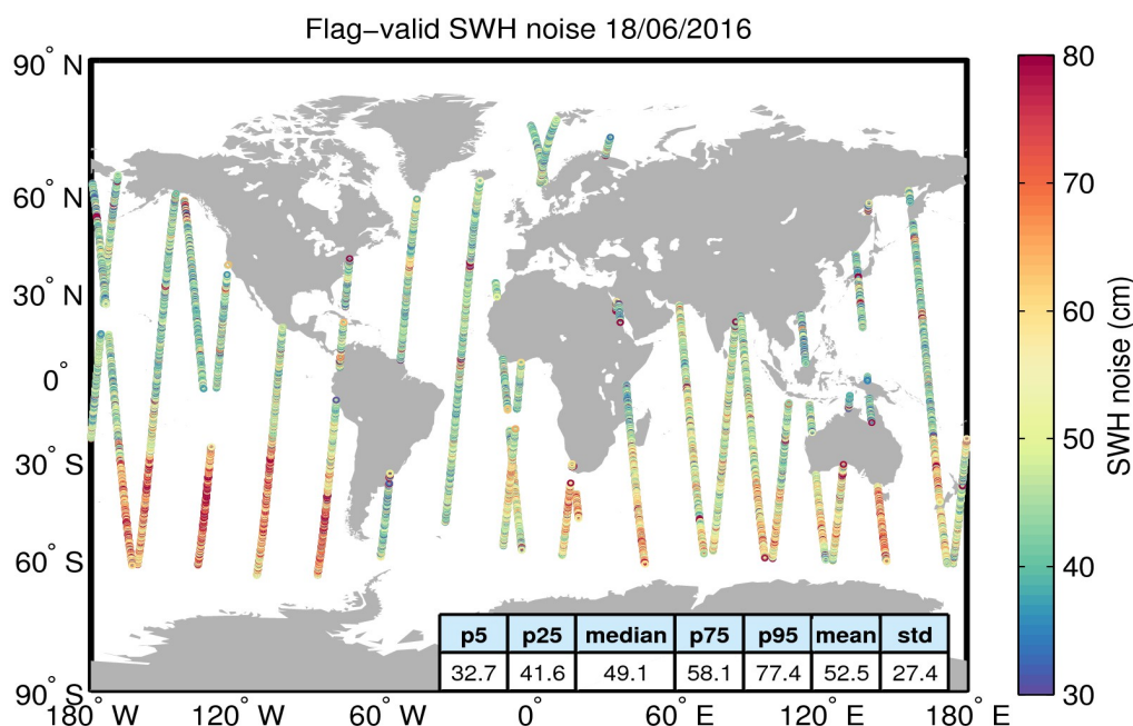
Figure 18. Geographical distribution of flag-valid 20-Hz SWH measurement noise over oceans and lakes for 18/06/2016. The statistical values shown in the figure refer to the SWH noise and are calculated over all measurements shown in the figure.
