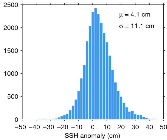
Figure 11. Histogram of science-valid SSH anomaly over oceans and lakes for 18/06/2016. The mean ( \mu ) and standard deviation ( \sigma ) are also shown. Note that values outside [-50 50] cm are excluded from the histogram for the sake of readability but not from the computation of \mu and \sigma .
