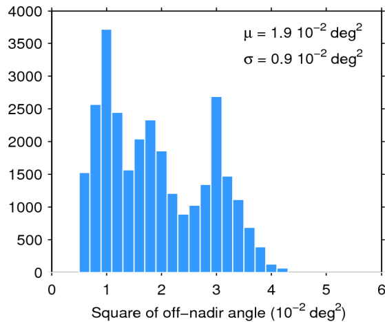
Figure 39. Histogram of flag-valid mispointing over oceans and lakes for 18/06/2016. The mean ( \mu ) and standard deviation ( \sigma ) are also shown. Note that values larger than 6 \cdot 10^{-2} \text{ deg}^2 are excluded from the histogram for the sake of readability but not from the computation of \mu and \sigma .
