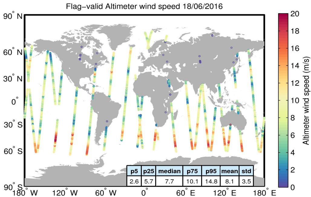
Figure 31. Geographical distribution of flag-valid wind data over oceans and lakes for 18/06/2016. The statistical values shown in the table refer to the wind in m/s and are calculated over all measurements shown in the figure.
