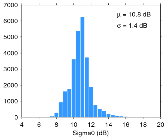
Figure 28. Histogram of science-valid sigma0 over oceans and lakes for 18/06/2016. The mean ( \mu ) and standard deviation ( \sigma ) are also shown. Note that values outside [4 20] dB are excluded from the histogram for the sake of readability but not from the computation of \mu and \sigma .
