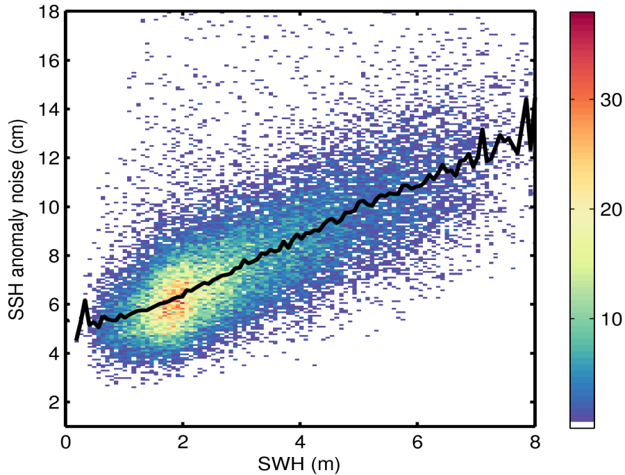
Figure 9. 2D histogram showing flag-valid SSH anomaly noise as a function of SWH for 18/06/2016. The black line denotes the median SSH anomaly noise as a function of SWH.
