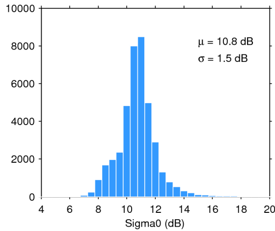
Figure 28. Histogram of science-valid sigma0 over oceans and lakes for 17/06/2016. The mean ( \mu ) and standard deviation ( \sigma ) are also shown. Note that values outside [4 20] dB are excluded from the histogram for the sake of readability but not from the computation of \mu and \sigma .
