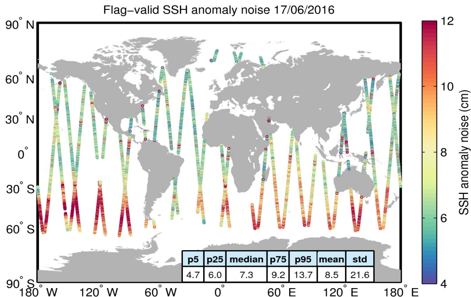
Figure 8. Geographical distribution of flag-valid 20-Hz SSH anomaly measurement noise over oceans and lakes for 17/06/2016. The statistical values shown in the table refer to the SSH anomaly noise and are calculated over all measurements shown in the figure.
