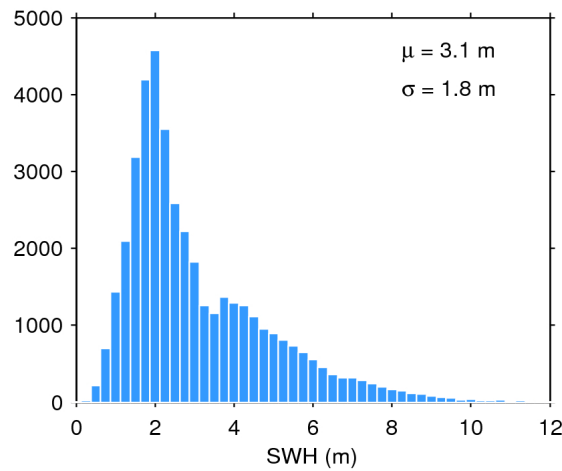
Figure 17. Histogram of flag-valid SWH over oceans and lakes for 17/06/2016. The mean ( \mu ) and standard deviation ( \sigma ) are also shown. Note that values larger than 12 m are excluded from the histogram for the sake of readability but not from the computation of \mu and \sigma .
