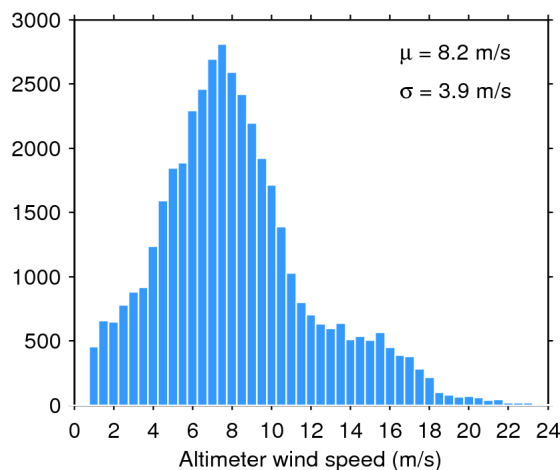
Figure 35. Histogram of science-valid wind over oceans and lakes for 17/06/2016. The mean ( \mu ) and standard deviation ( \sigma ) are also shown. Note that values larger than 24 m/s are excluded from the histogram for the sake of readability but not from the computation of \mu and \sigma .
