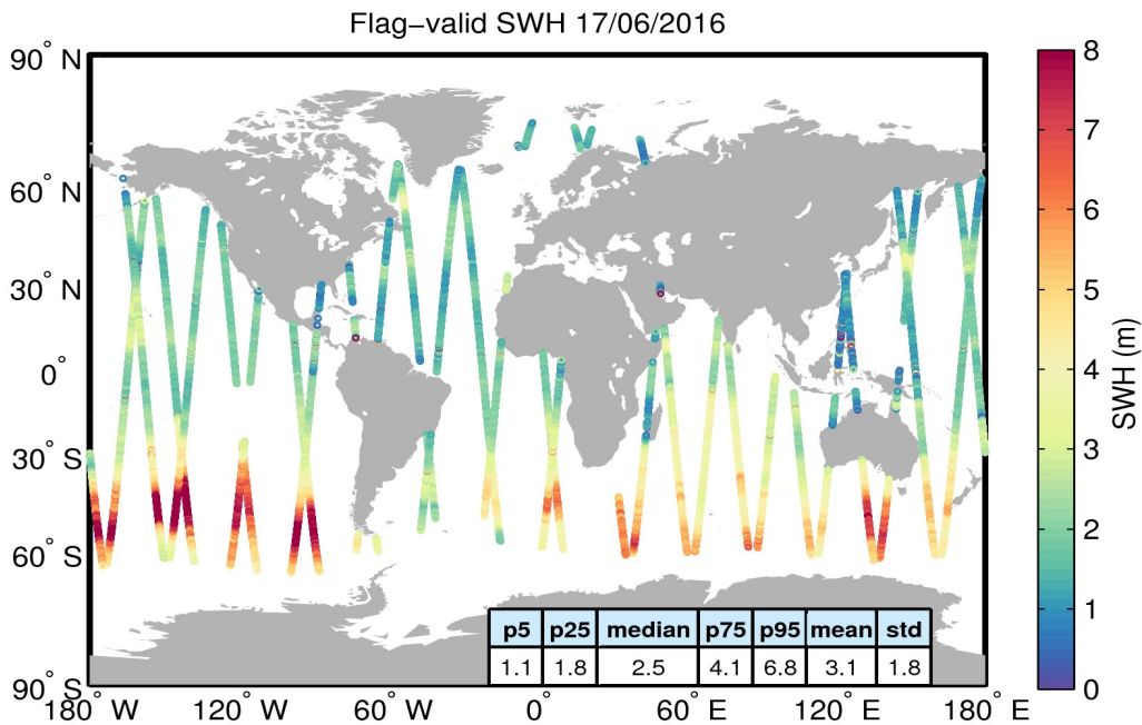
Figure 15. Geographical distribution of flag-valid SWH data over oceans and lakes for 17/06/2016. The statistical values shown in the table refer to the SWH in m and are calculated over all measurements shown in the figure.
