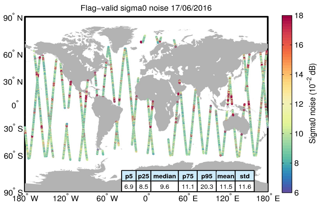
Figure 26. Geographical distribution of flag-valid 20-Hz sigma0 measurement noise over oceans and lakes for 17/06/2016. The statistical values shown in the table refer to the sigma0 noise and are calculated over all measurements shown in the figure.
