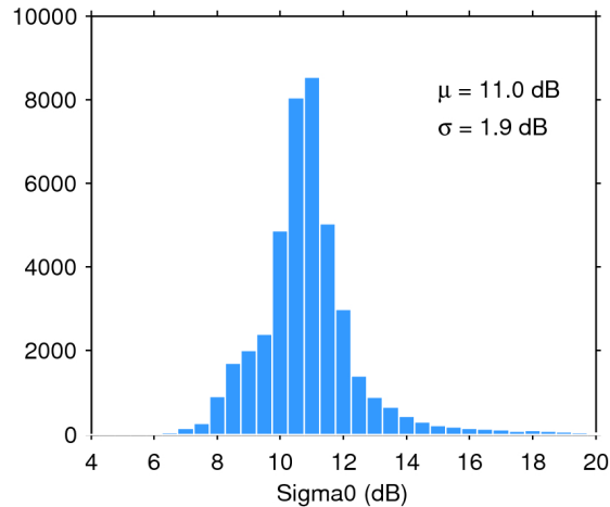
Figure 25. Histogram of flag-valid sigma0 over oceans and lakes for 17/06/2016. The mean ( \mu ) and standard deviation ( \sigma ) are also shown. Note that values outside [4 20] dB are excluded from the histogram for the sake of readability but not from the computation of \mu and \sigma .
