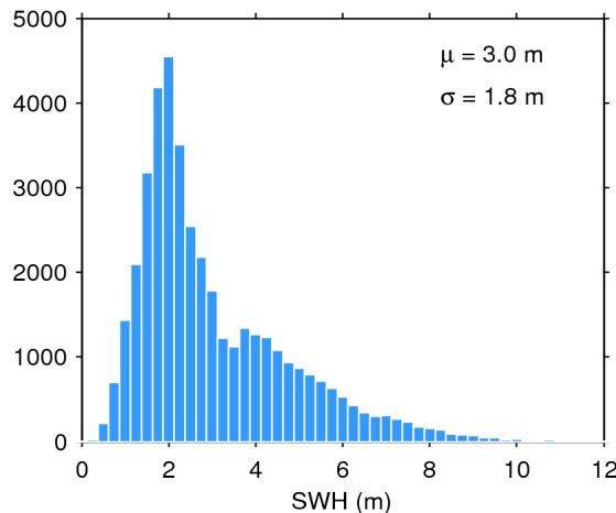
Figure 20. Histogram of science-valid SWH over oceans and lakes for 17/06/2016. The mean ( \mu ) and standard deviation ( \sigma ) are also shown. Note that values larger than 12 m are excluded from the histogram for the sake of readability but not from the computation of \mu and \sigma .
