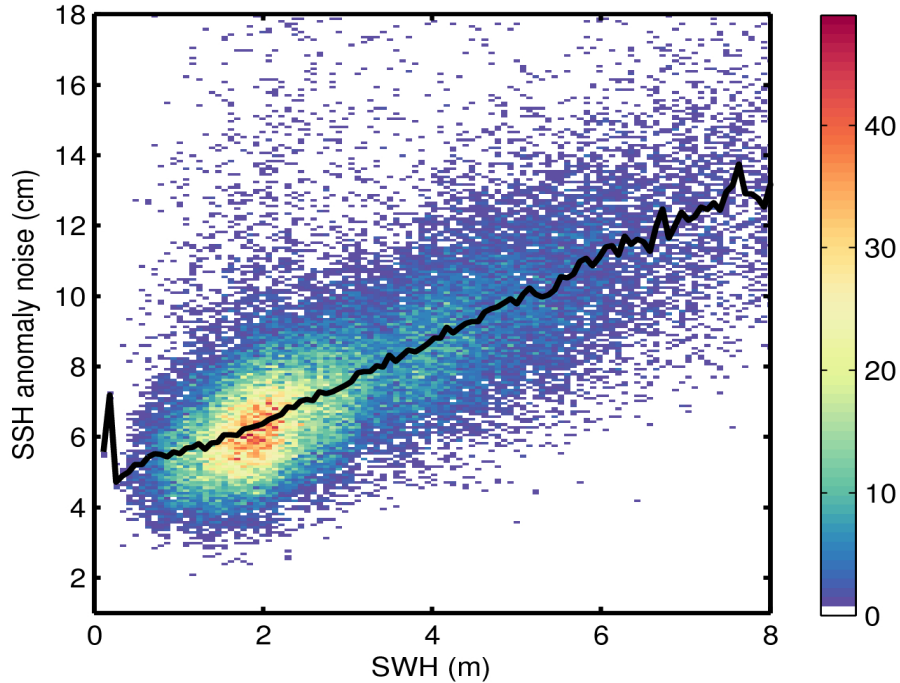
Figure 9. 2D histogram showing flag-valid SSH anomaly noise as a function of SWH for 17/06/2016. The black line denotes the median SSH anomaly noise as a function of SWH.
