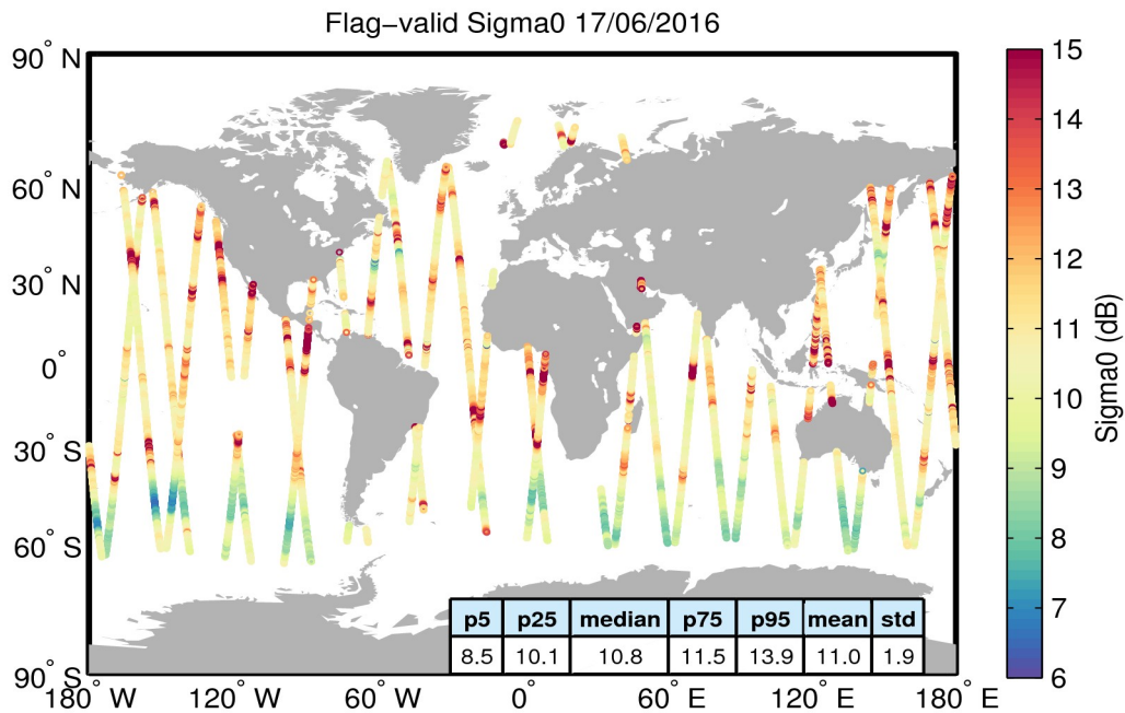
Figure 23. Geographical distribution of flag-valid sigma0 data over oceans and lakes for 17/06/2016. The statistical values shown in the table refer to the sigma0 in dB and are calculated over all measurements shown in the figure.
