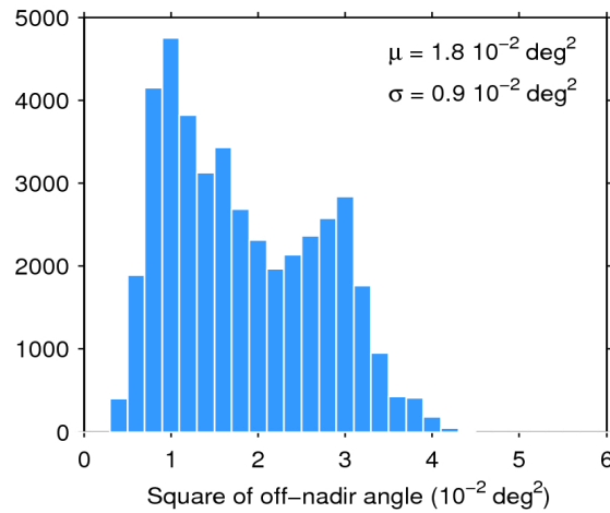
Figure 39. Histogram of flag-valid mispointing over oceans and lakes for 17/06/2016. The mean ( \mu ) and standard deviation ( \sigma ) are also shown. Note that values larger than 6 \cdot 10^{-2} \text{ deg}^2 are excluded from the histogram for the sake of readability but not from the computation of \mu and \sigma .
