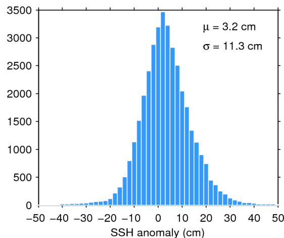
Figure 11. Histogram of science-valid SSH anomaly over oceans and lakes for 17/06/2016. The mean ( \mu ) and standard deviation ( \sigma ) are also shown. Note that values outside [-50 50] cm are excluded from the histogram for the sake of readability but not from the computation of \mu and \sigma .
